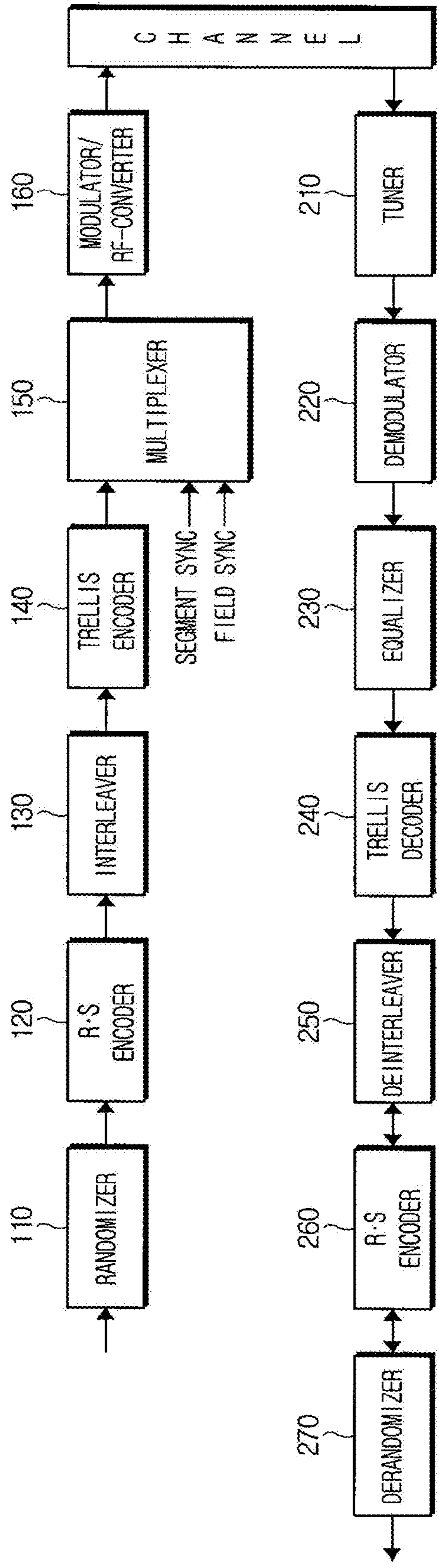
FIG. 1 (PRIOR ART)
