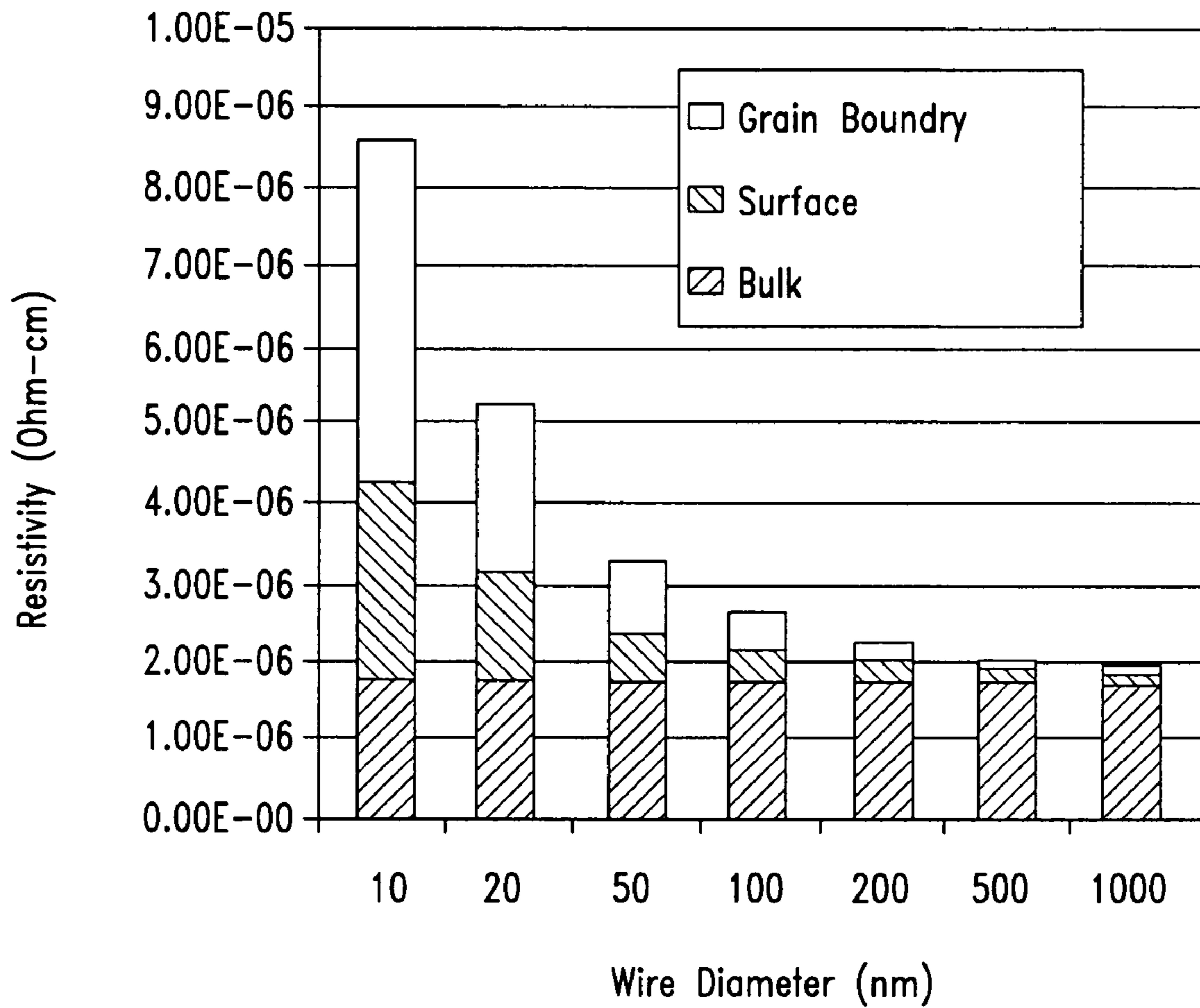
Effects of Surface Scattering and Grain Boundries on Resistance
