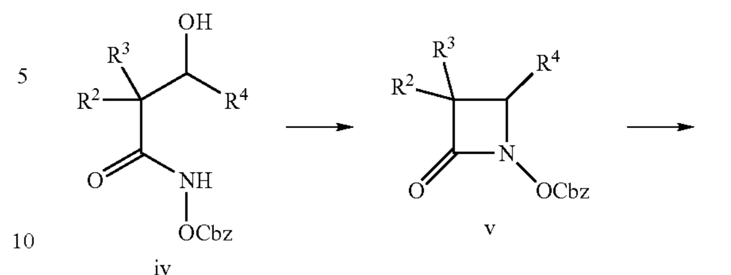
Synthetic Scheme II
