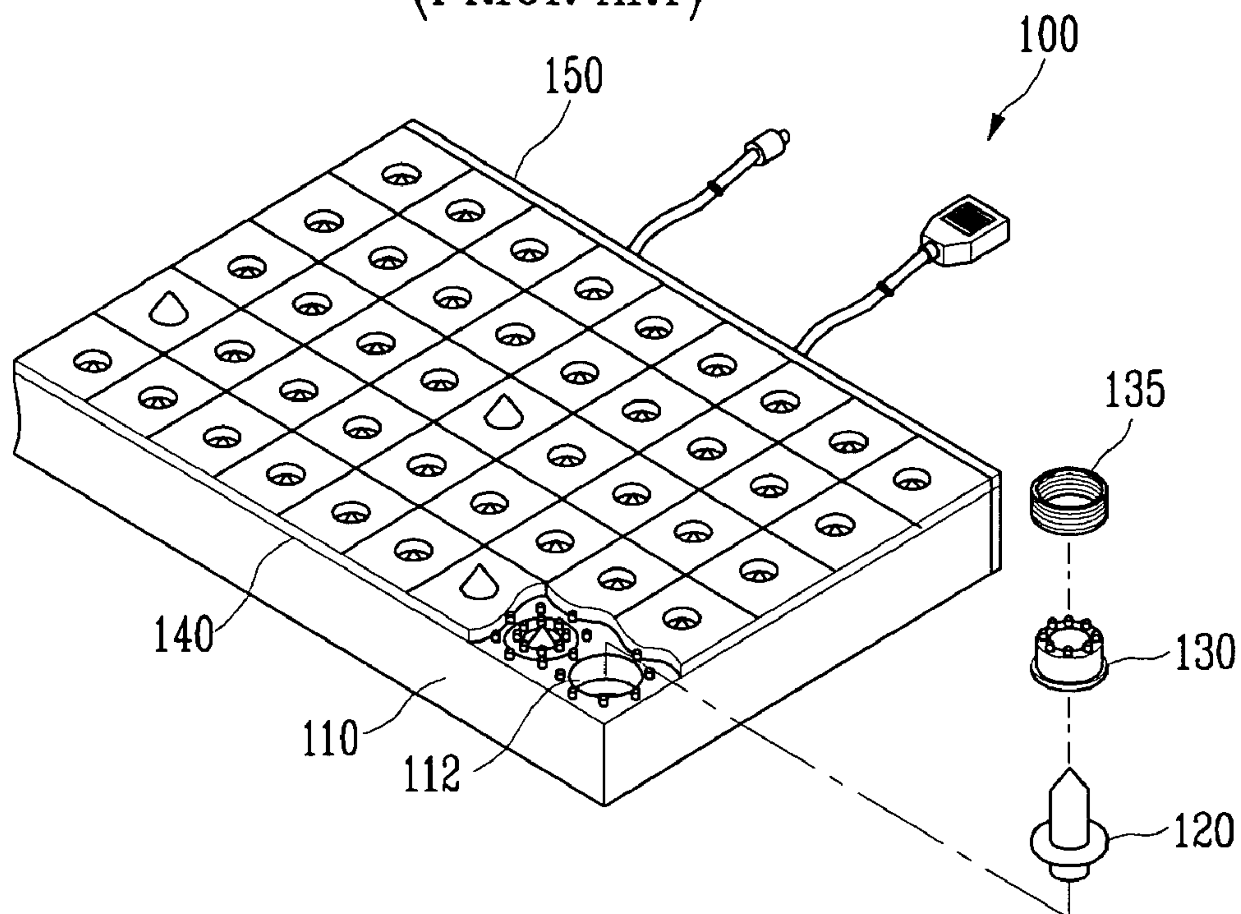
FIG. 1 (PRIOR ART)
