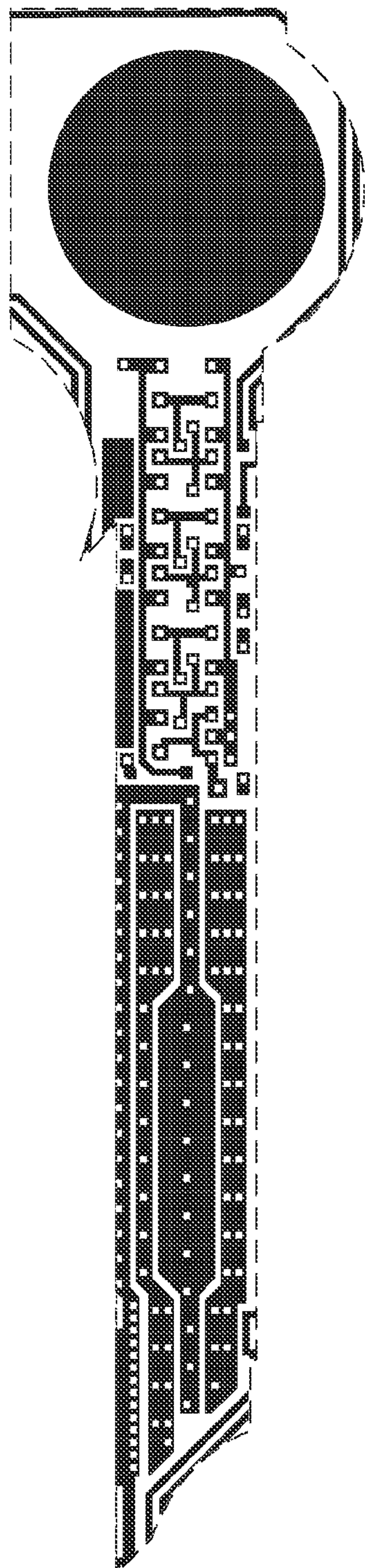
Metal 1 mask
