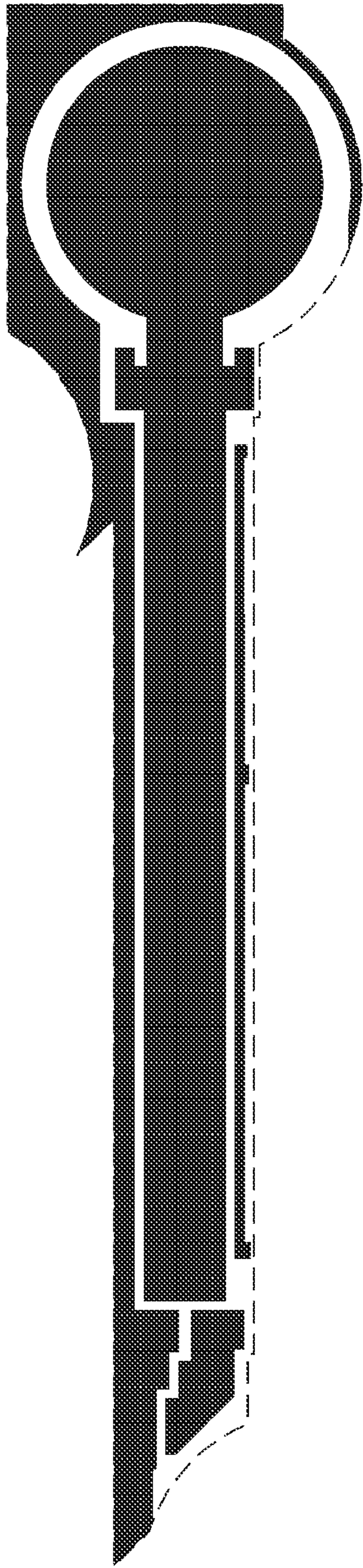
Metal 3 mask
