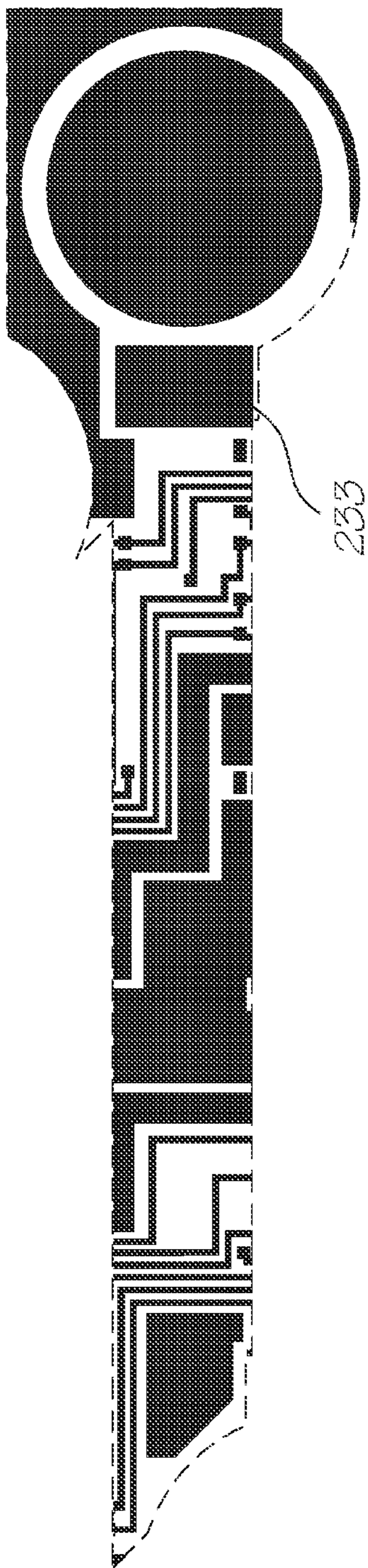
Metal 2 mask
