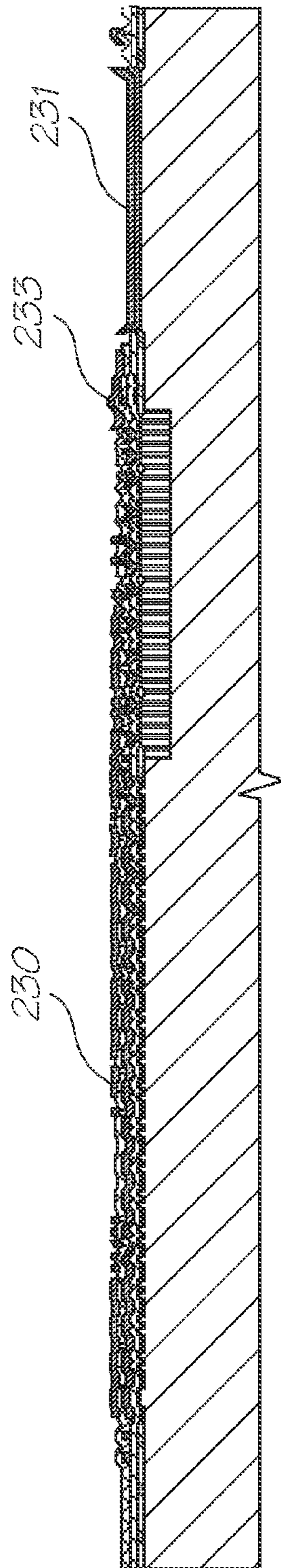
Deposit metal 2
