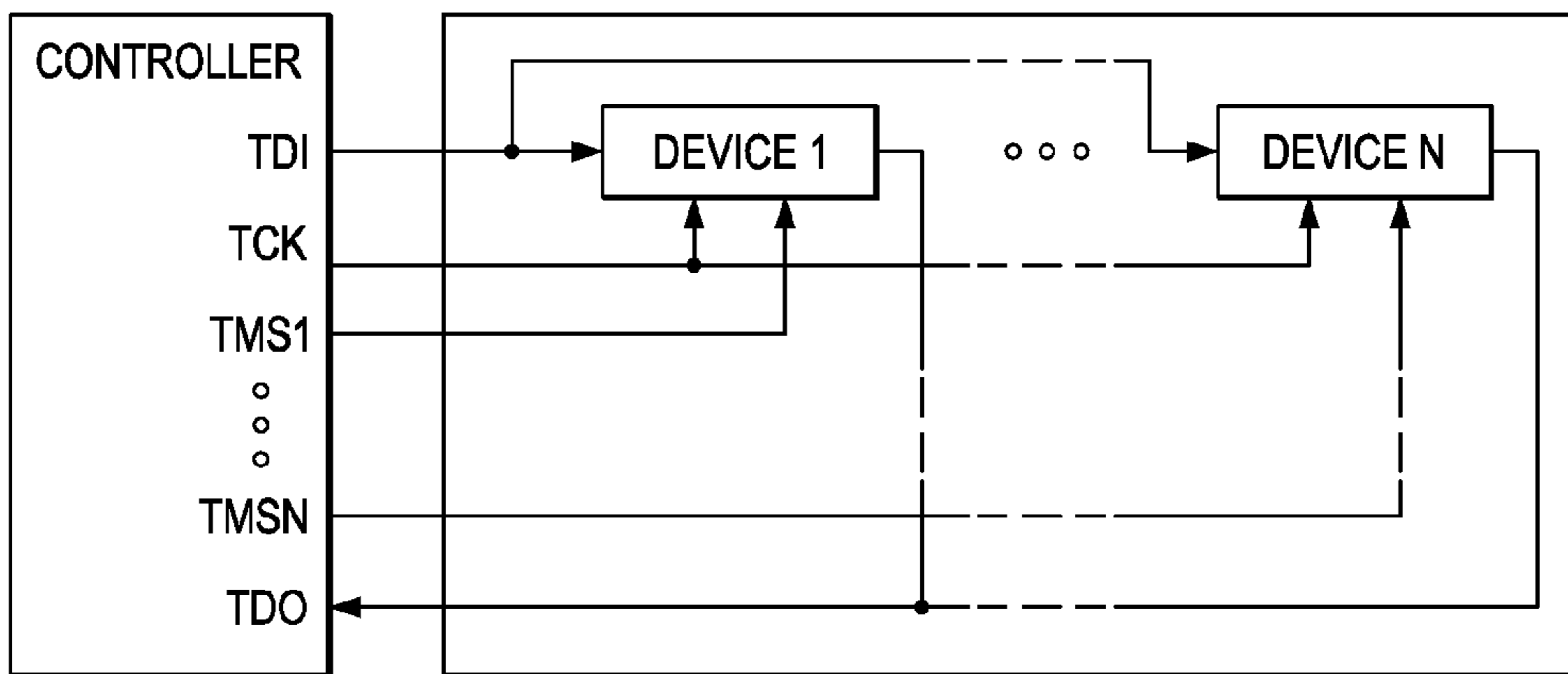
FIG. 5 (PRIOR ART)
