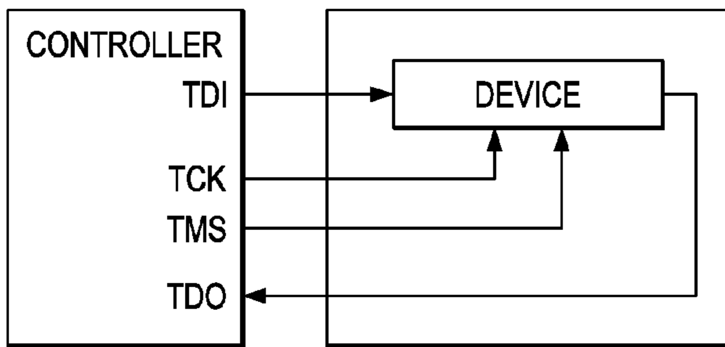
FIG. 4 (PRIOR ART)
