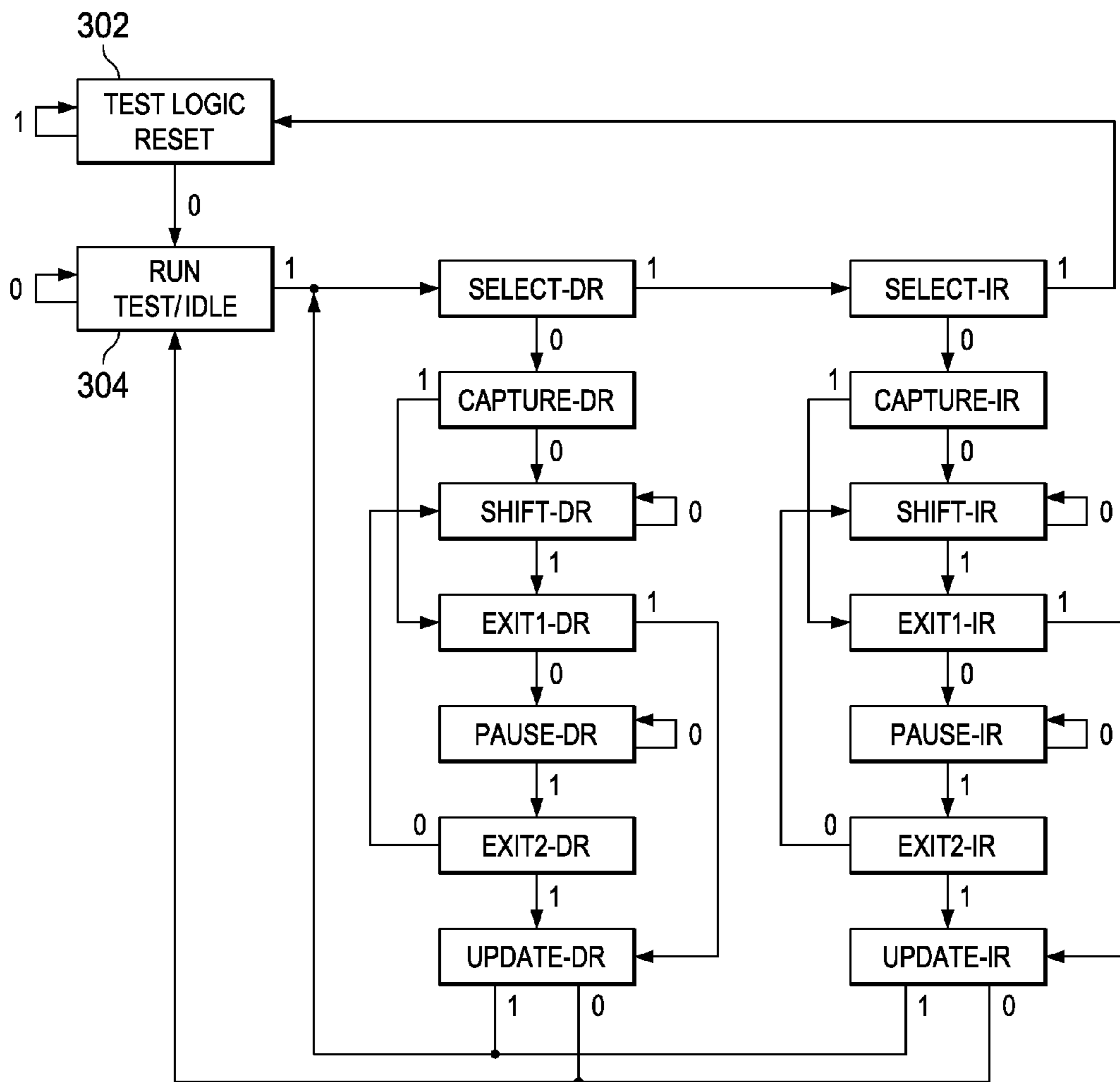
FIG. 3 (PRIOR ART)
