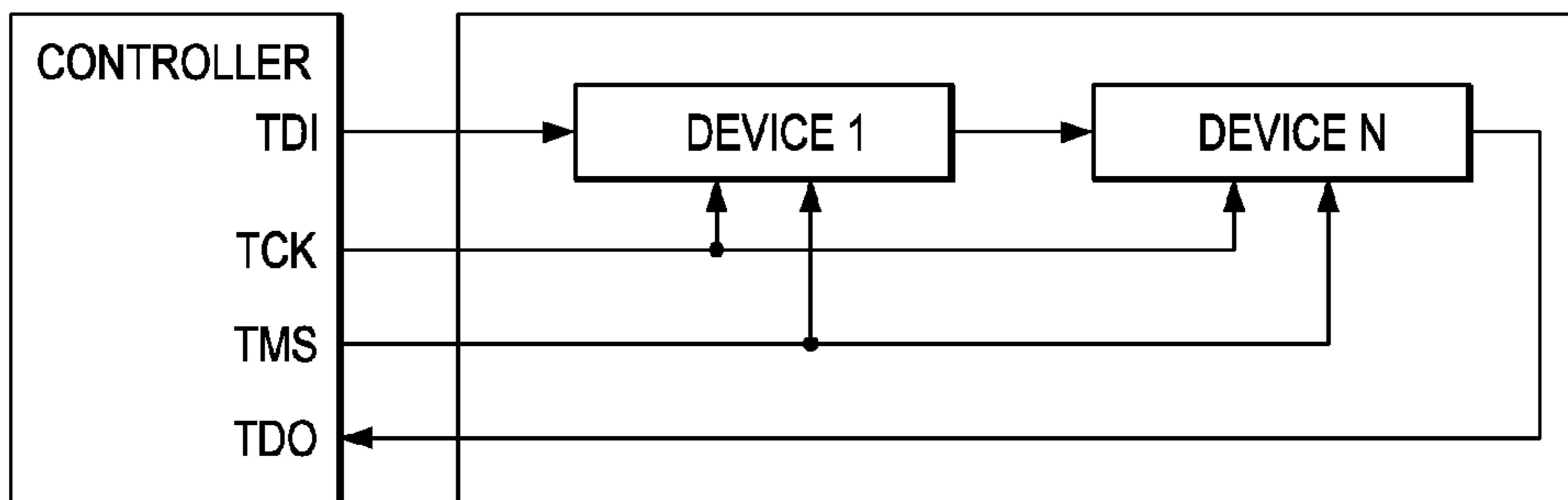
FIG. 6 (PRIOR ART)
