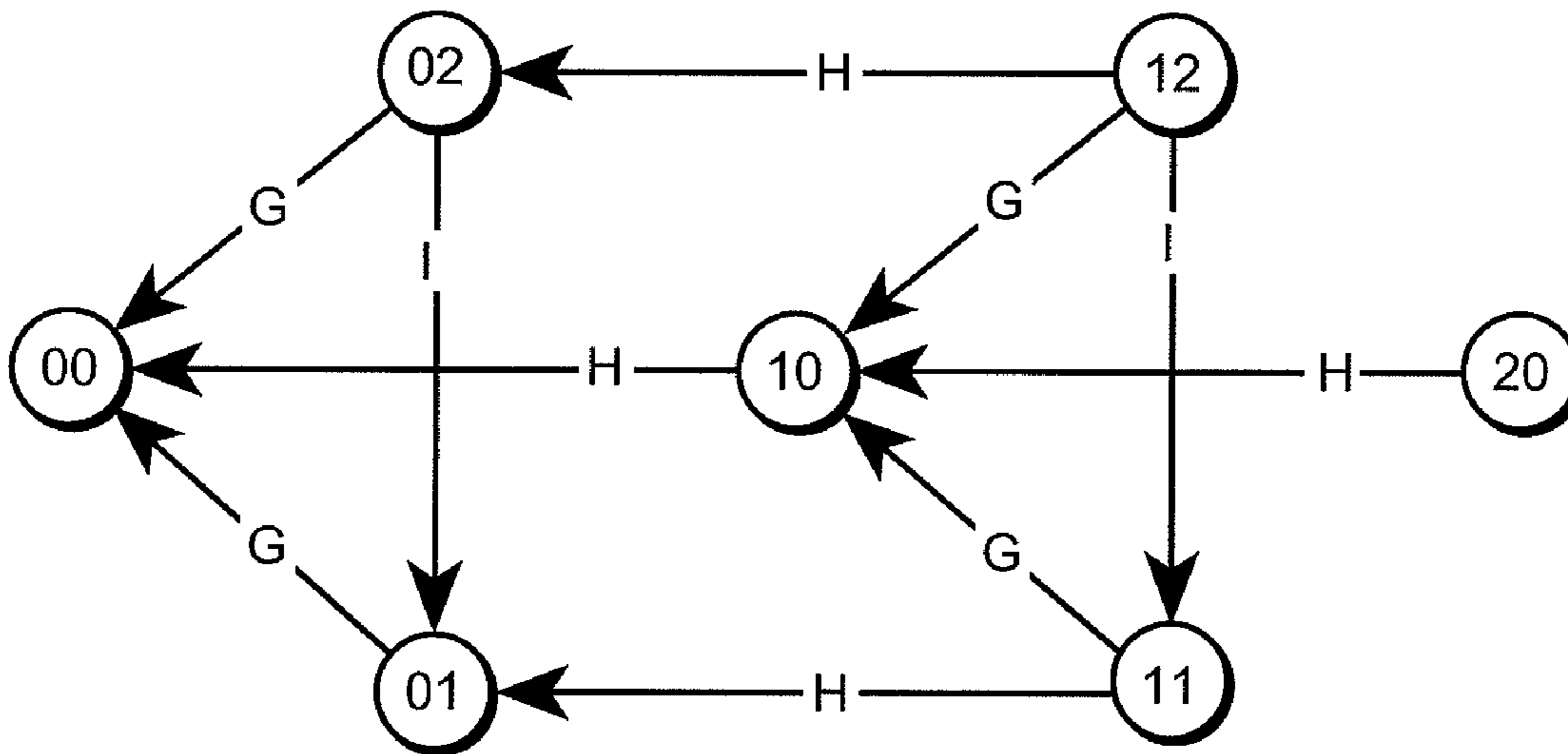
File State Transitions Due to Obsolete Data
