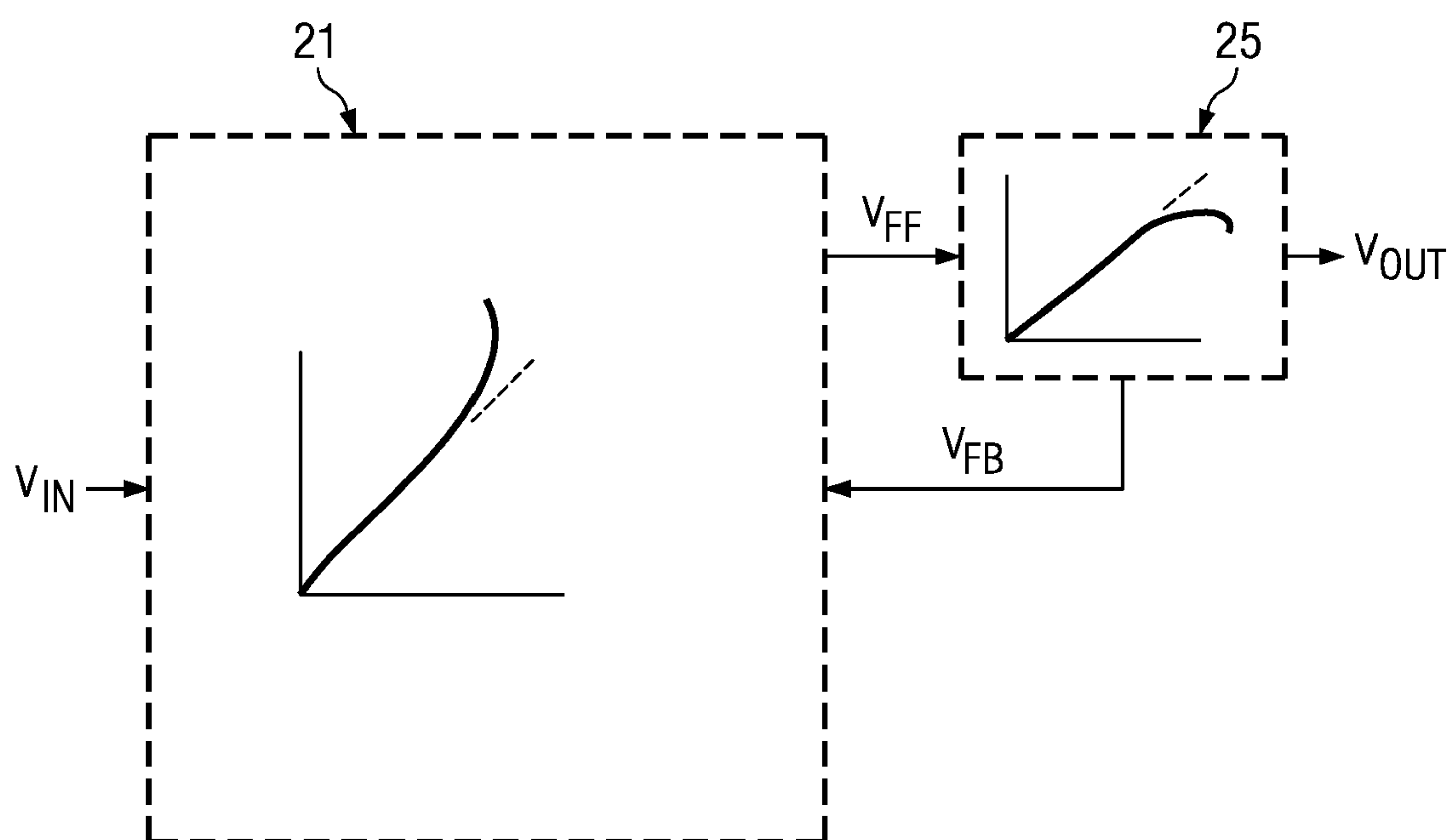
FIG. 4 (PRIOR ART)
