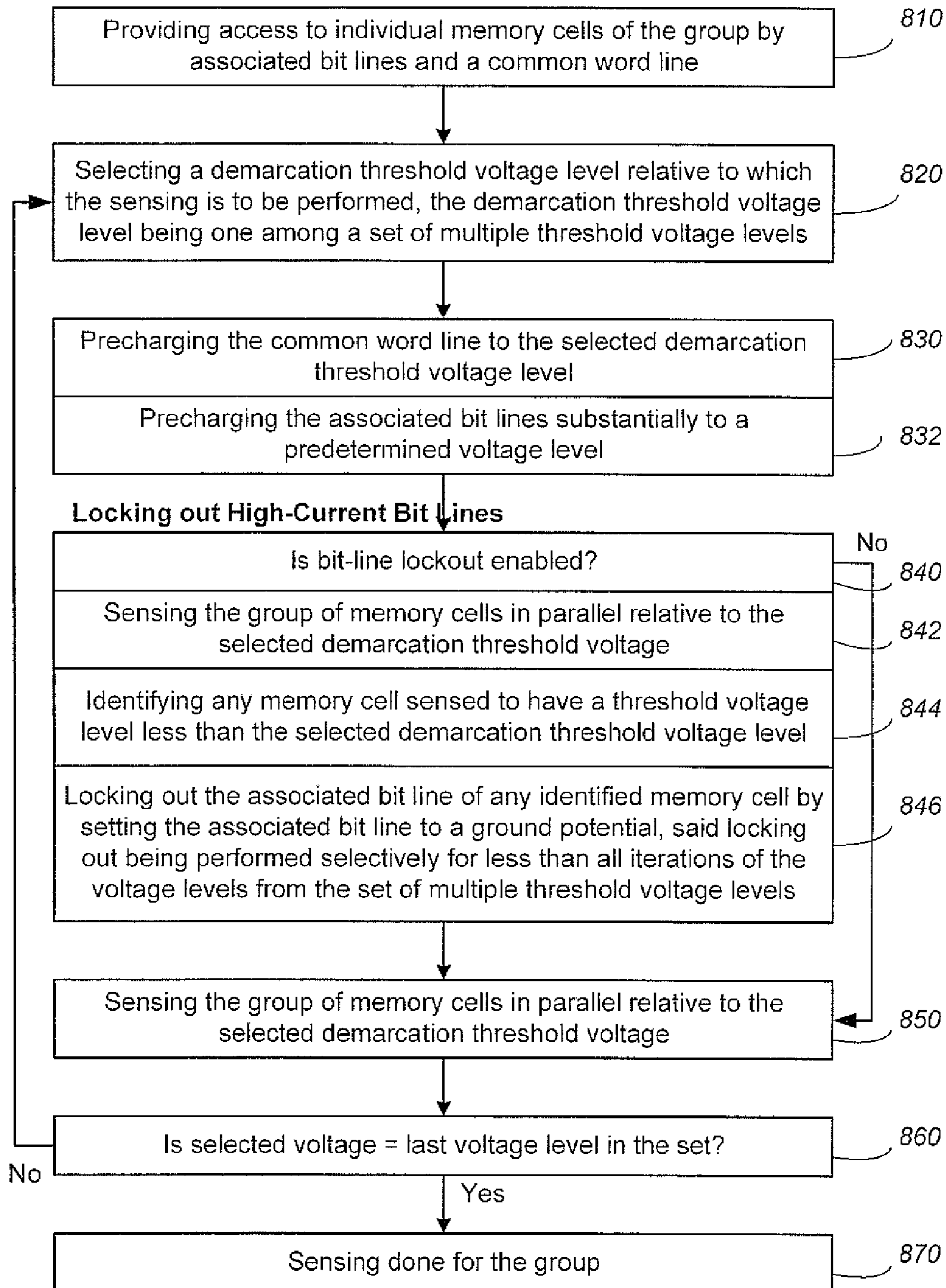
Sensing with Bit-line Lockout Control
