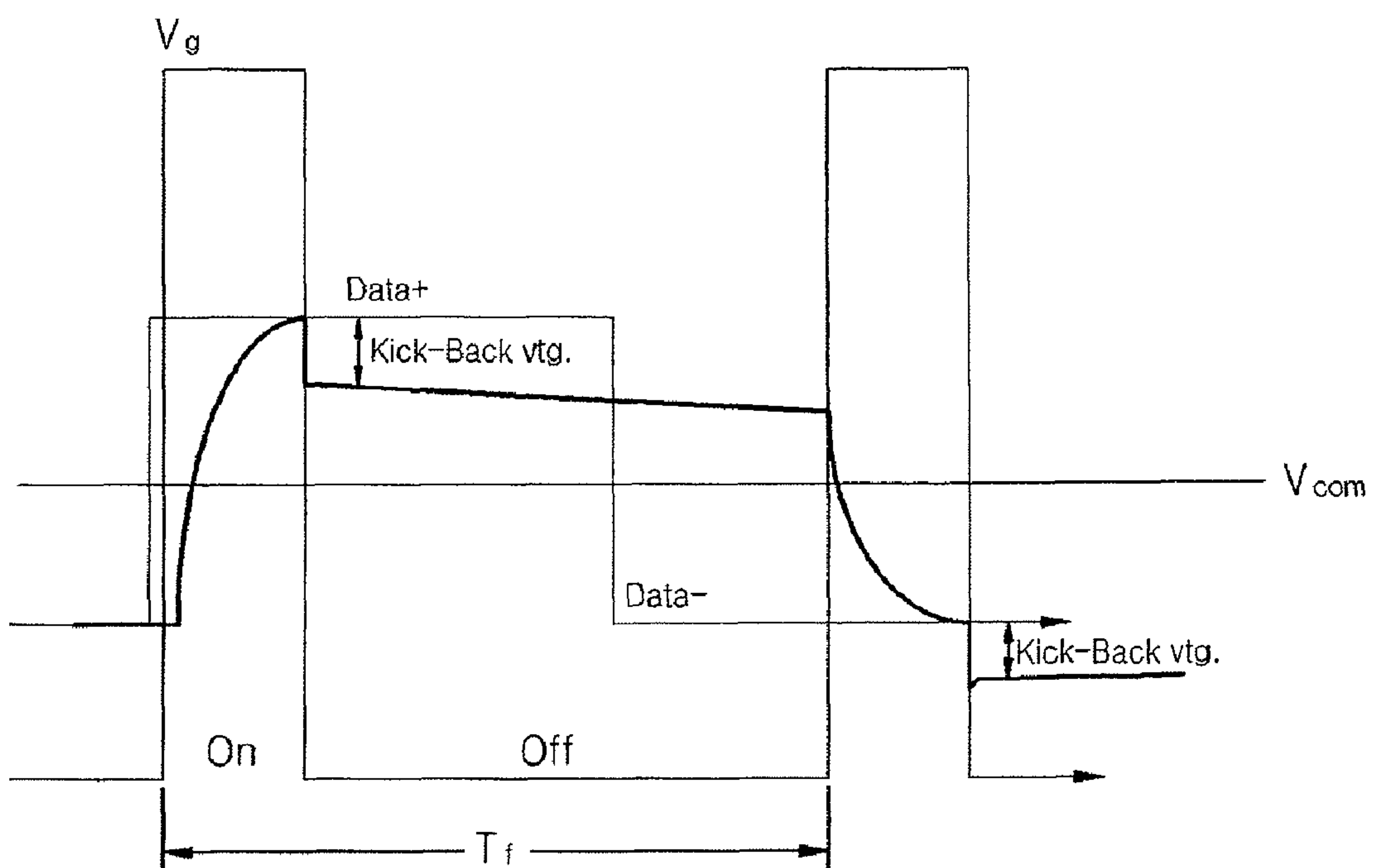
FIG. 2 (PRIOR ART)
