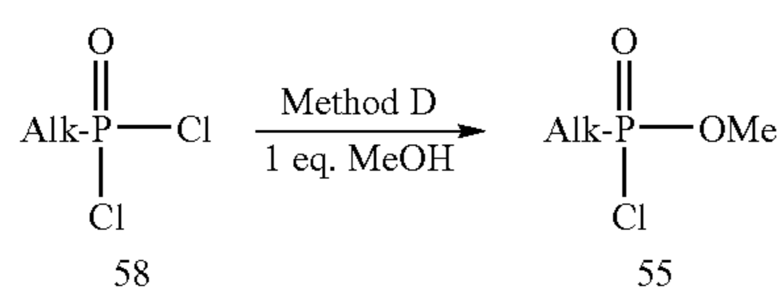
Scheme 14: Alkyl Phosphinates
