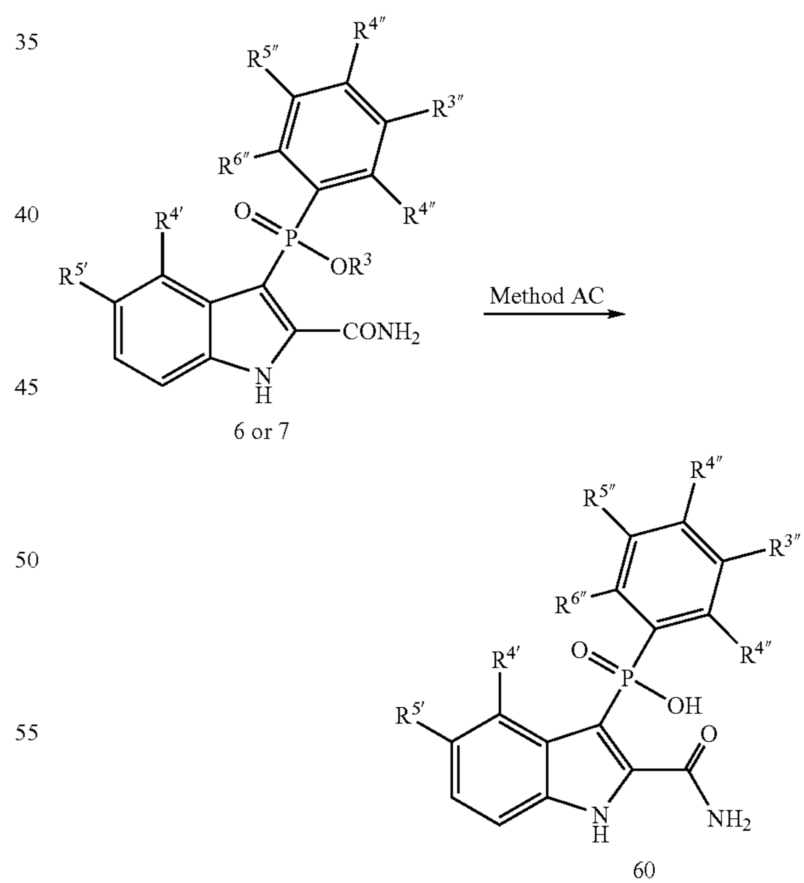
Scheme 16: Phosphinic Acids
