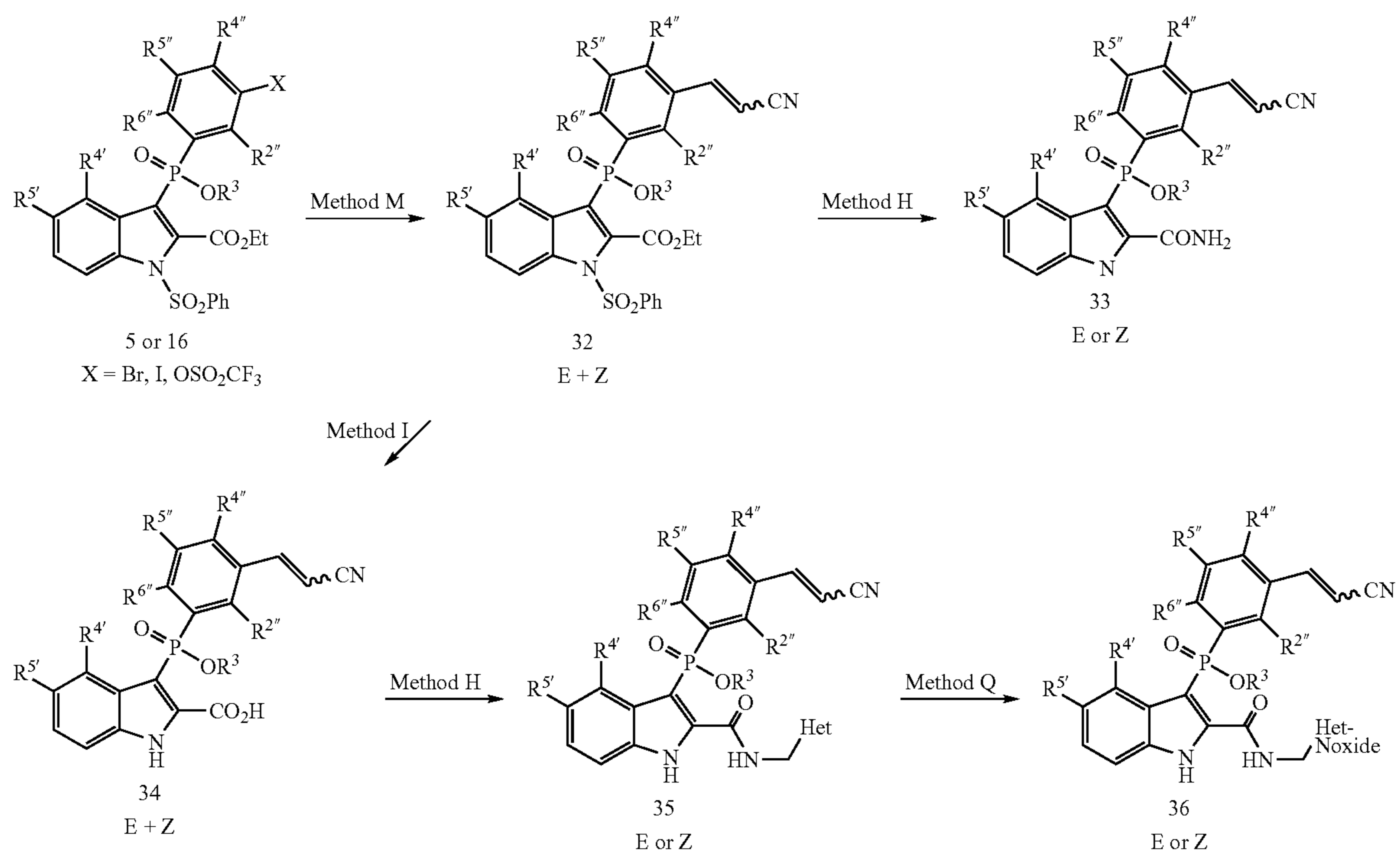
Scheme 9:
