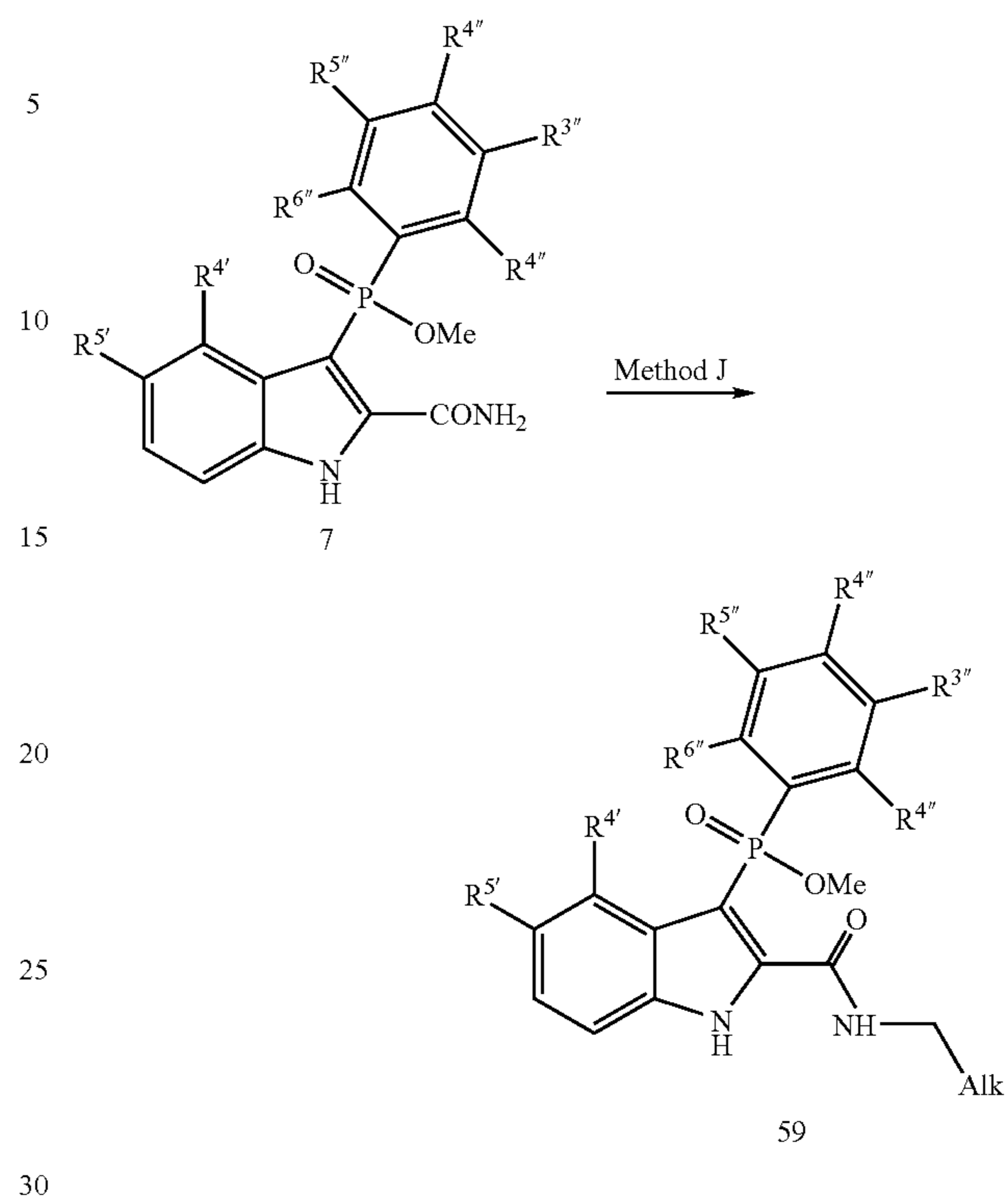
Scheme 15: Alkyl Methyl Carboxamides
