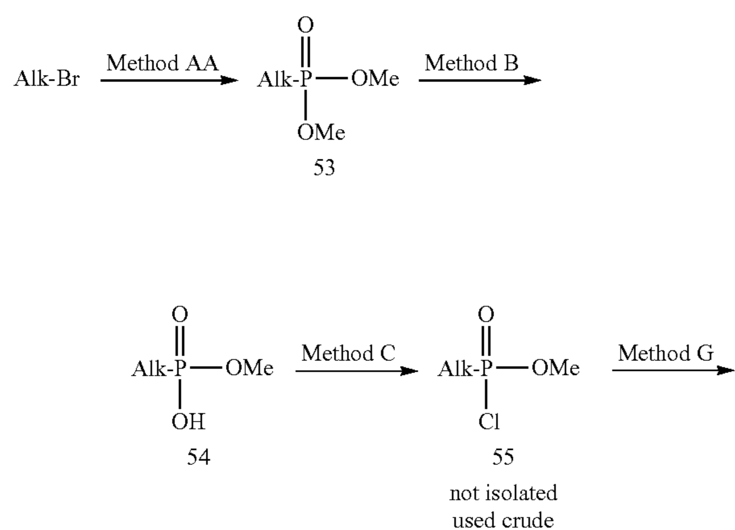
Scheme 13: Alkyl/Alkenyl/Alkynyl Phosphinates
