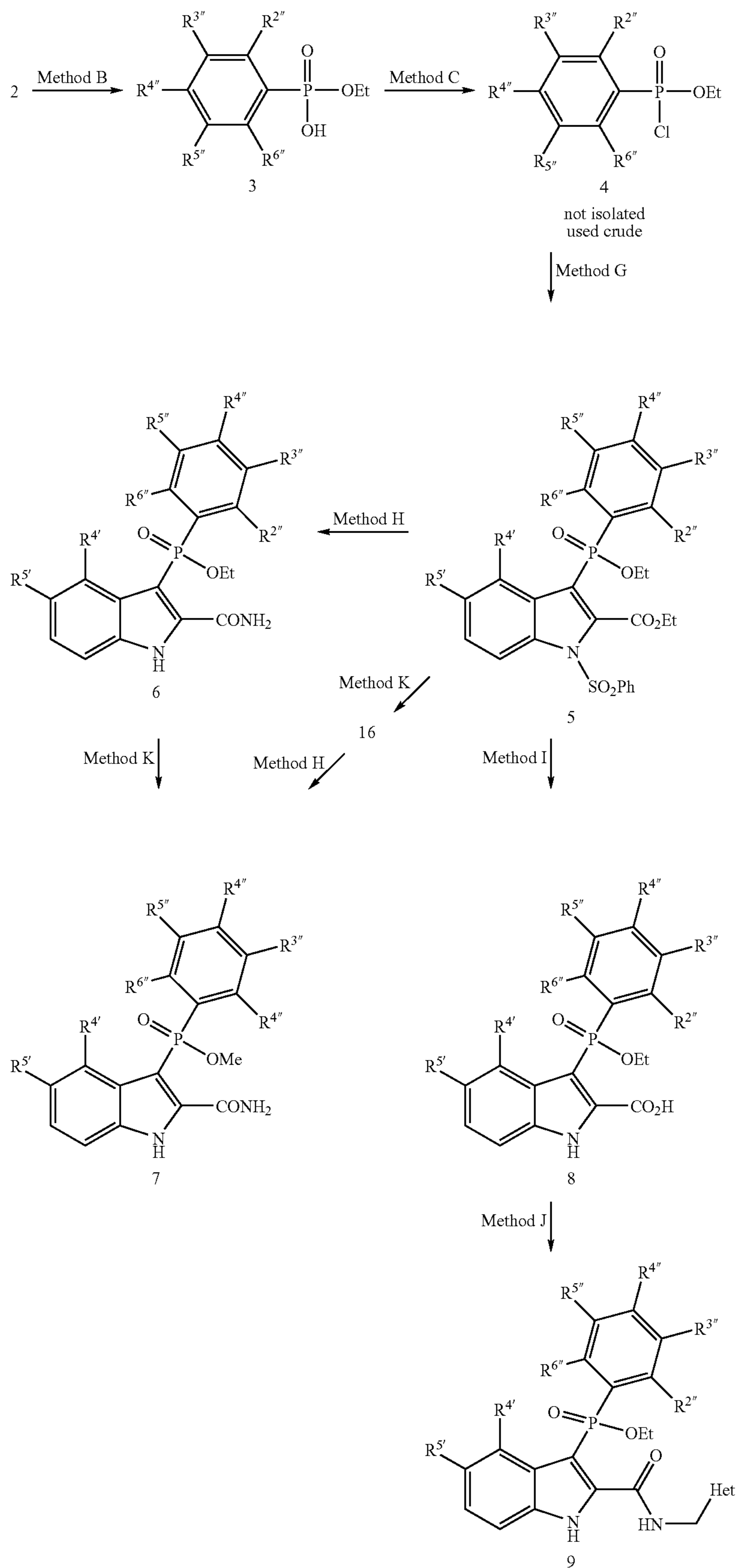
Scheme 2:
