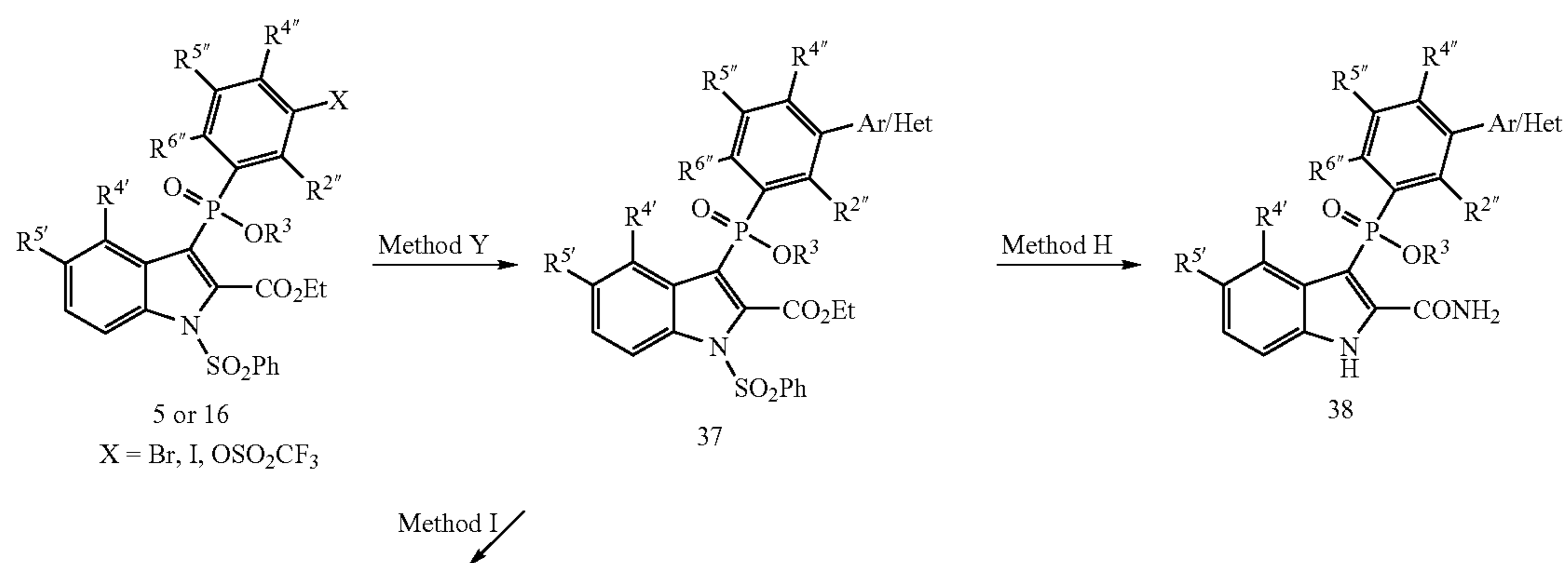
Scheme 10:
