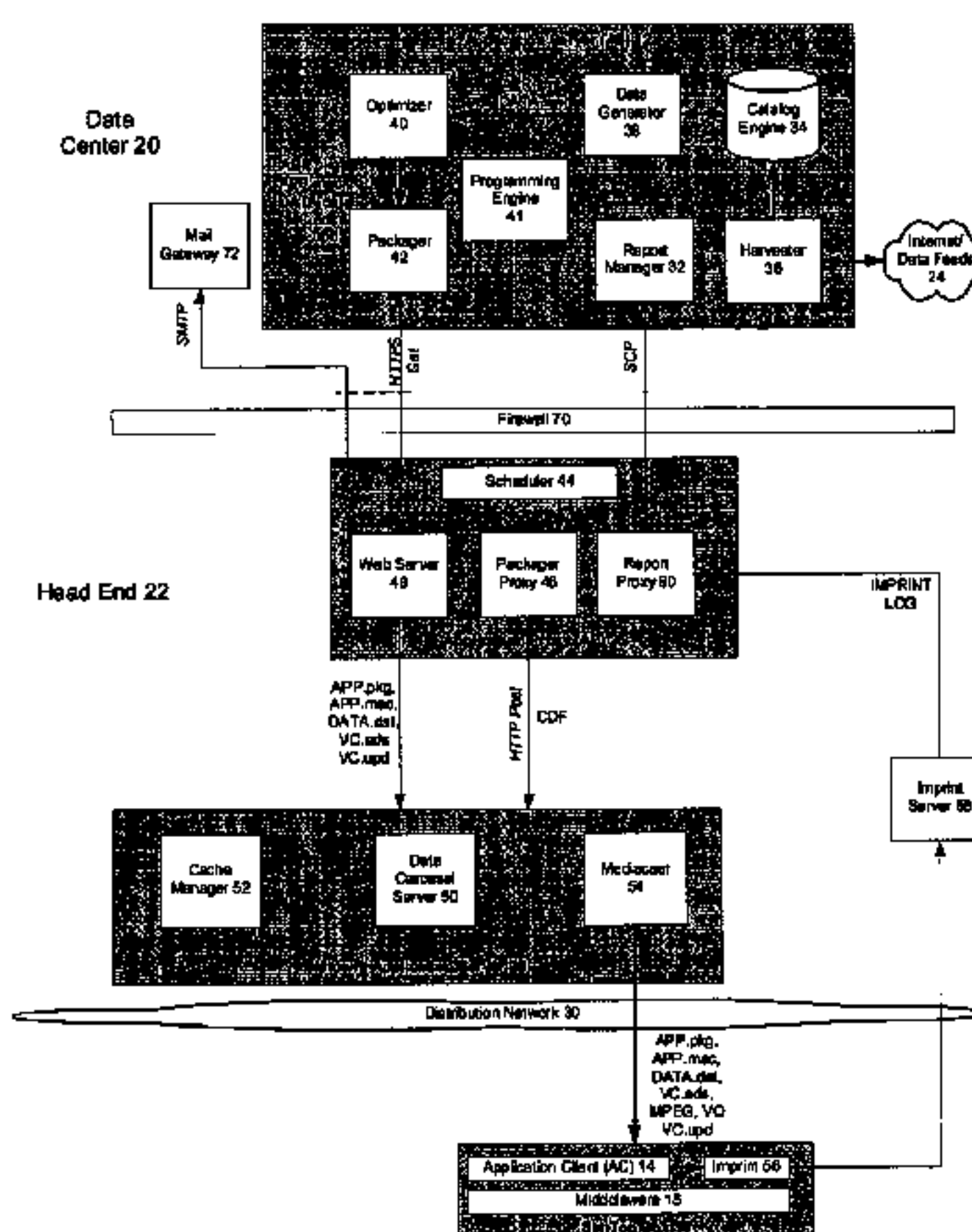
Unified Application System 10
