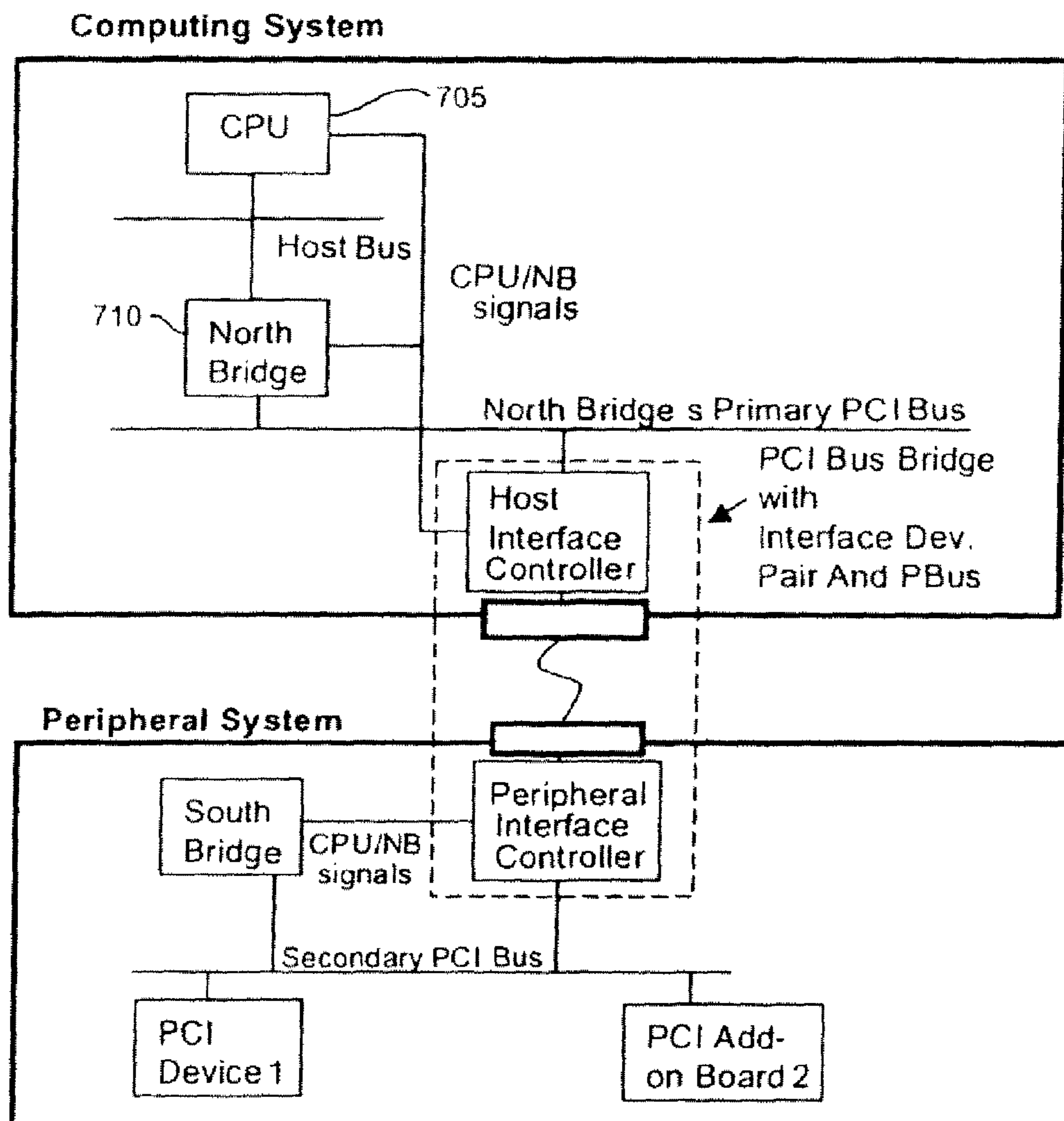
FIGURE 7
