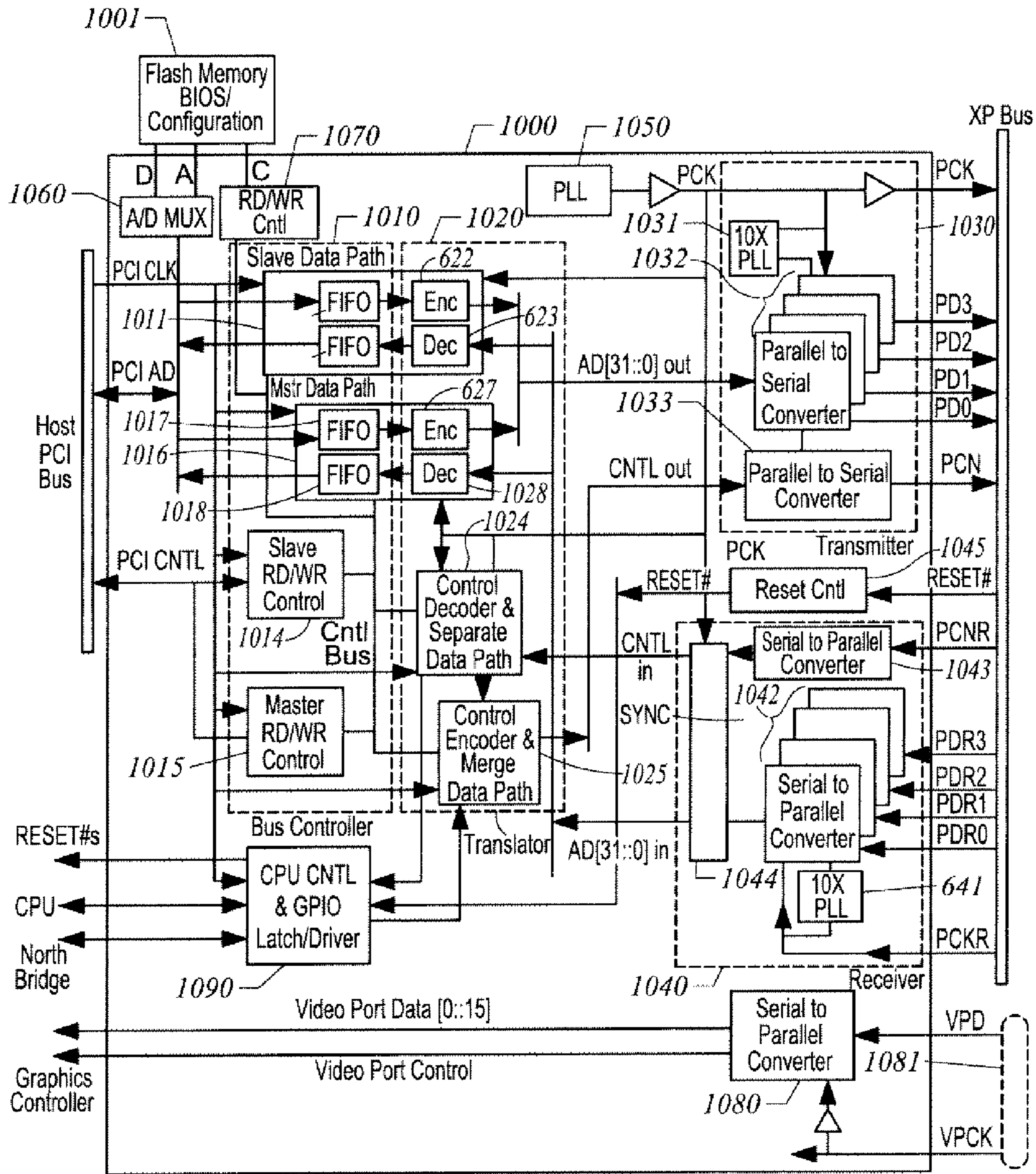
FIGURE 10
