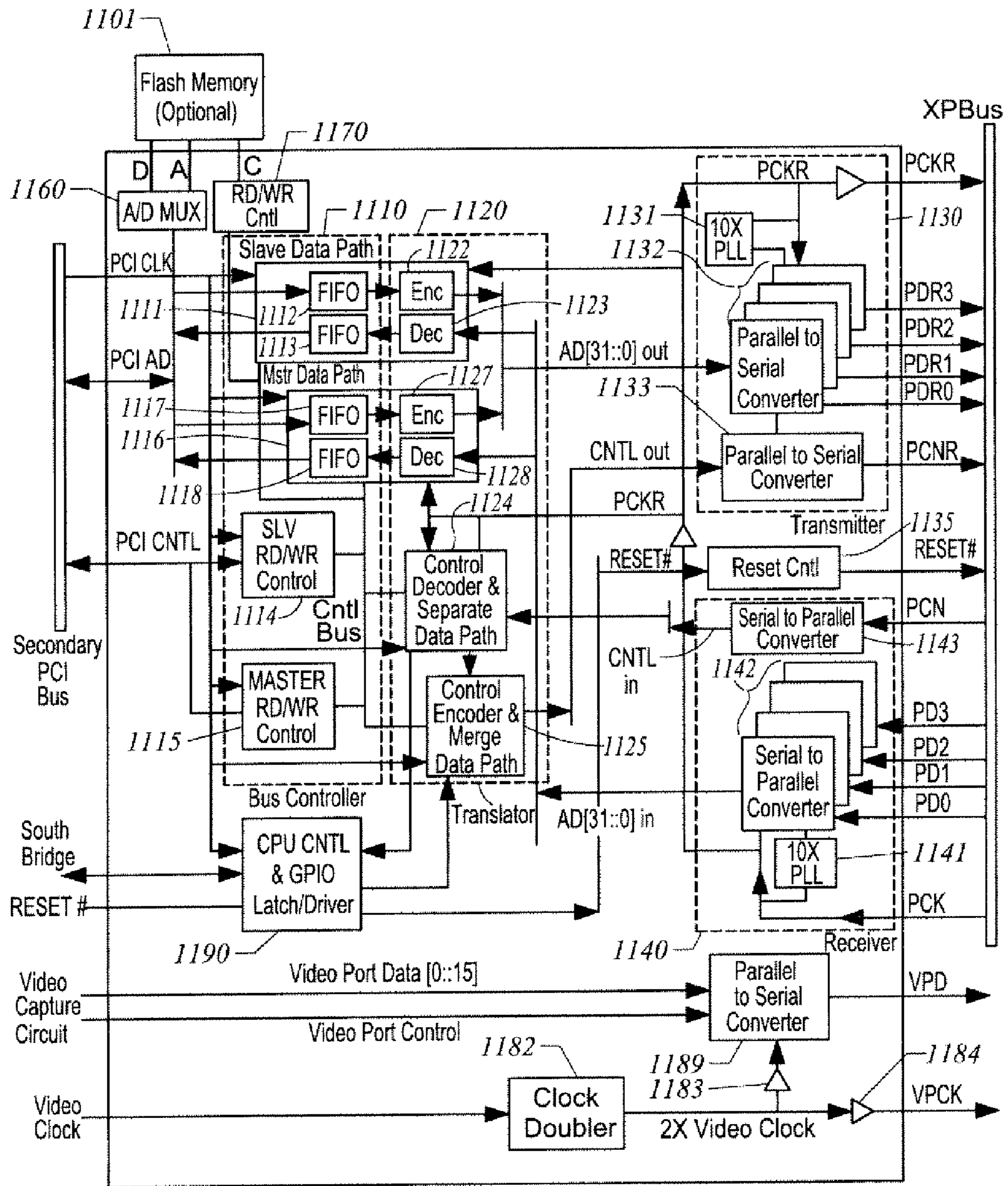
FIGURE 11
