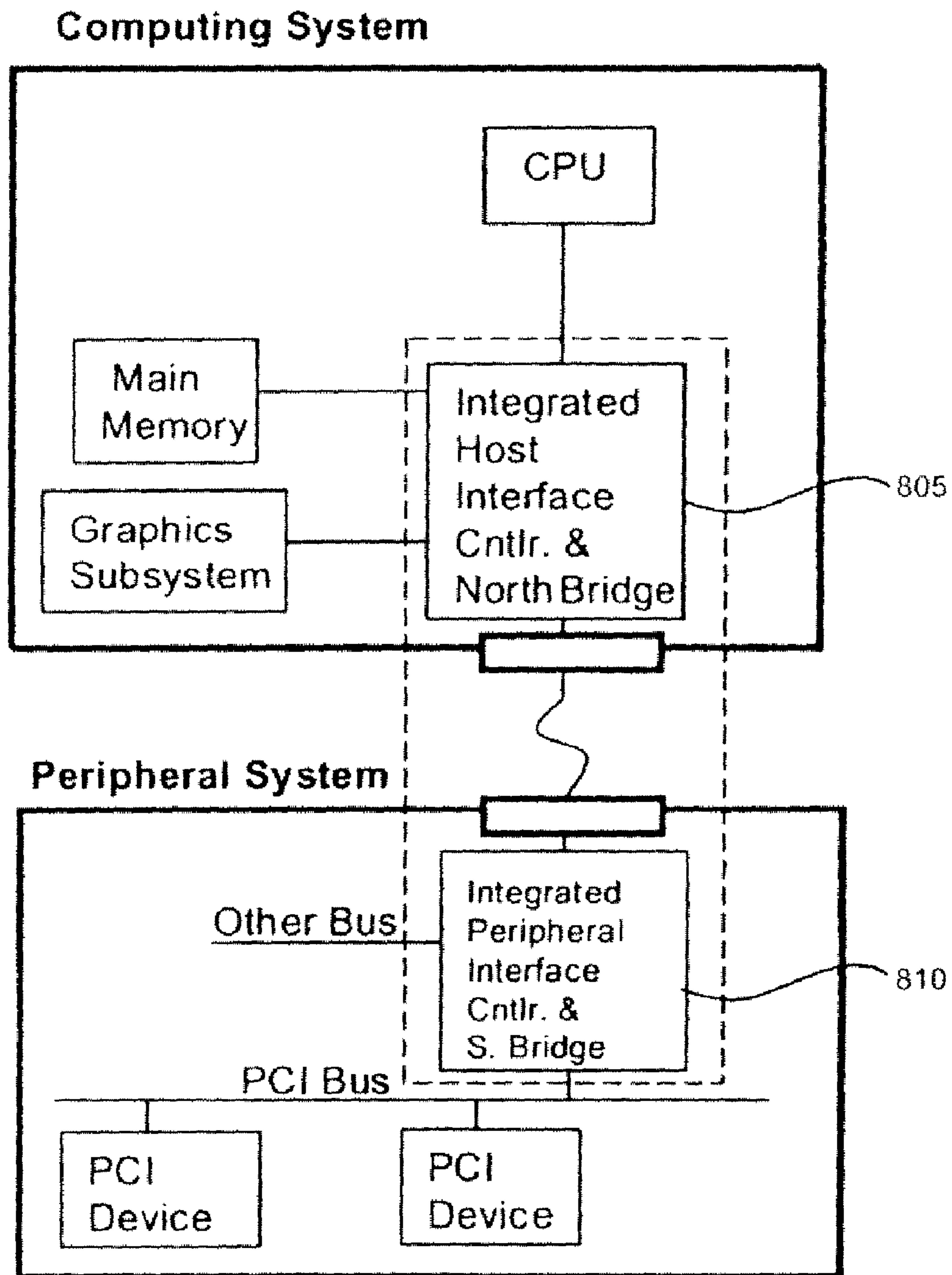
FIGURE 8
