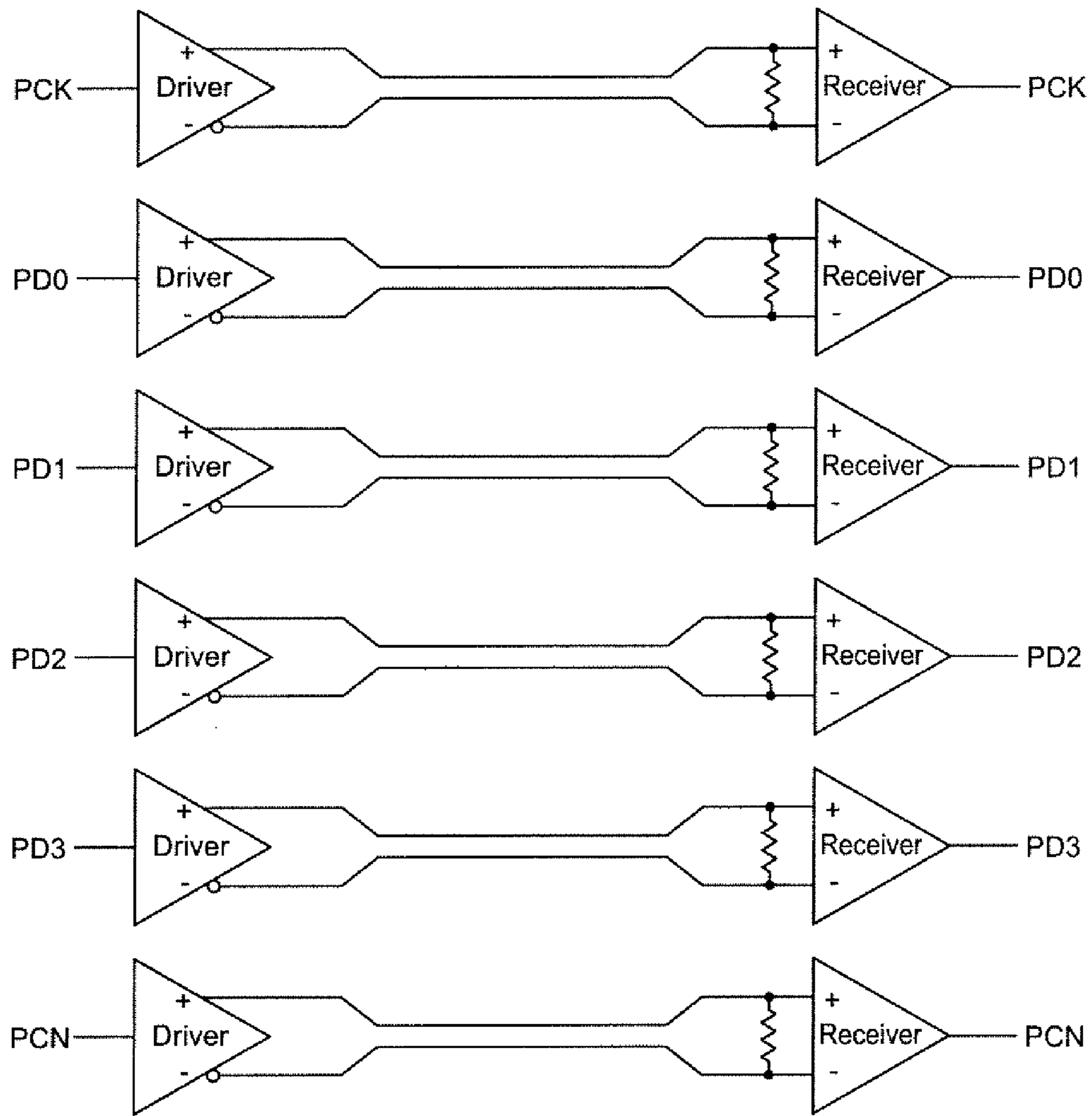
FIGURE 15
