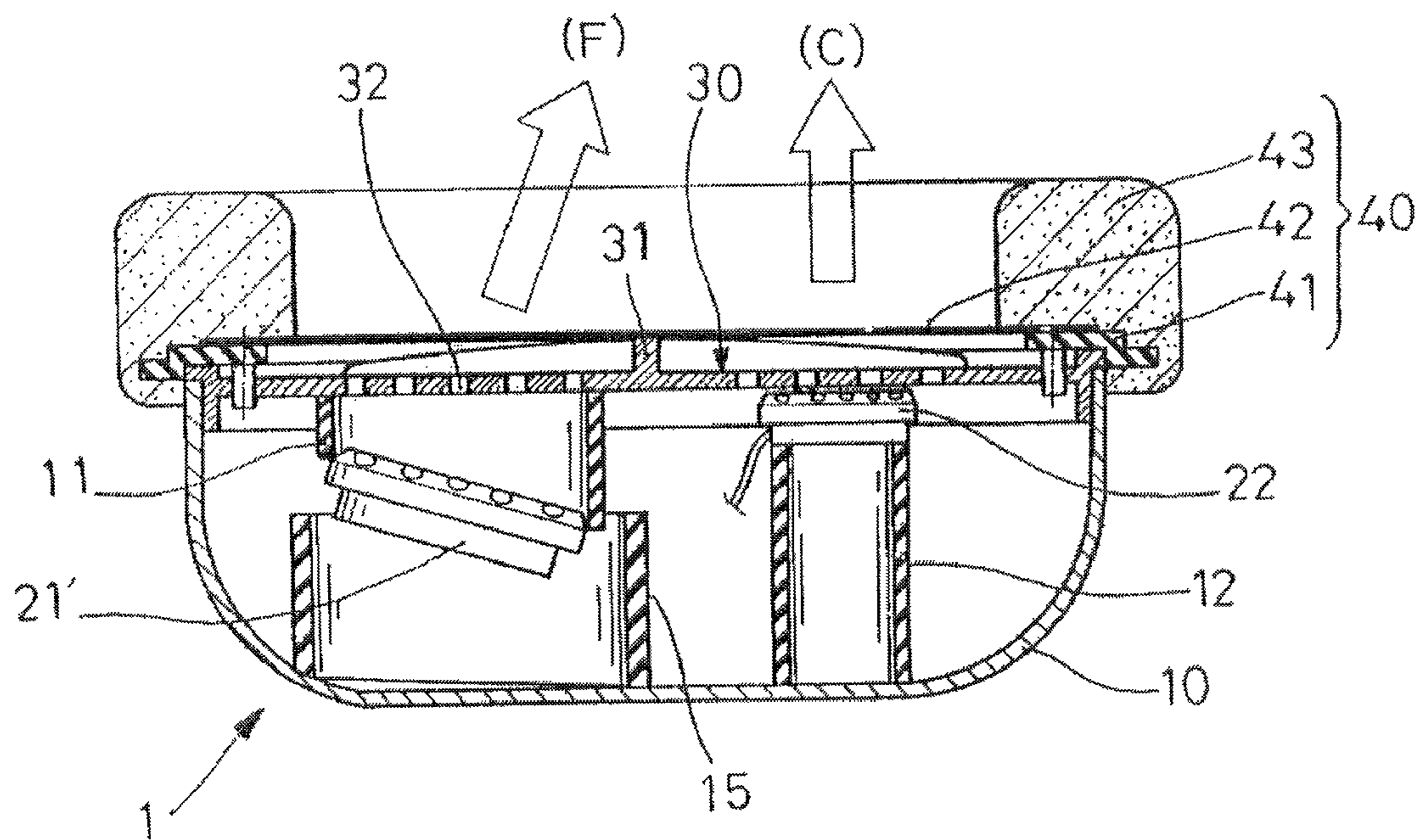
FIG. 2C (PRIOR ART)
