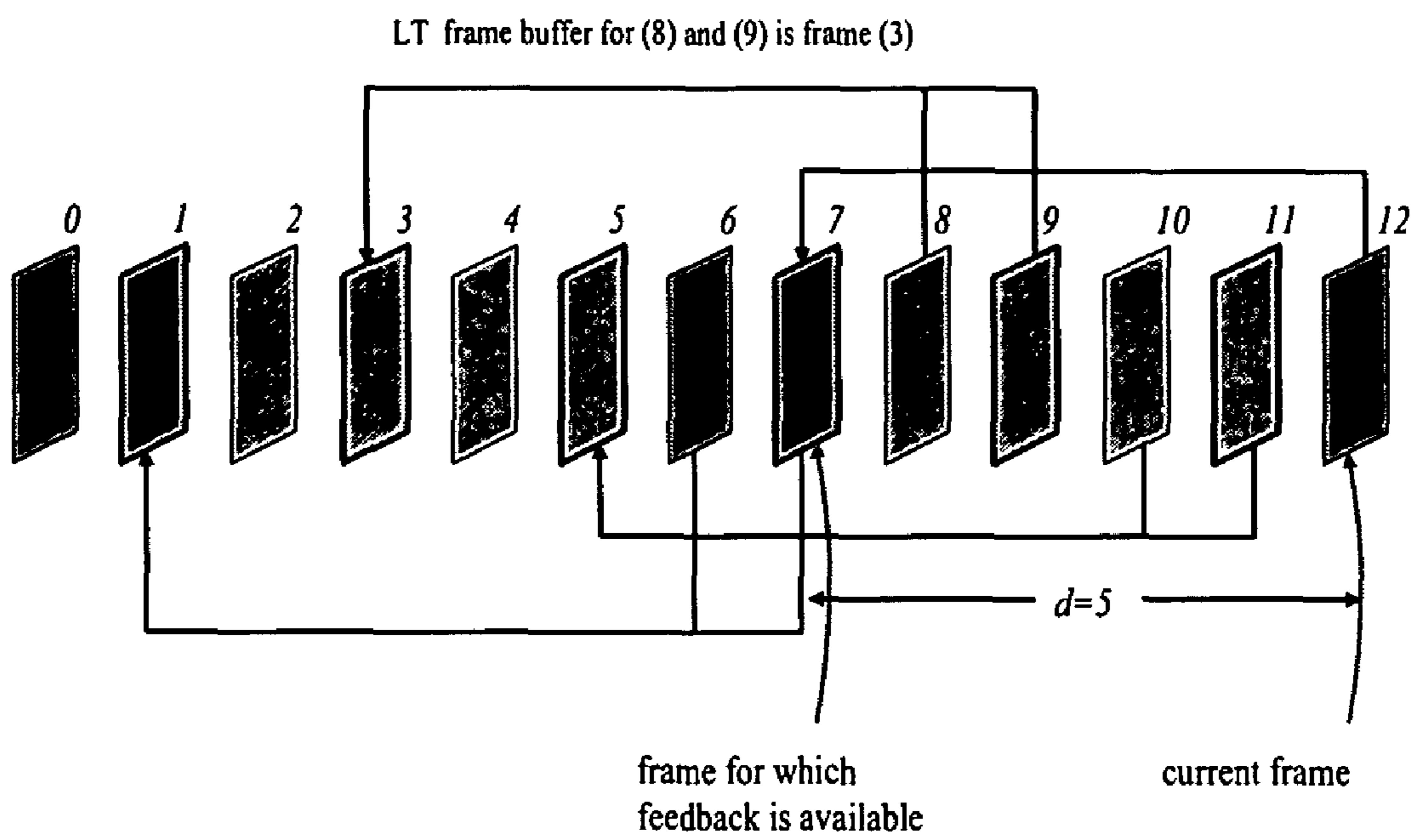
ENCODING METHOD WITH FEEDBACK FOR PARAMETERS SN=2 , D=5 and d=5
