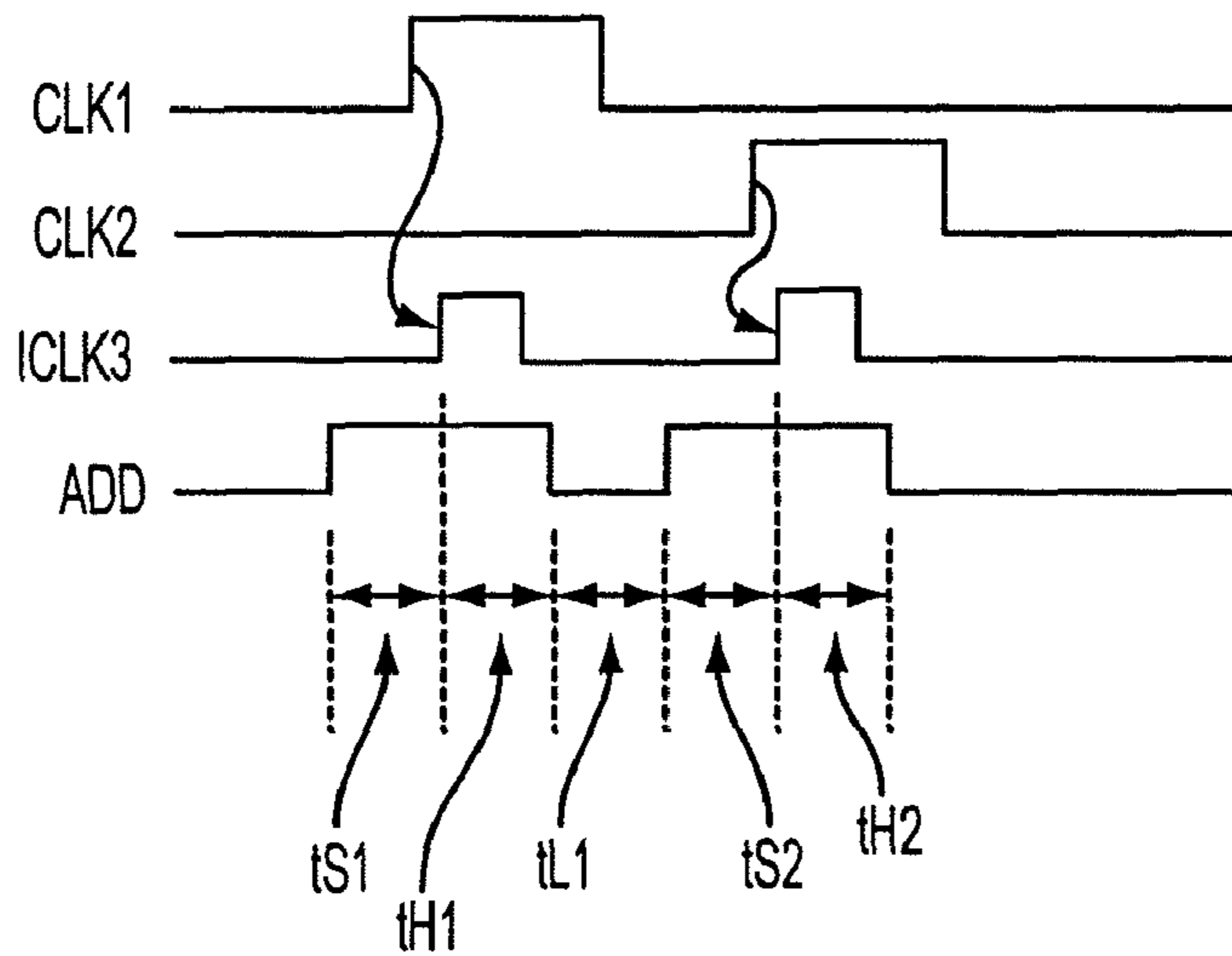
FIG. 4 PRIOR ART
