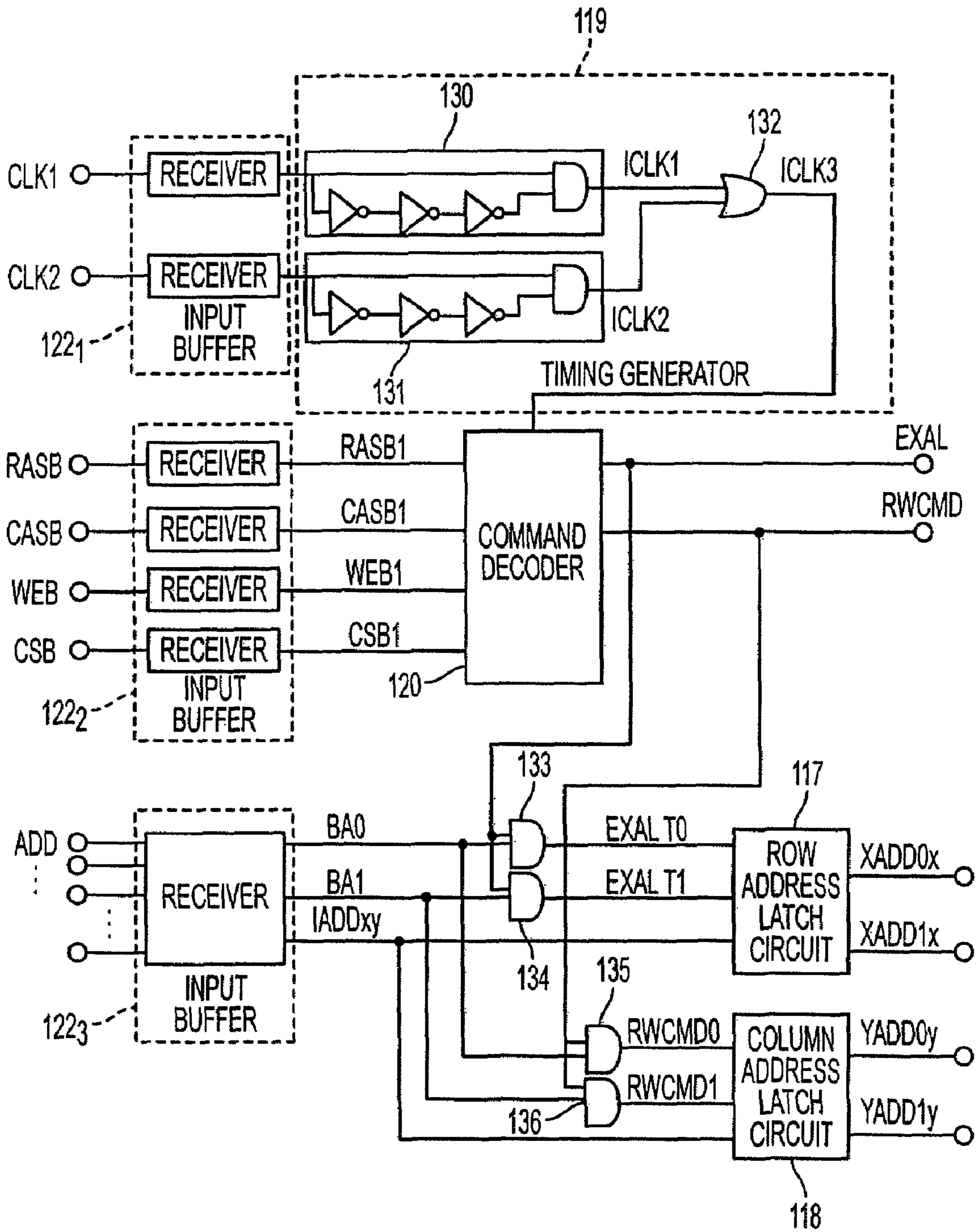
FIG. 2 PRIOR ART
