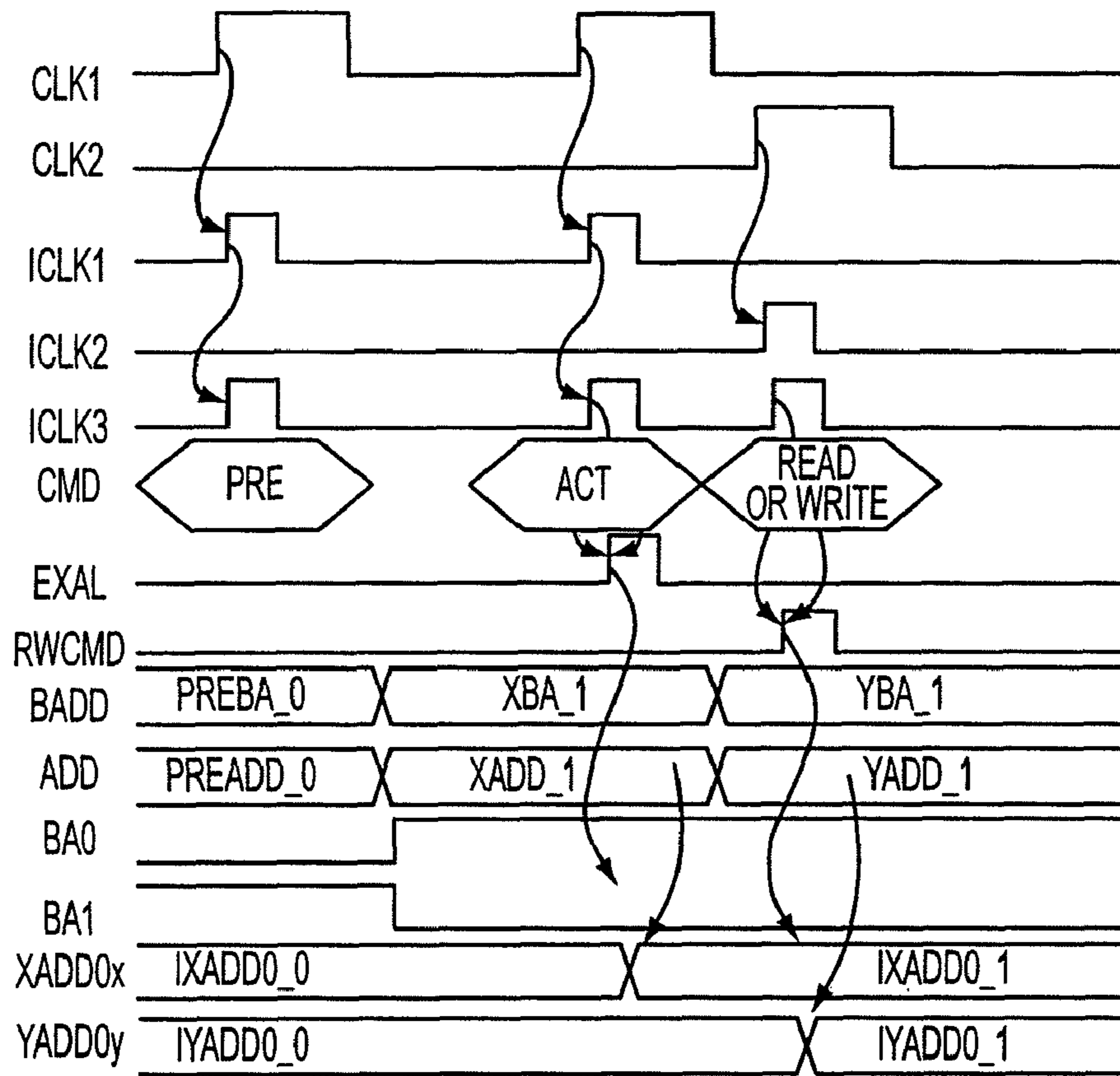
FIG. 3 PRIOR ART
