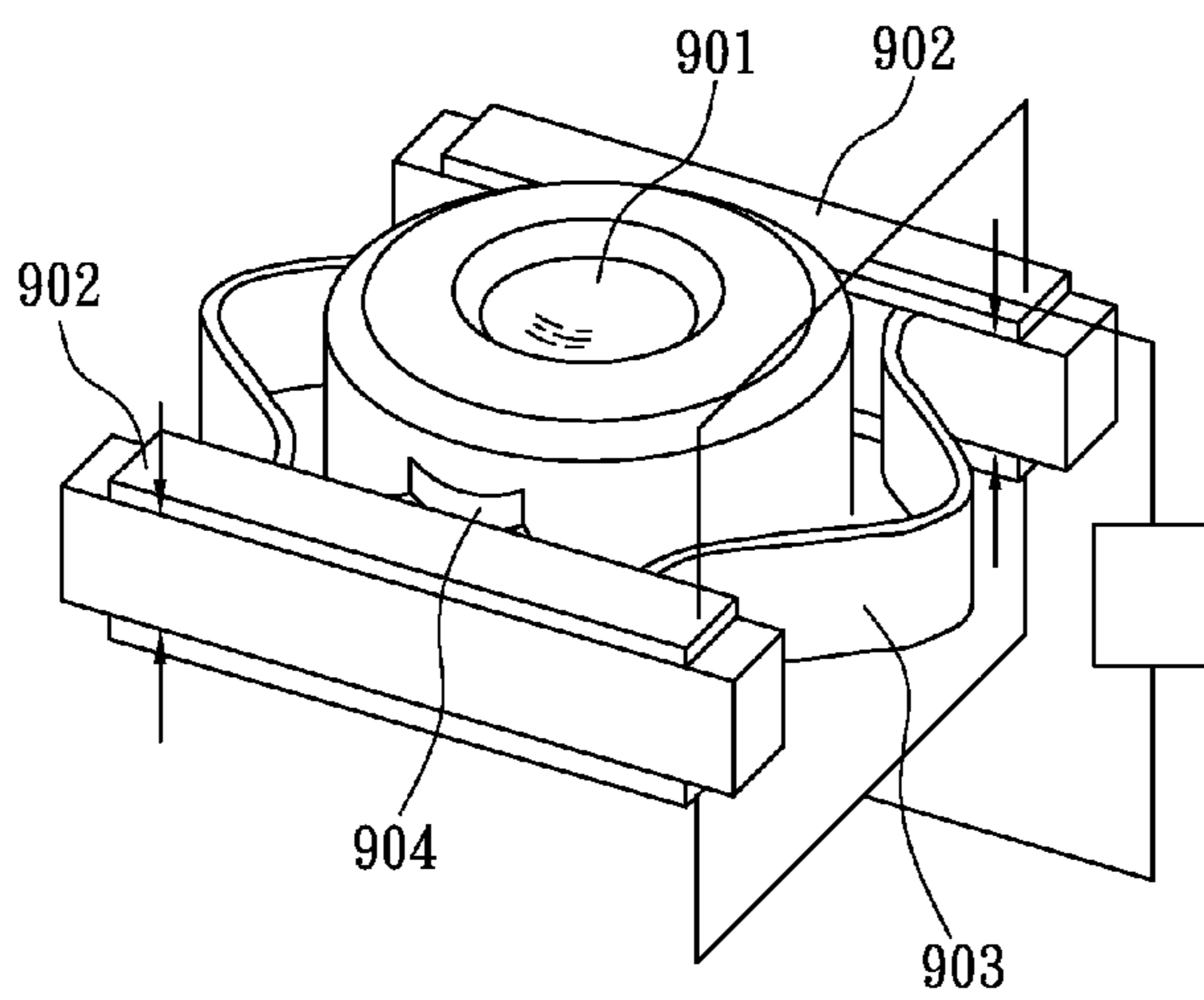
FIG. 3 (PRIOR ART)
