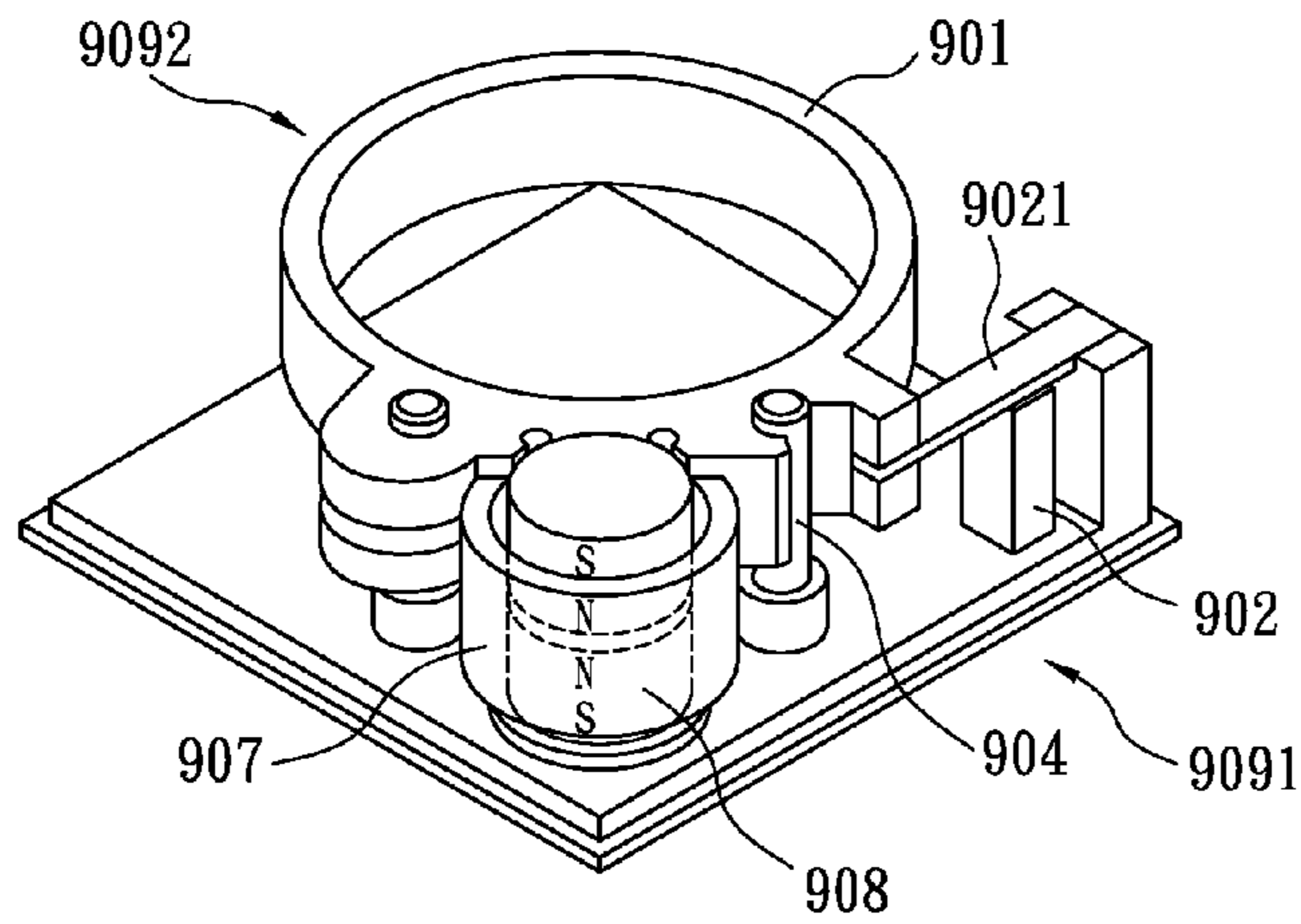
FIG. 1 (PRIOR ART)
