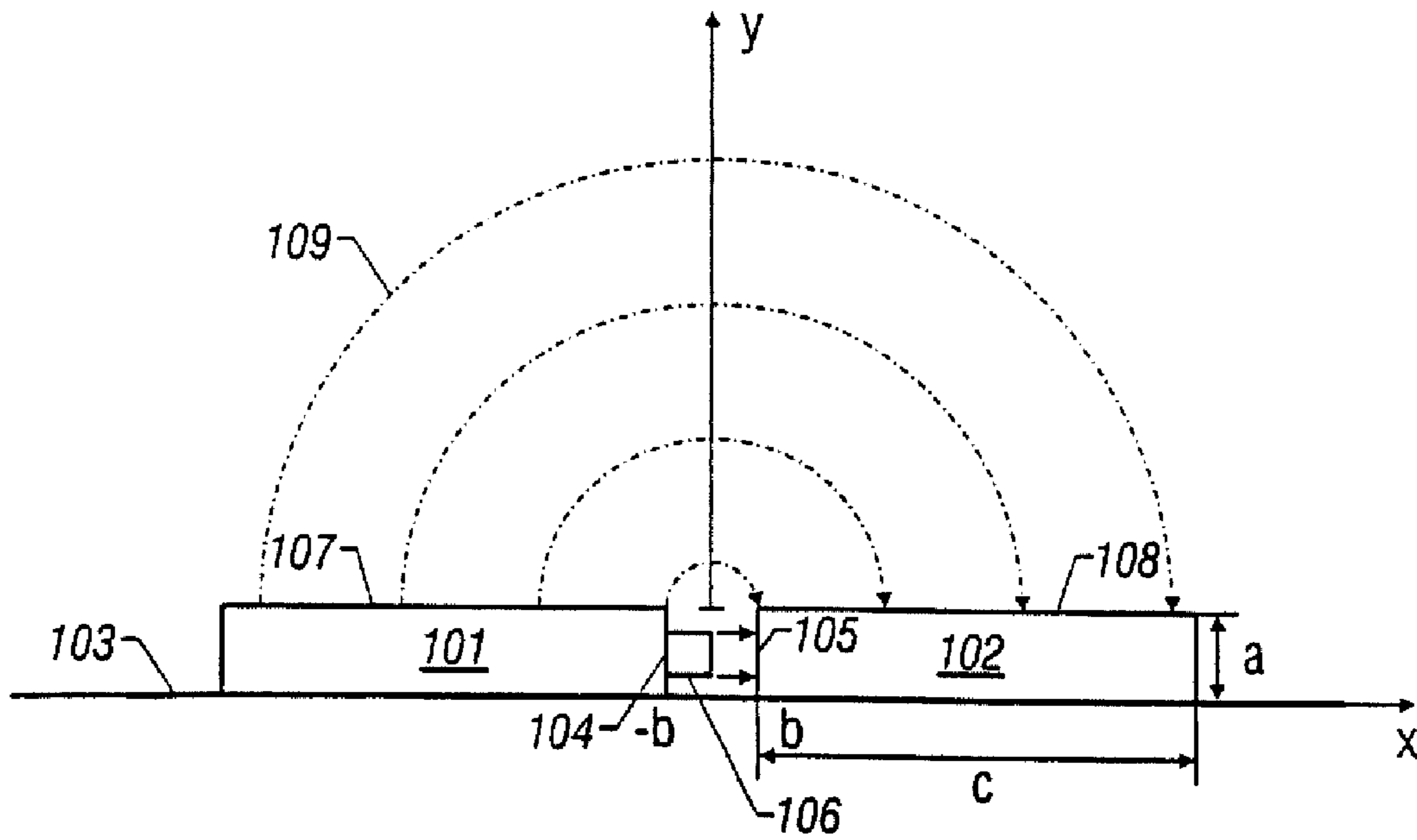
FIG. 1 (PRIOR ART)
