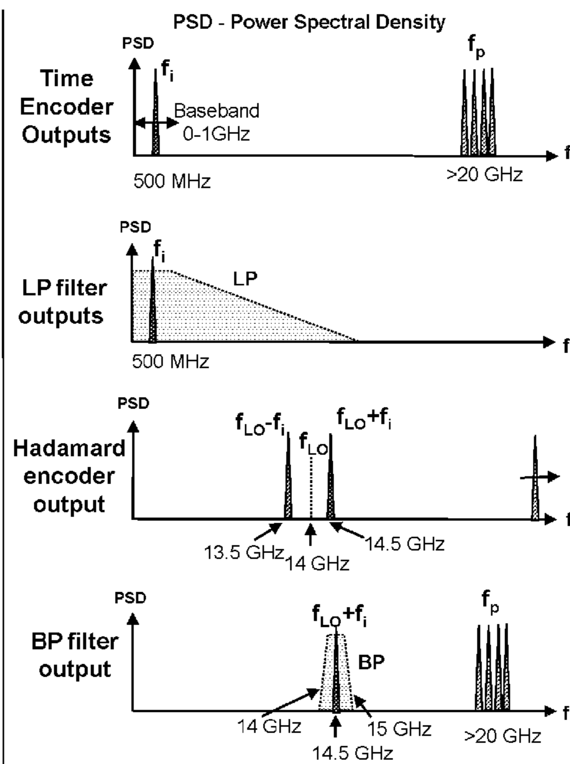
Example of Up-Conversion from 0-1GHz to 14-15 GHz
