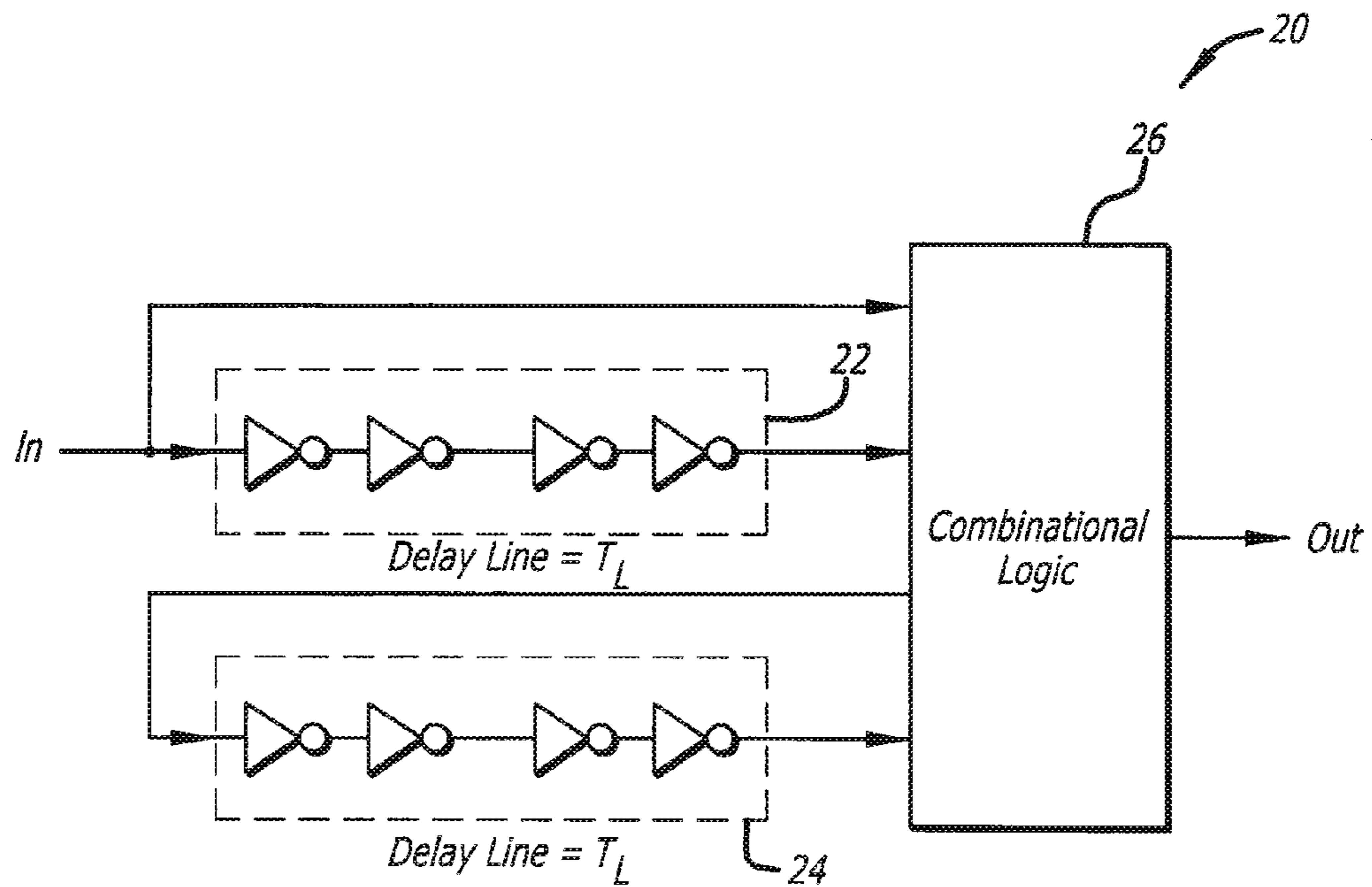
FIG. 4 (Prior Art)
