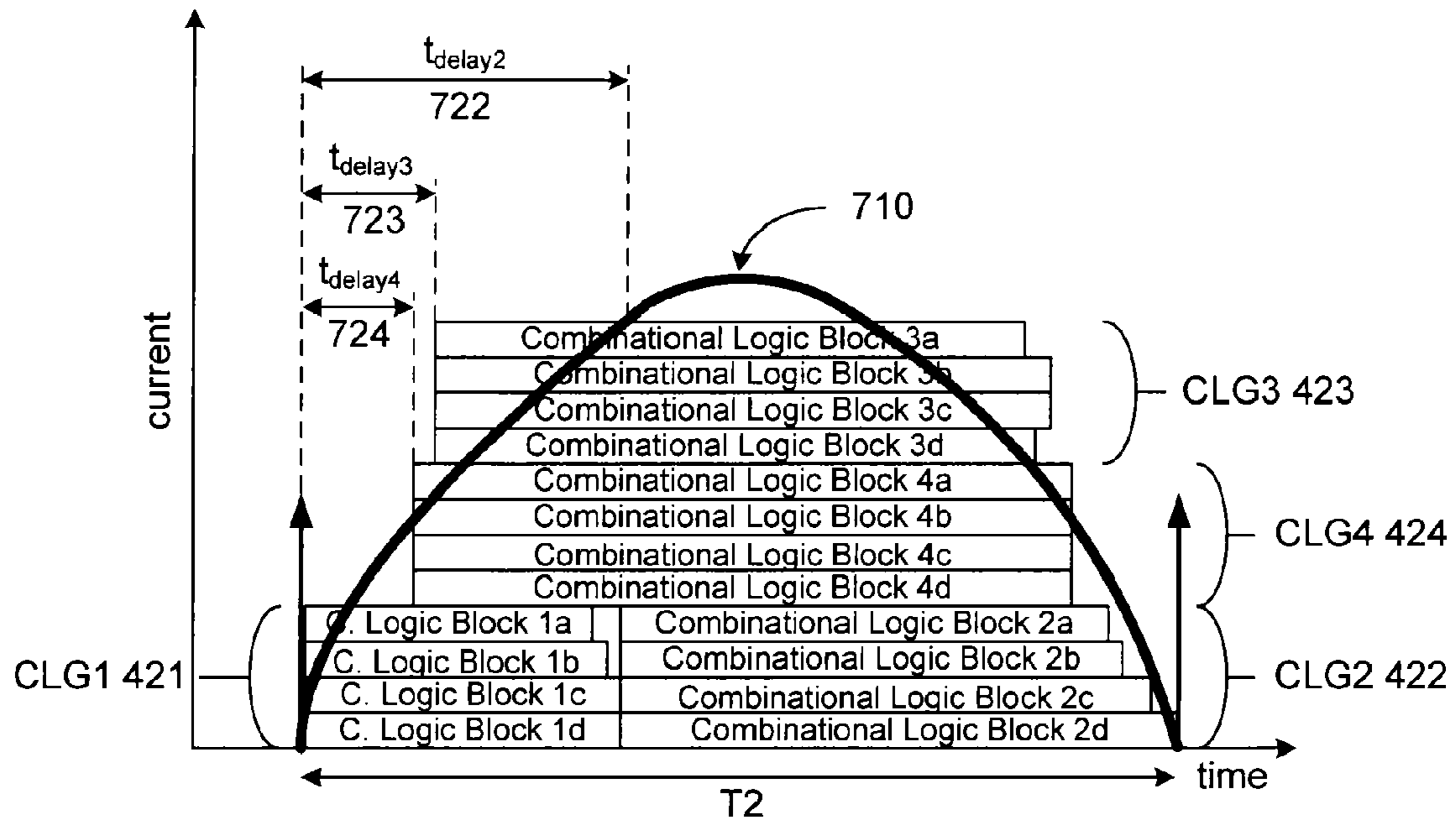
Idealized Current Distribution
