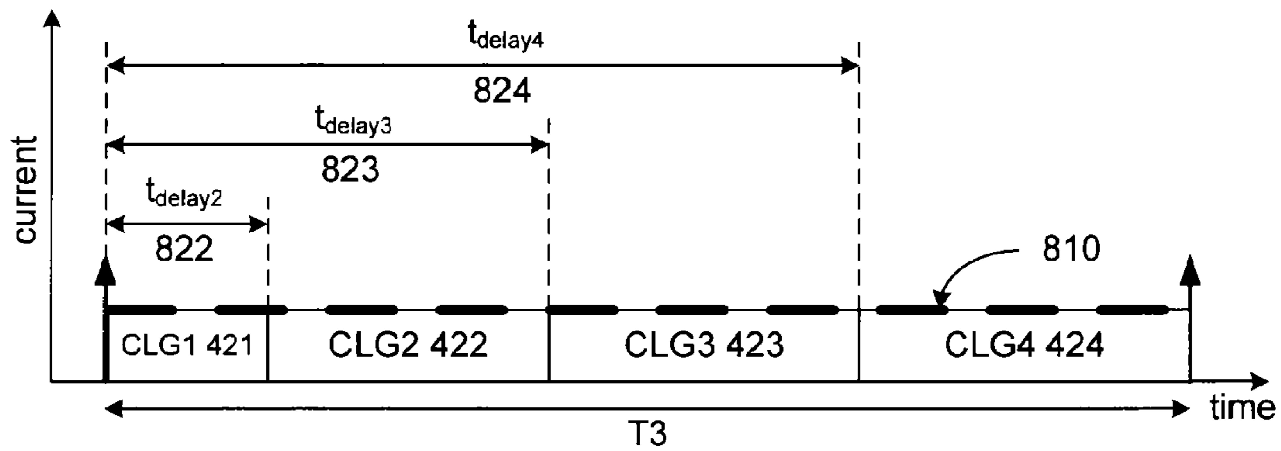
Idealized Current Distribution
