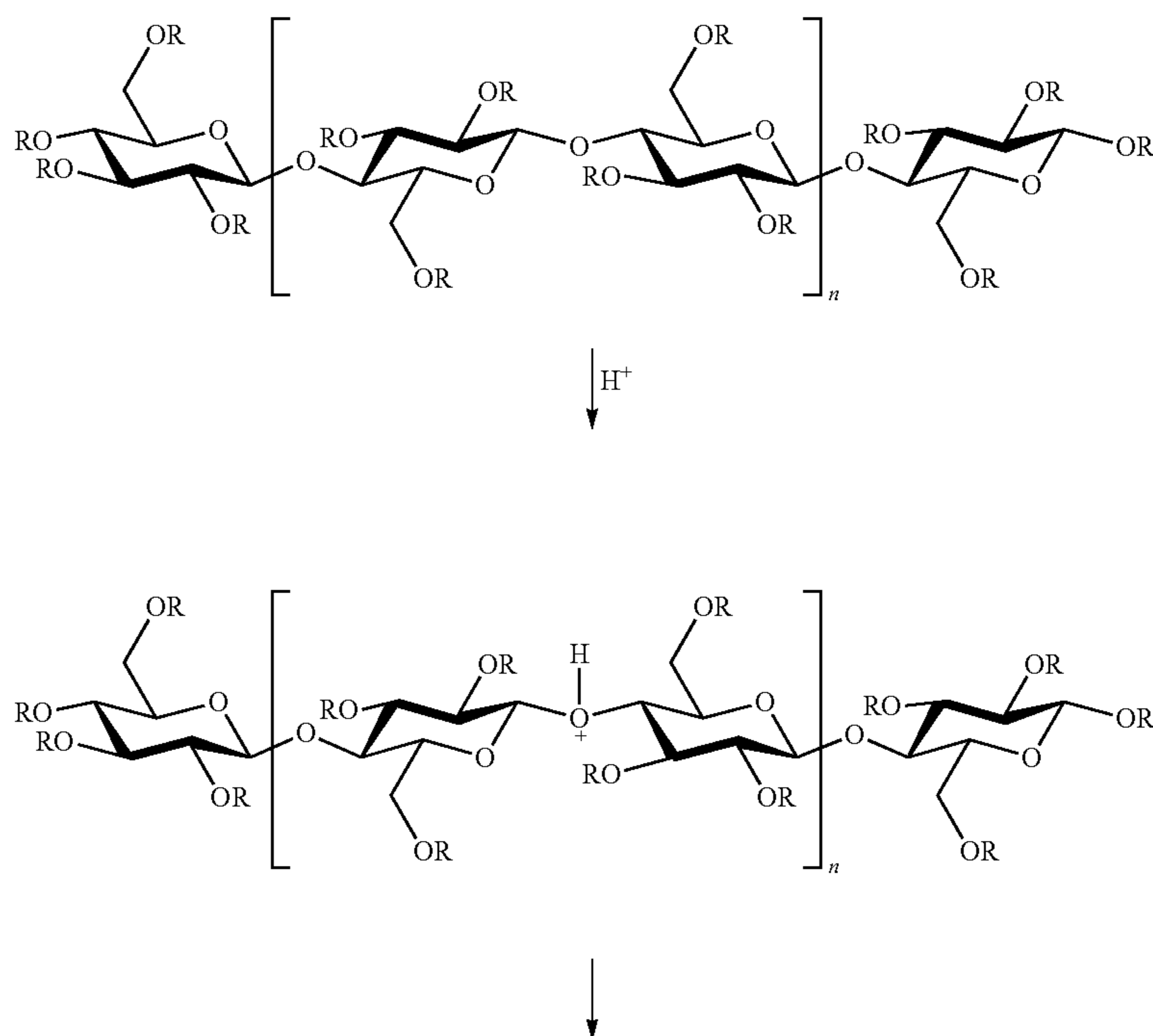
Scheme 1. Proposed mechanism for the hydrolysis and acetolysis of glycosidic bonds.
