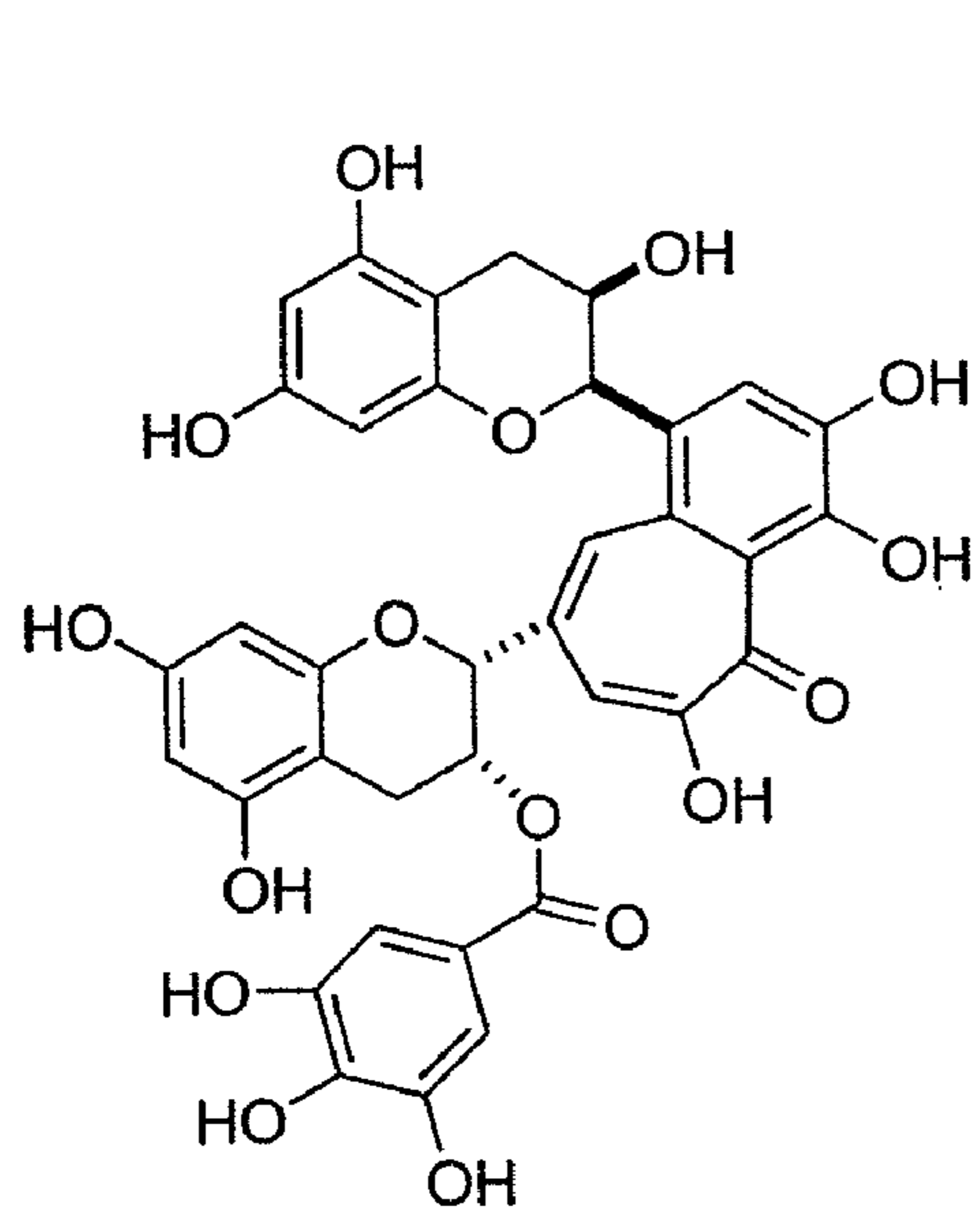
Theaflavin-3'-gallate
