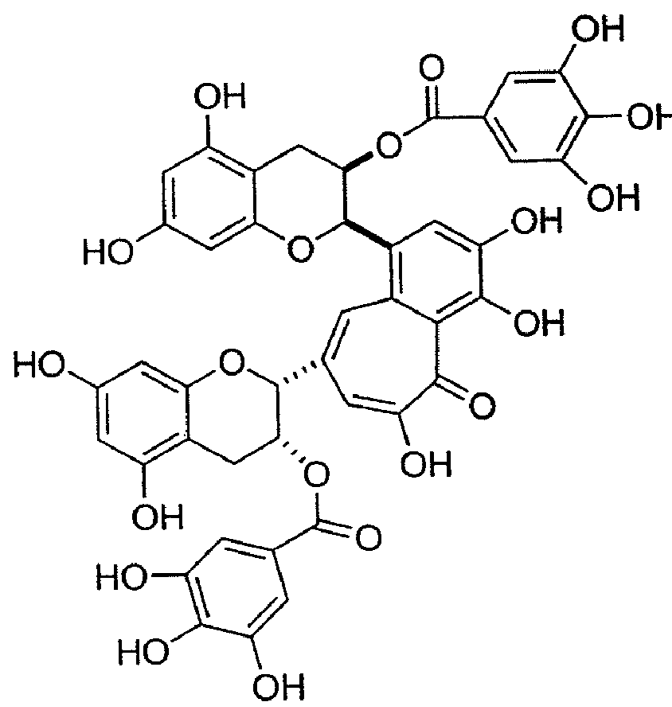
Theaflavin-3,3'-gallate
