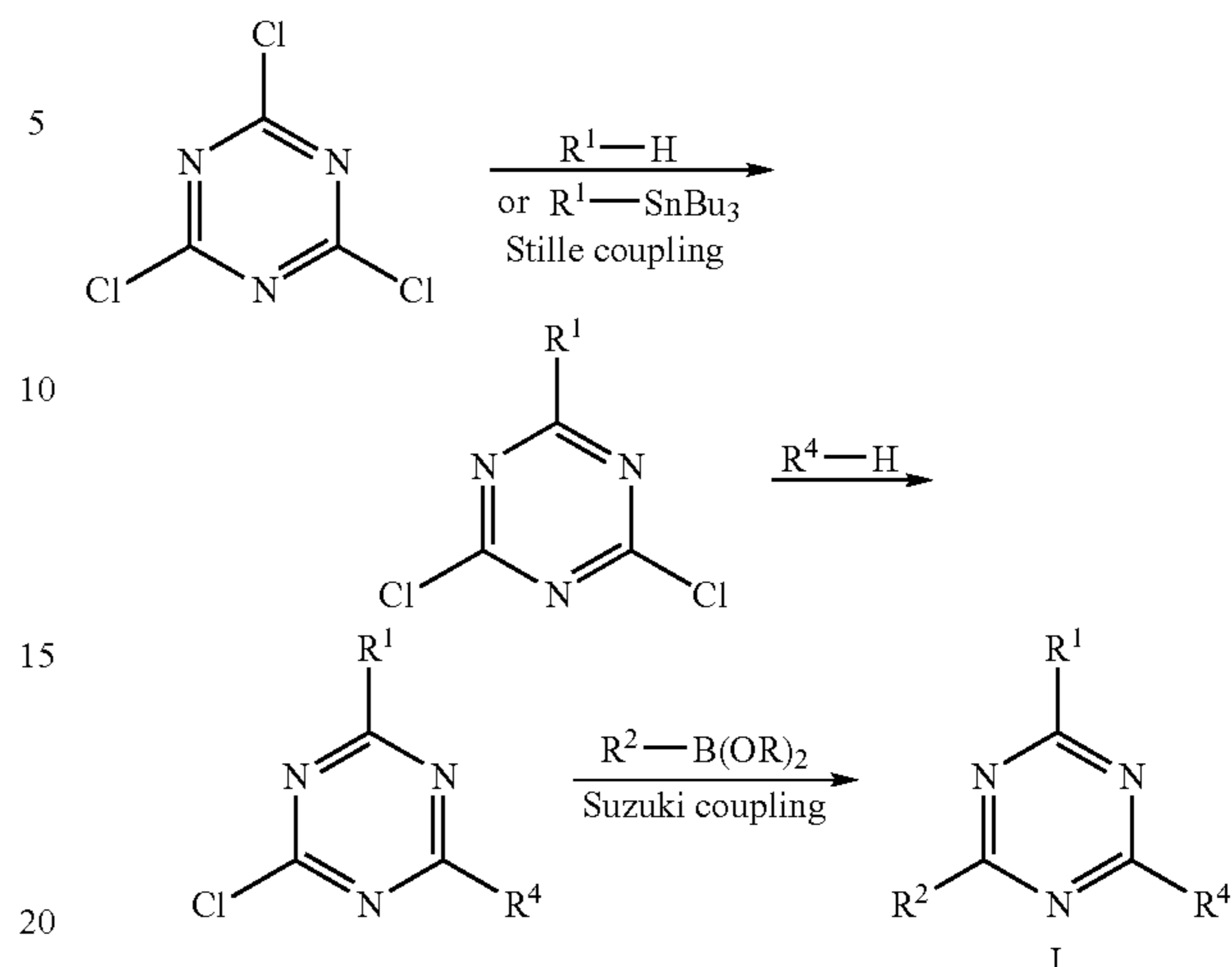
Scheme 12
