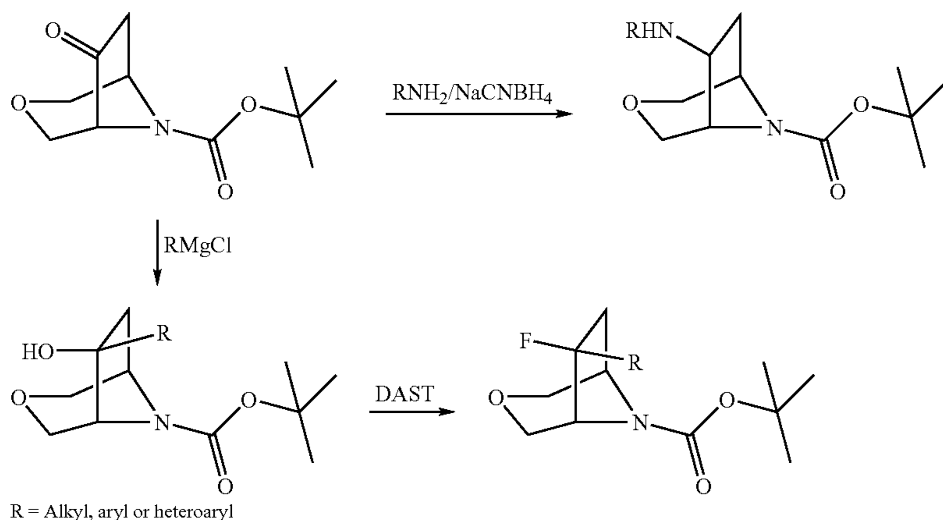
Scheme 11
