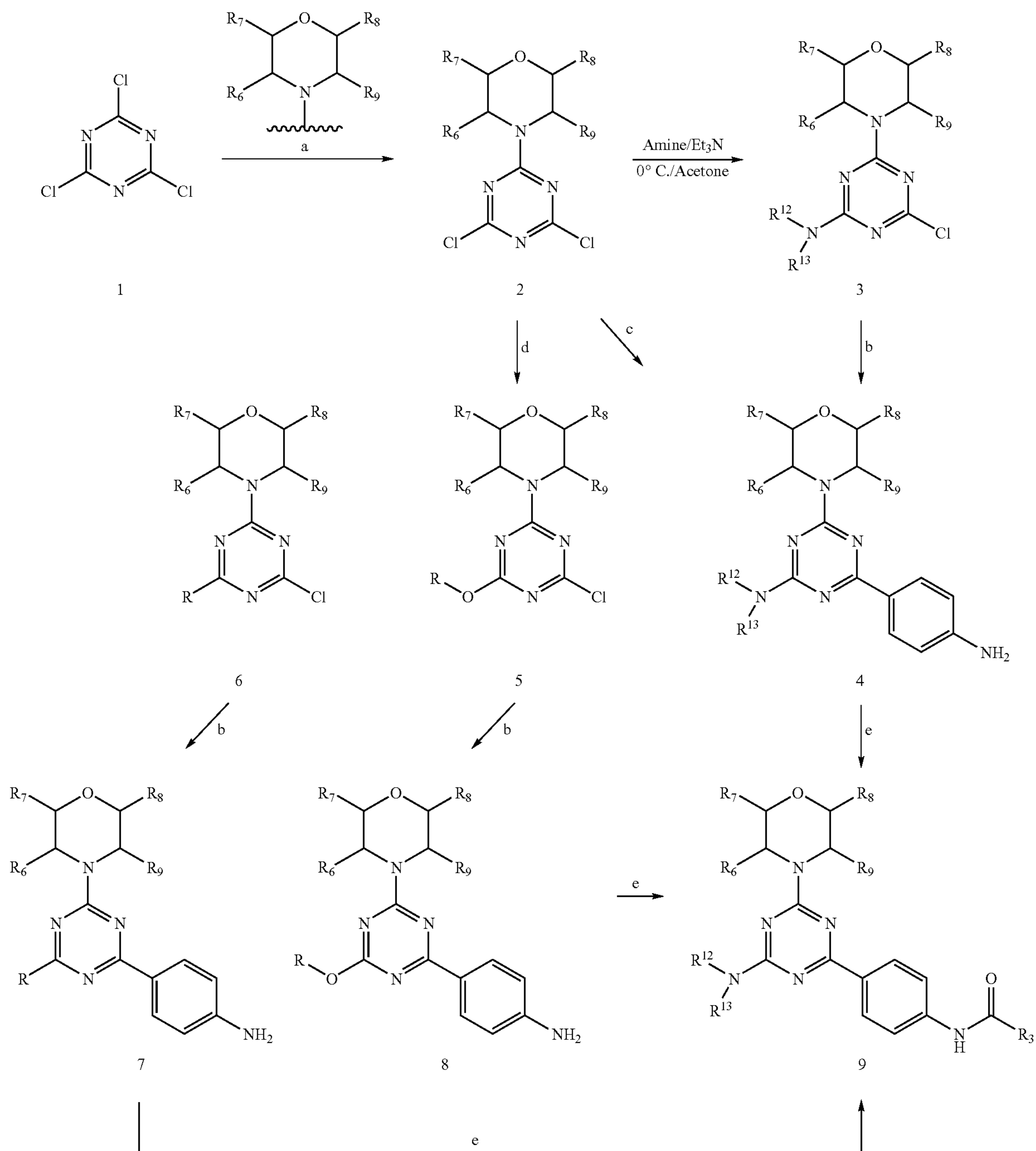
Scheme 1
