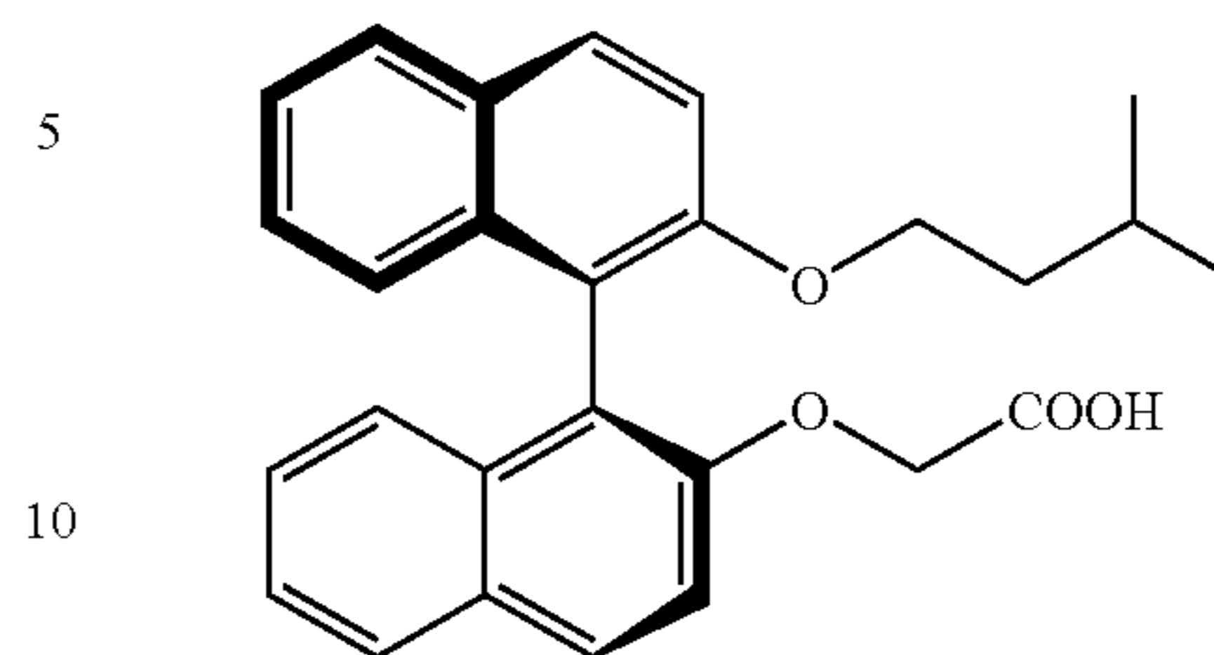
[2'-(3-Methylbutoxy)-[1,1']-(S)-binaphthalen-2-yloxy]-acetic acid (105)
