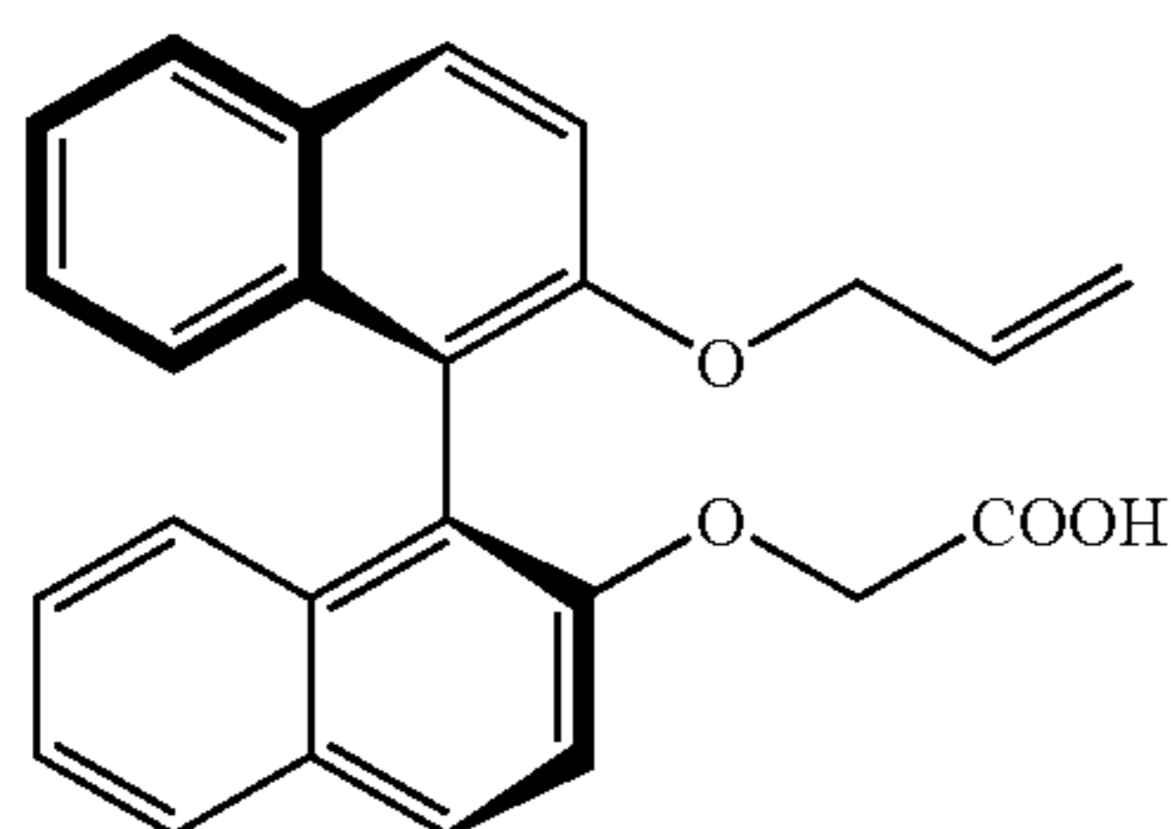
(2'-Allyloxy-[1,1']-(S)-binaphthalen-2-yloxy)-acetic acid (101)
