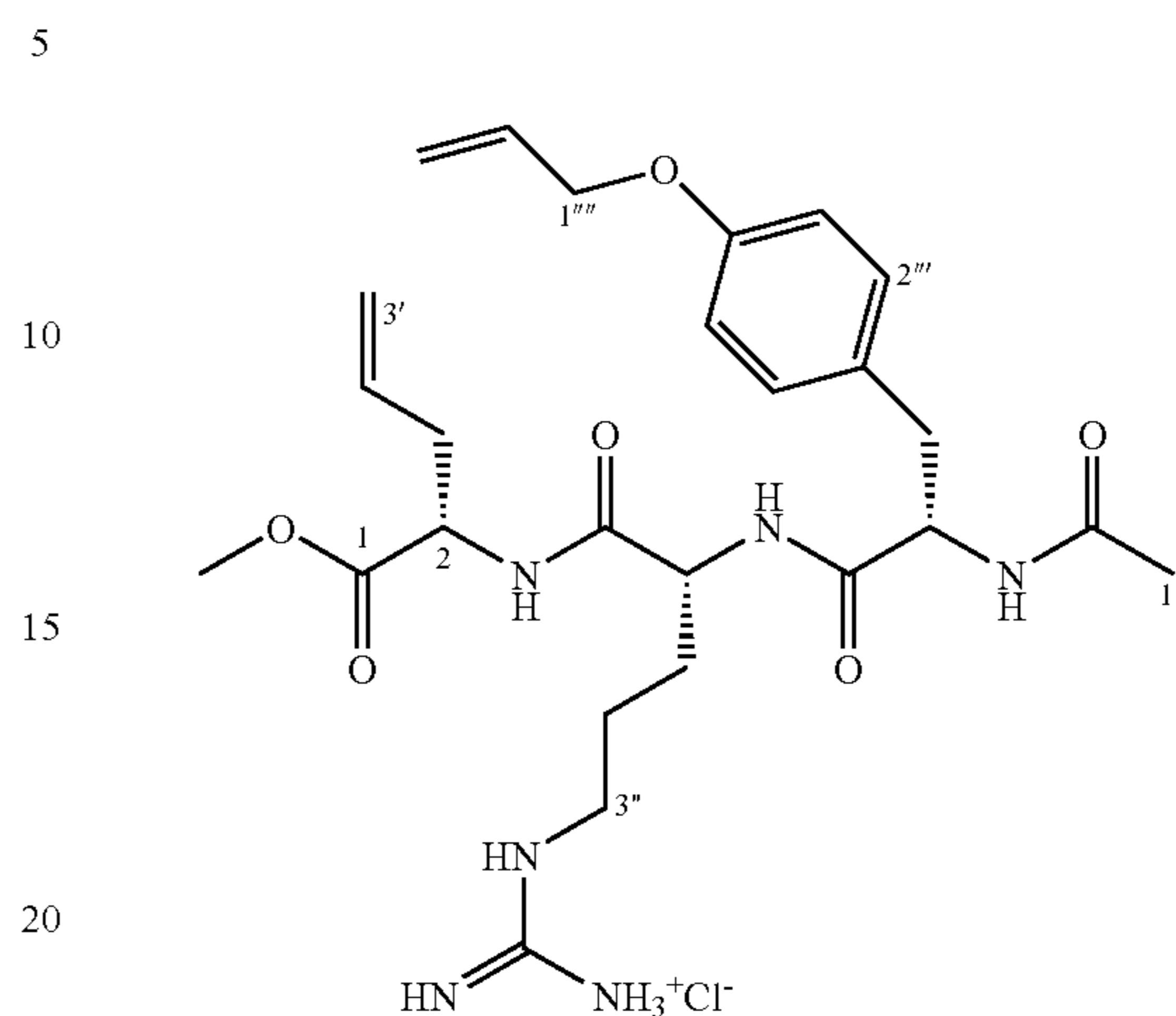
Methyl(2S,5R,8S)-2-allyl-8-(4-allyloxybenzyl)-3,6,9-triaza-5-(3-[guanidino]propyl)-4,7,10-oxoundecanoate hydrochloride (82)
