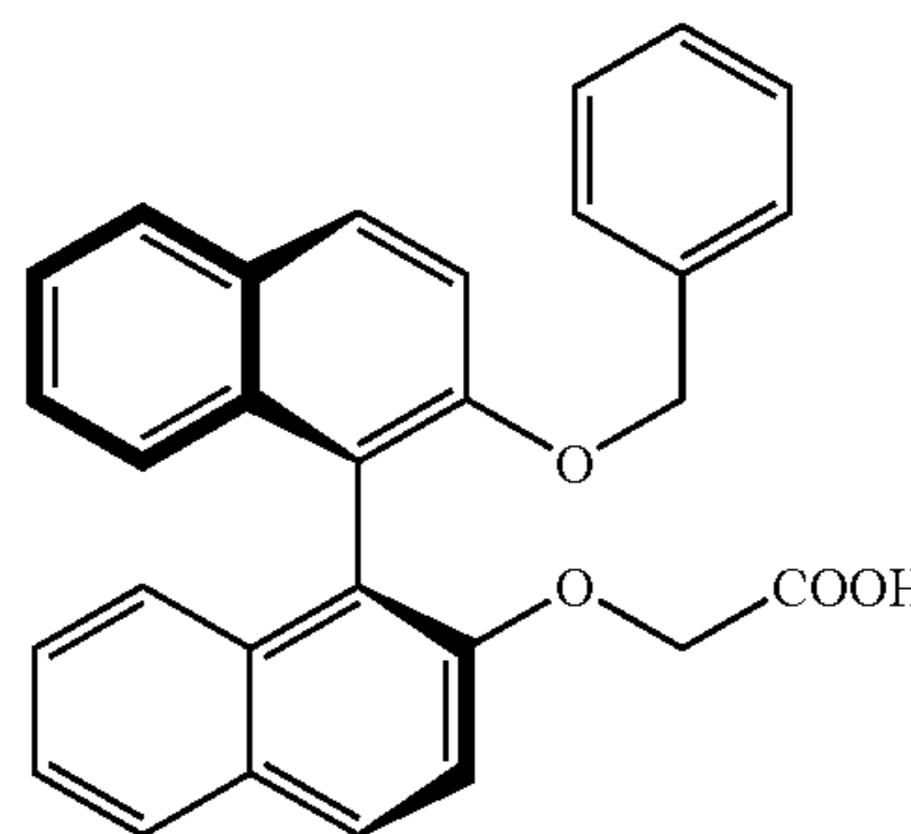
(2'-Benzyloxy-[1,1']-(S)-binaphthalen-2-yloxy)-acetic acid (102)
