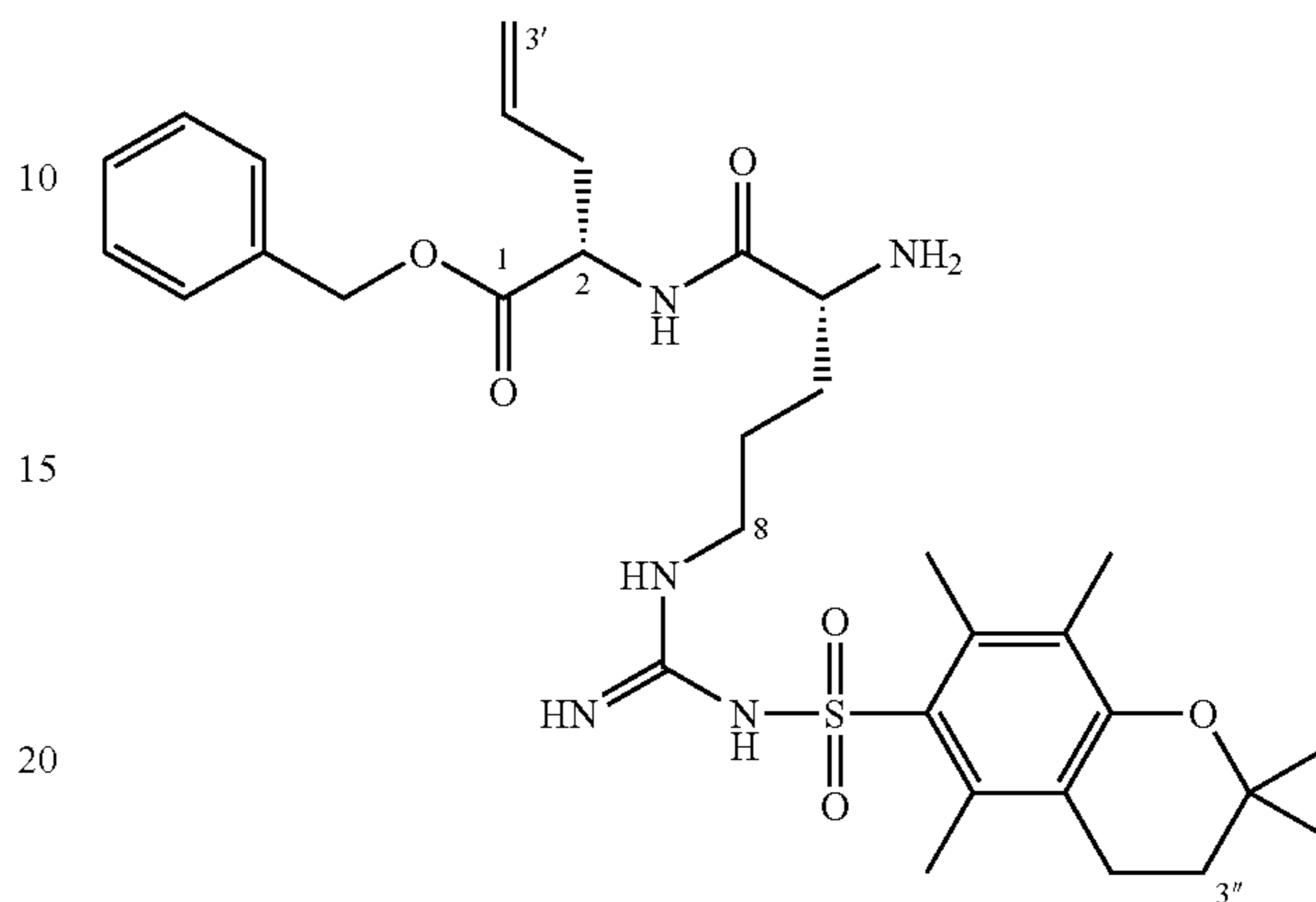
Benzyl(2S,5R)-2-allyl-5-amino-3-aza-8-[(2,2,5,7,8-pentamethyl-3,4-dihydro-2H-6-chromenylsulfonyl)guanidino]octanoate (110)
