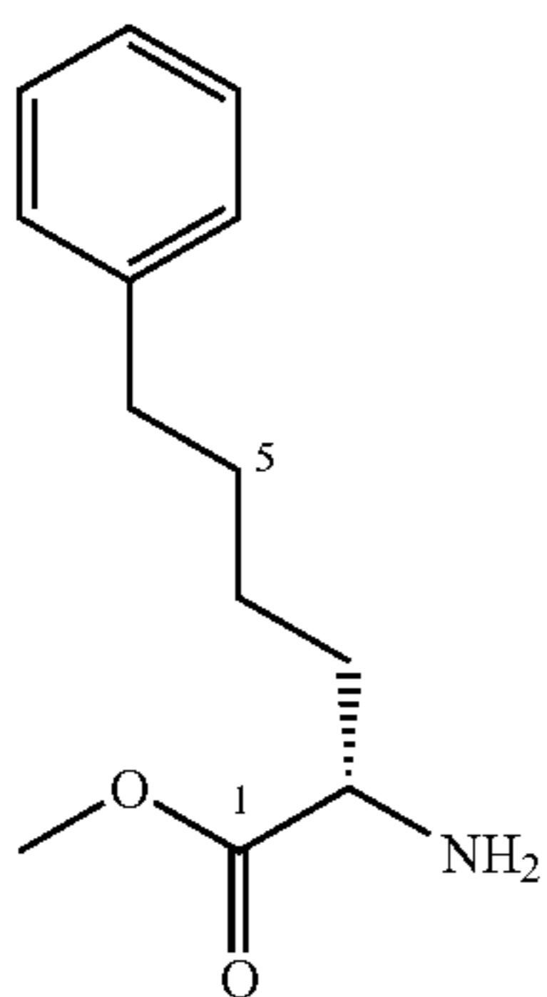
Methyl(2S)-2-amino-6-phenylhexanoate (175)
