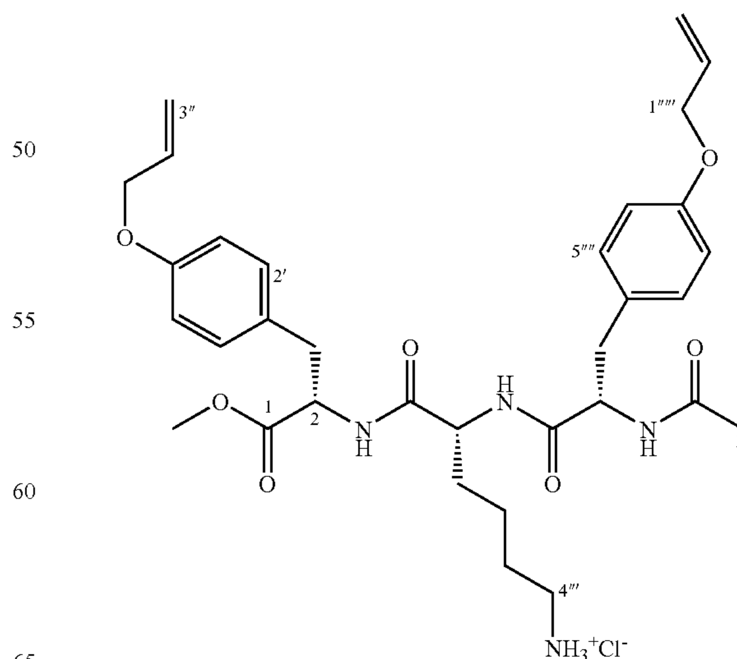
Methyl(2S,5R,8S)-2,8-di(4-allyloxybenzyl)-5-(4-aminobutyl)-3,6,9-triaza-4,7,10-trioxoundecanoate hydrochloride (83)
