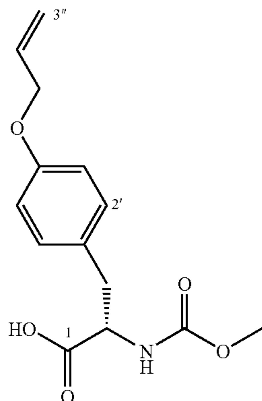
(2S)-3-(4-Allyloxyphenyl)-2-methoxycarboxamidopropanoic acid (172)
