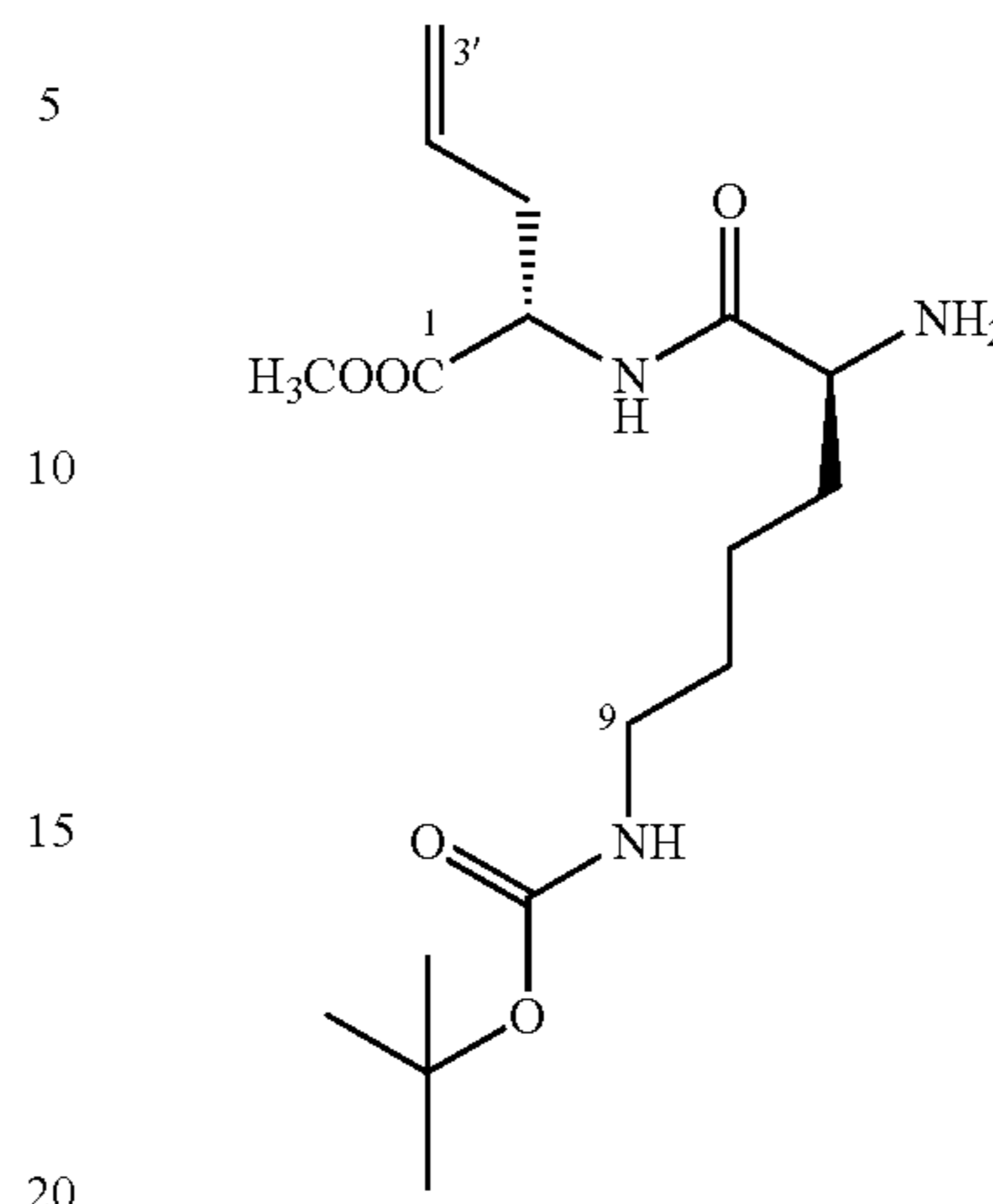
Methyl(2S,5S)-2-allyl-5-amino-3-aza-9-(tert-butoxycarboxamido)-4-oxononanoate (24)
