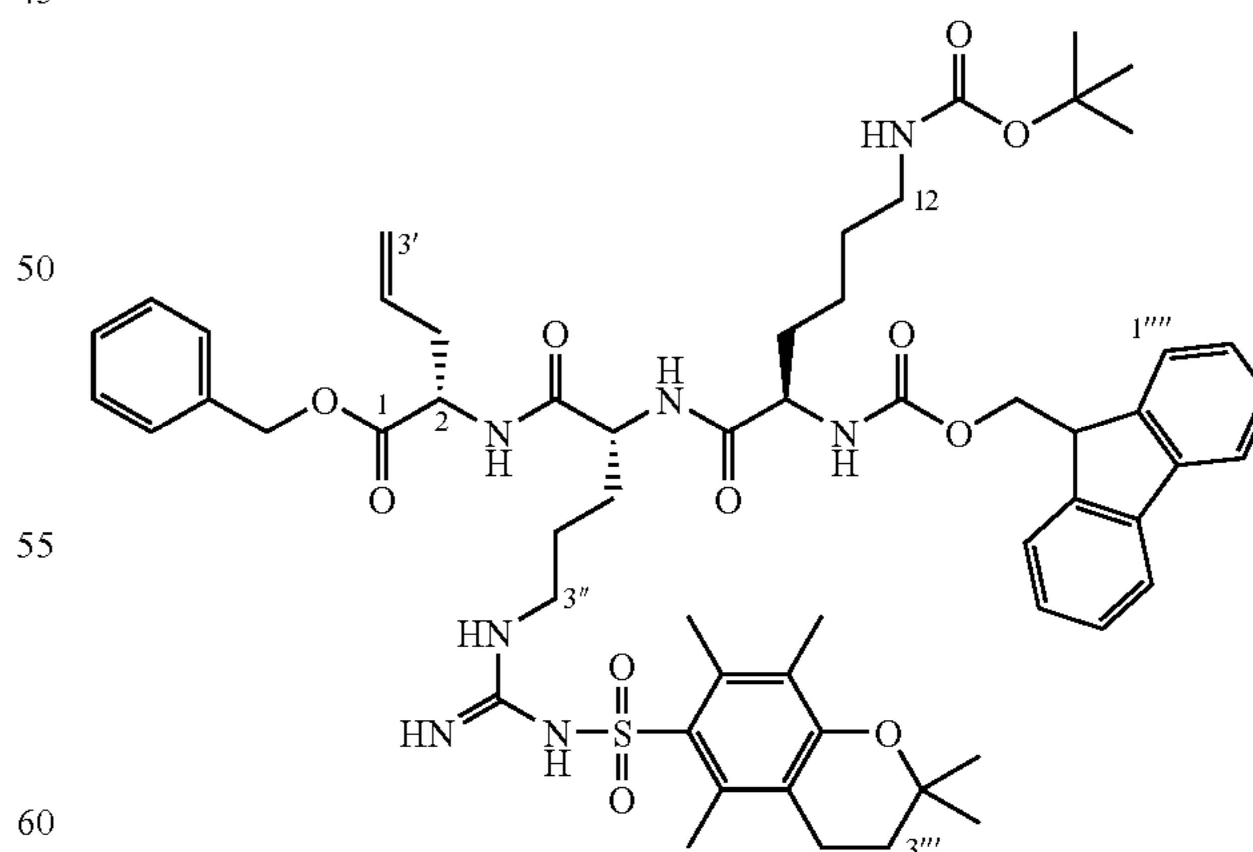
Benzyl(2S,5R,8R)-2-allyl-3,6-diaza-12-(tert-butoxycarboxamido)-8-(9H-9-fluorenylmethyloxycarboxamido)-5-[(2,2,5,7,8-pentamethyl-3,4-dihydro-2H-6-chromenylsulfonyl)guanidino]propyl)-4,7-dioxododecanoate (111)
