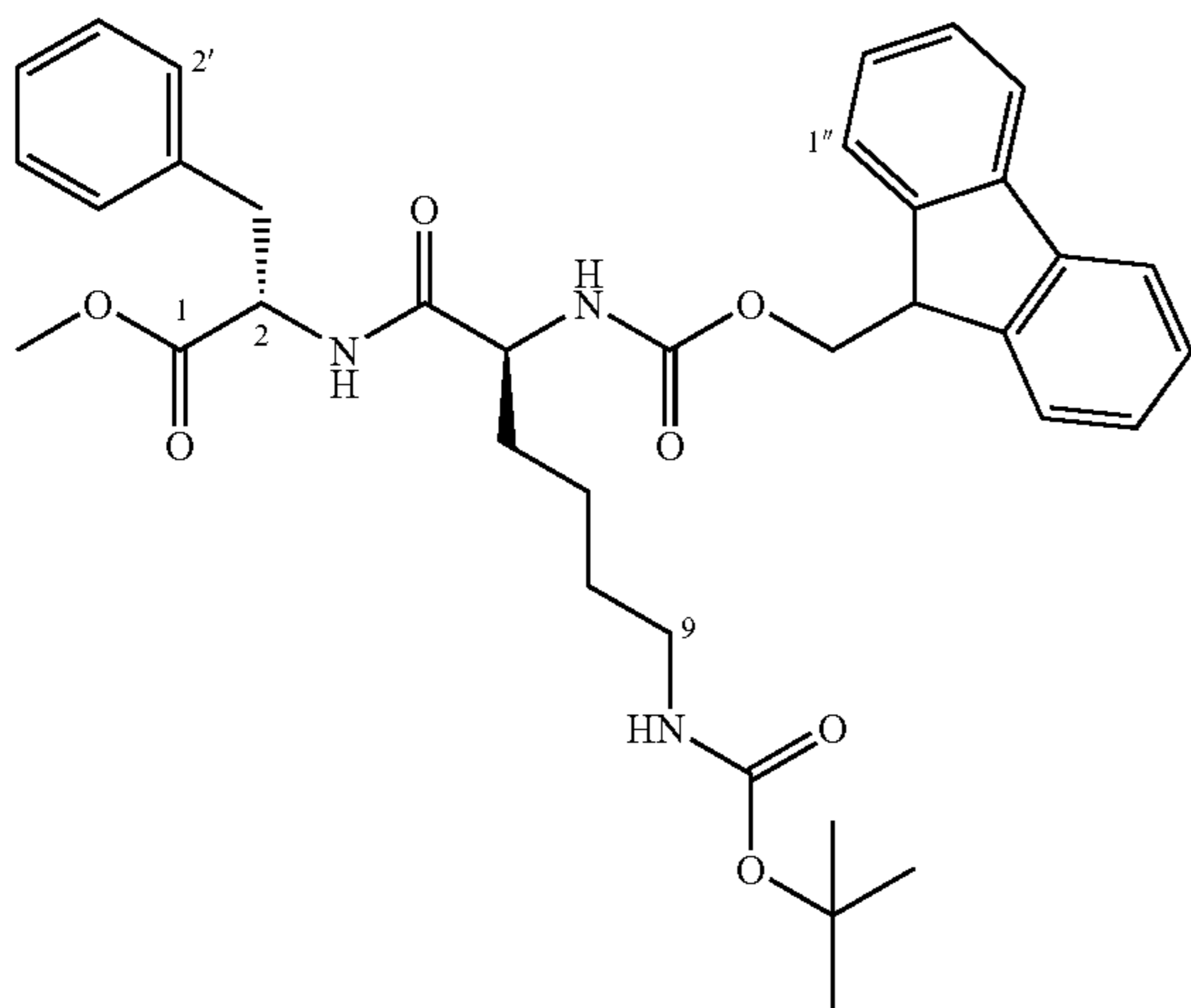
Methyl(2S,5S)-3-aza-2-benzyl-9-(tert-butoxycarboxamido)-5-(9H-9-fluorenylmethylloxycarboxamido)-4-oxononanoate (176)
