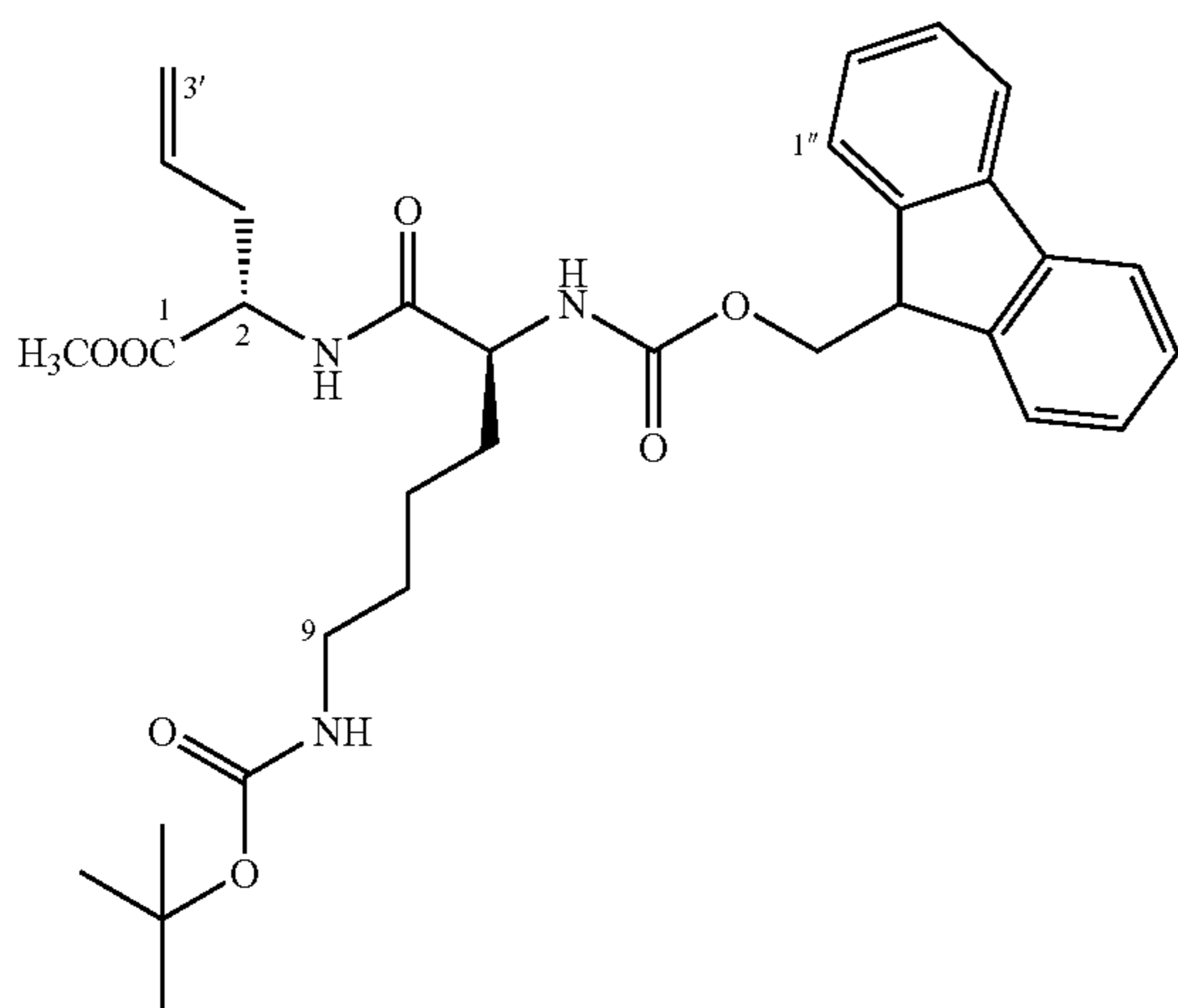
Methyl(2S,5S)-2-allyl-3-aza-9-(tert-butoxycarboxamido)-5-(9H-9-fluorenylmethyloxycarboxamido)-4-oxononanoate (23)
