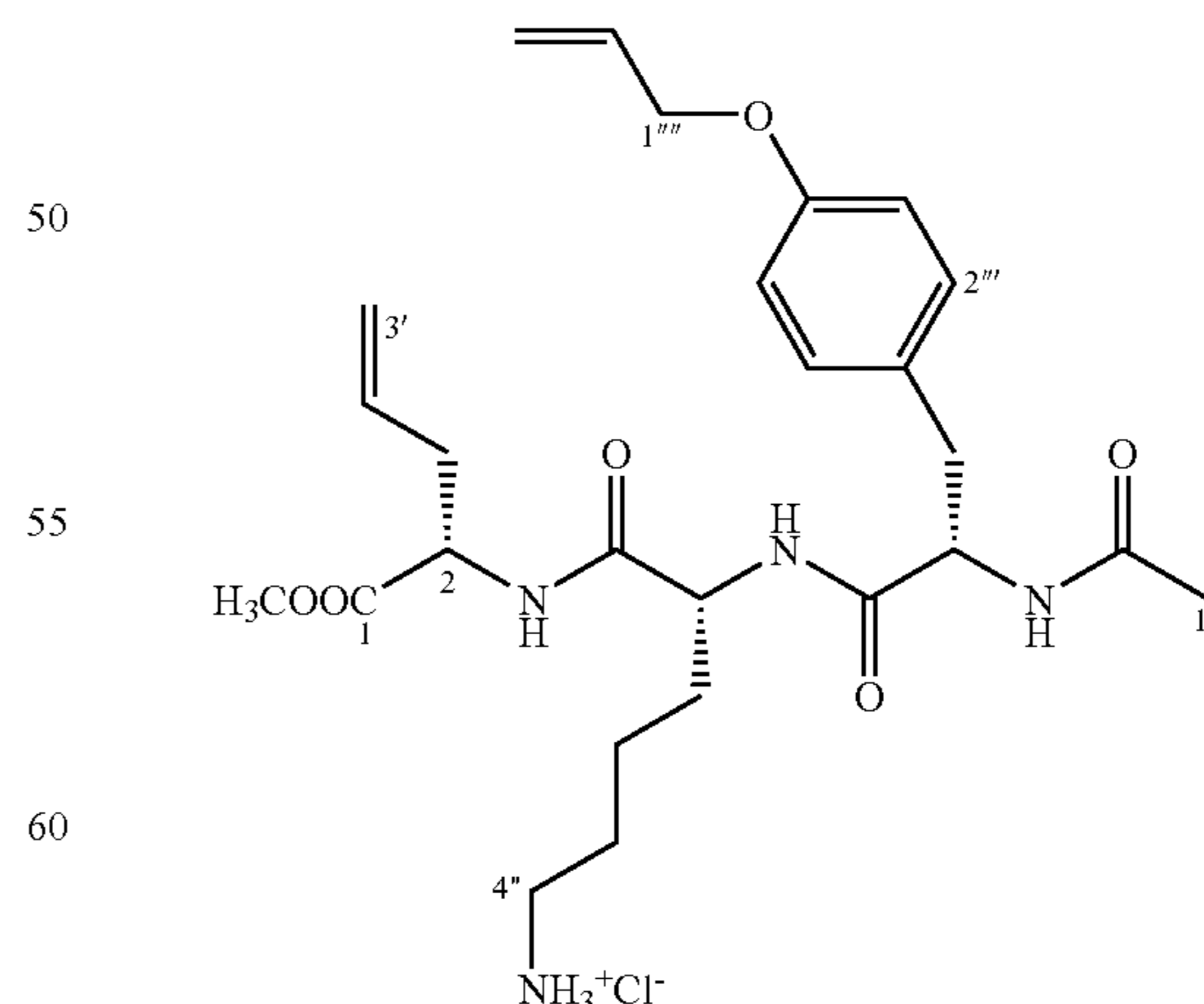
Methyl(2S,5R,8S)-2-allyl-8-(4-allyloxyphenyl)-5-(4-aminobutyl)-3,6,9-triaza-4,7,10-trioxoundecanoate hydrochloride (77)
