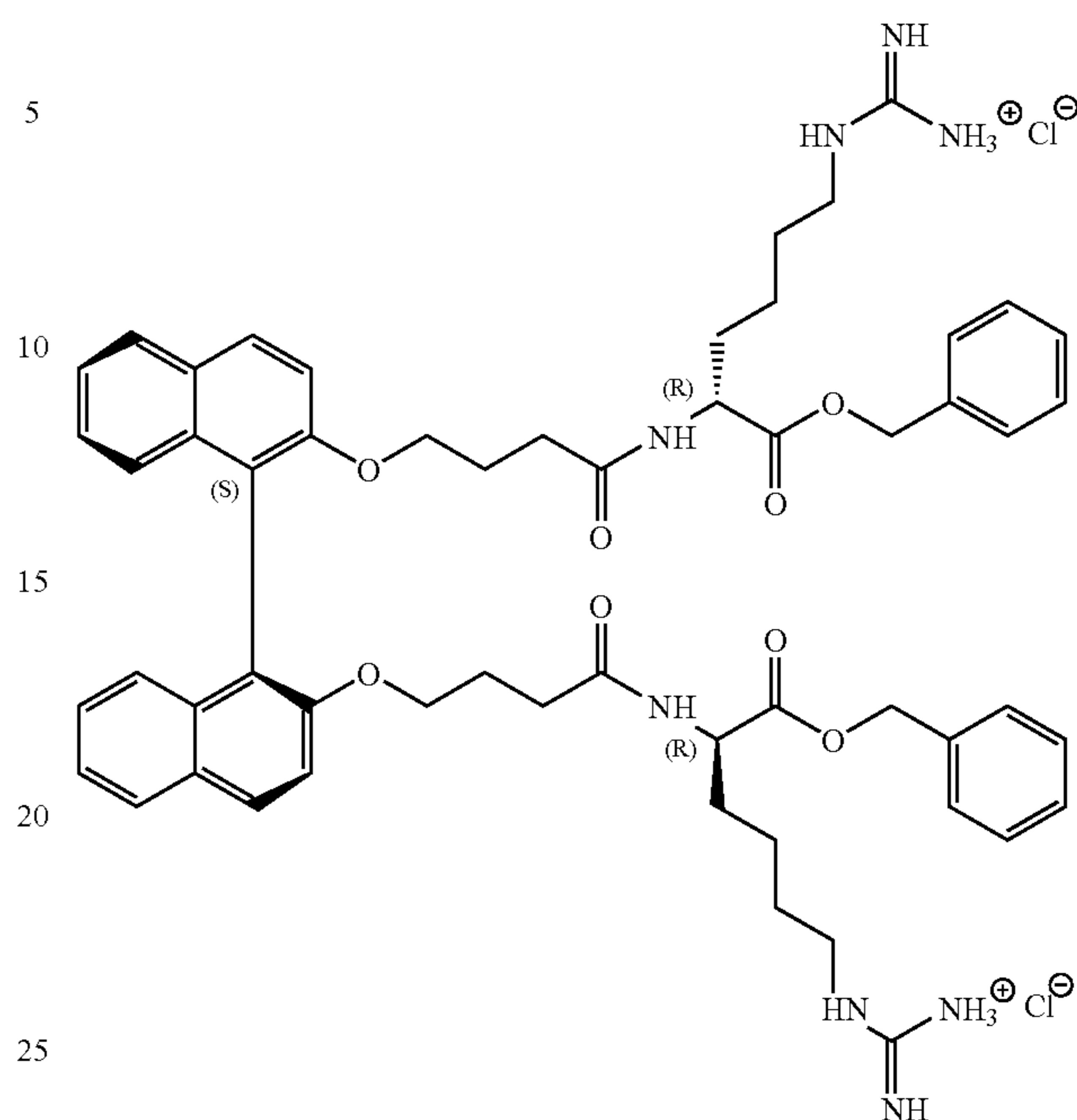
Compound 39
