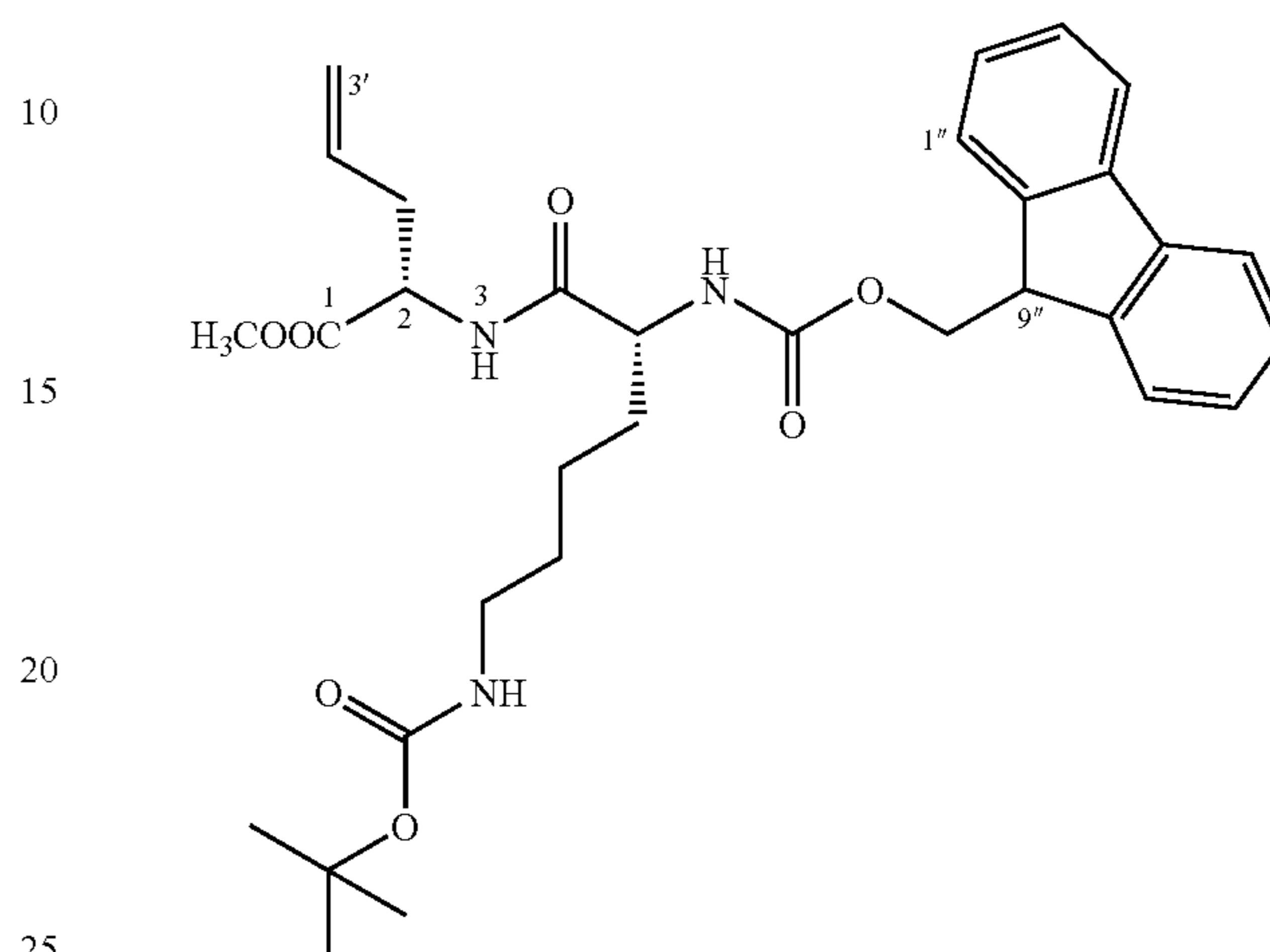
Methyl(2S,5R)-2-allyl-3-aza-9-(tert-butoxycarboxamido)-5-(9H-9-fluorenylmethyloxycarboxamido)-4-oxononanoate (19)
