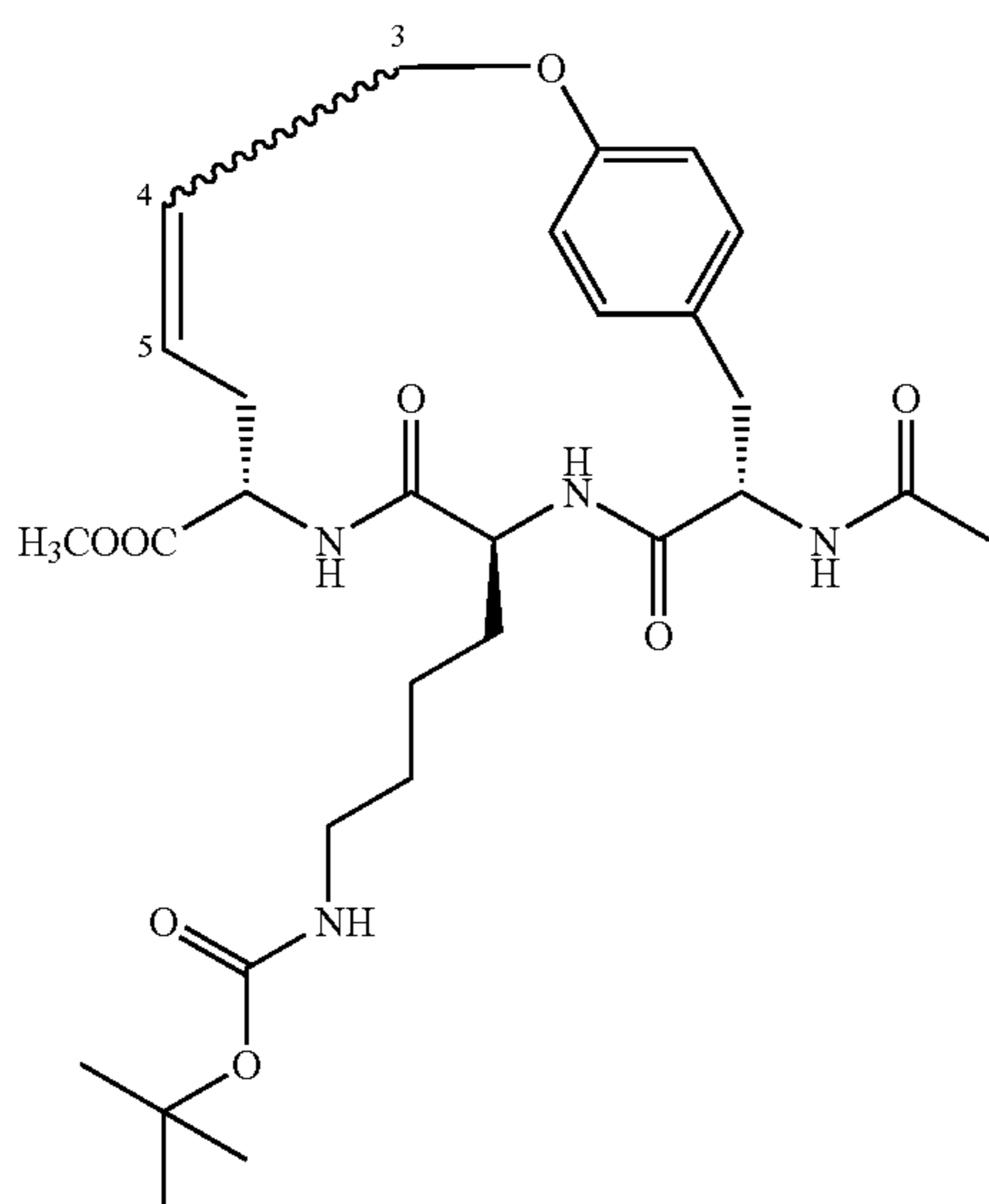
(7S,10S,13S,4E/Z)-13-Acetamido-8,11-diaza-10-(4-(tert-butoxycarbonylamido)butyl)-7-methoxycarbonyl-2-oxa-9,12-dioxo-1(1,4)phenylenacyclotetradecaphane-4-ene (26)
