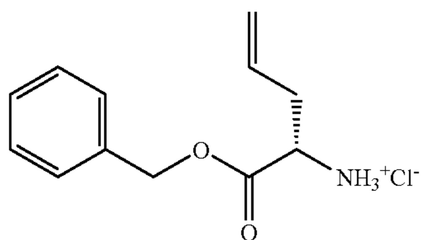
Benzyl(2S)-2-amino-4-pentenoate hydrochloride (108)
