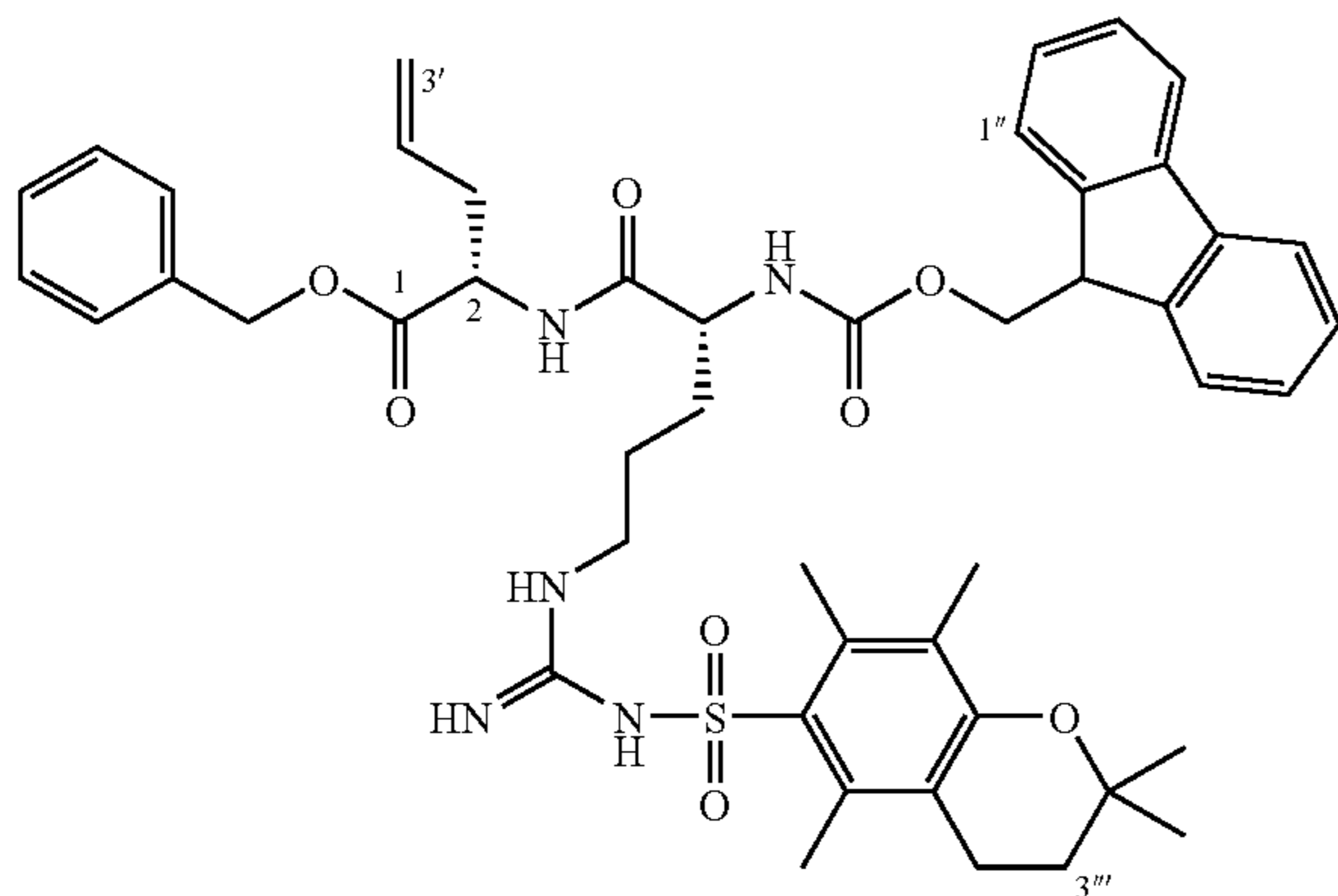
Benzyl(2S,5R)-2-allyl-3-aza-5-(9H-9-fluorenylmethyloxycarboxamido)-4-oxo-8-[(2,2,5,7,8-pentamethyl-3,4-dihydro-2H-6-chromenylsulfonyl)guanidino]octanoate (109)
