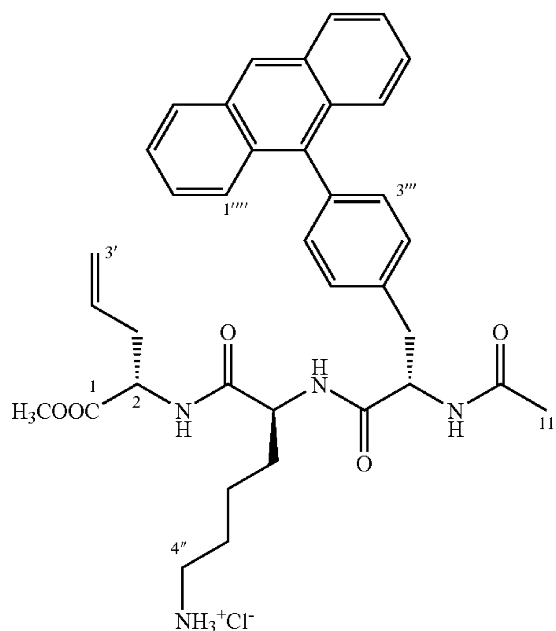
Methyl(2S,5S,8S)-2-allyl-5-(4-aminobutyl)-8-(4-[9-anthracenyl]benzyl)-3,6,9-triaza-5-butylamino-4,7,10-trioxoundecanoate hydrochloride (118)
