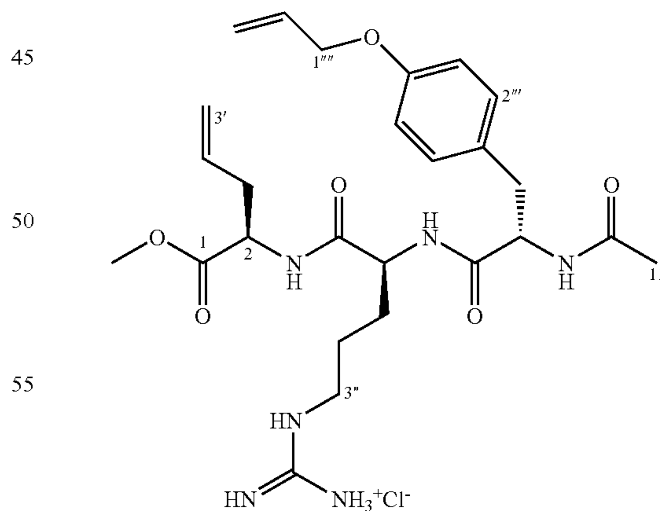
Methyl(2R,5S,8S)-2-allyl-8-(4-allyloxybenzyl)-3,6,9-triaza-5-(3-[guanidino]-4,7,10-oxoundecanoate hydrochloride (80)
