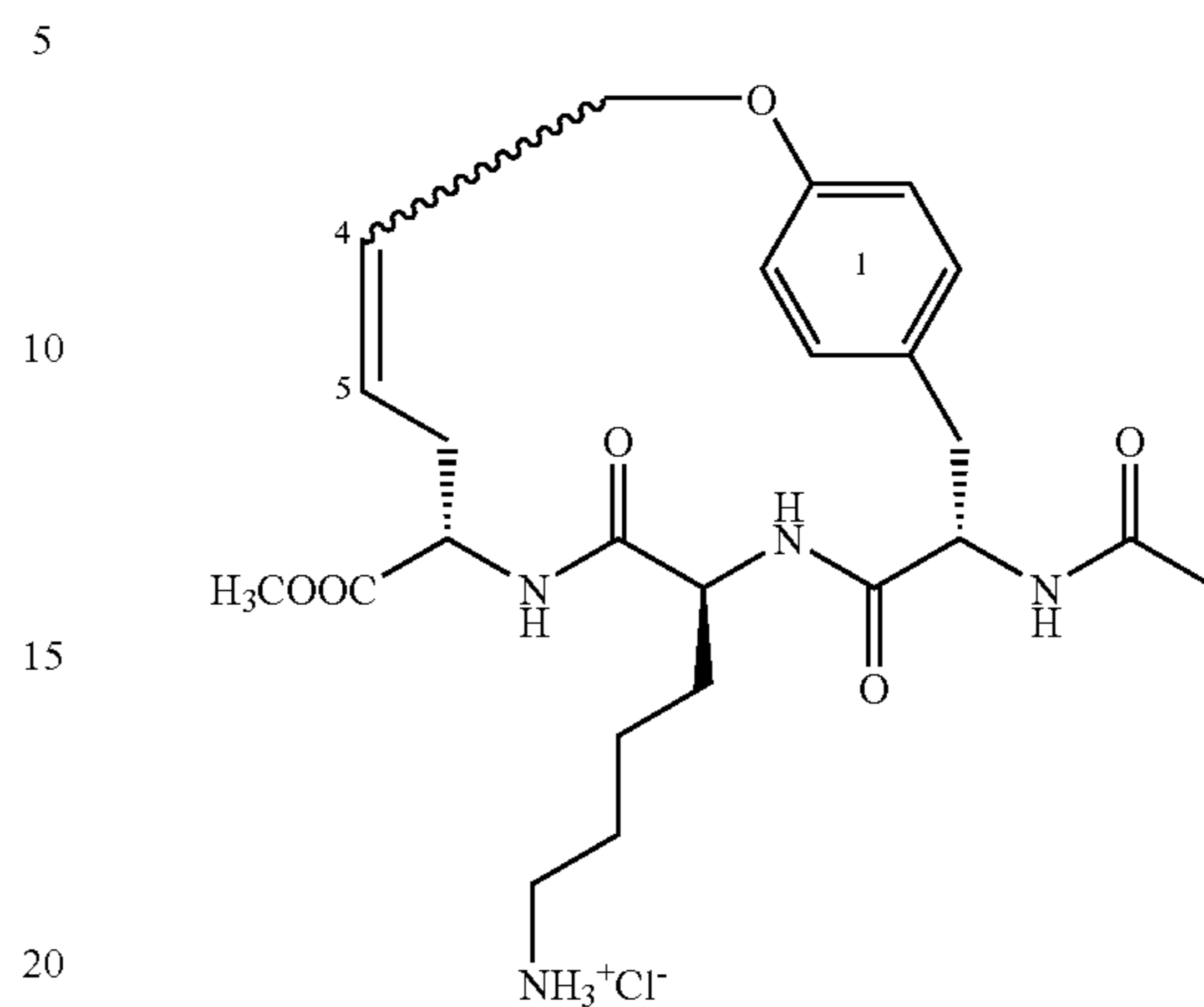
(7S,10S,13S,4E/Z)-13-Acetamido-10-(4-aminobutyl)-8,11-diaza-7-methoxycarbonyl-2-oxa-9,12-dioxo-1(1,4)phenylenacyclotetradecaphane-4-ene hydrochloride (27)
