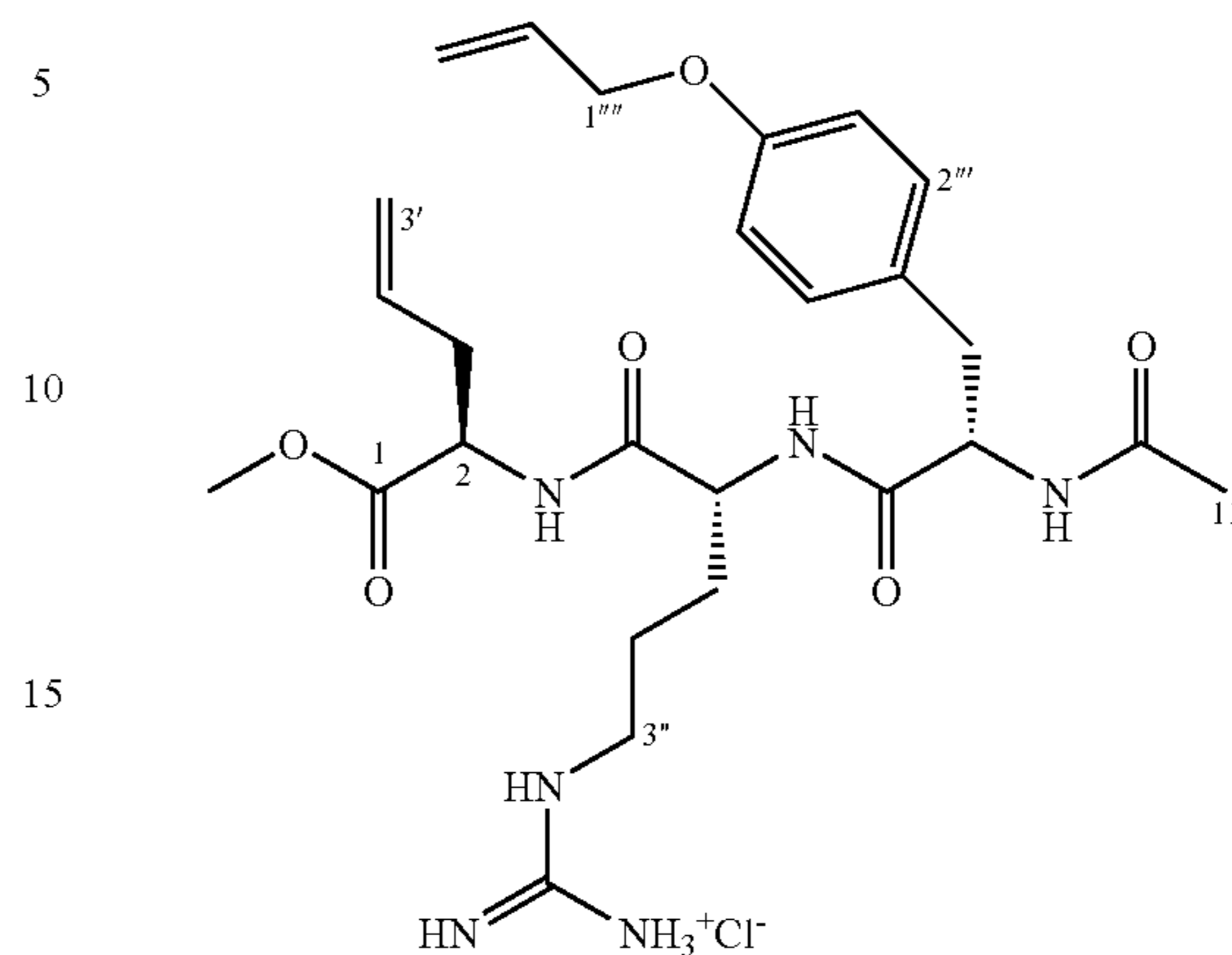
Methyl(2R,5R,8S)-2-allyl-8-(4-allyloxybenzyl)-3,6,9-triaza-5-(3-[guanidino]-4,7,10-oxoundecanoate hydrochloride (79)
