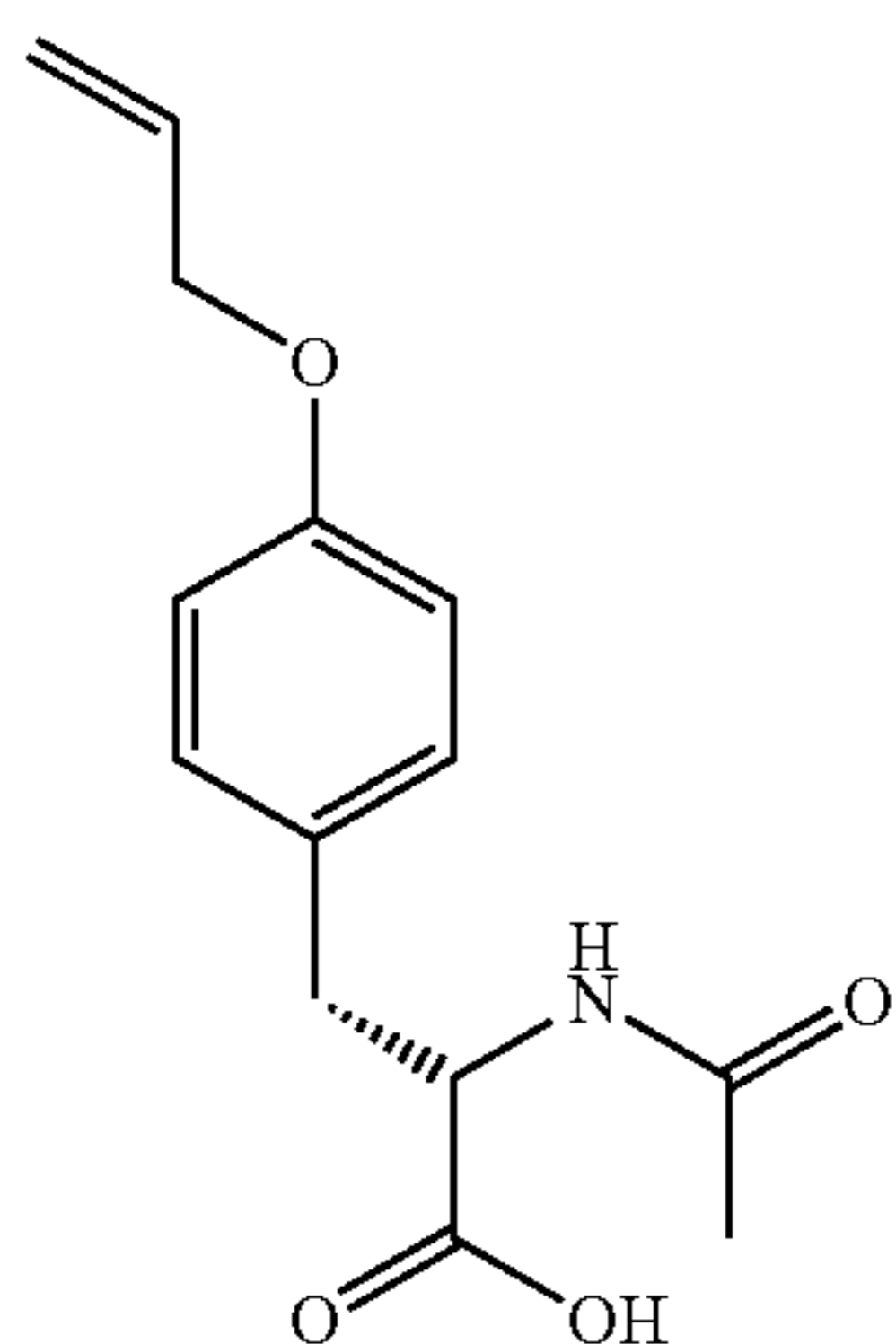
(2S)-2-Acetamido-3-(4-allyloxyphenyl)propanoic acid (16)
