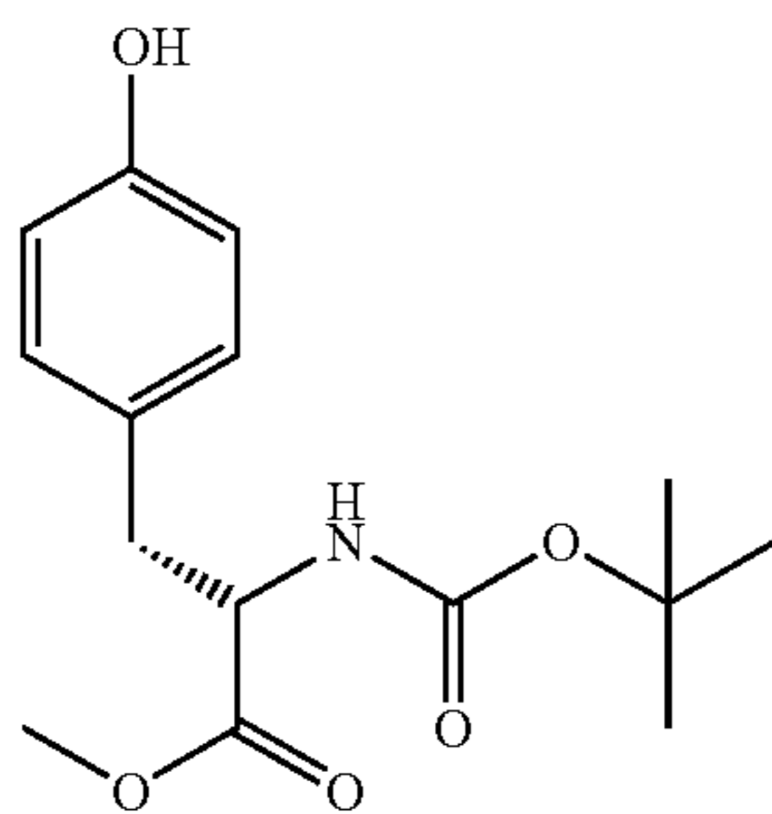
Methyl(2S)-(4-hydroxyphenyl)-2-tert-butoxycarboxamido propanoate (58)
