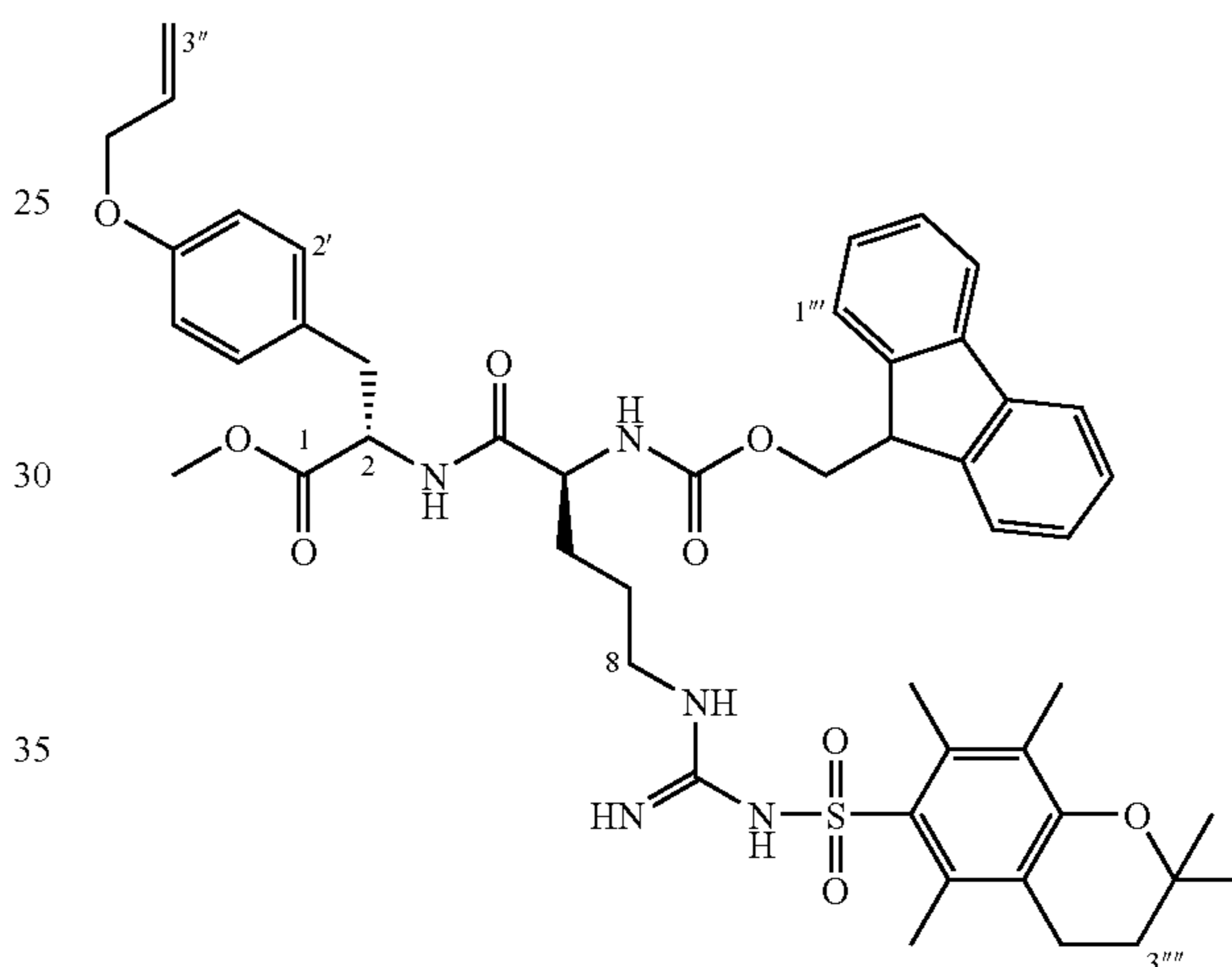
Methyl(2S,5R)-2-(4-allyloxybenzyl)-3-aza-5-(9H-9-fluorenylmethylcarboxamido)-4-oxo-8-[(2,2,5,7,8-pentamethyl-3,4-dihydro-2H-6-chromenylsulfonyl)guanidino]nonanoate (67)
