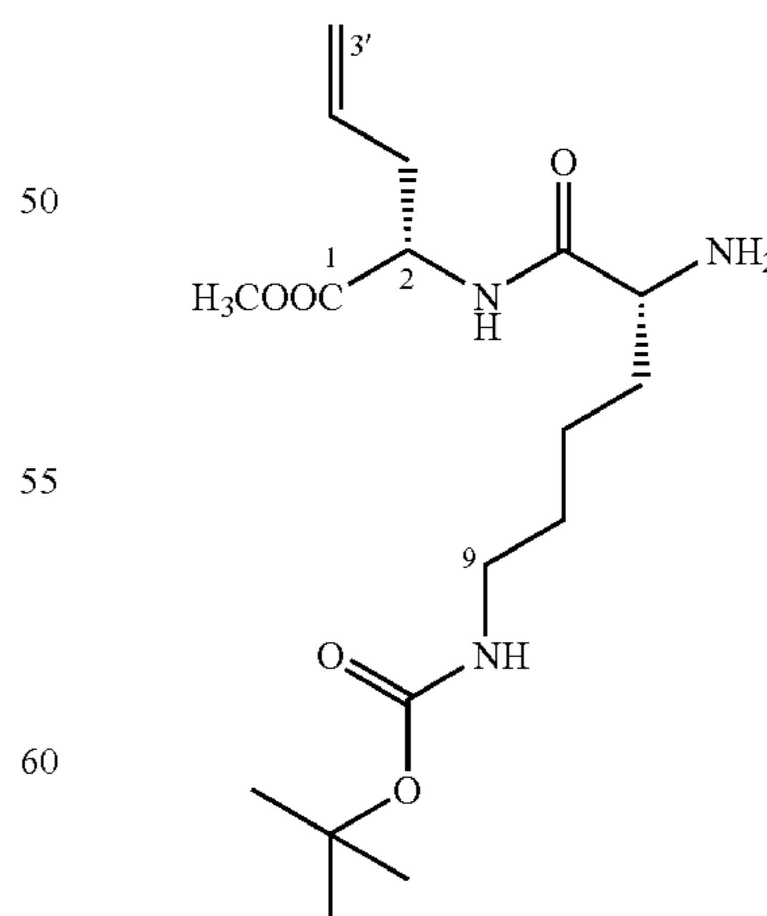
Methyl(2S,5R)-2-allyl-5-amino-3-aza-9-(tert-butoxycarboxamido)-4-oxononanoate (20)
