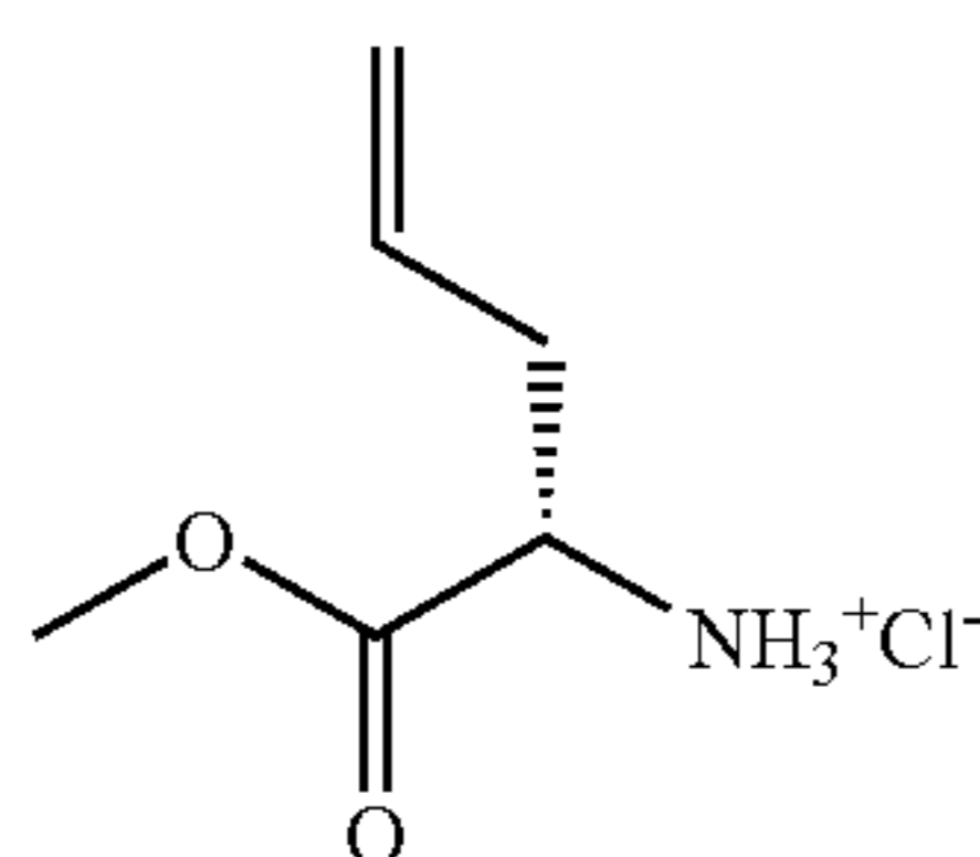
Methyl(2S)-2-amino-4-pentenoate hydrochloride (18)
