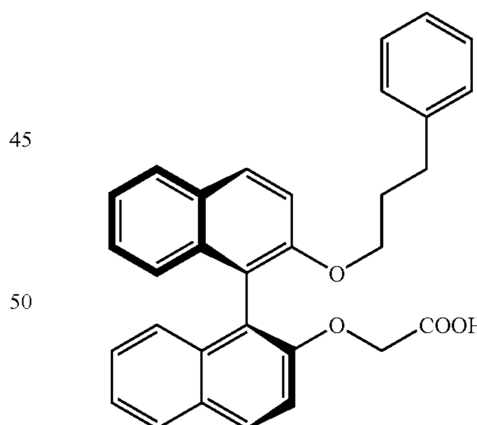
(2'-(3-Phenylpropyloxy)-[1,1']-(S)-binaphthalen-2-yloxy)-acetic acid (107)
