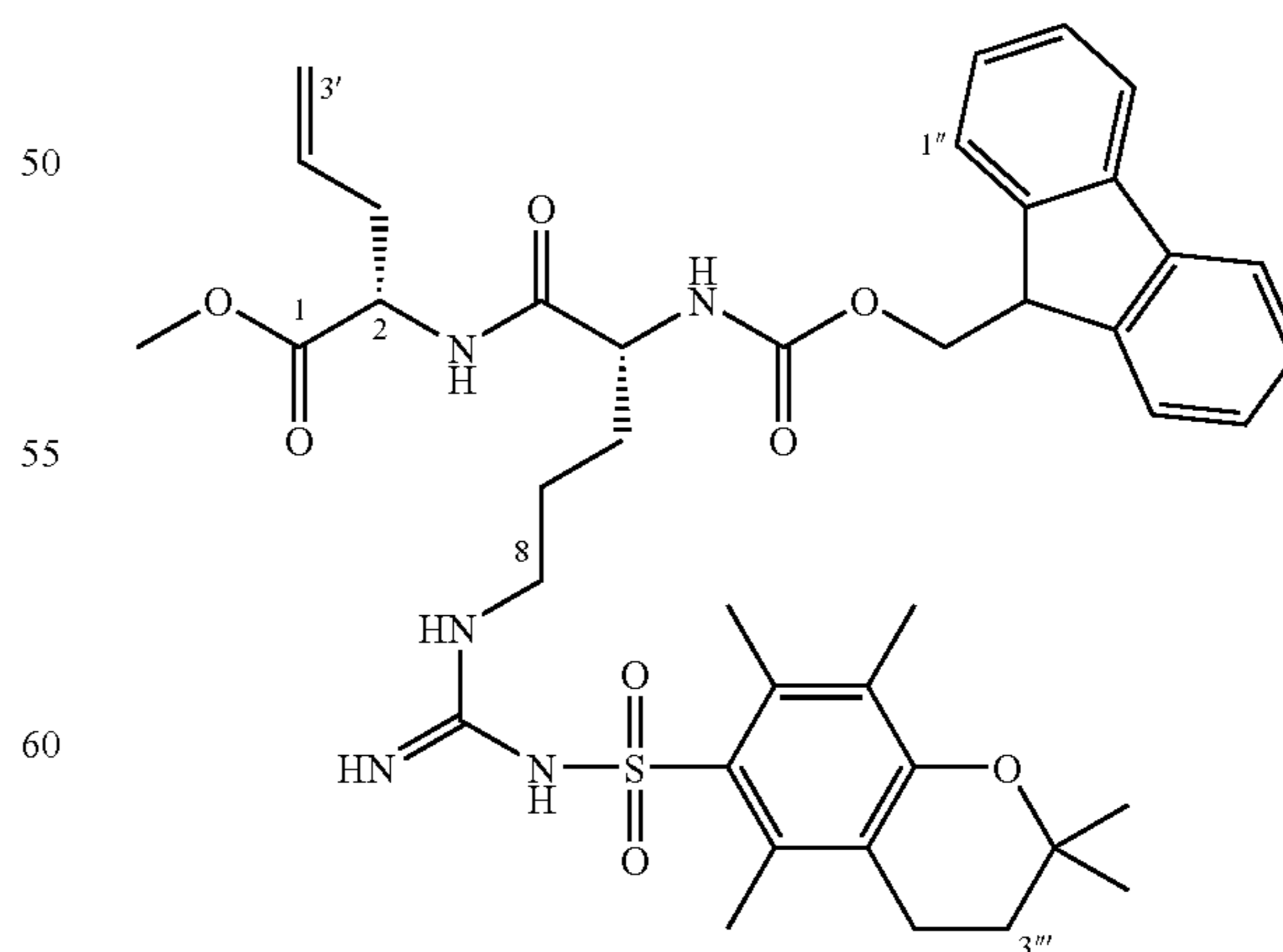
Methyl(2S,5R)-2-allyl-3-aza-5-(9H-9-fluorenylmethyloxycarbonylamido)-8-[(2,2,5,7,8-pentamethyl-3,4-dihydro-2H-6-chromenylsulfonyl)guanidino]-4-oxooctanoate (28)
