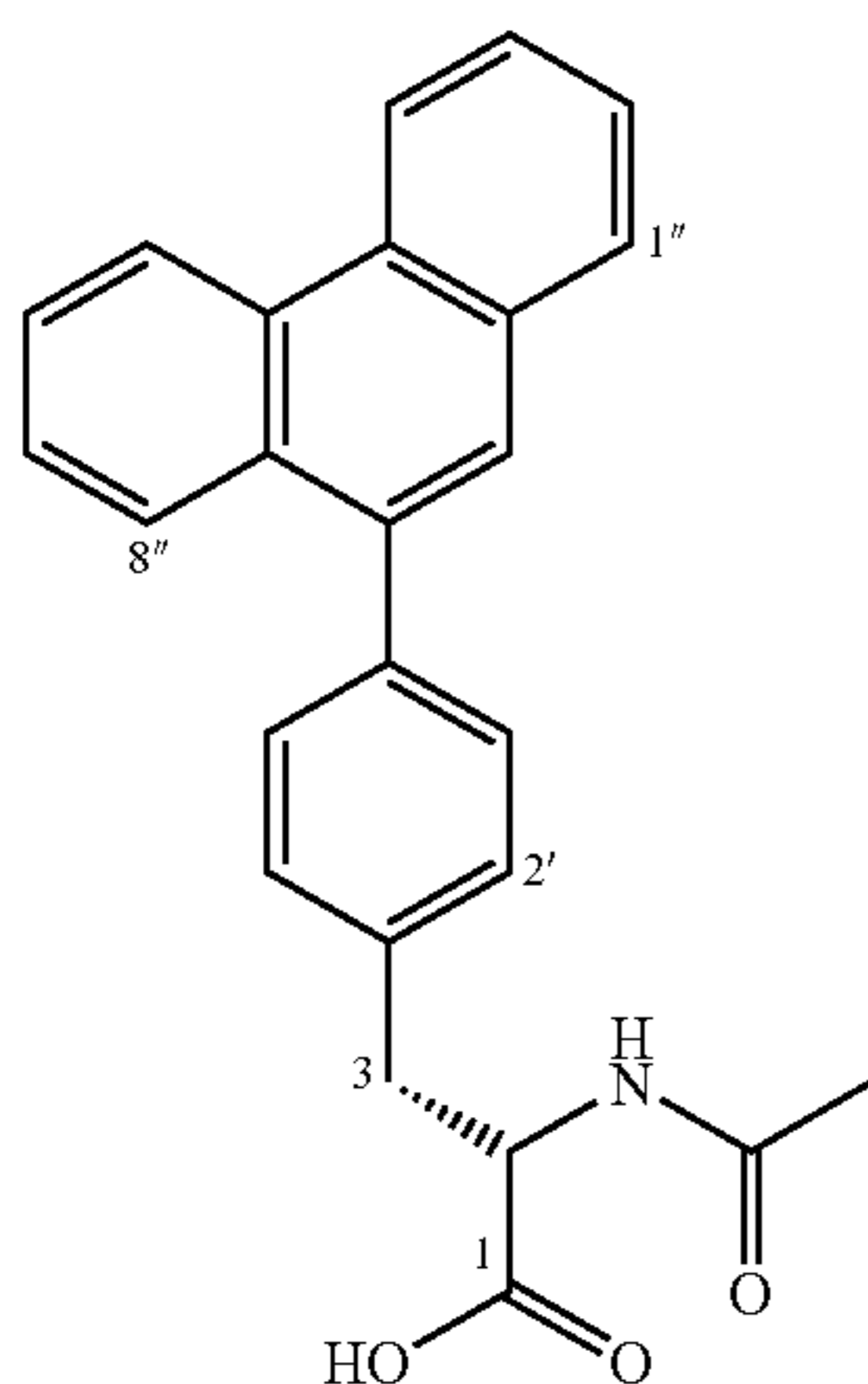
(2S)-2-Acetamido-3-(4-[9-phenanthrenyl]phenyl)propanoic acid (99)
