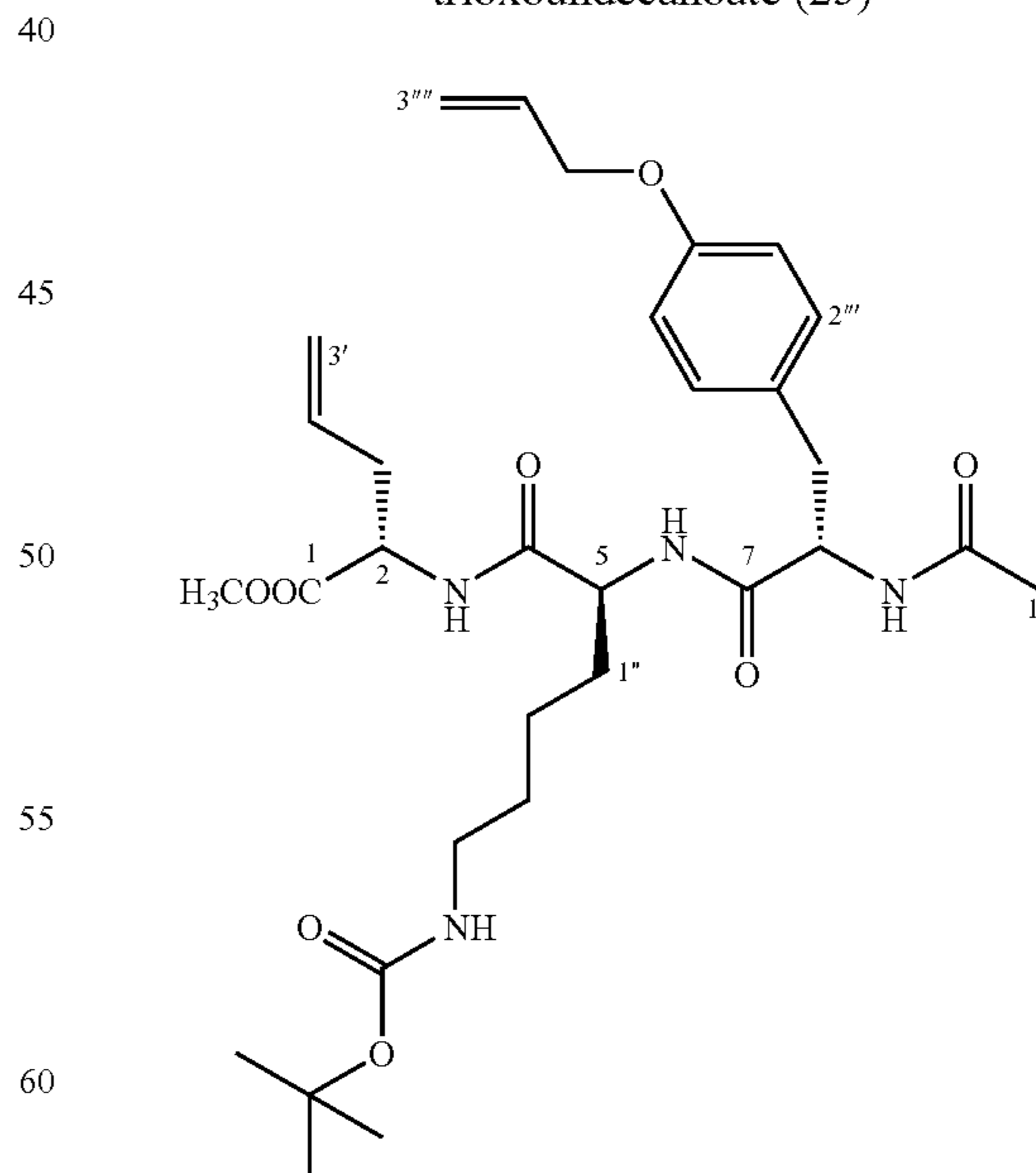
Methyl(2S,5S,8S)-2-allyl-8-(4-allyloxybenzyl)-3,6,9-triaza-5-(4-[tert-butoxycarboxamido]butyl)-4,7,10-trioxoundecanoate (25)
