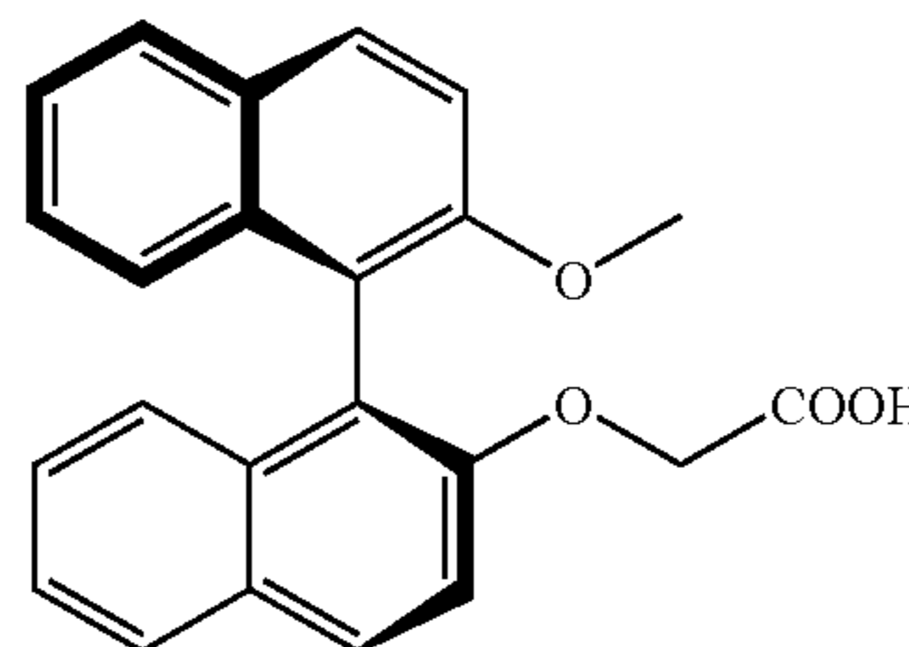
(2'-Methyloxy-[1,1']-(S)-binaphthalen-2-yloxy)-acetic acid (103)
