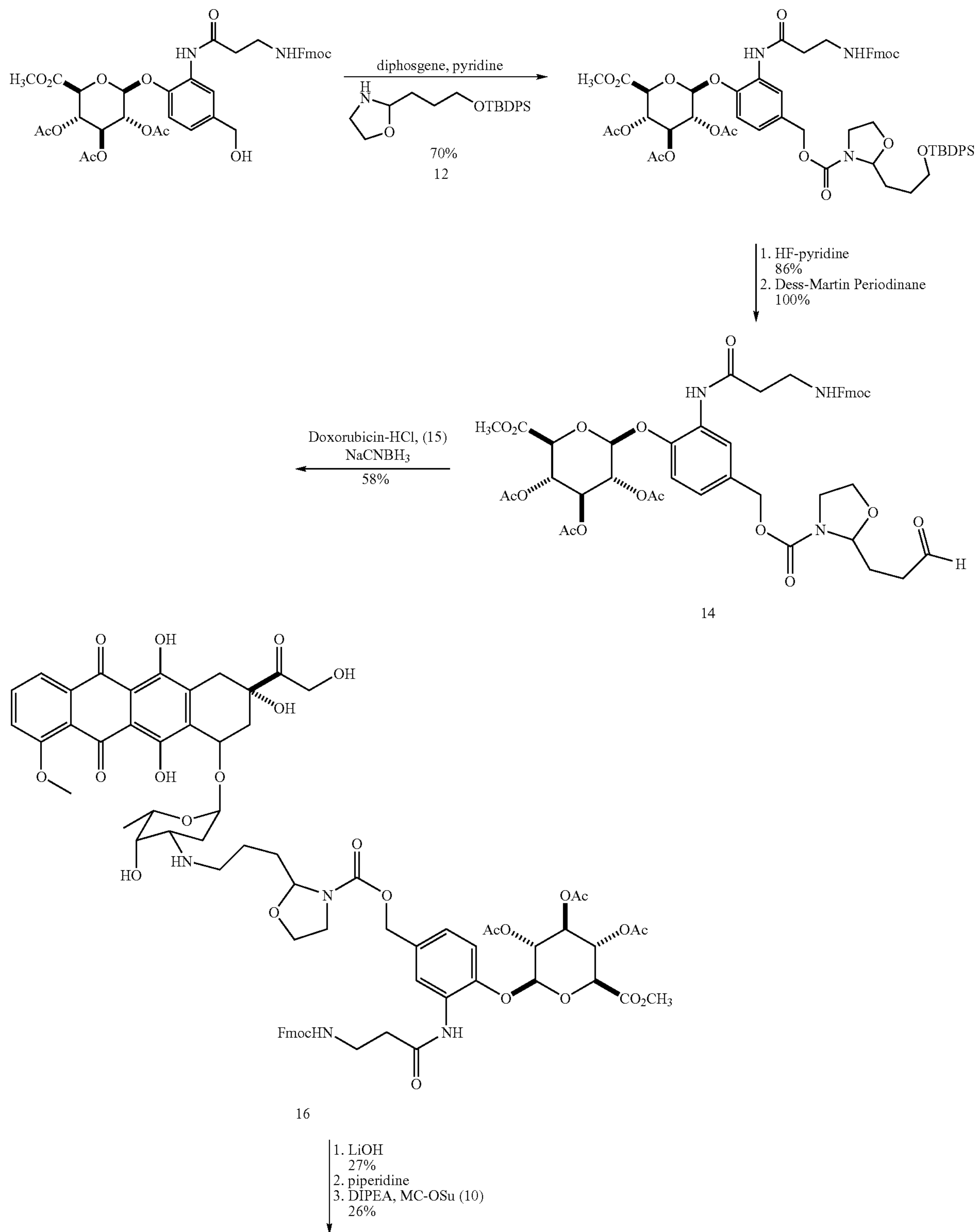
Scheme 4
