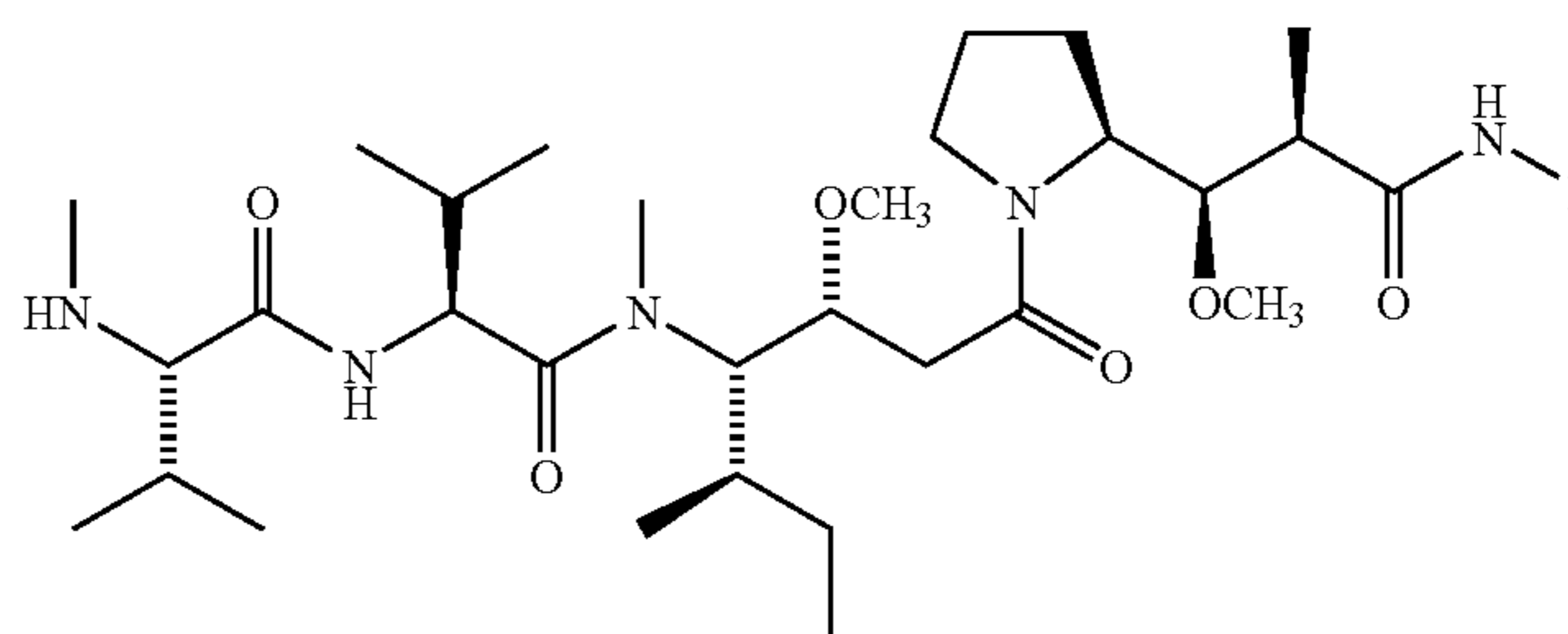
Monomethyl auristatin E (MMAE; 1a) R = 1S, 2R-norephedrine Monomethyl auristatin F (MMAF; 1b) R = phenylalanine
