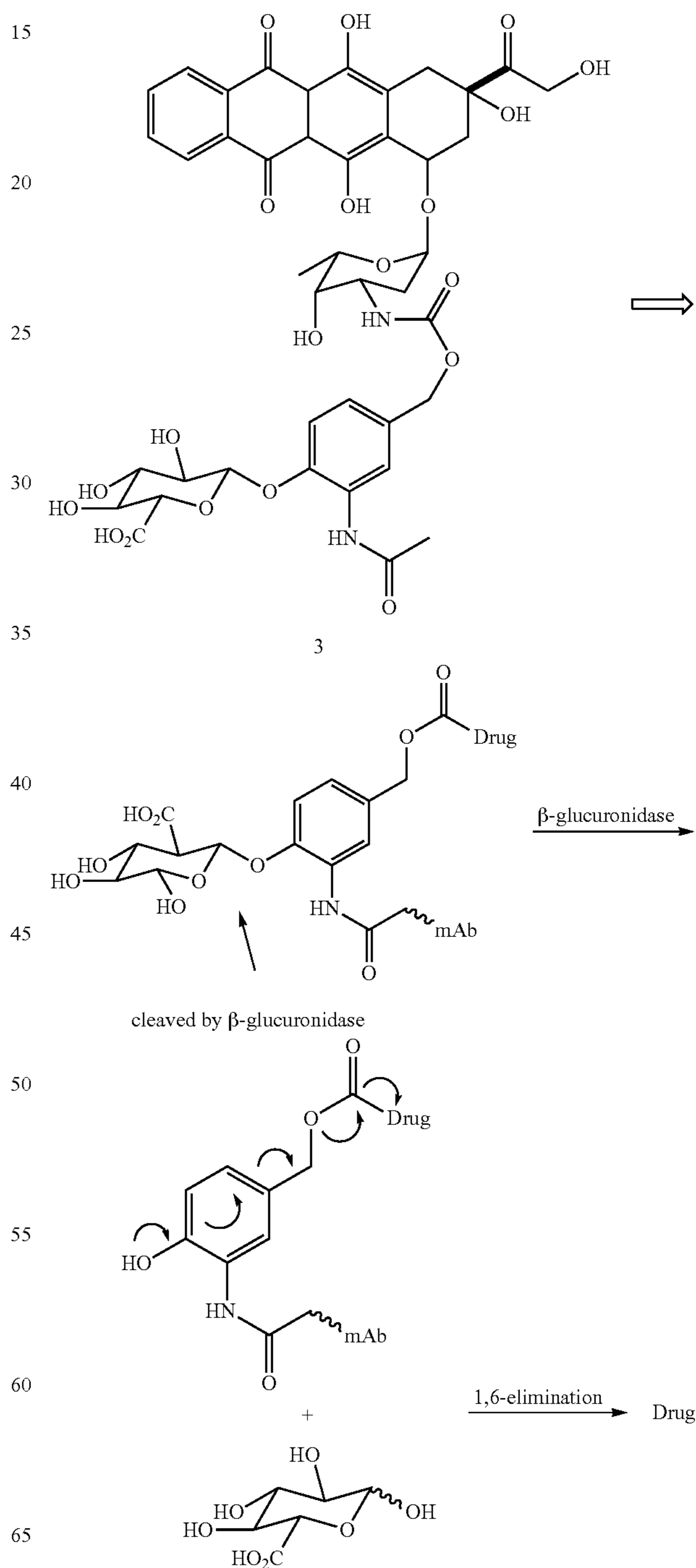
Scheme 1.
