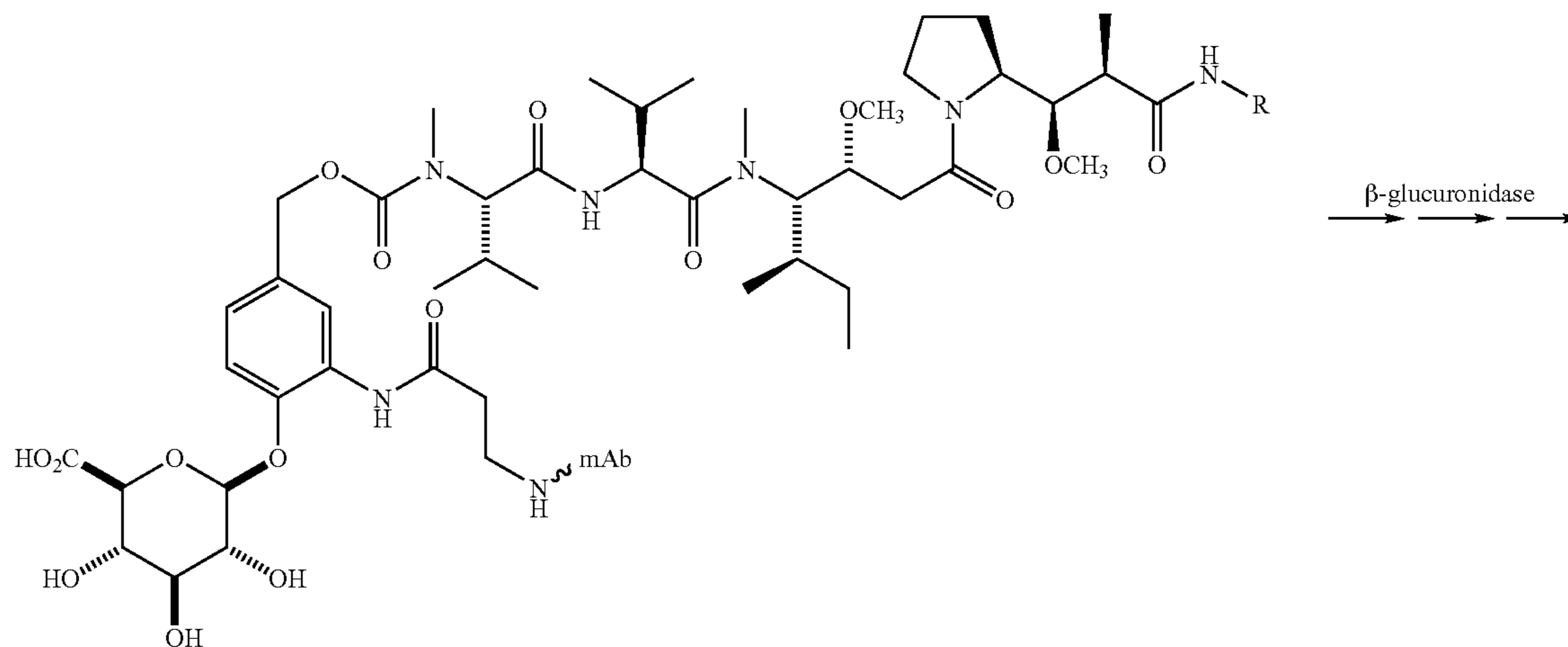
Scheme 2.
