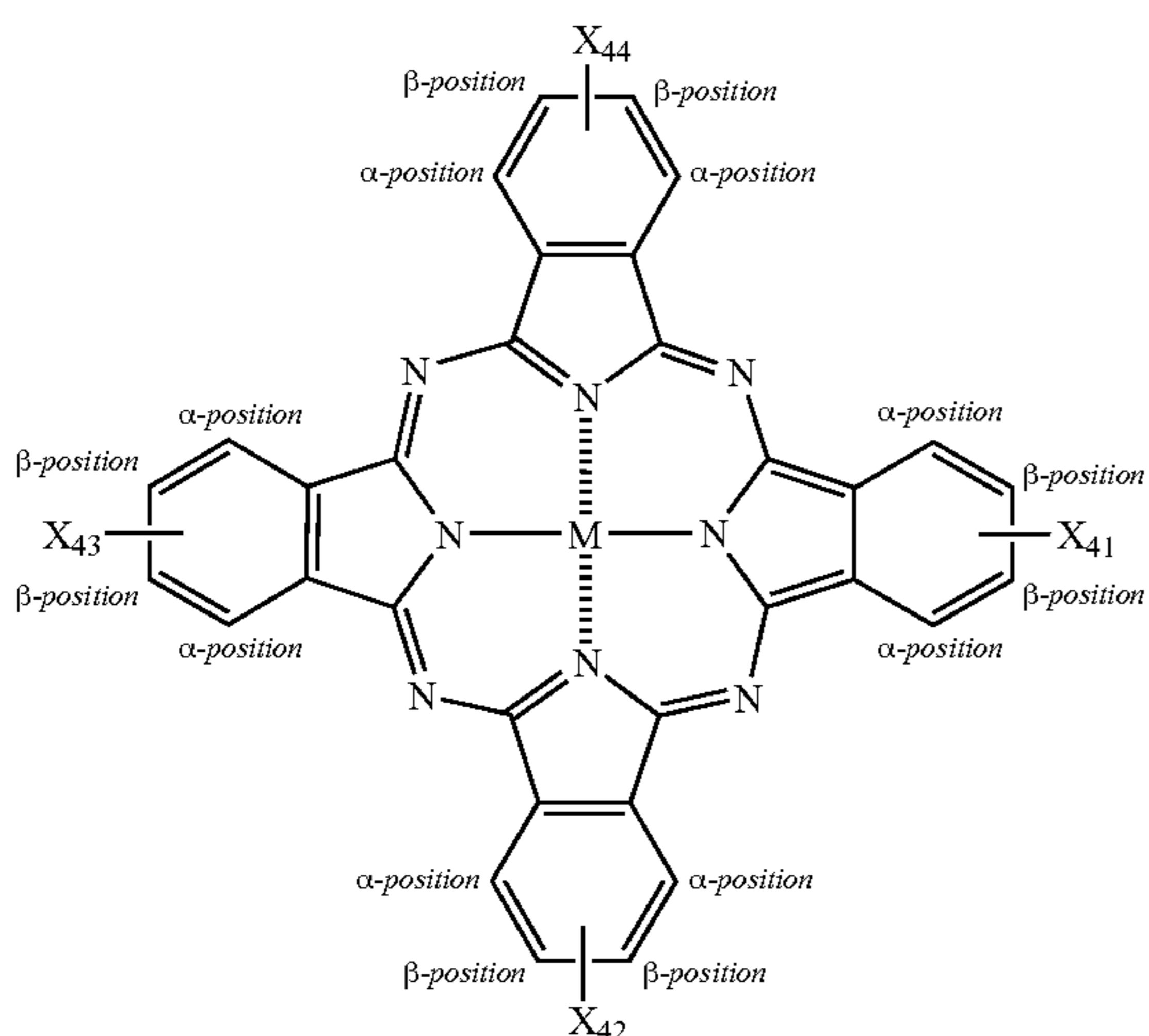
Formula (V)
