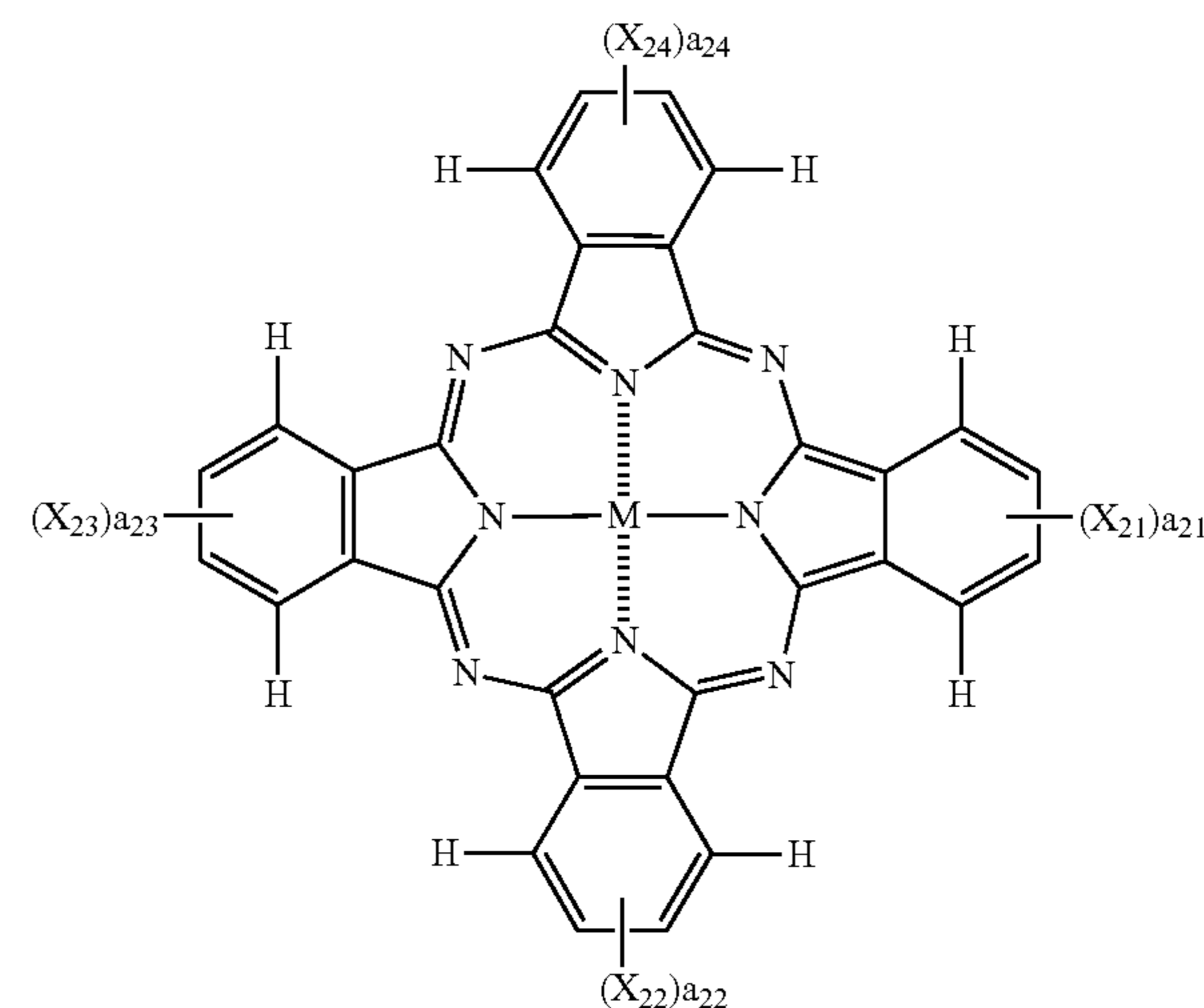
Formula (III)
