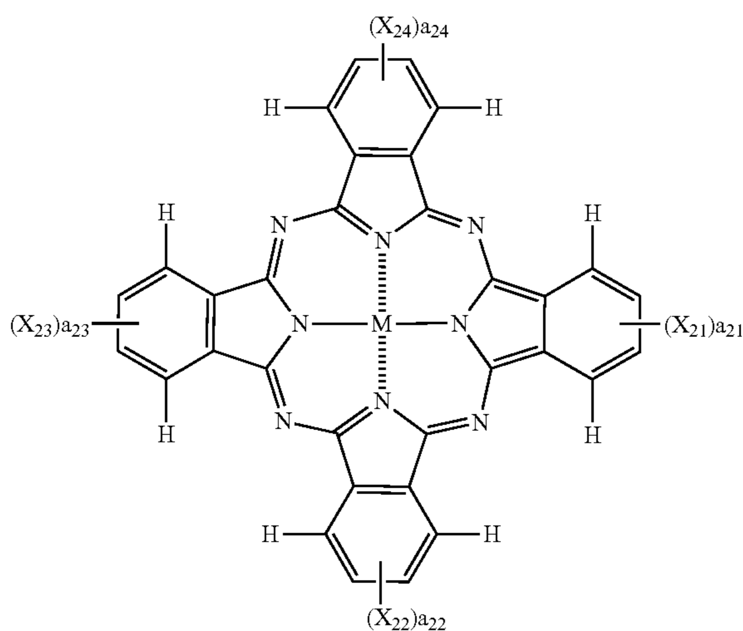
Formula (III)
