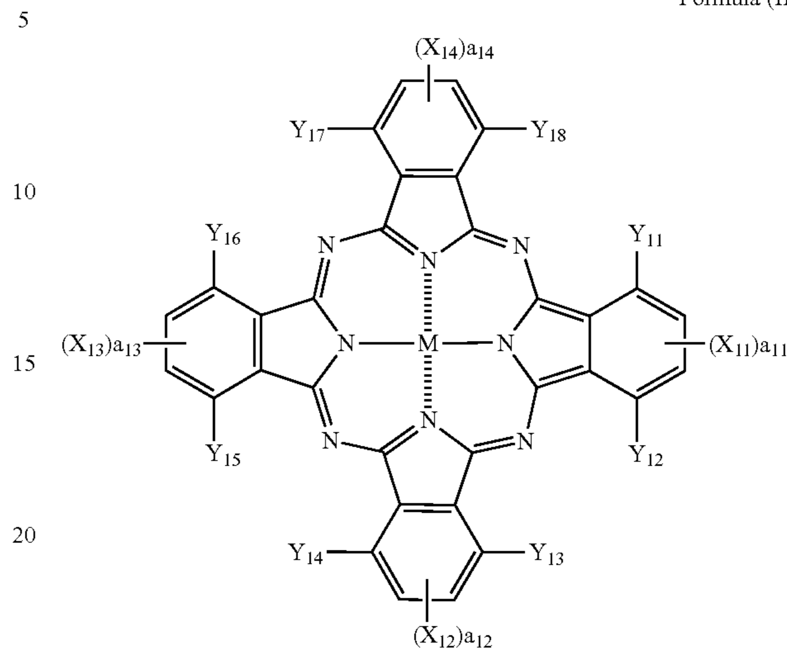
Formula (II)
