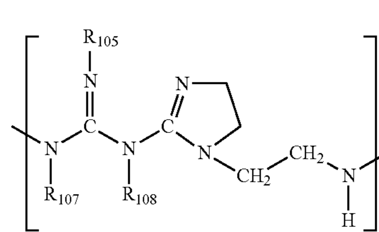
Formula (2-Ac)
