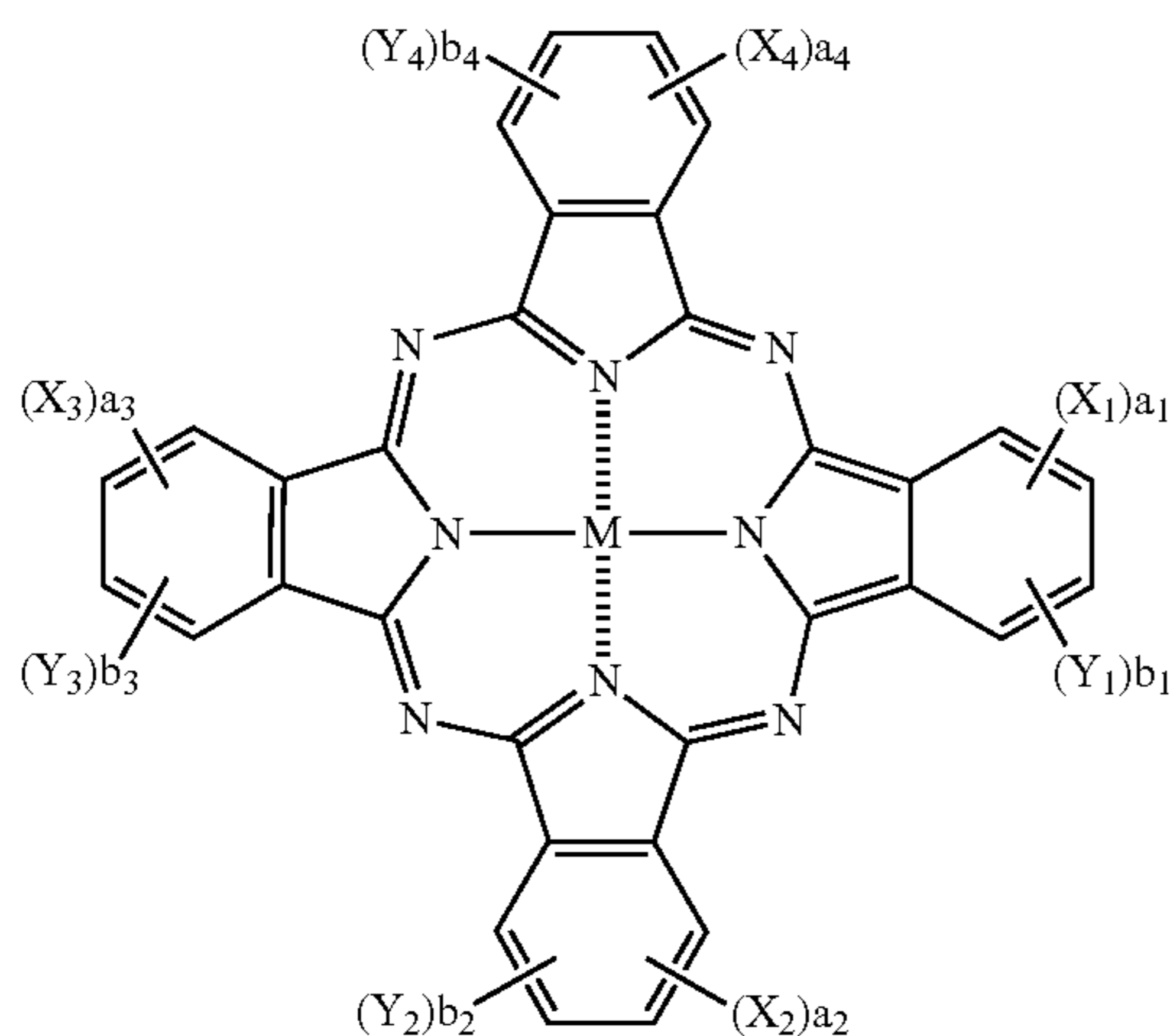
Formula (I)
