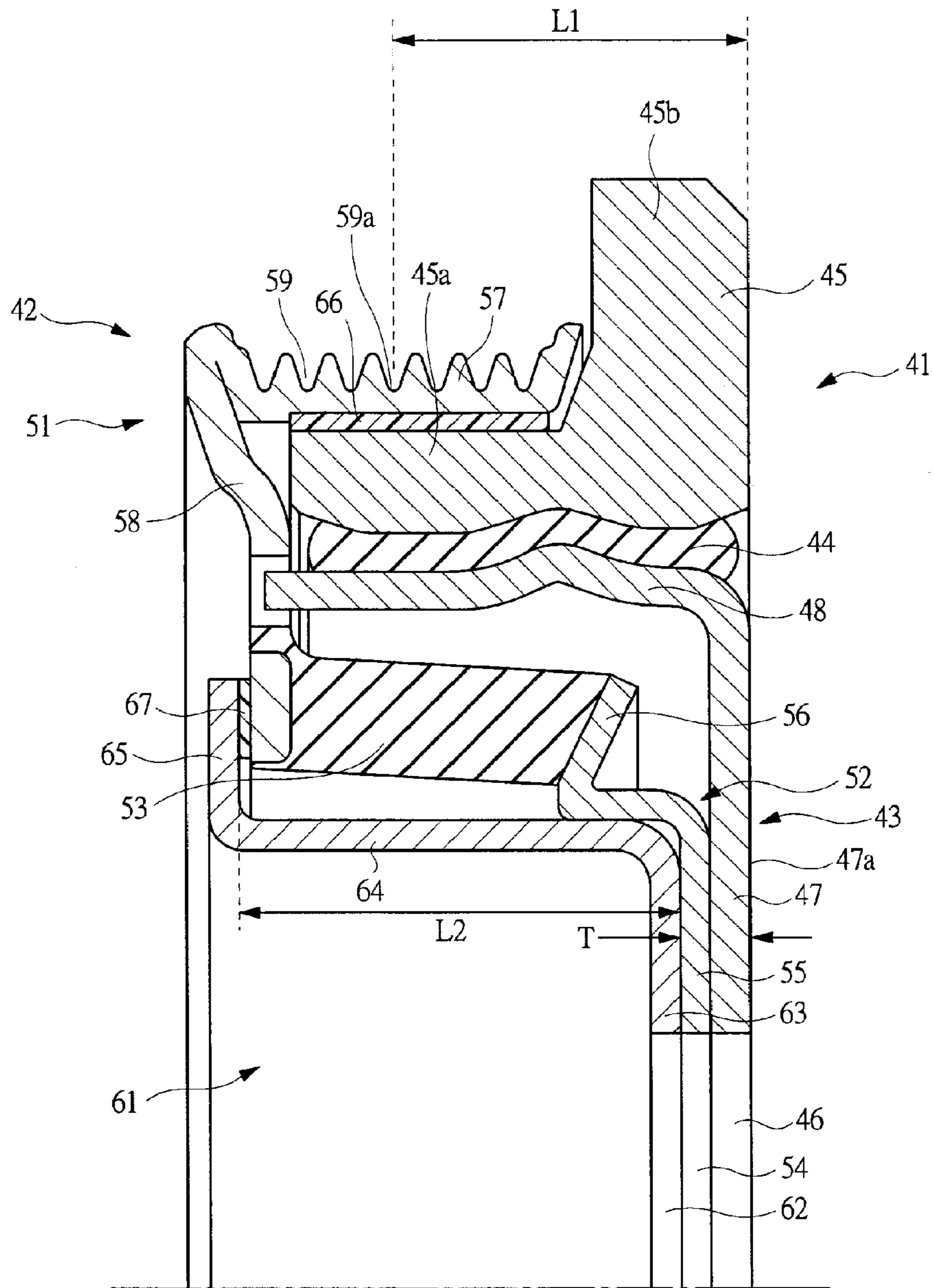
FIG. 5 Prior Art
