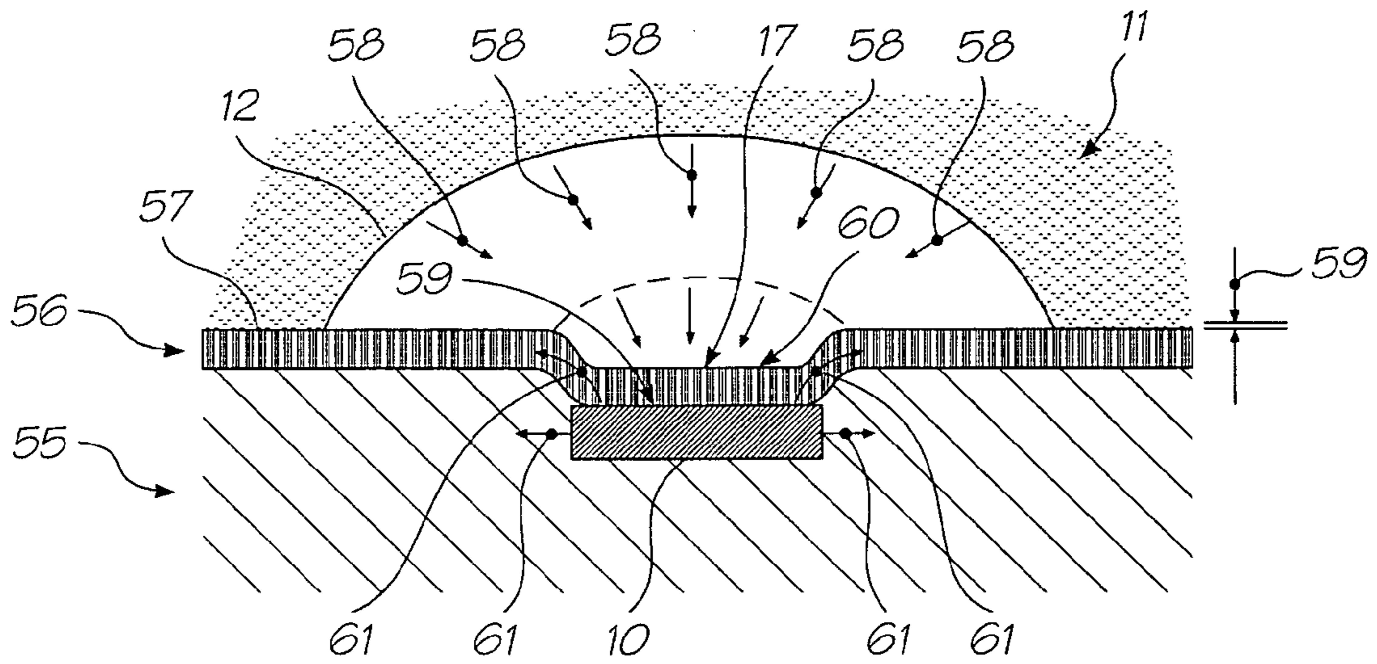
FIG. 47 (PRIOR ART)
