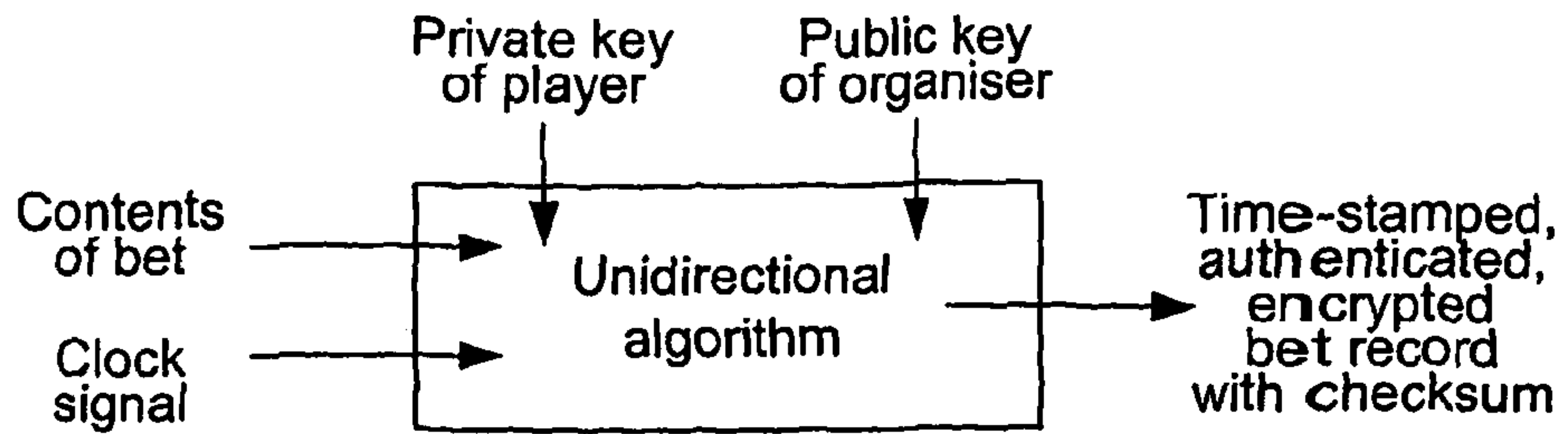
FIG. 1 PRIOR ART
