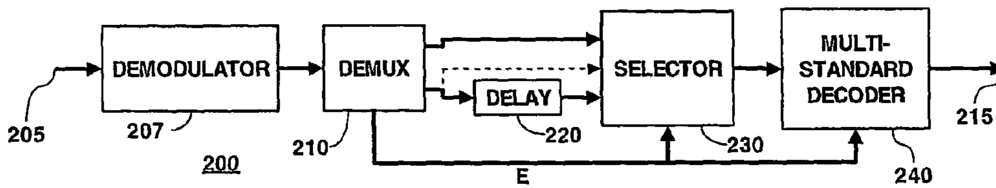
Fig. 2 Receiver
