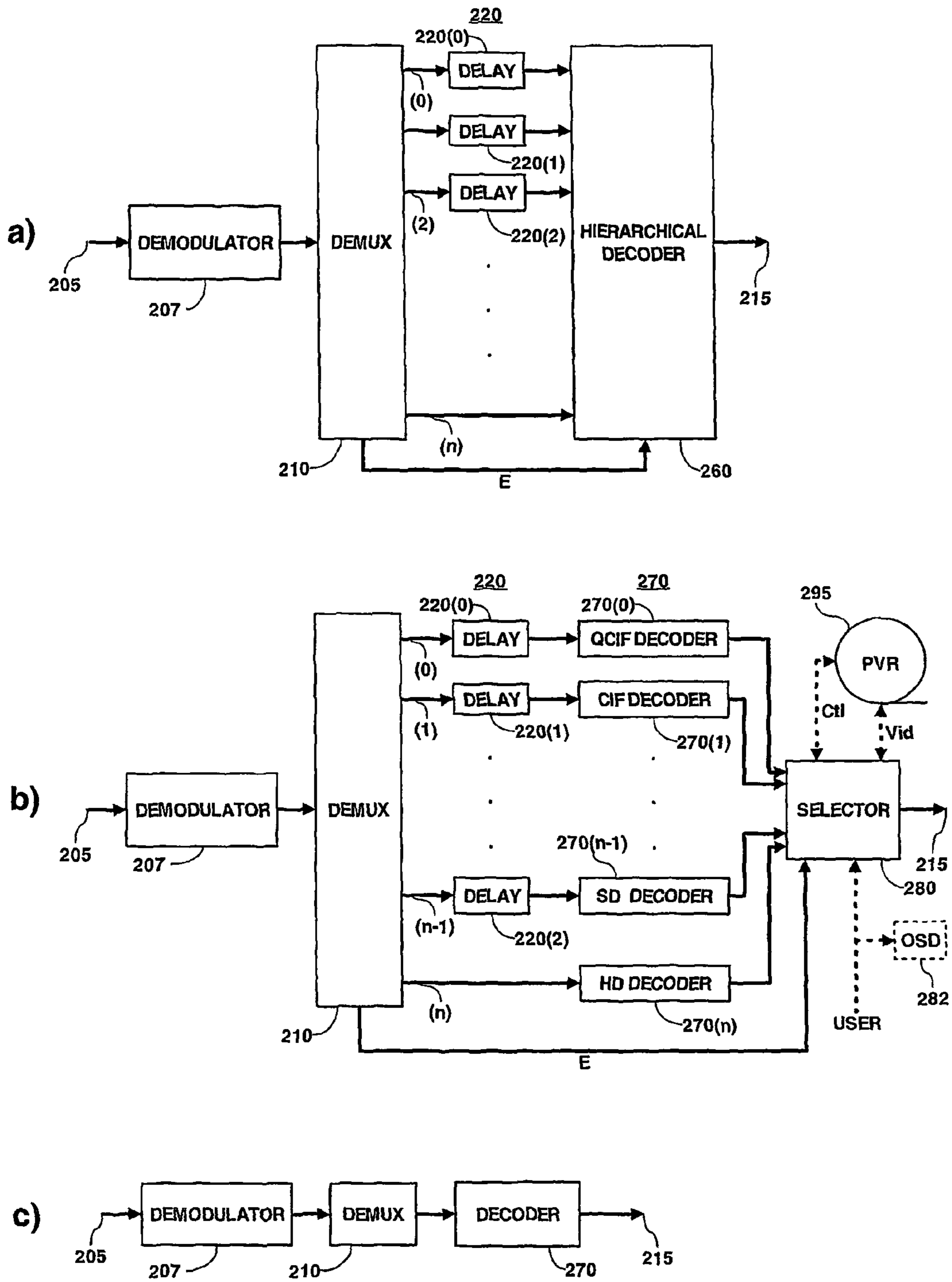
Fig. 10 Multiresolution receiver
