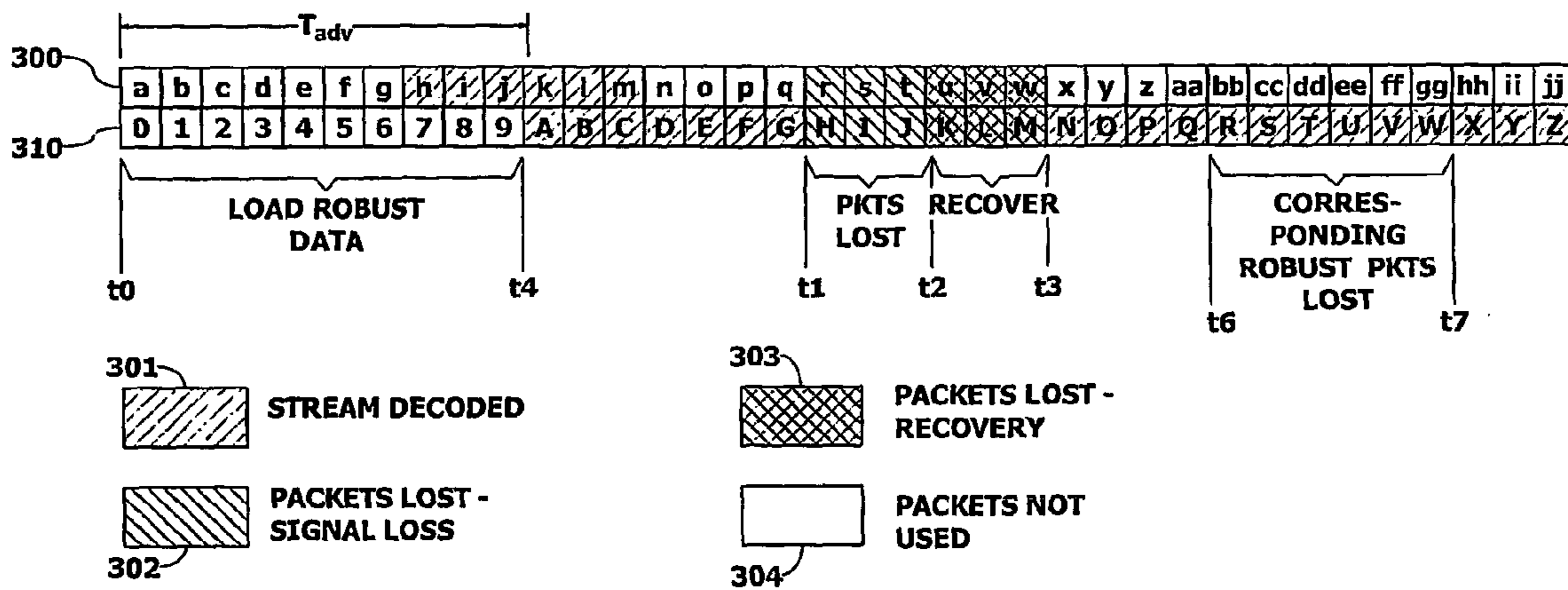
Fig. 3 Packet Streams
