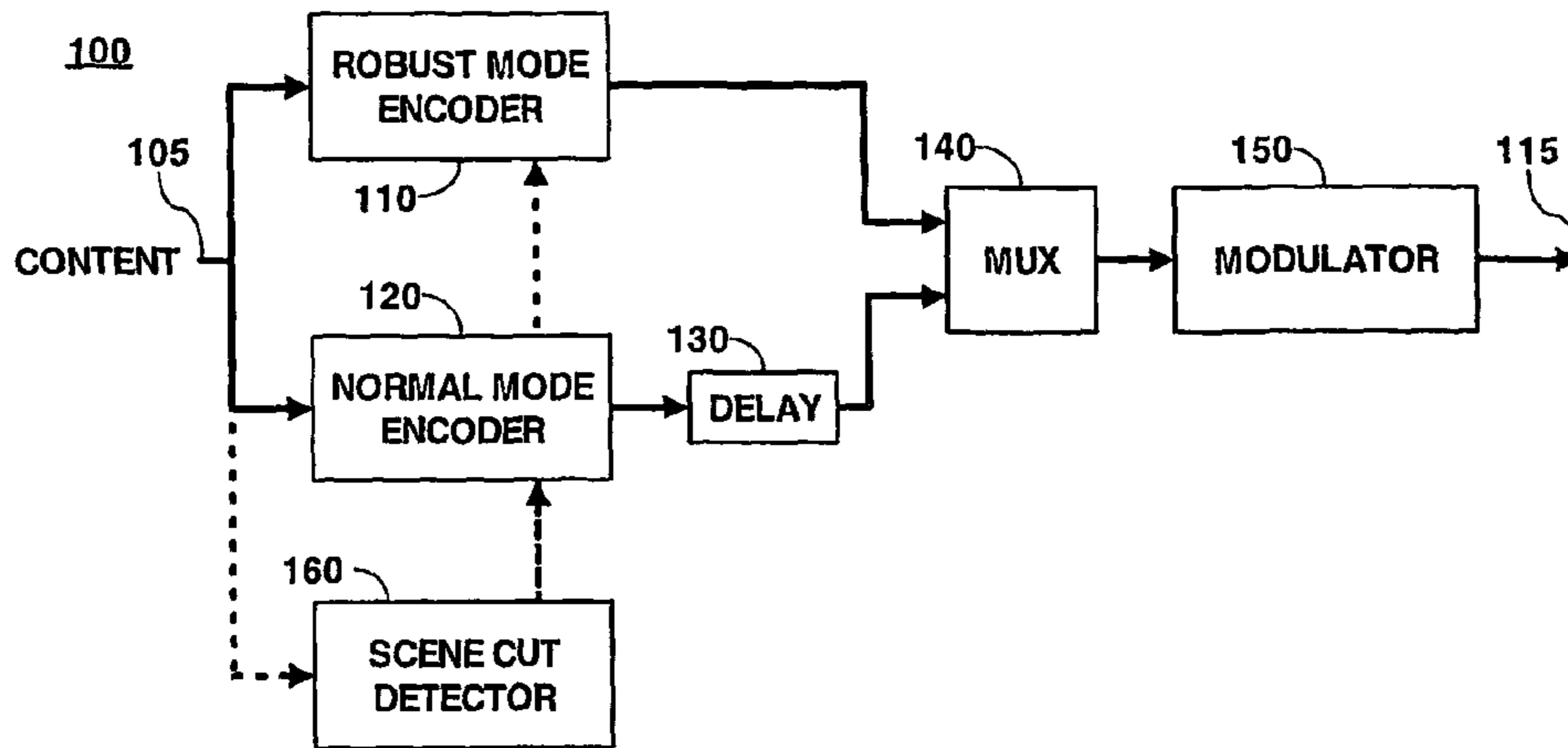
Fig. 1 Transmitter
