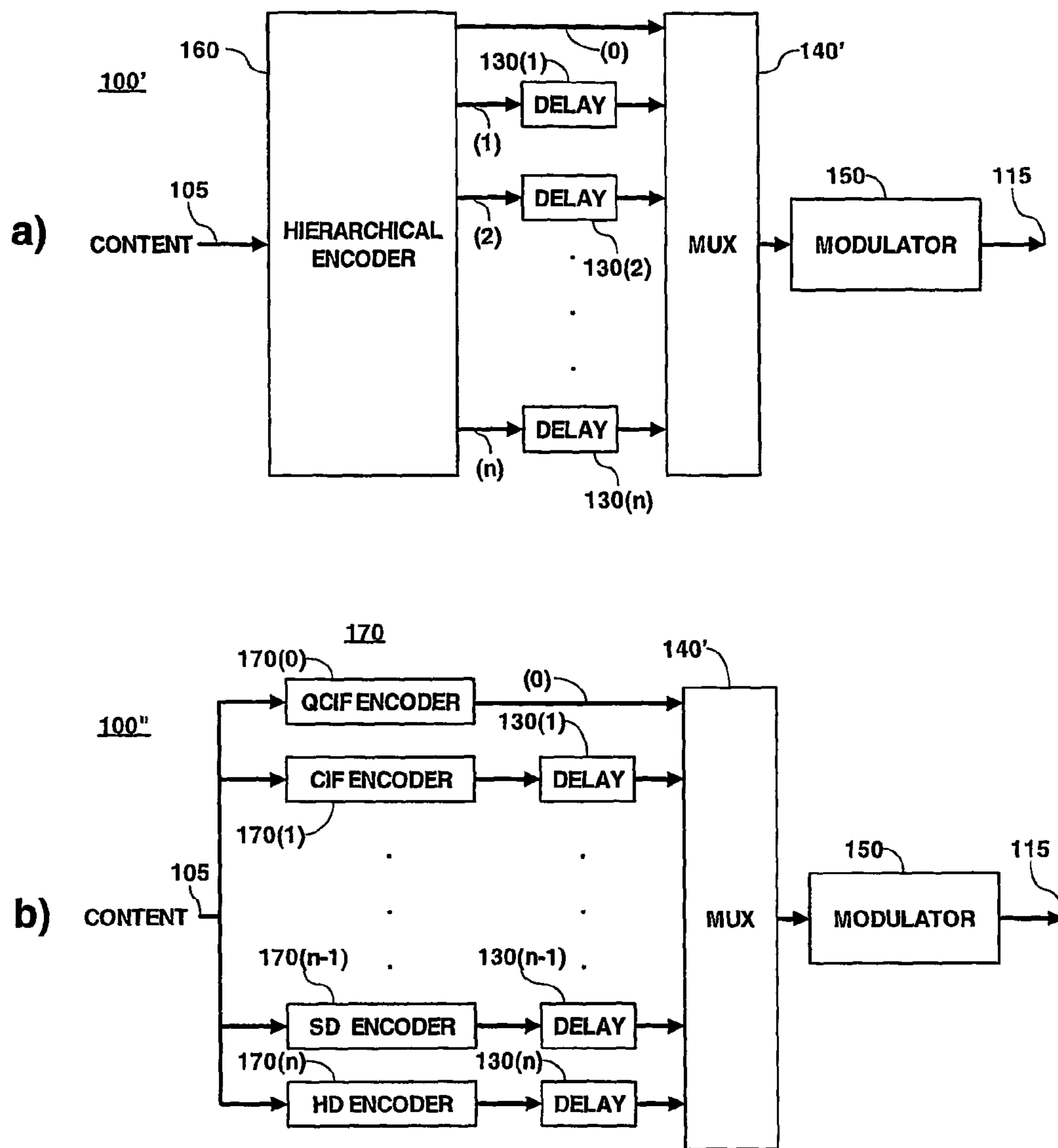
Fig. 9 Multiresolution transmitter
