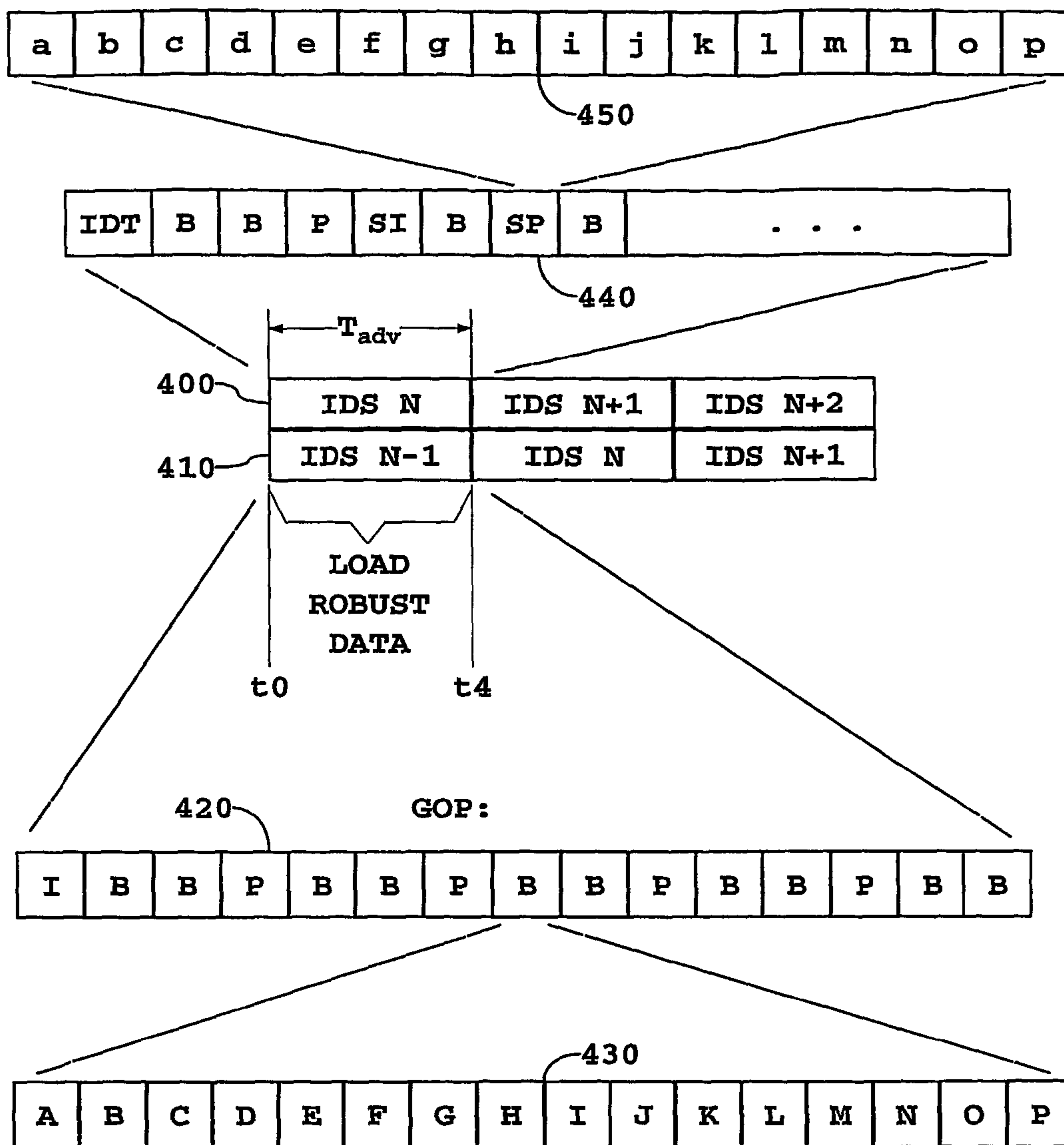
Fig. 4 GOP Streams
