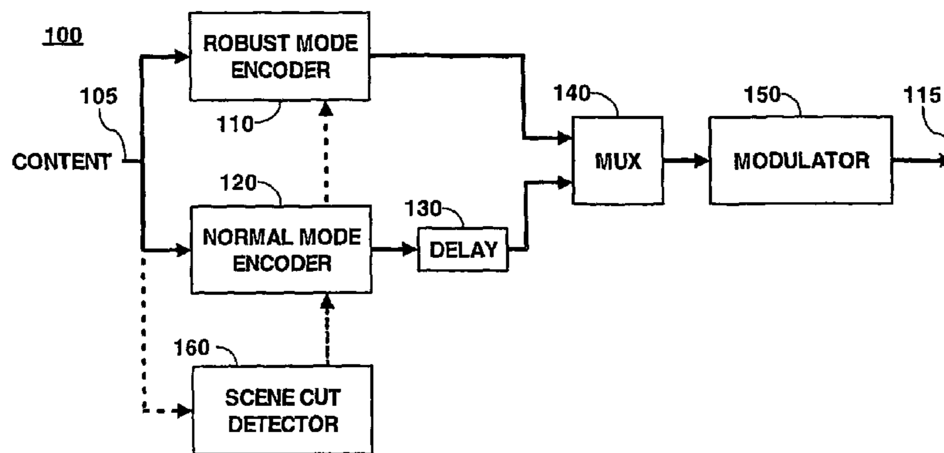
Transmitter
