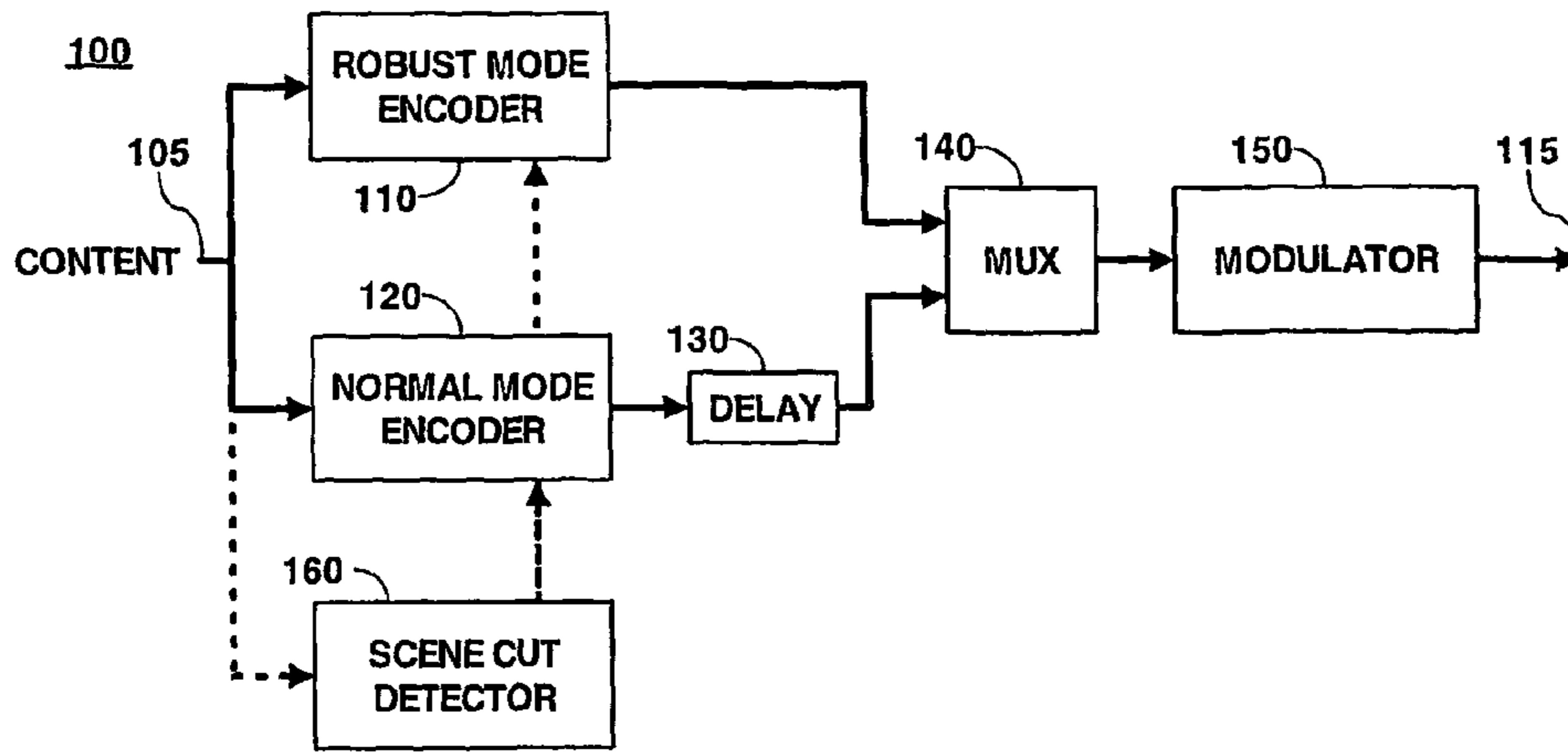
Fig. 1 Transmitter
