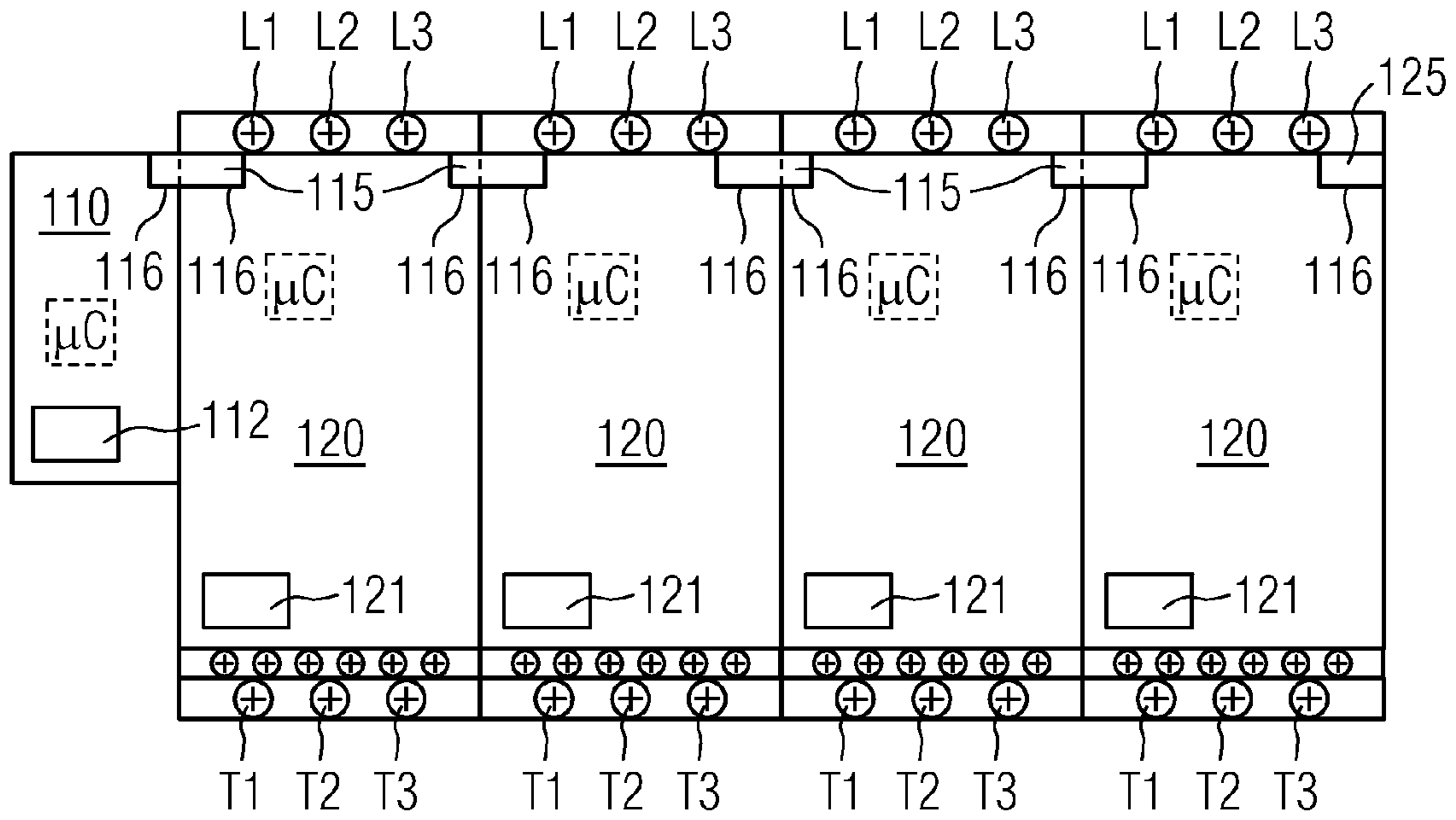
FIG 1 (PRIOR ART)
