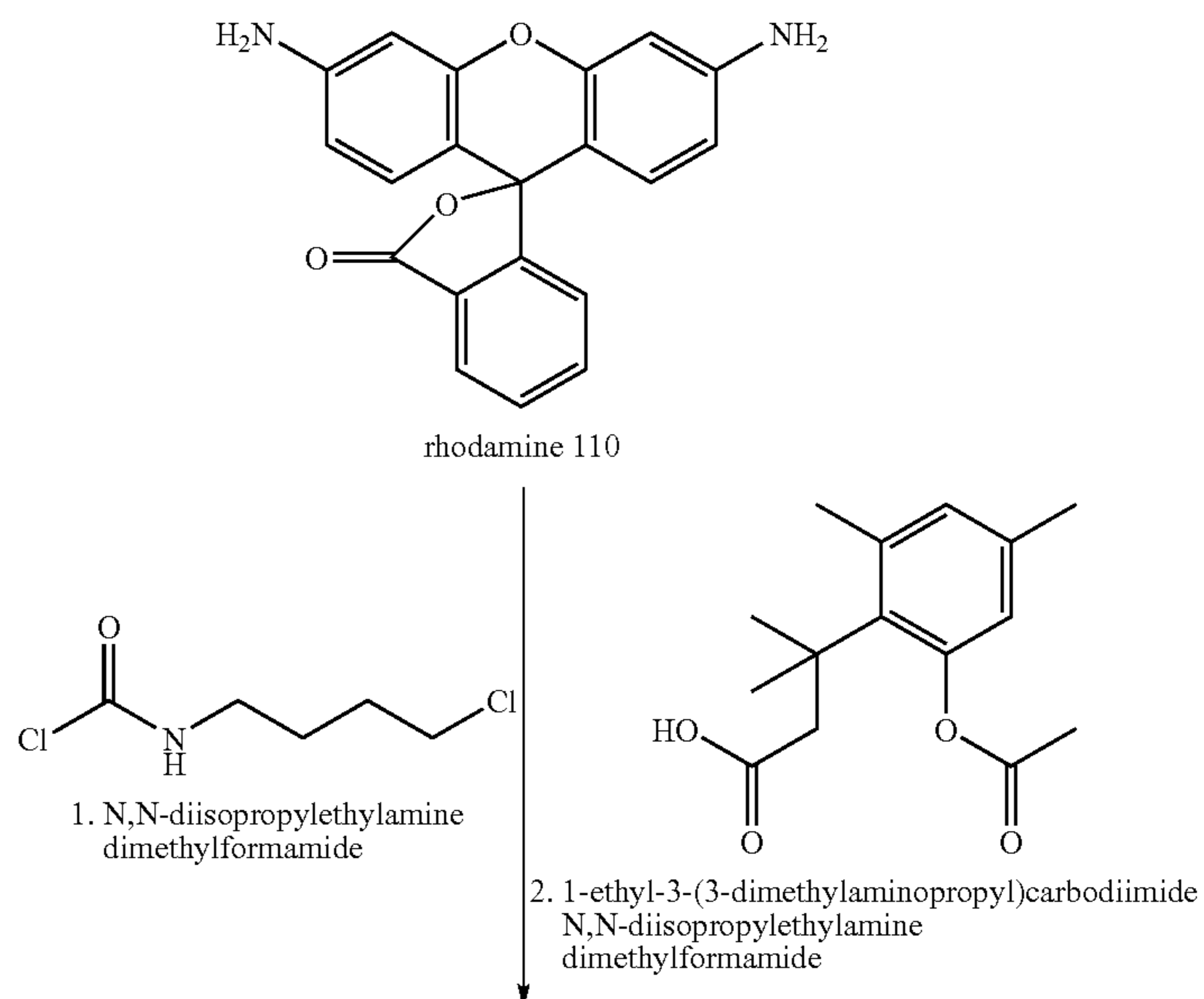
Scheme XVII
