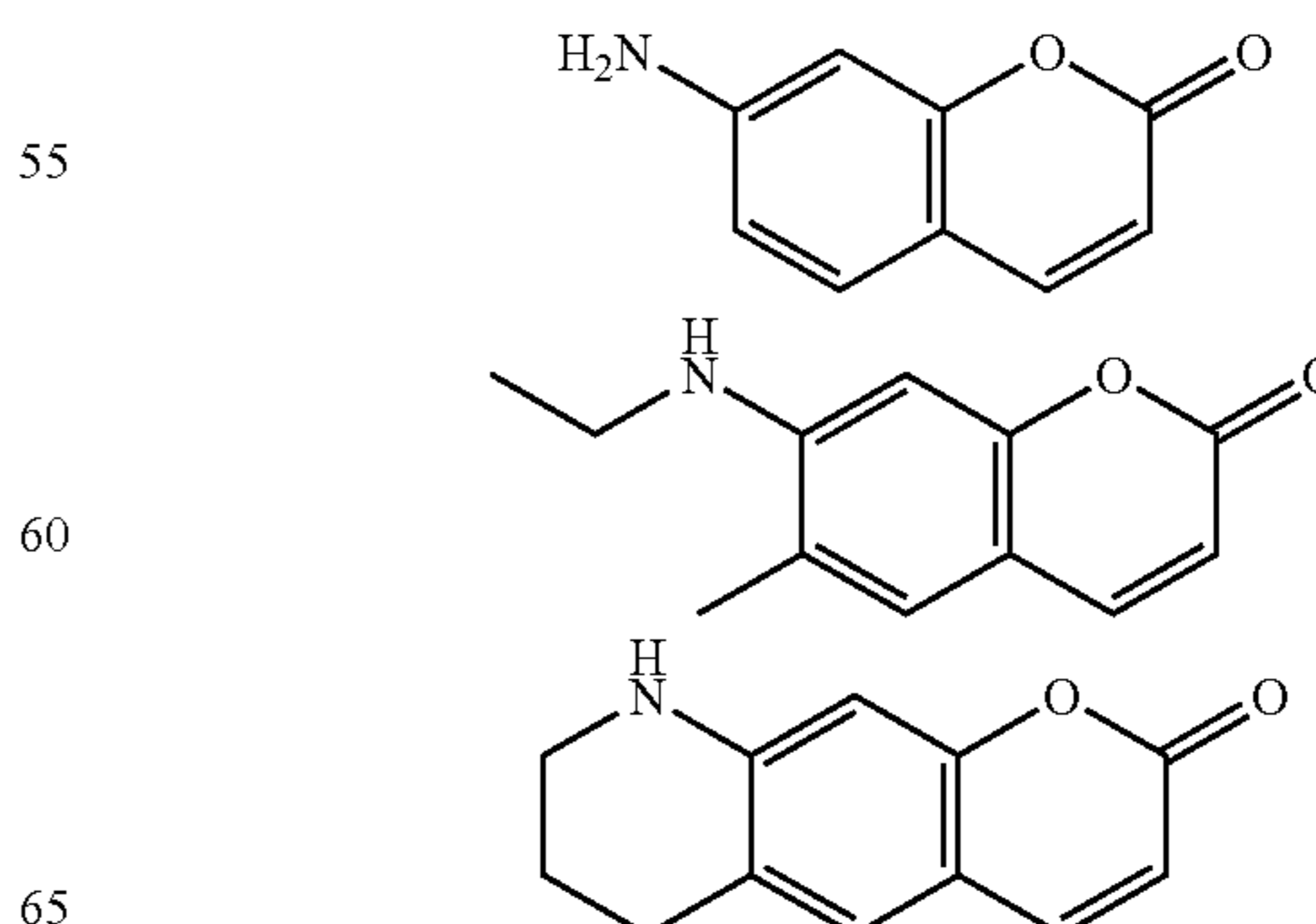
Scheme VII
