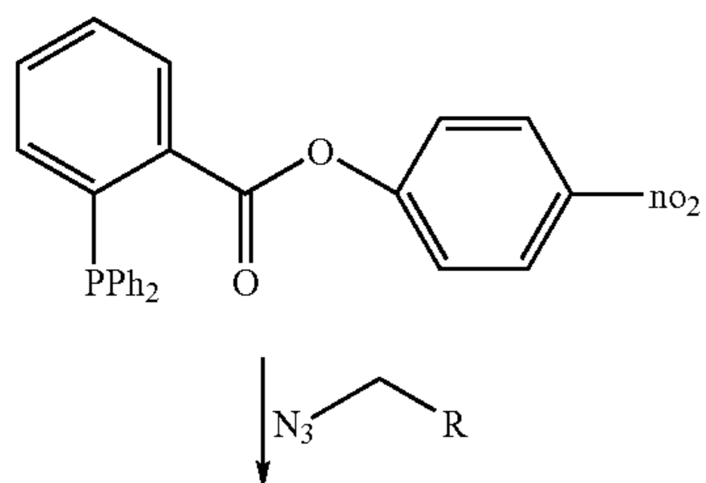
Scheme XVI
