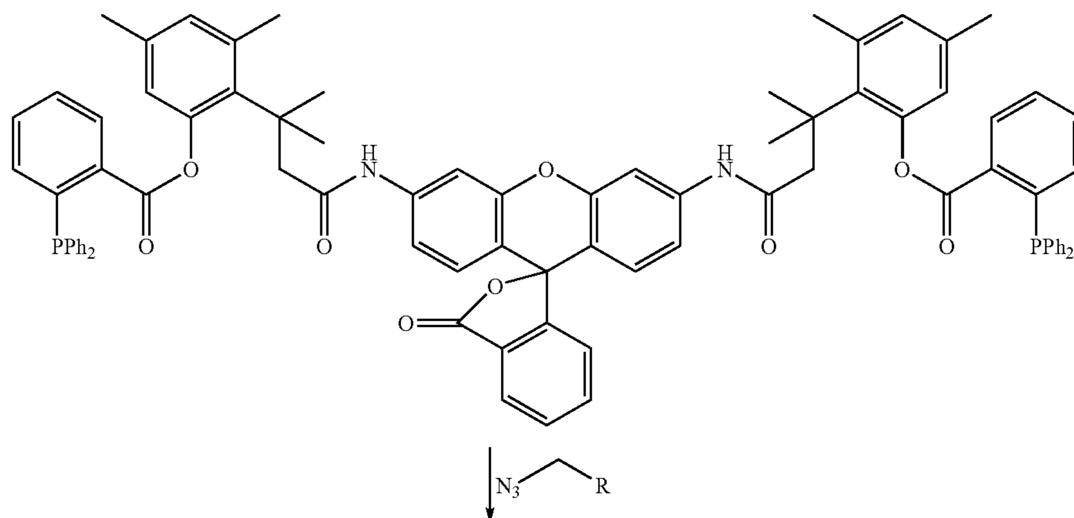
Scheme XIV
