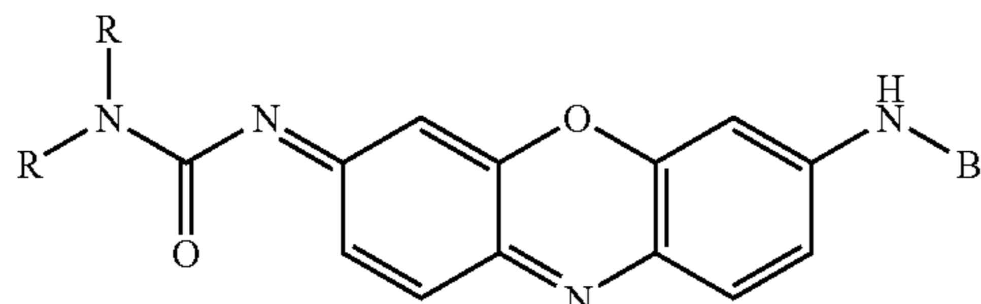
Scheme VIII
