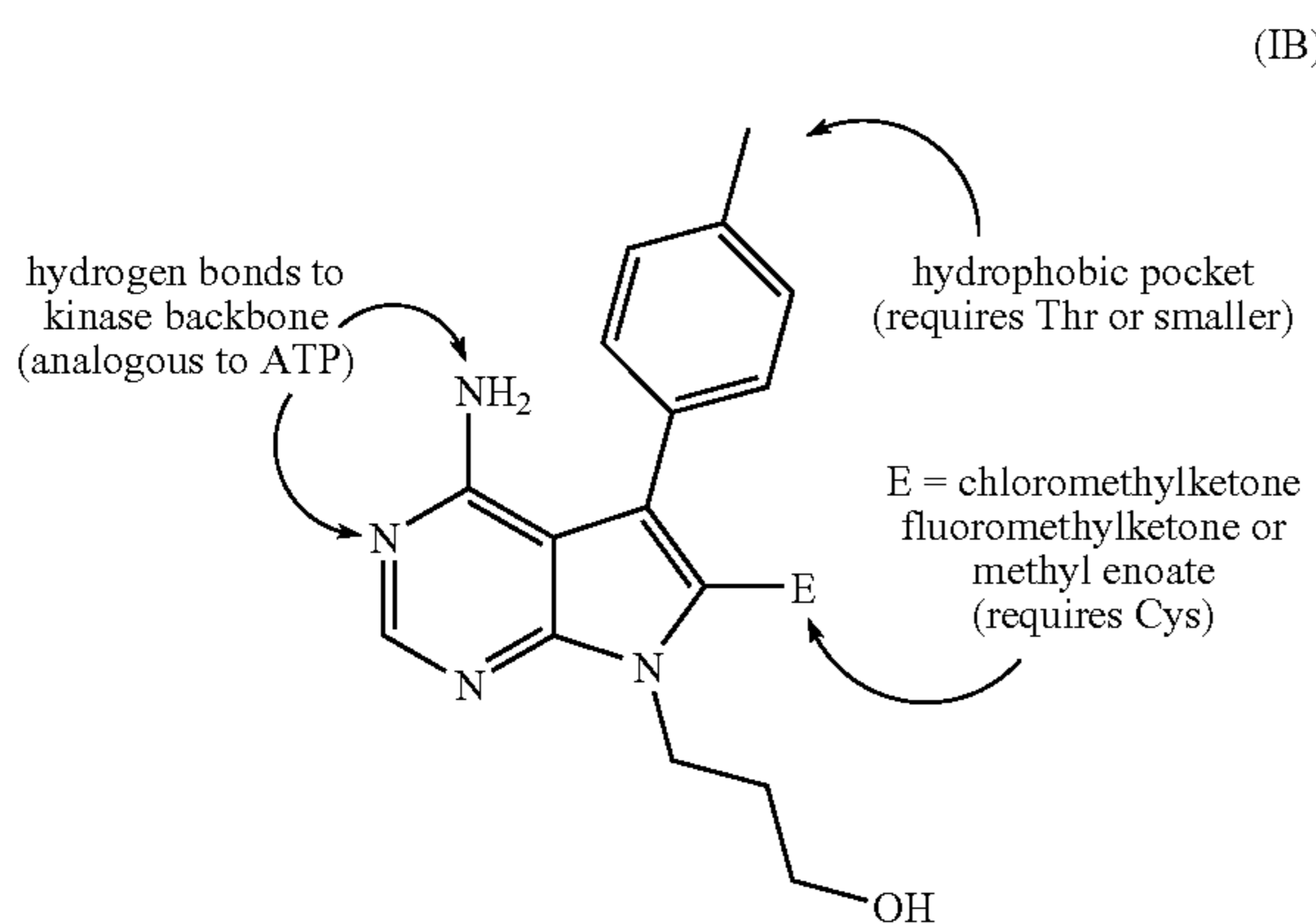
Rsk inhibitors based on a pyrrolopyrimidine scaffold.
