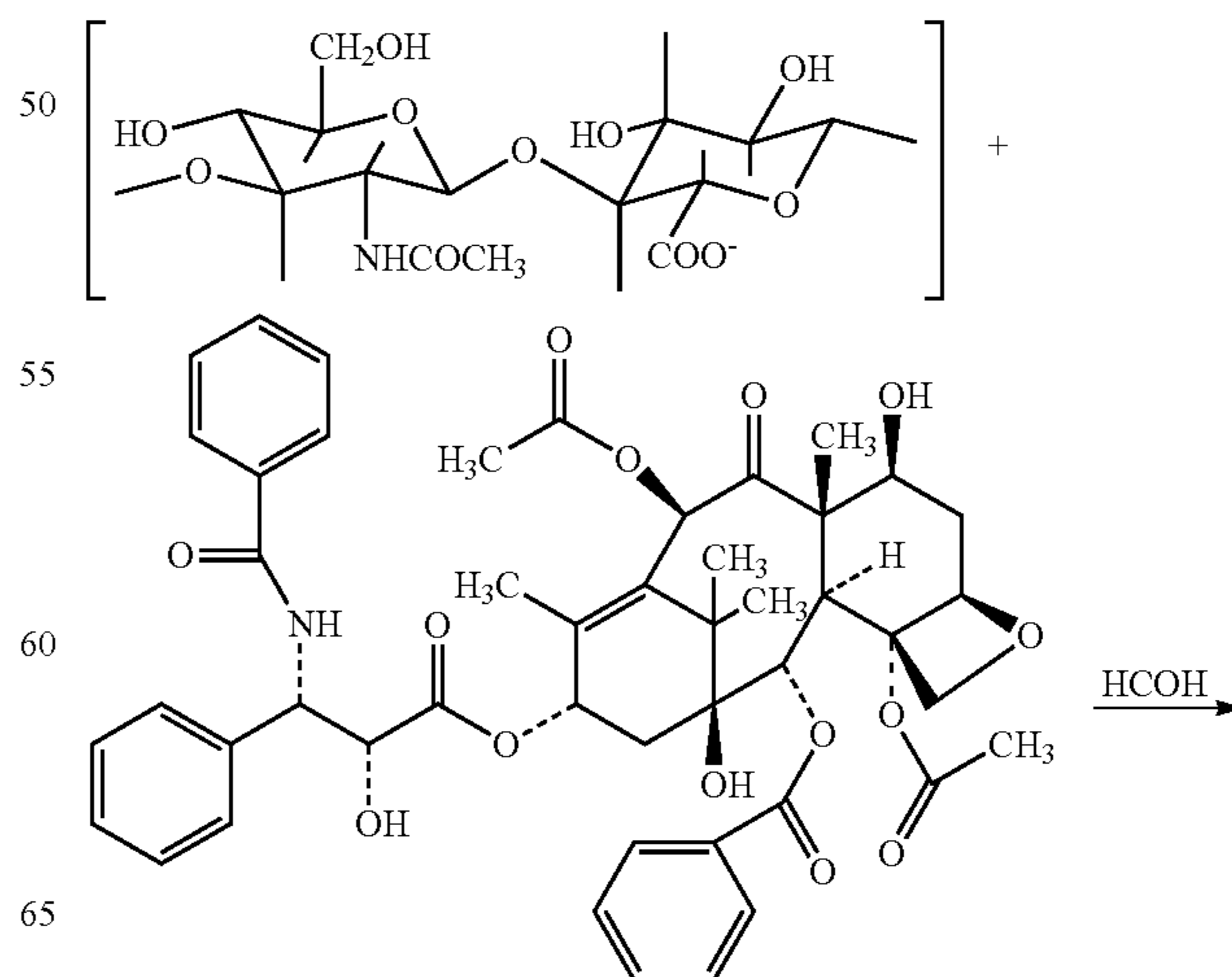
Scheme 10
