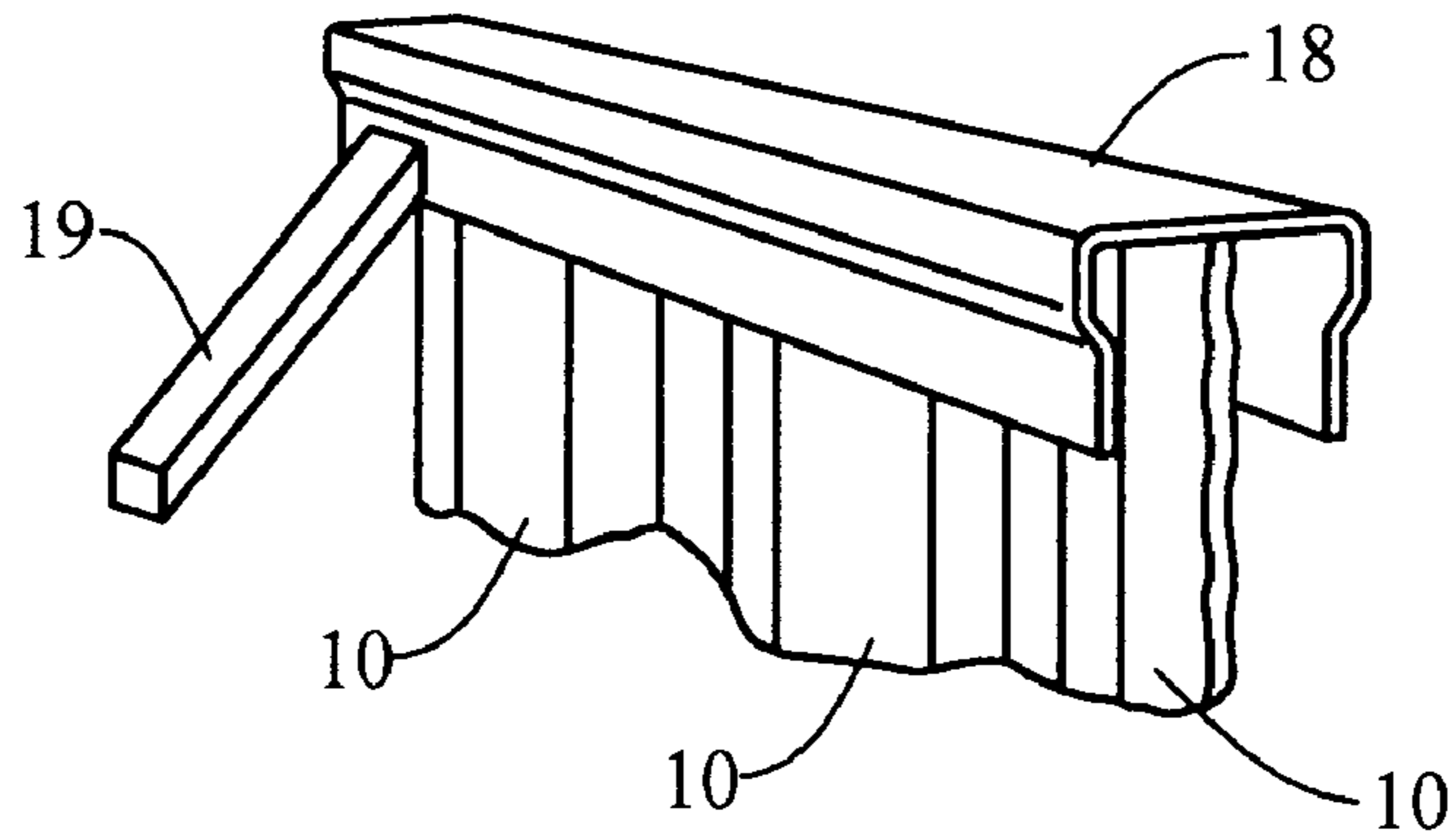
FIG. 9 PRIOR ART
