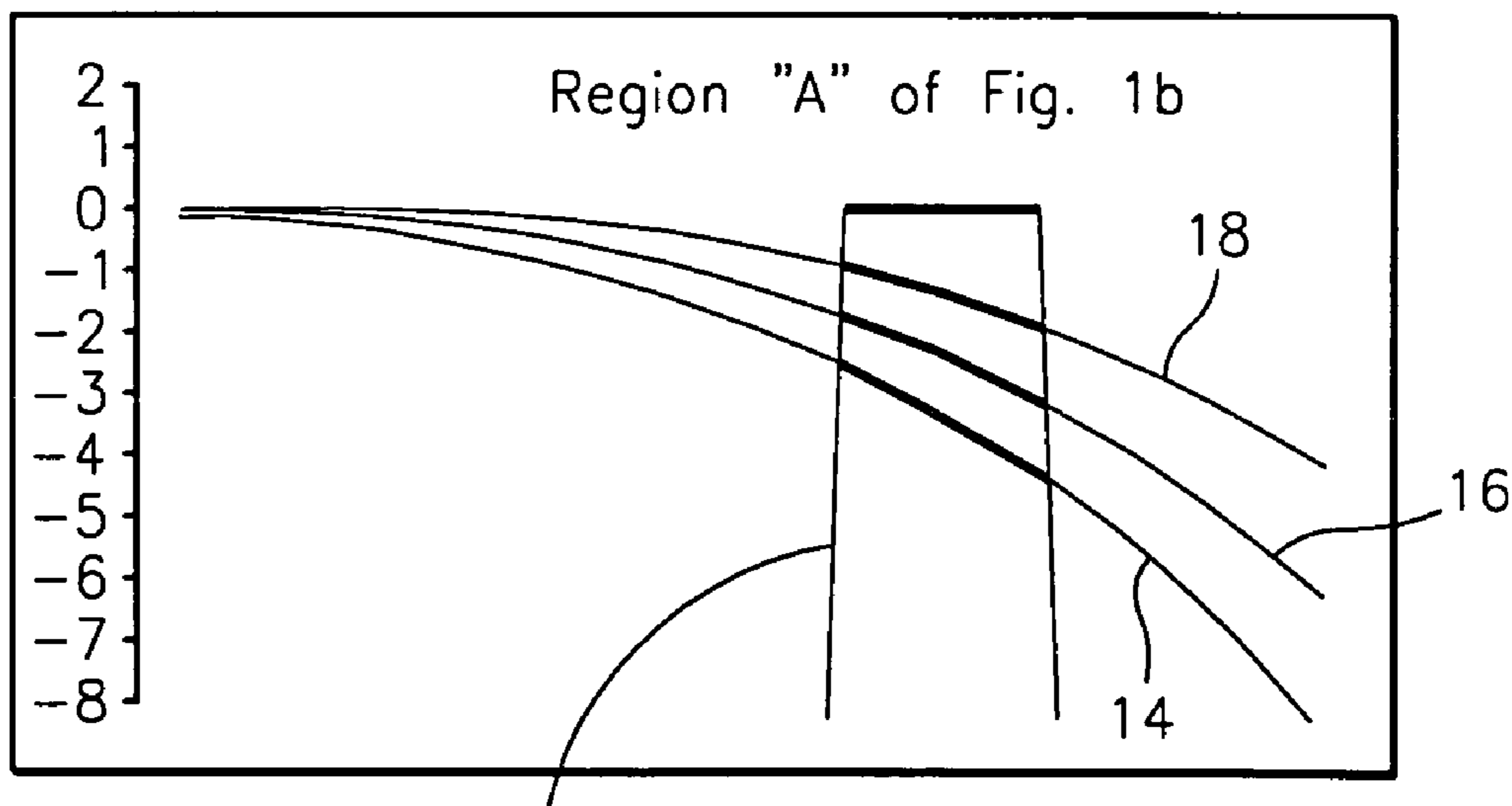
Interfering antenna signal, 30
