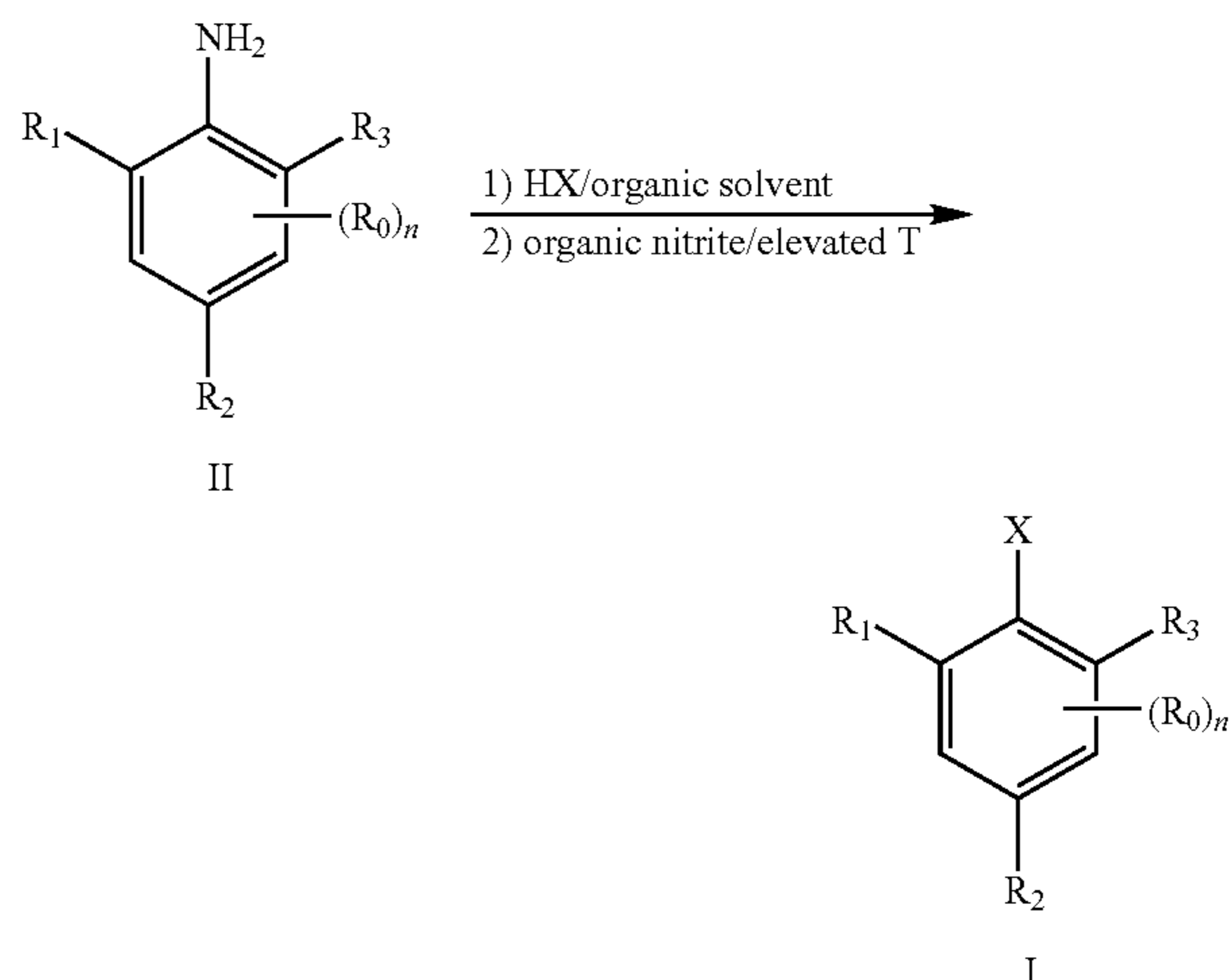
Reaction Scheme 1
