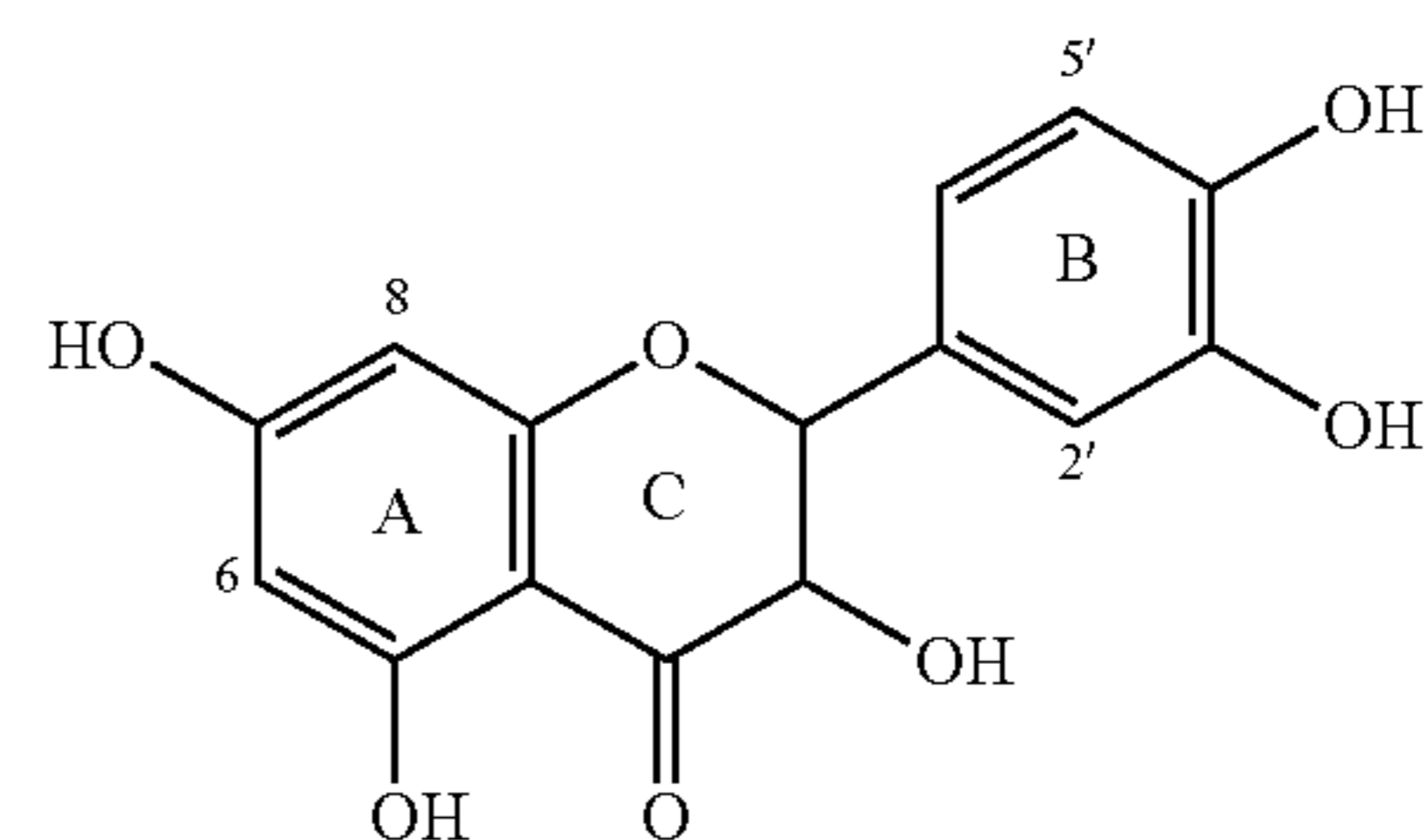
Quercetin
