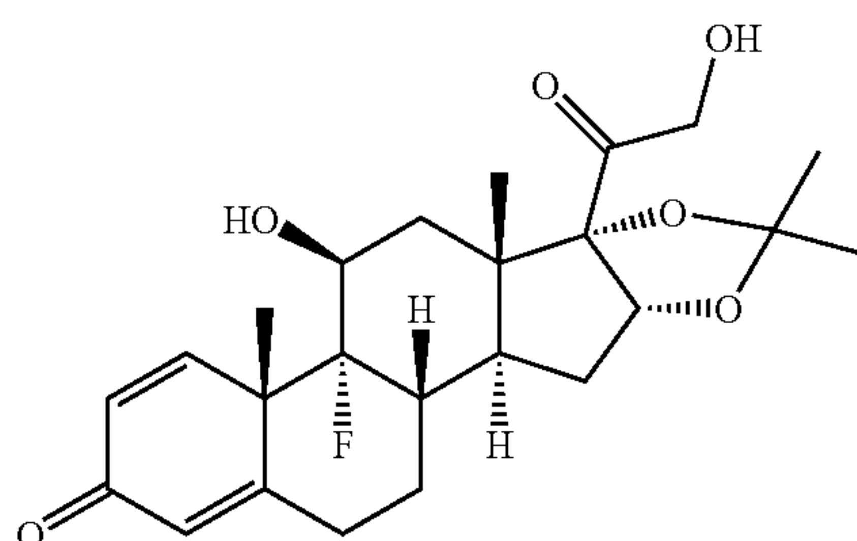
triamcinolone acetonide
