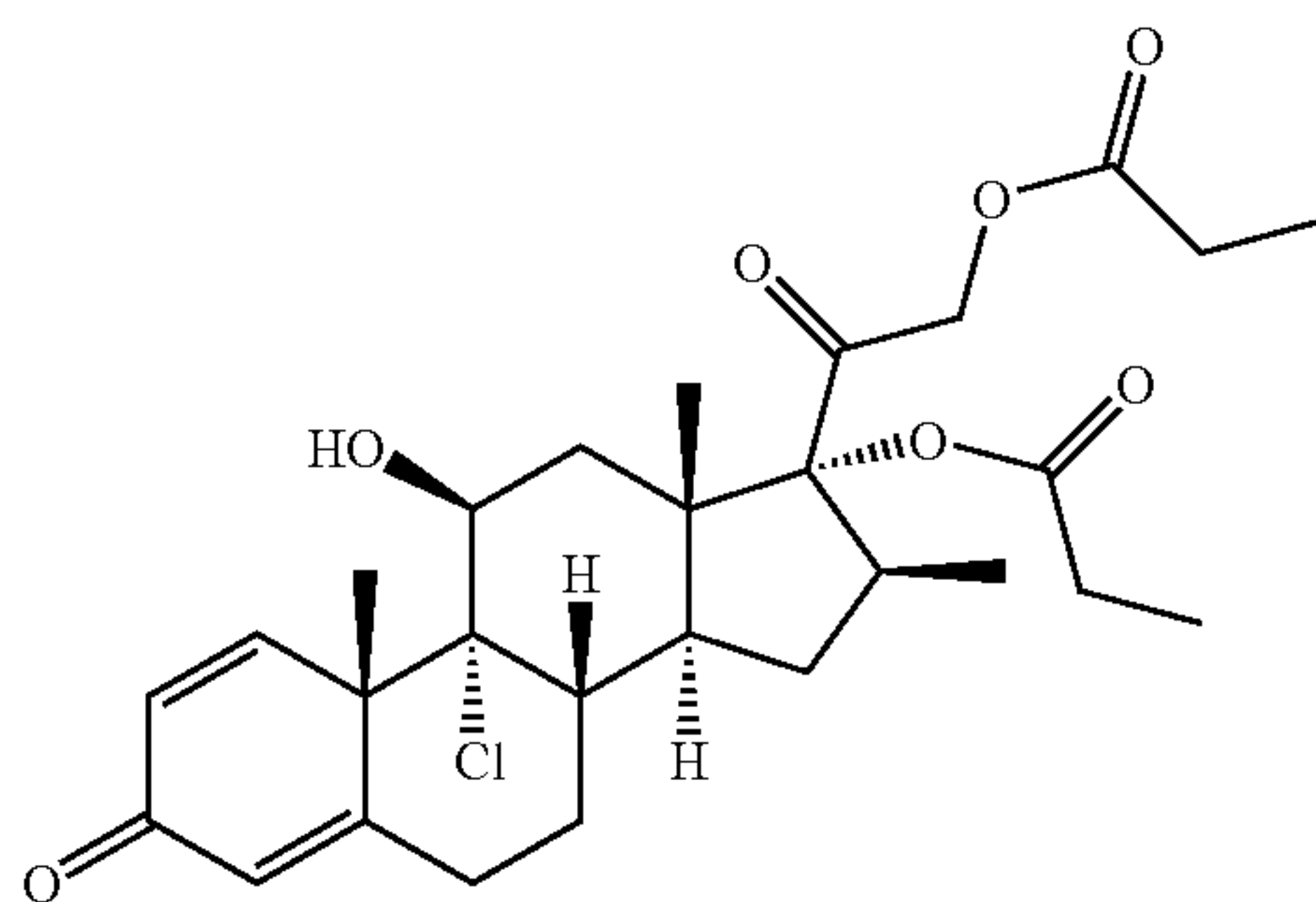
beclomethasone dipropionate
