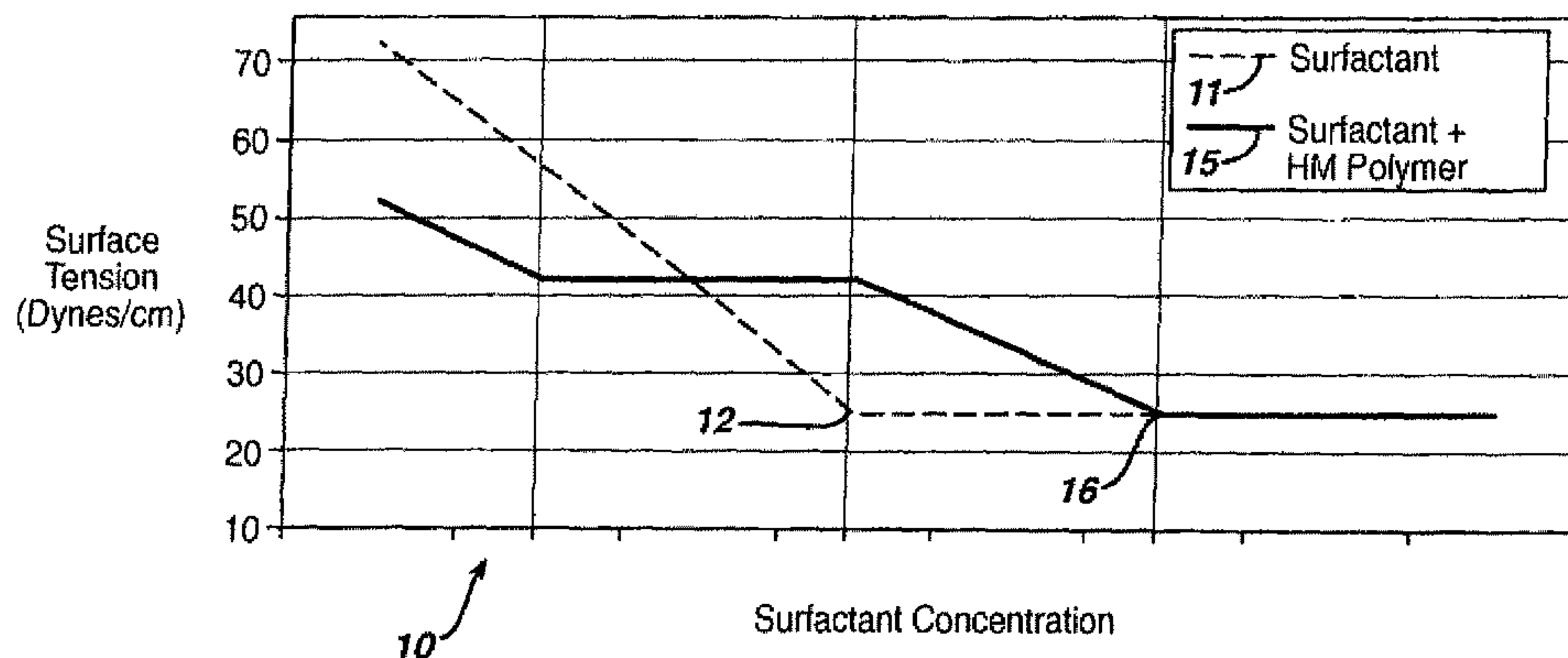
Interaction of Hydrophobically Modified Polymer and Surfactant
