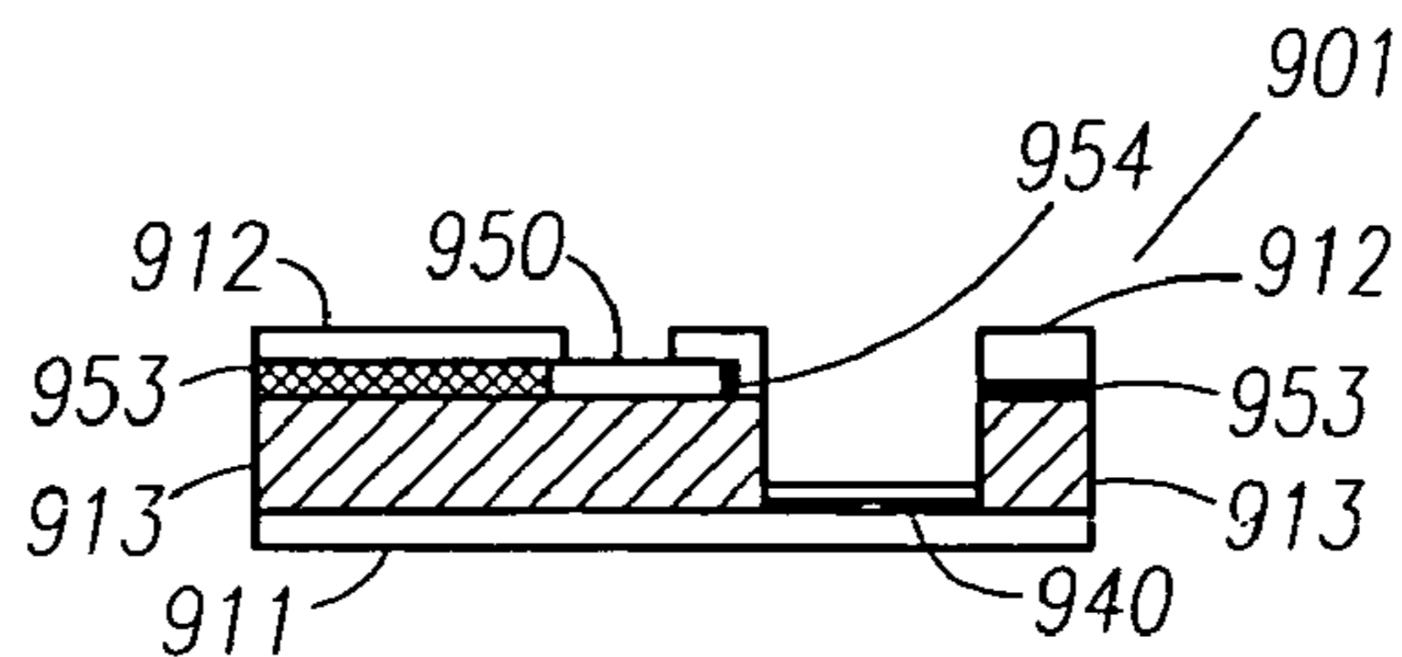
SECTION "E-E"
