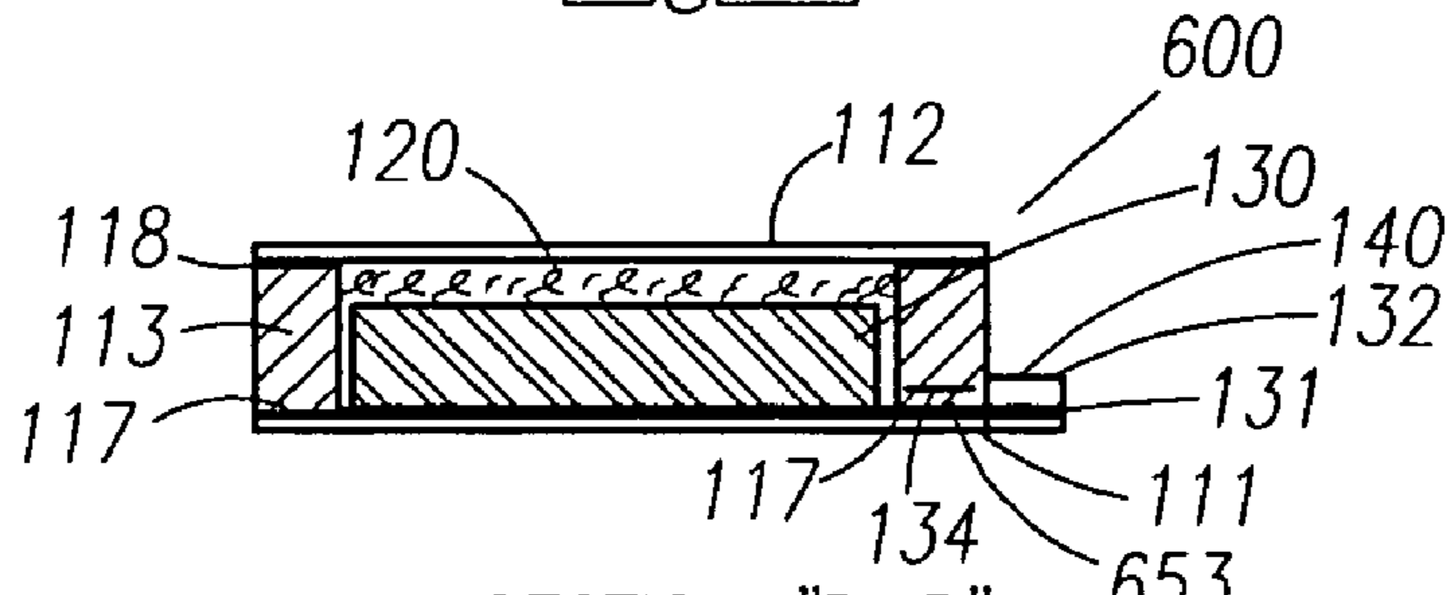
SECTION "B-B"
