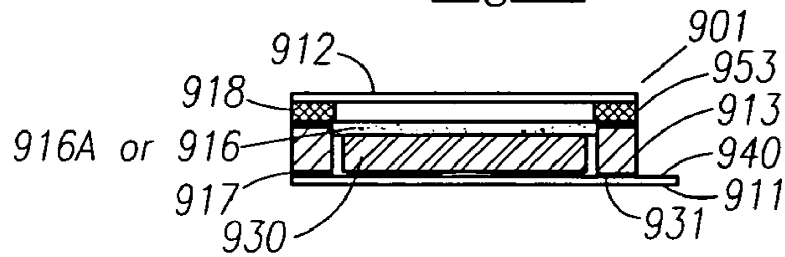
SECTION "C-C"
