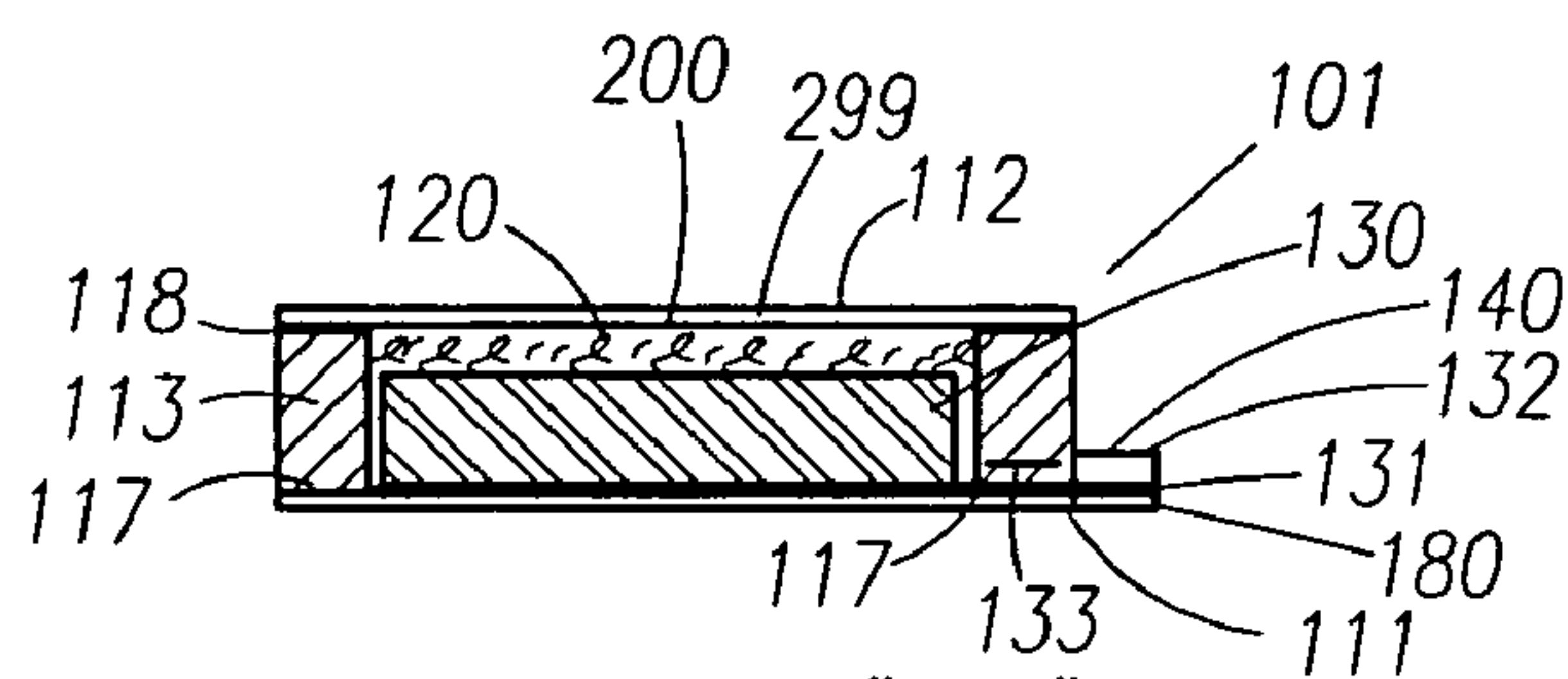
SECTION "B-B"
