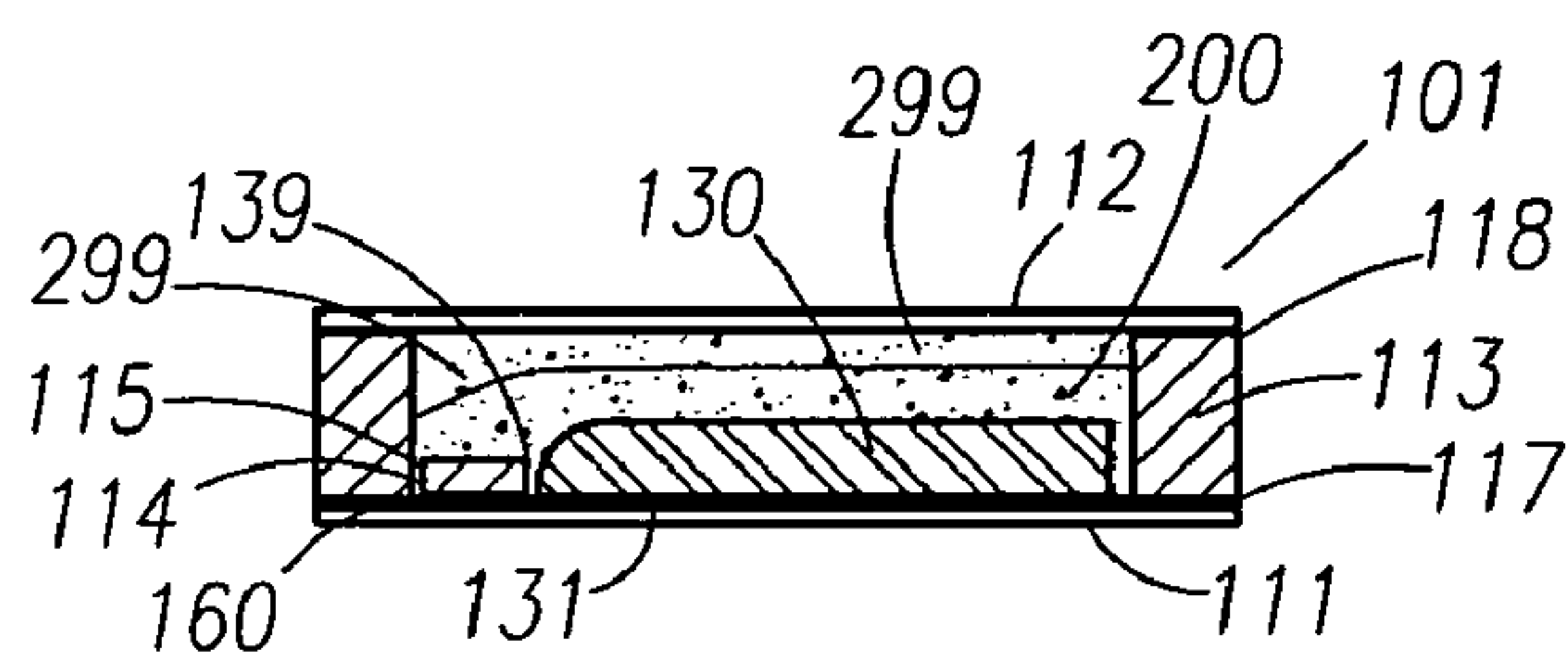
SECTION "A-A"
