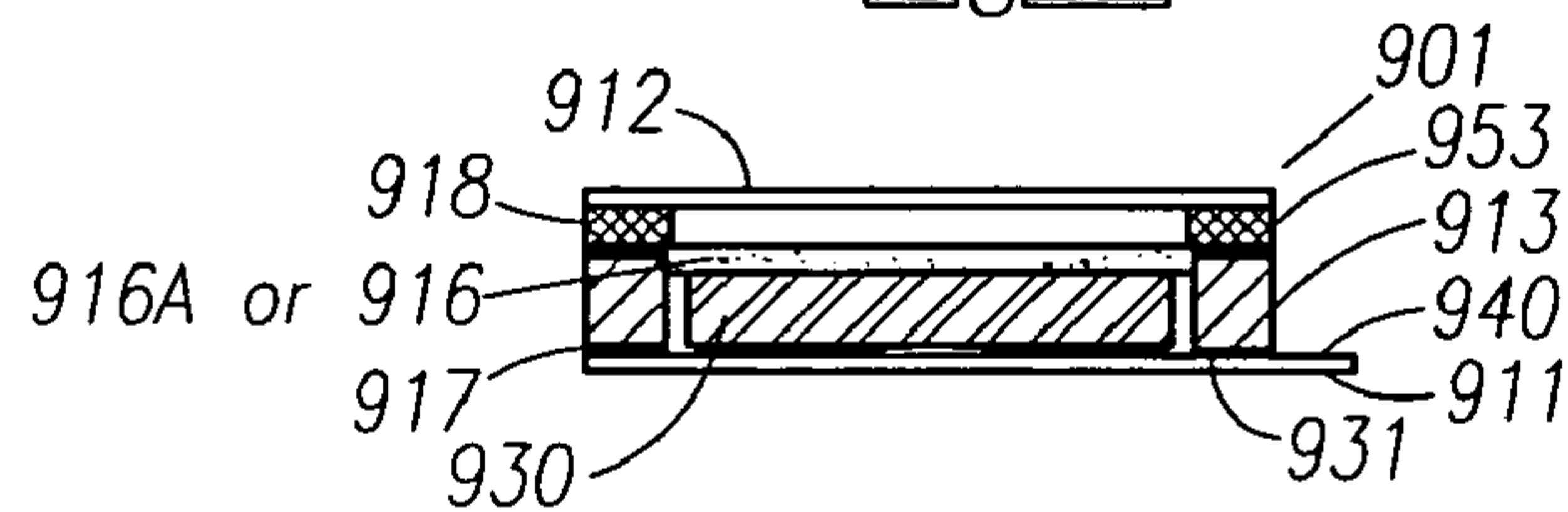
SECTION "C-C"
