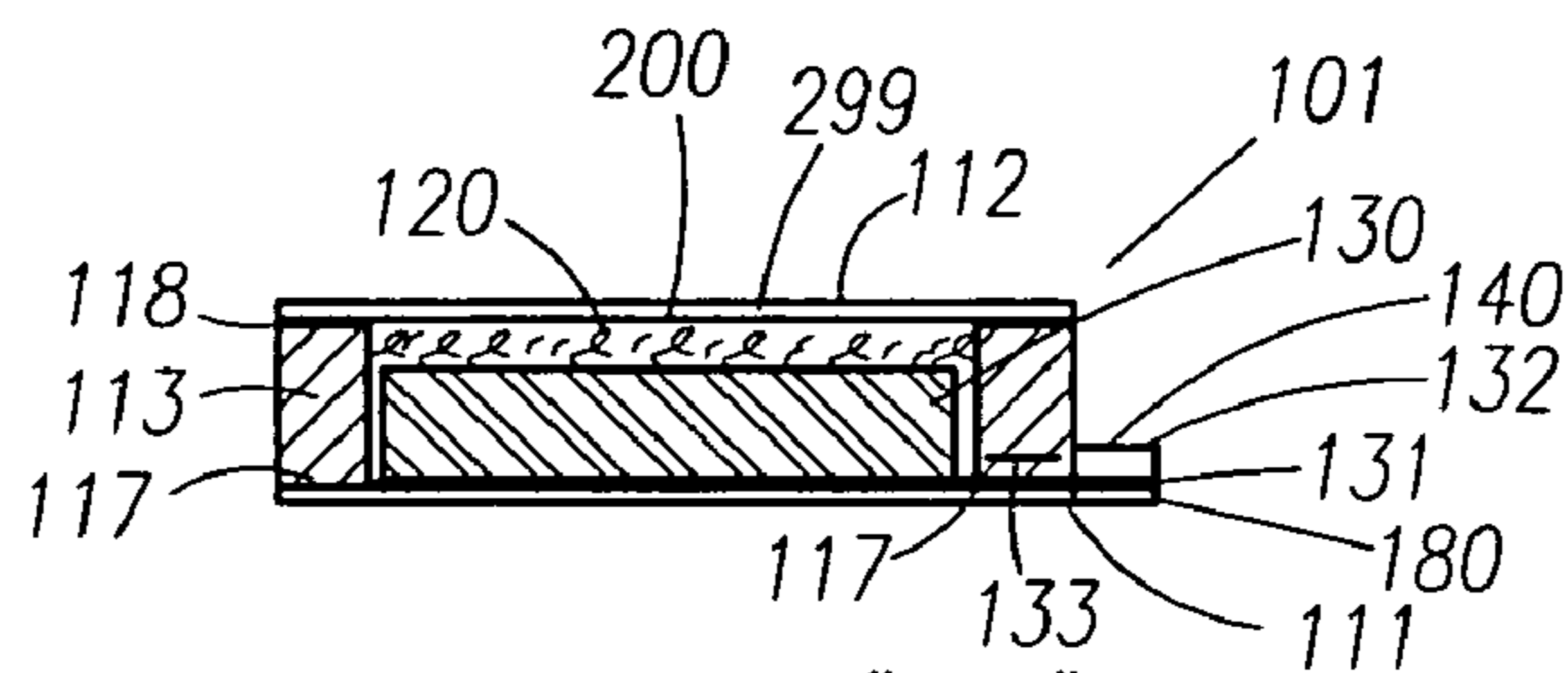
SECTION "B-B" Fig. 3
