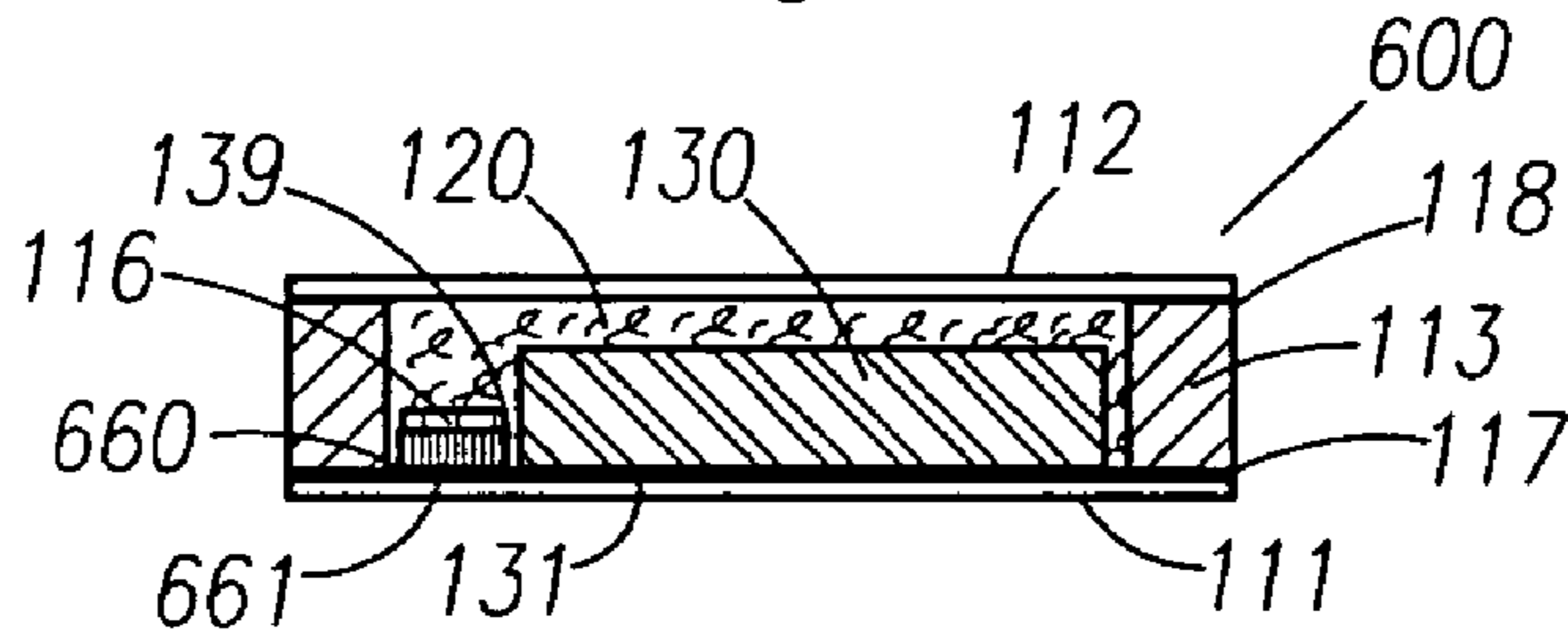
SECTION "A-A"
