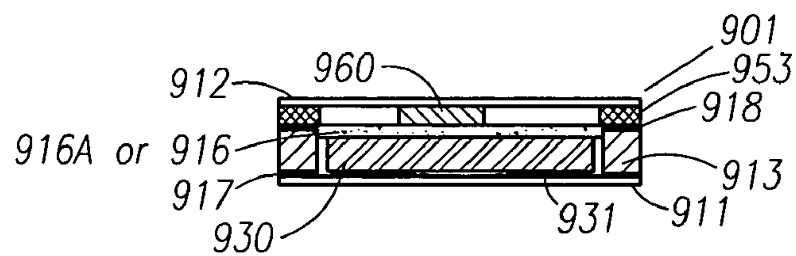
SECTION "B-B"
