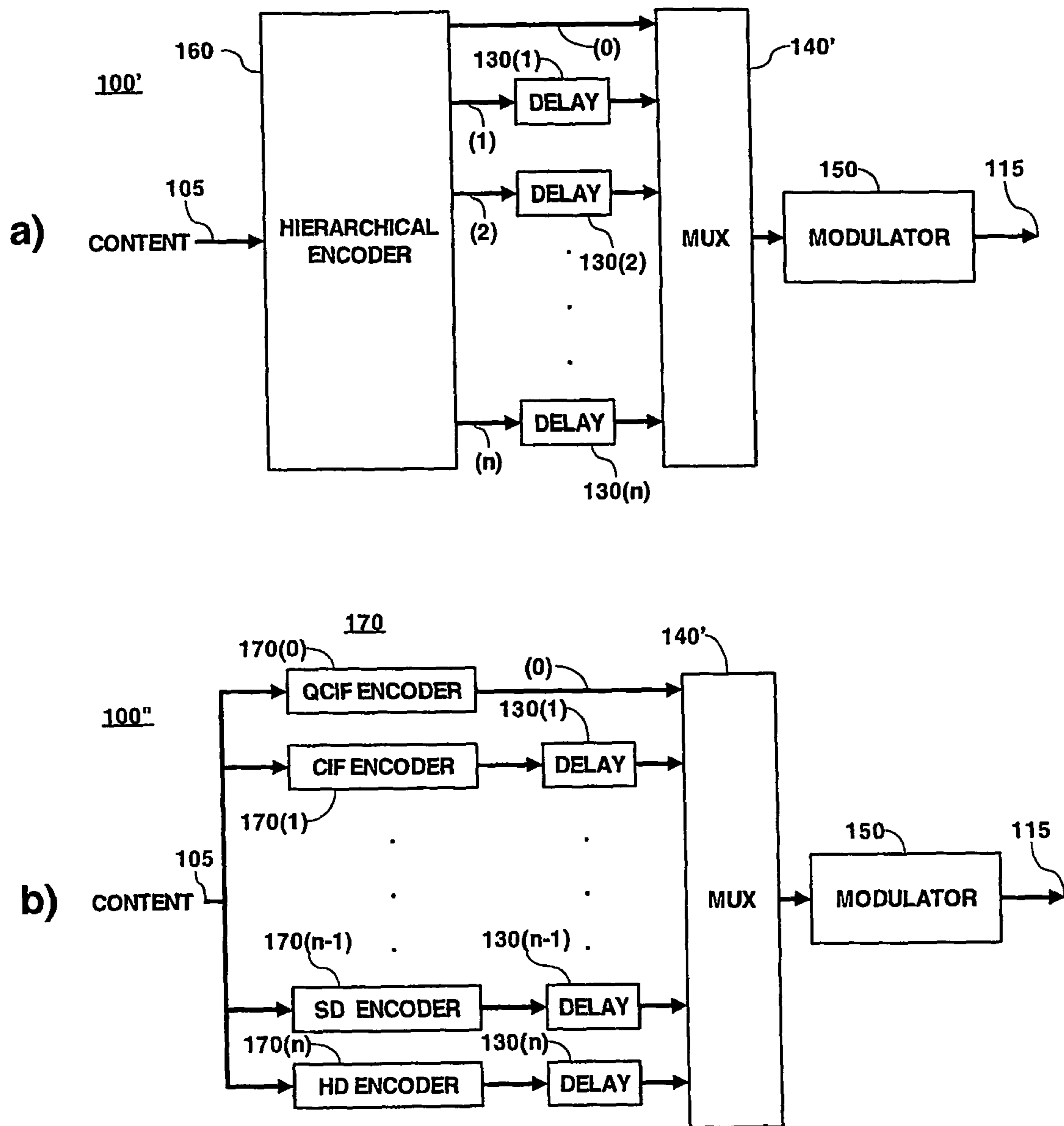
Fig. 9 Multiresolution transmitter
