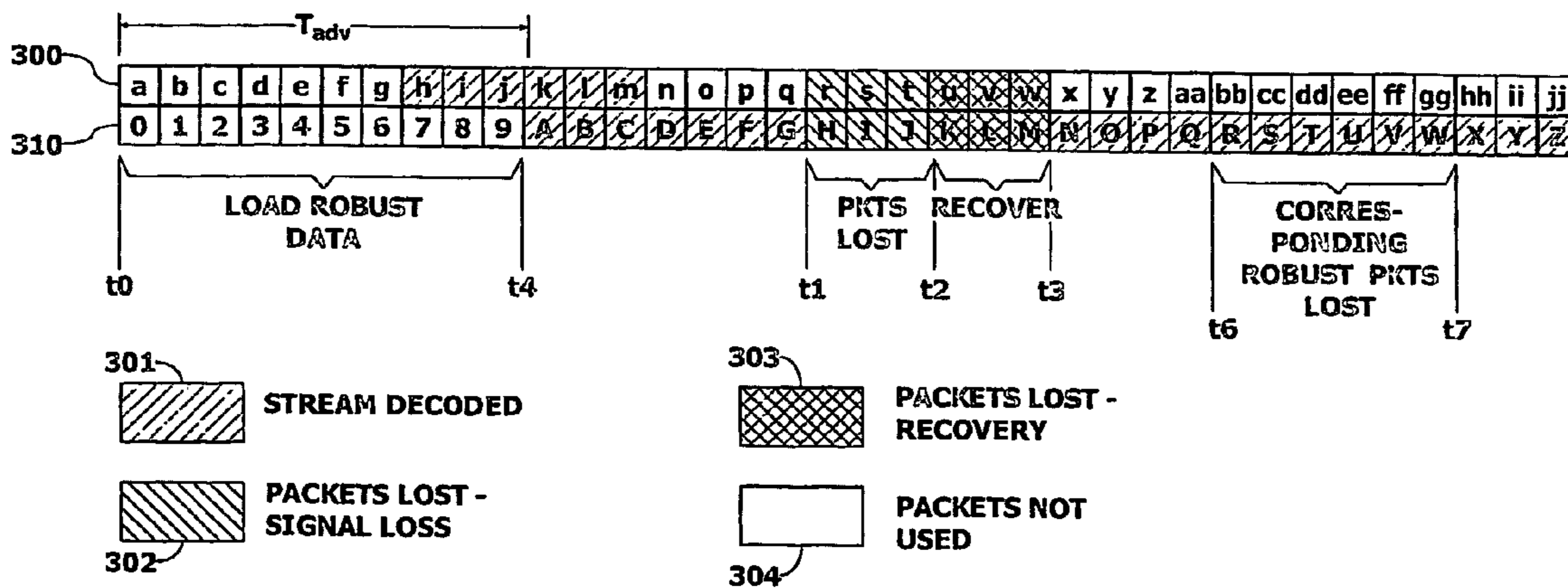
Fig. 3 Packet Streams
