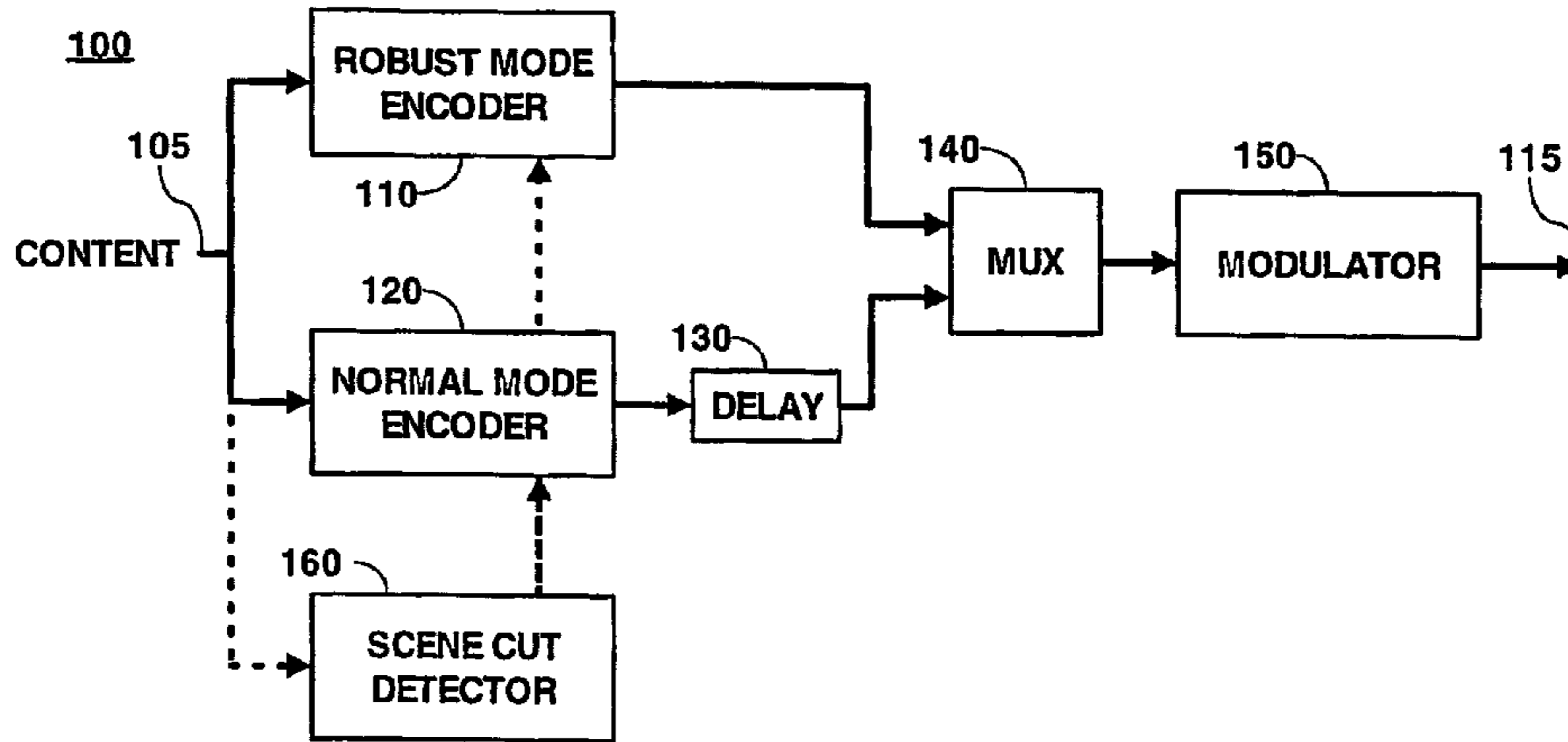
Fig. 1 Transmitter
