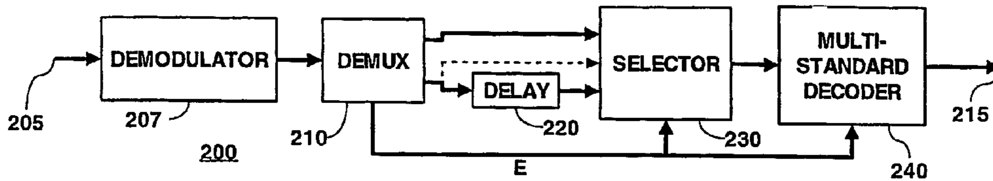
Fig. 2 Receiver
