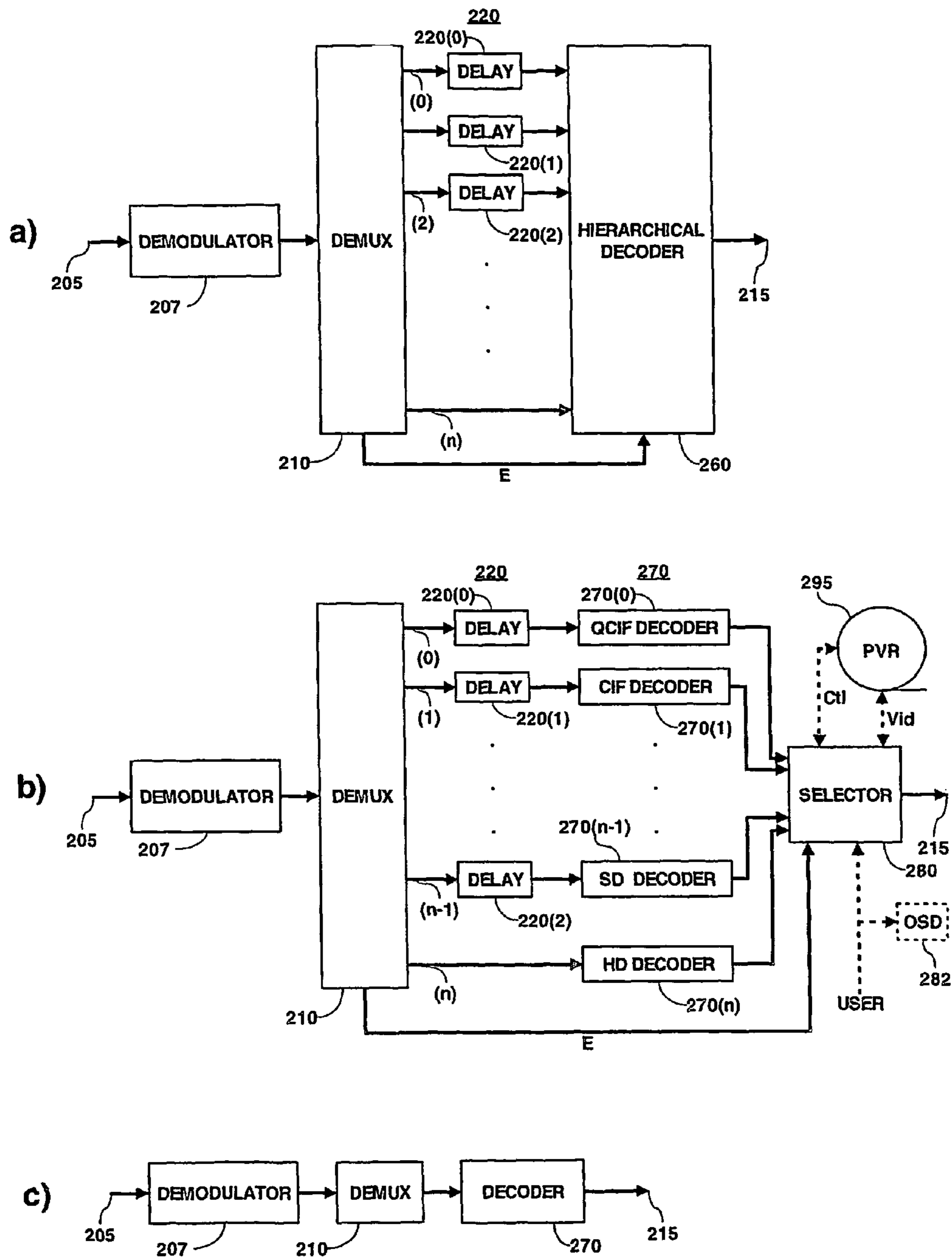
Fig. 10 Multiresolution receiver
