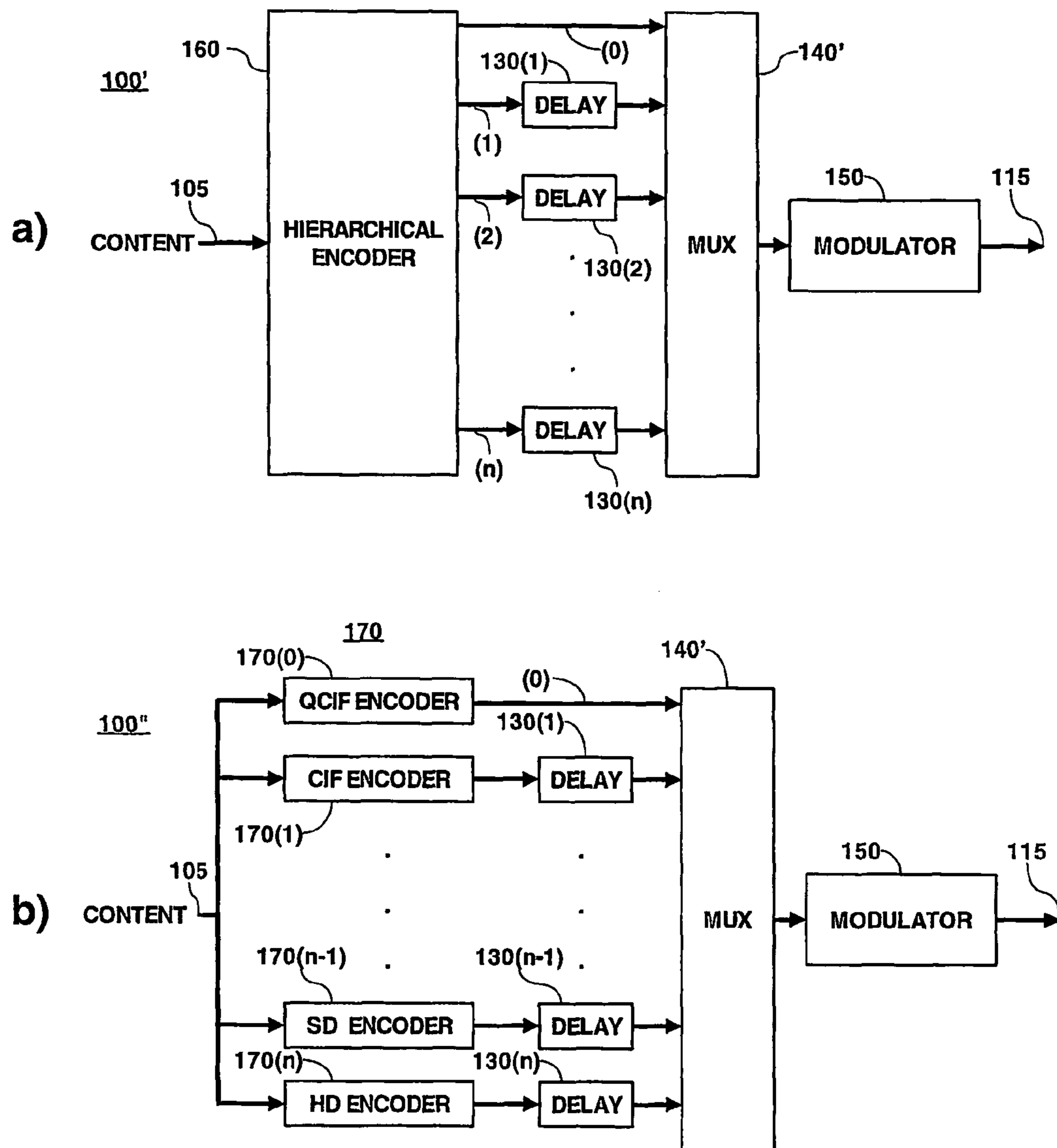
Fig. 9 Multiresolution transmitter
