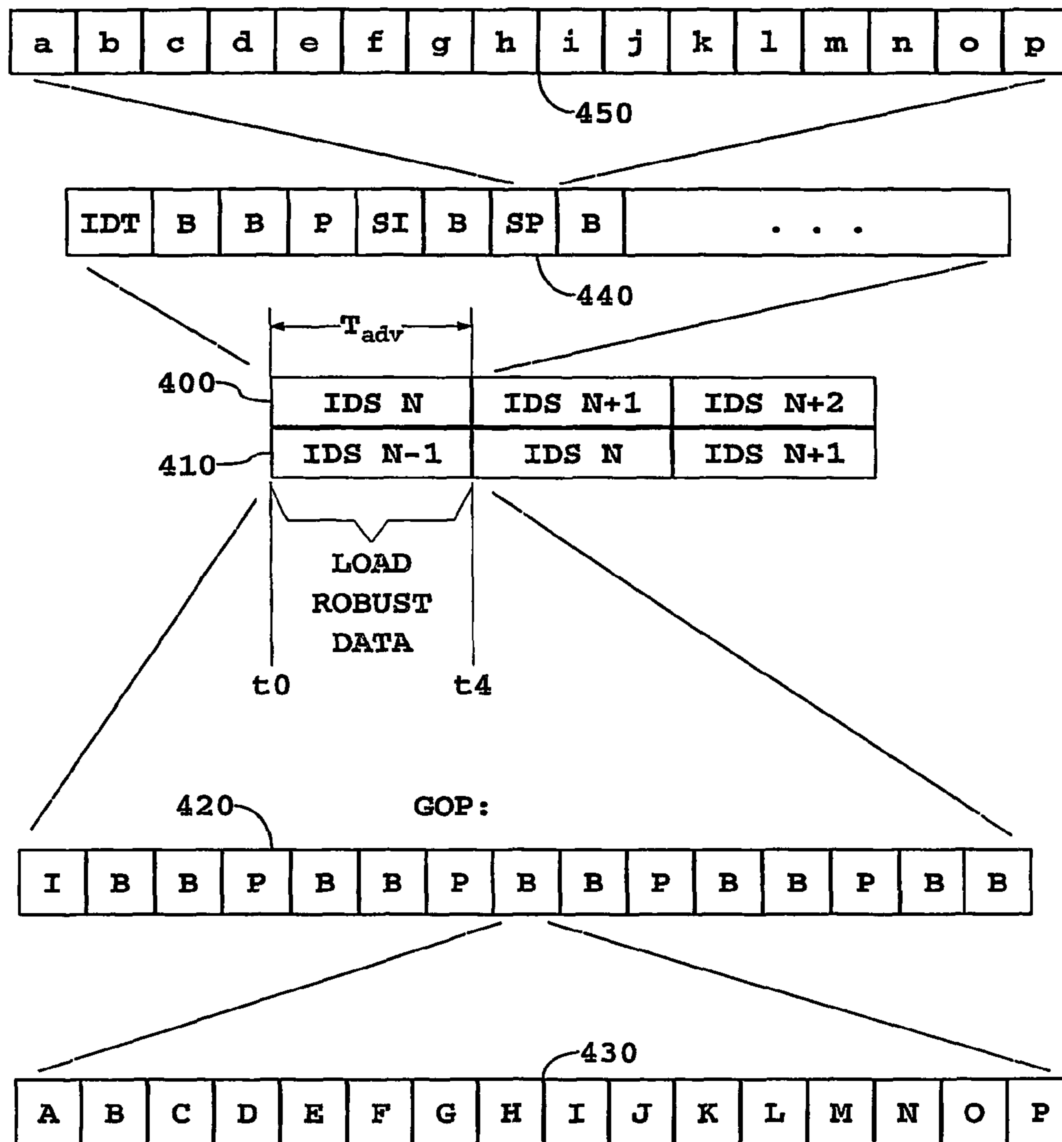
Fig. 4 GOP Streams
