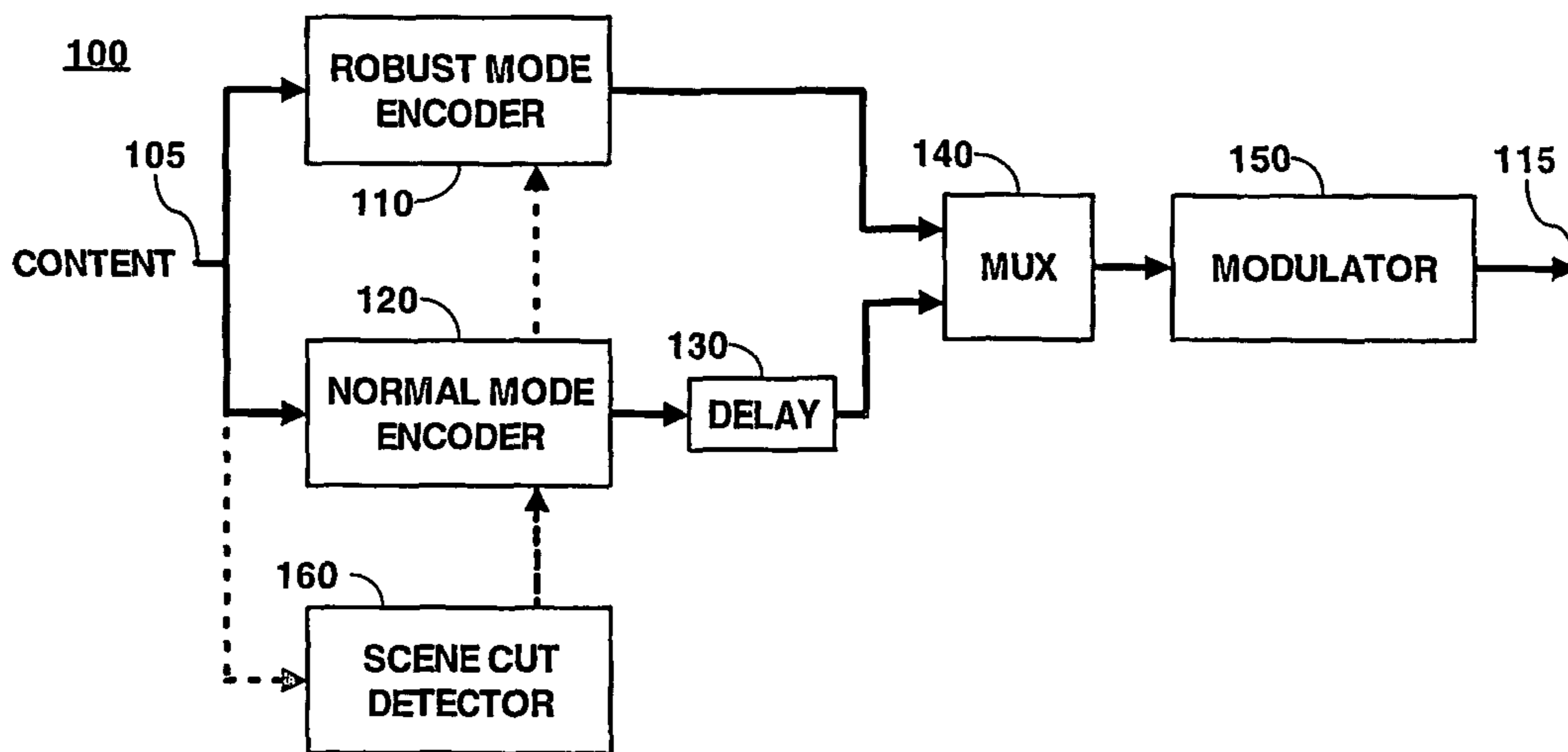
Fig. 1 Transmitter
