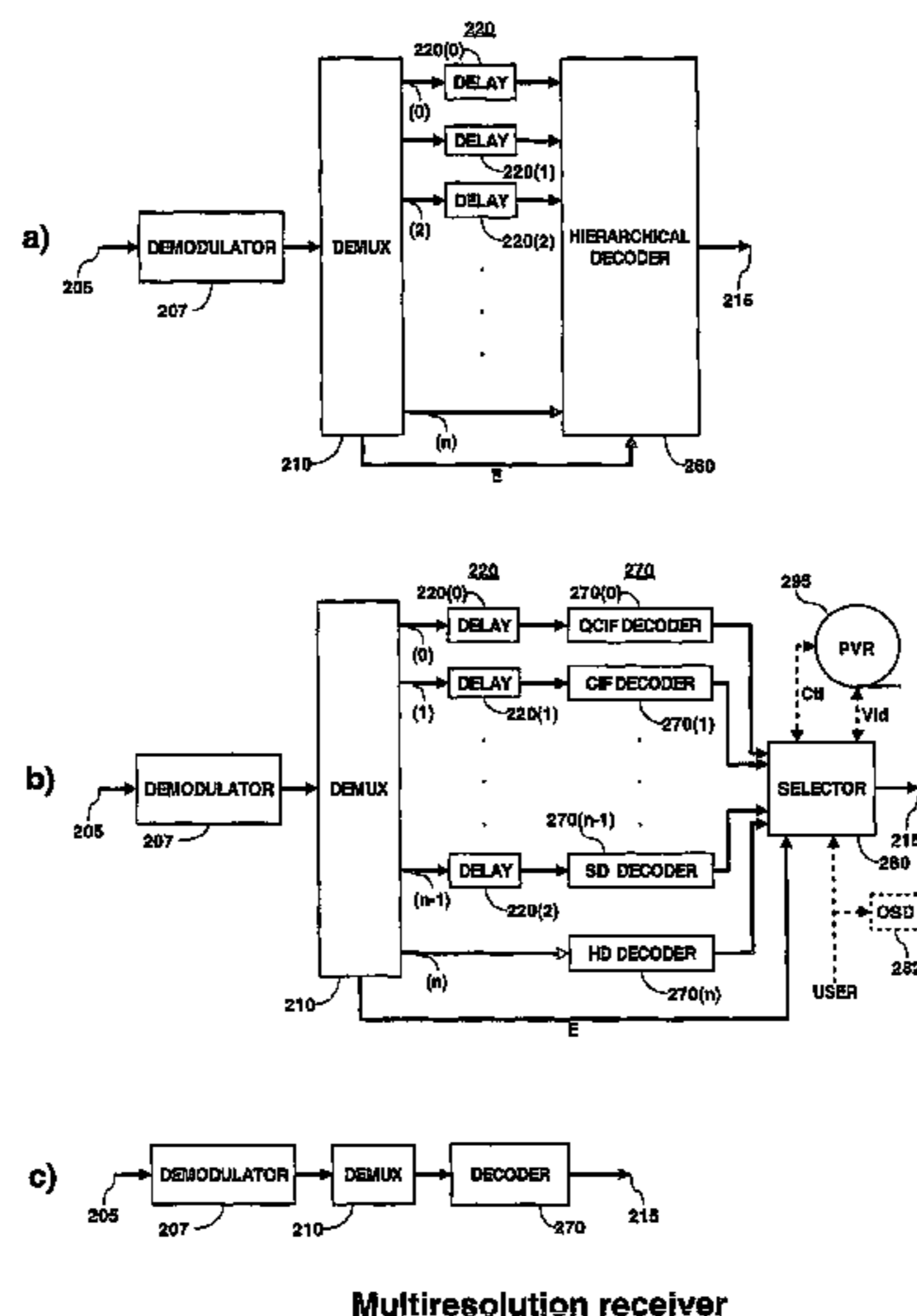
Multiresolution receiver
