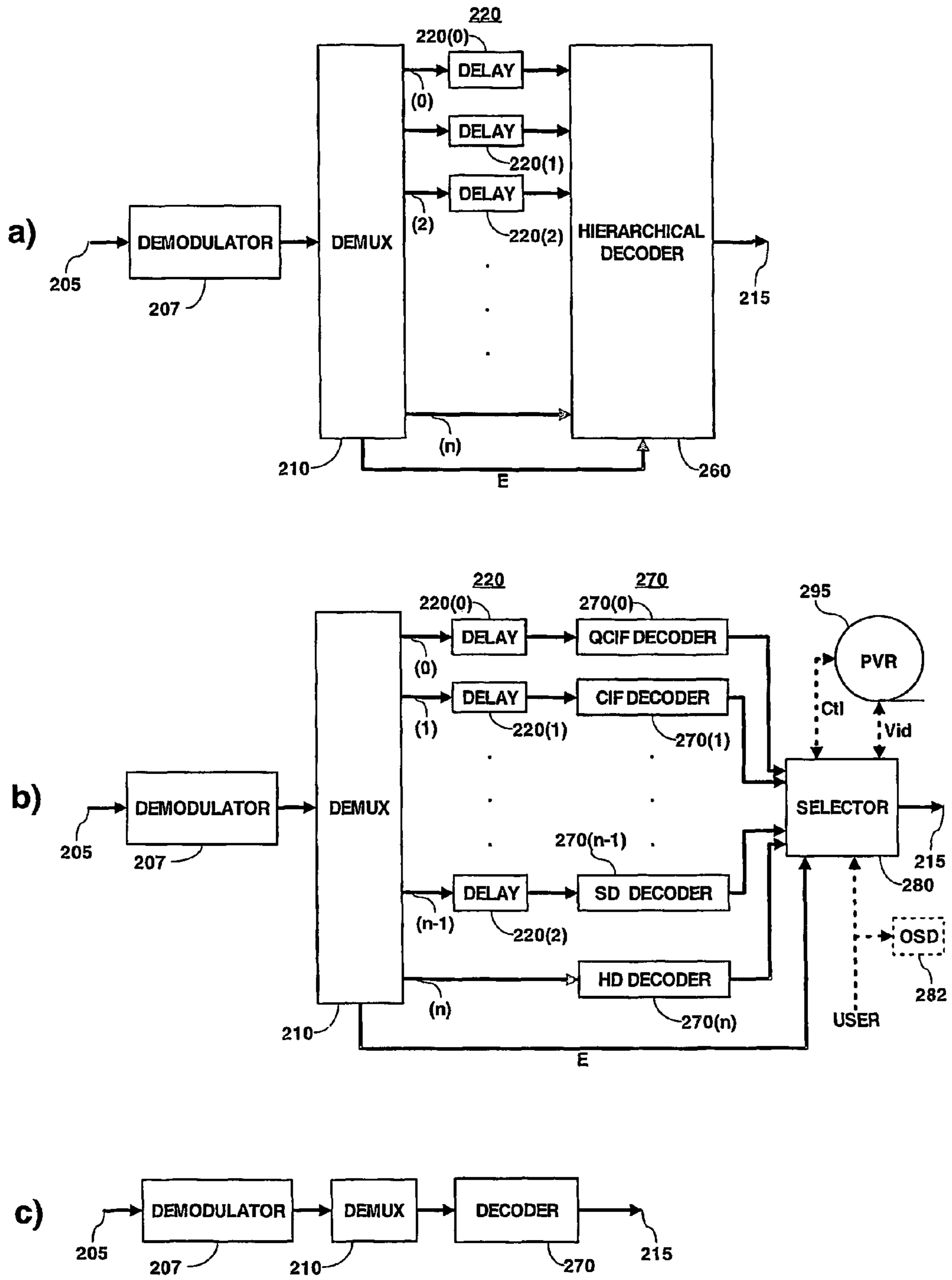
Fig. 10 Multiresolution receiver
