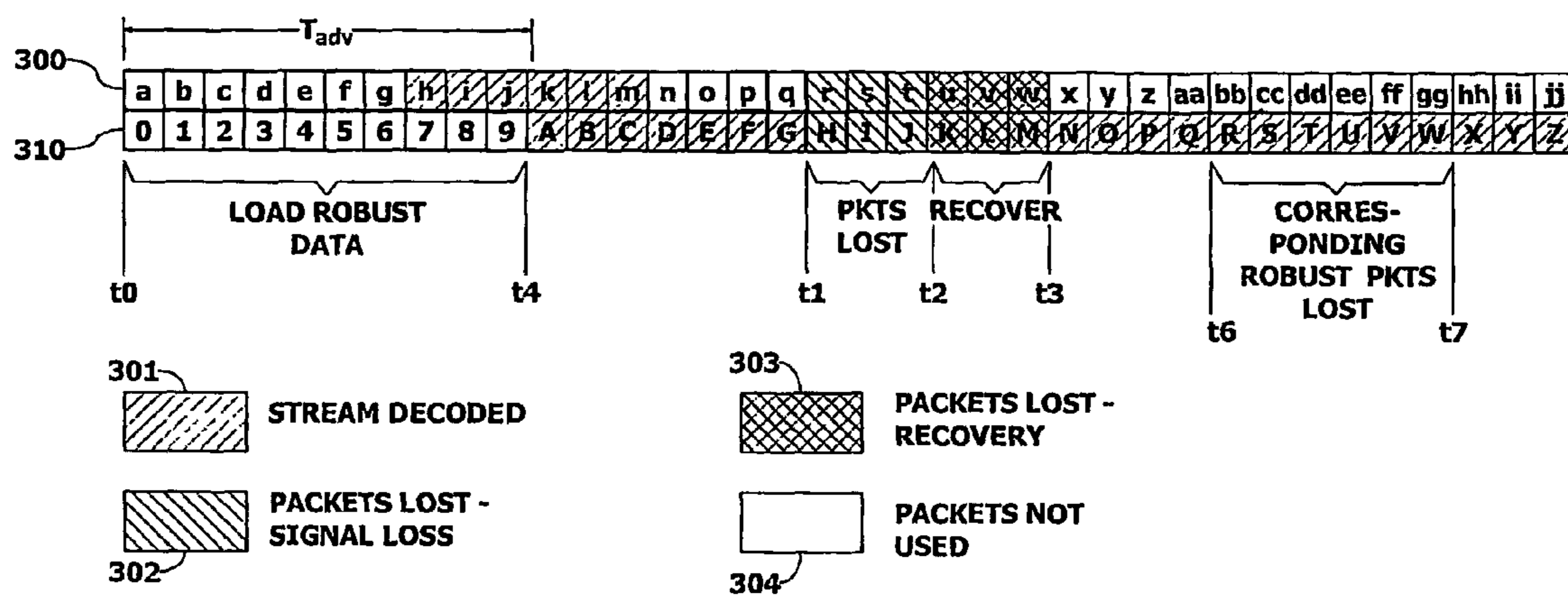
Fig. 3 Packet Streams
