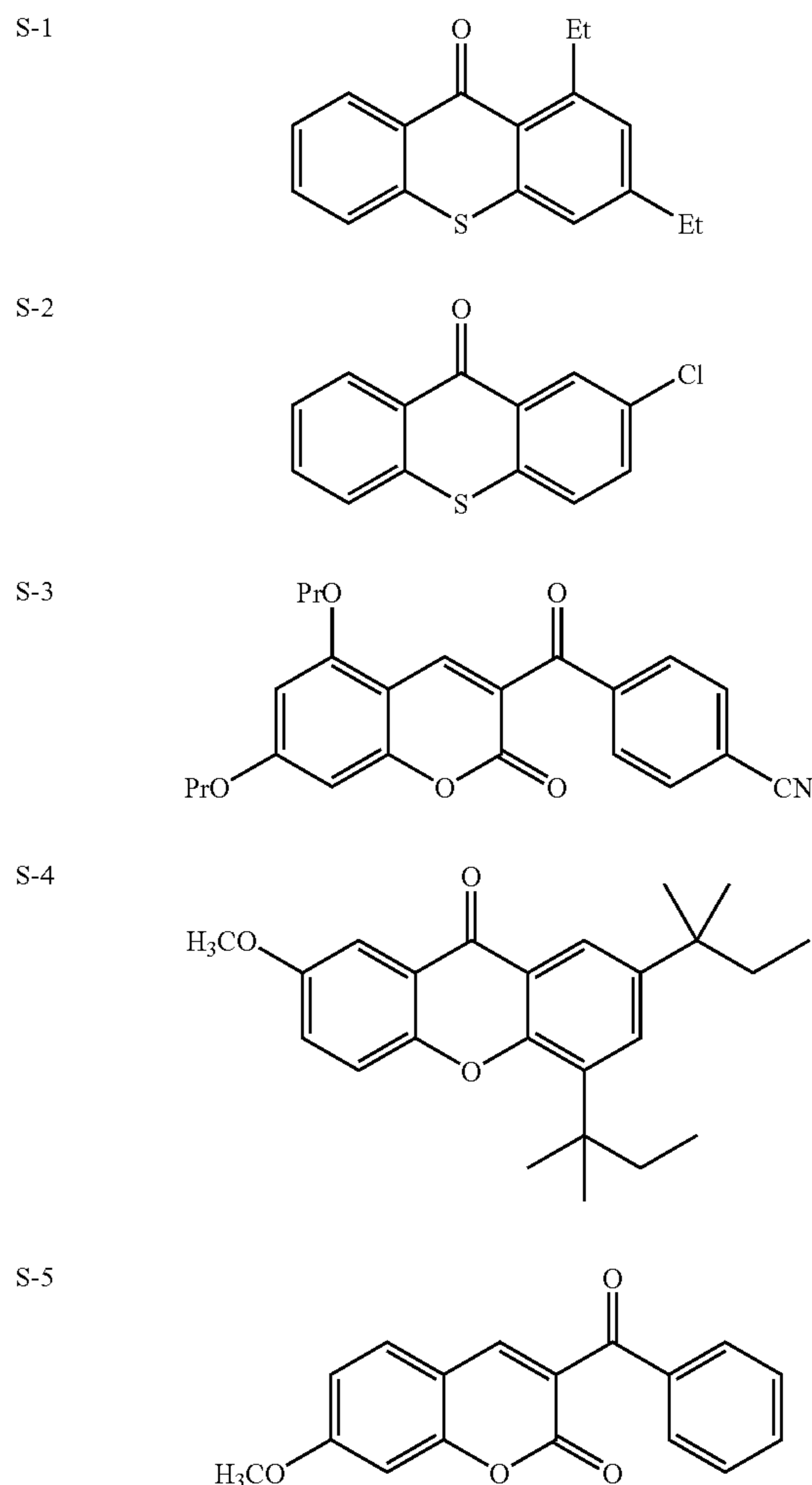
Triplet Sensitizers
