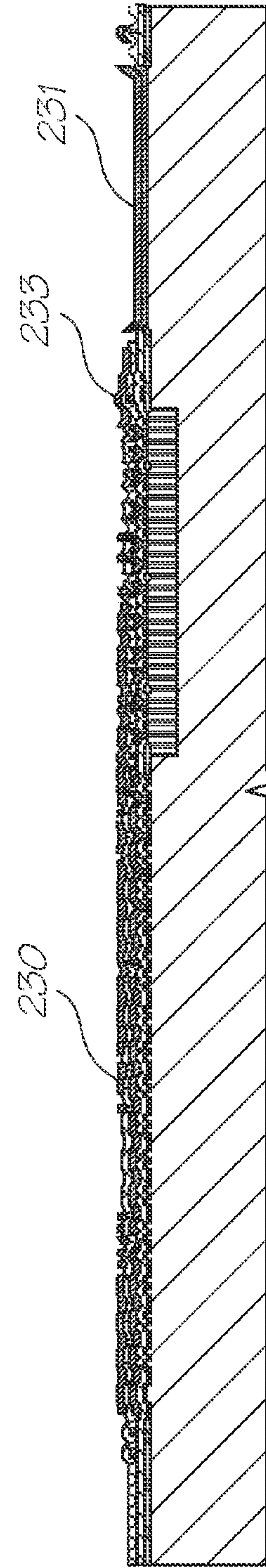
Deposit metal 2
