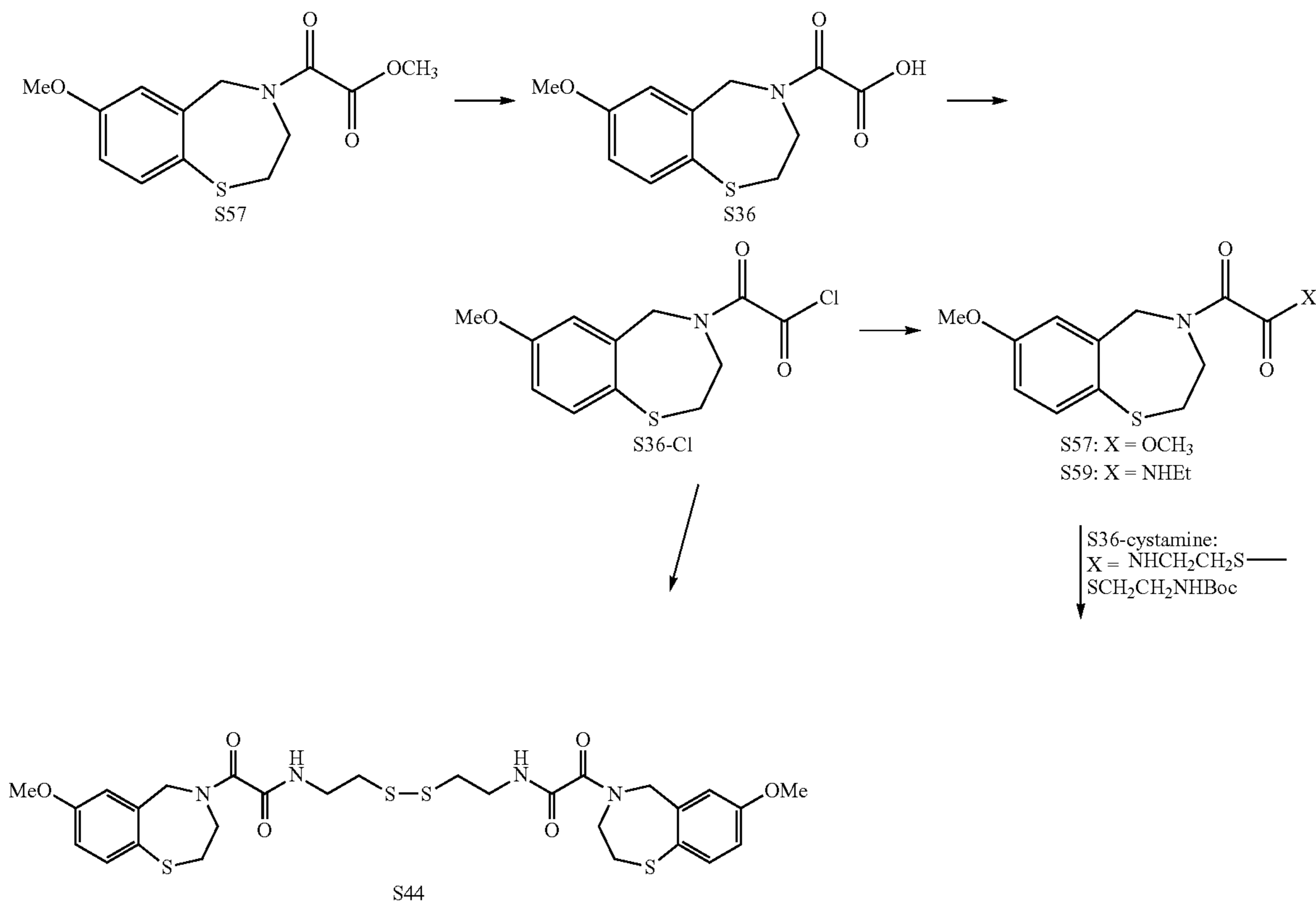
Scheme 8: Synthesis of S36, S43, S44, S45, S57, S59
