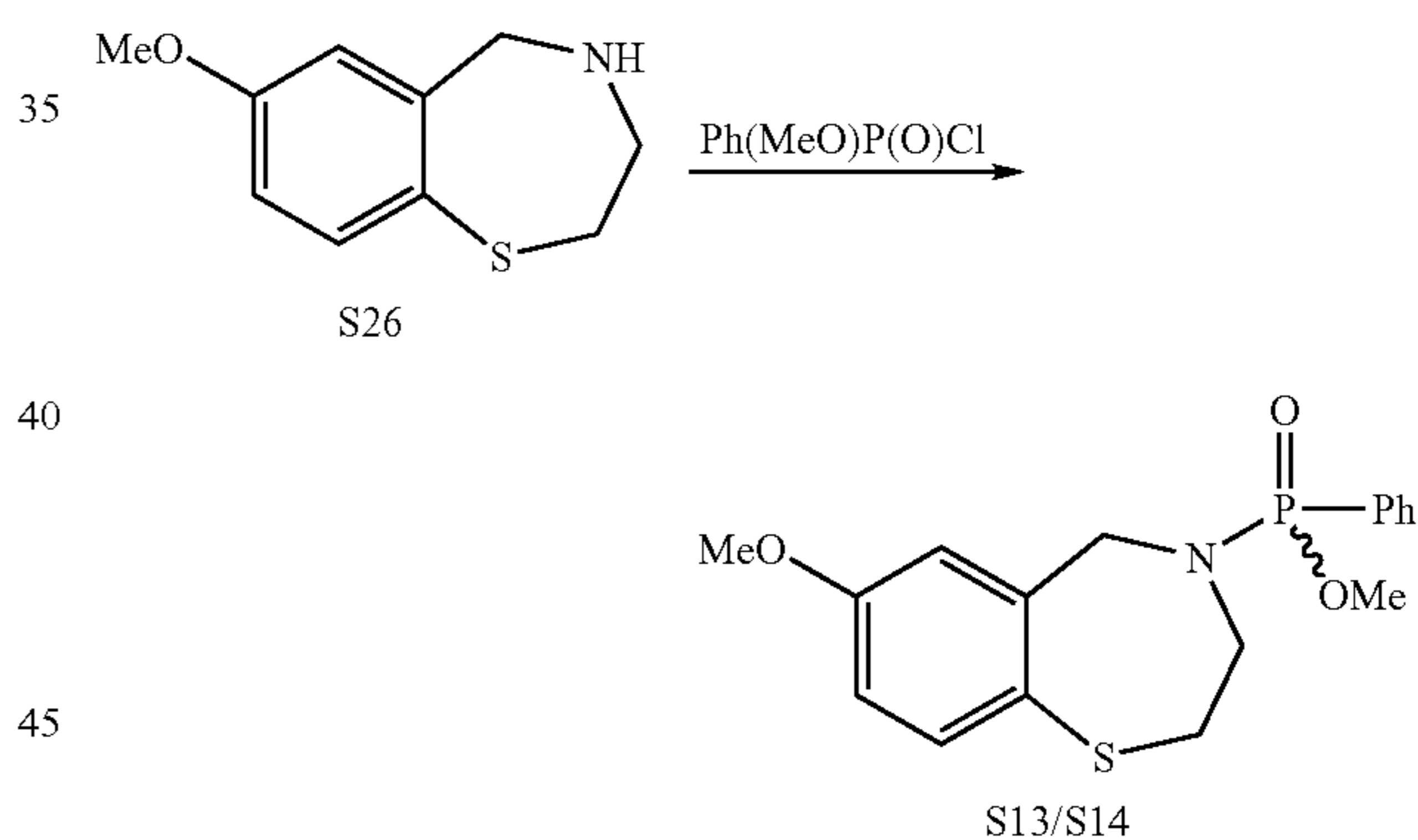
Scheme 5: Synthesis of S13 and S14
