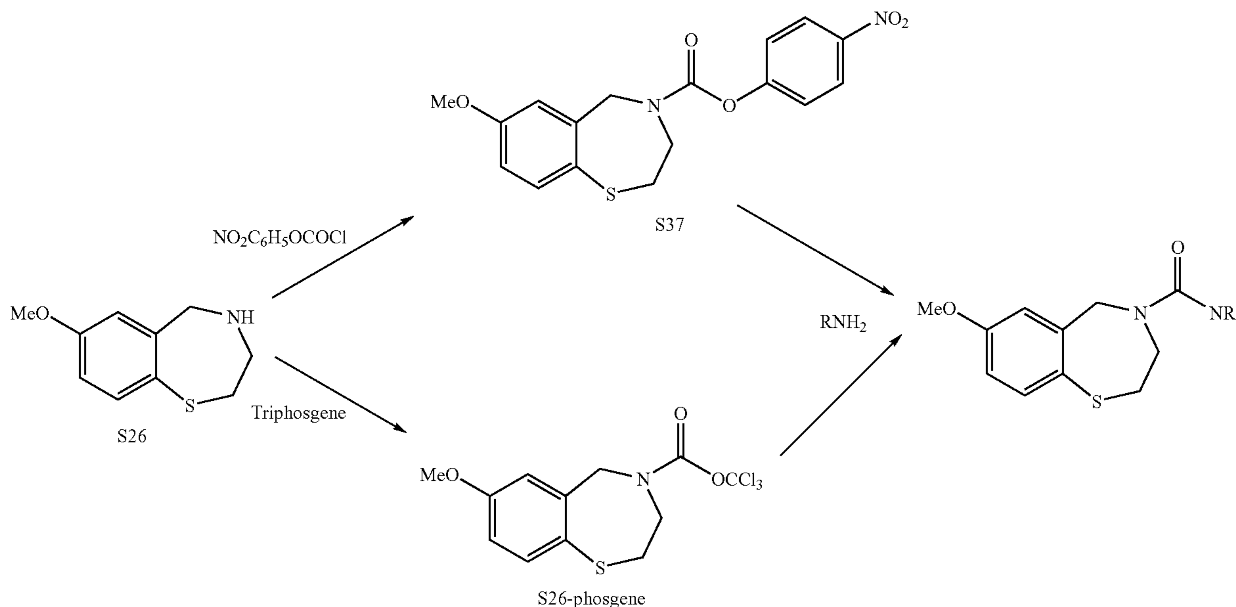
Scheme 9: Synthesis of urea-based analogs S6, S46–S53, S64, S66, S67
