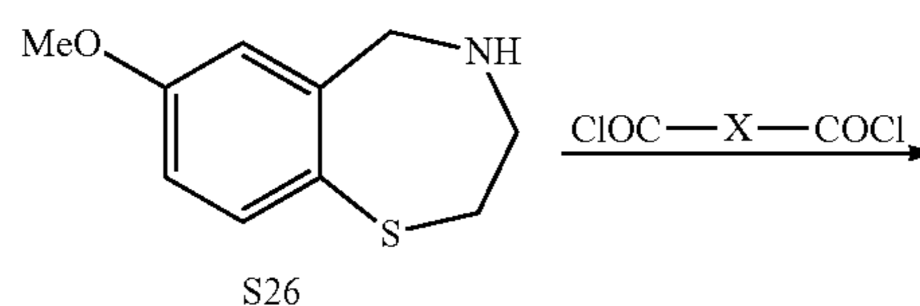
Scheme 6: Synthesis of S19, S22
