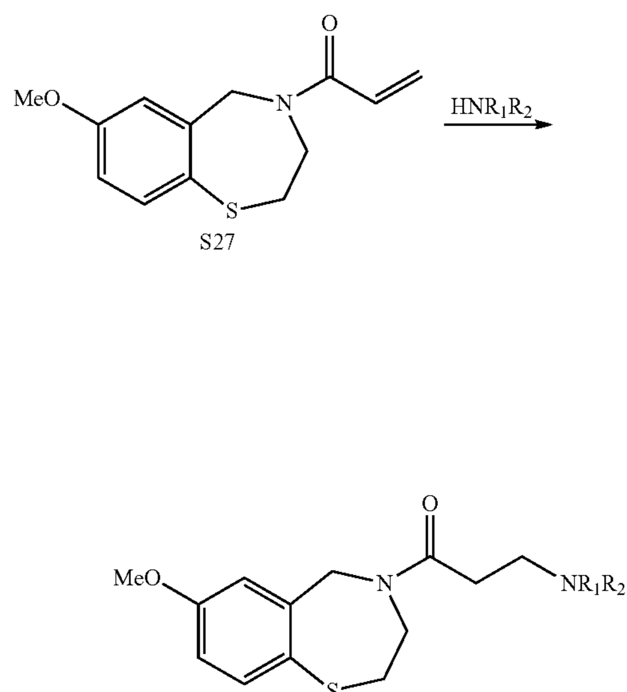
Scheme 10: Synthesis of S55, S56, S58, S60 - S63
