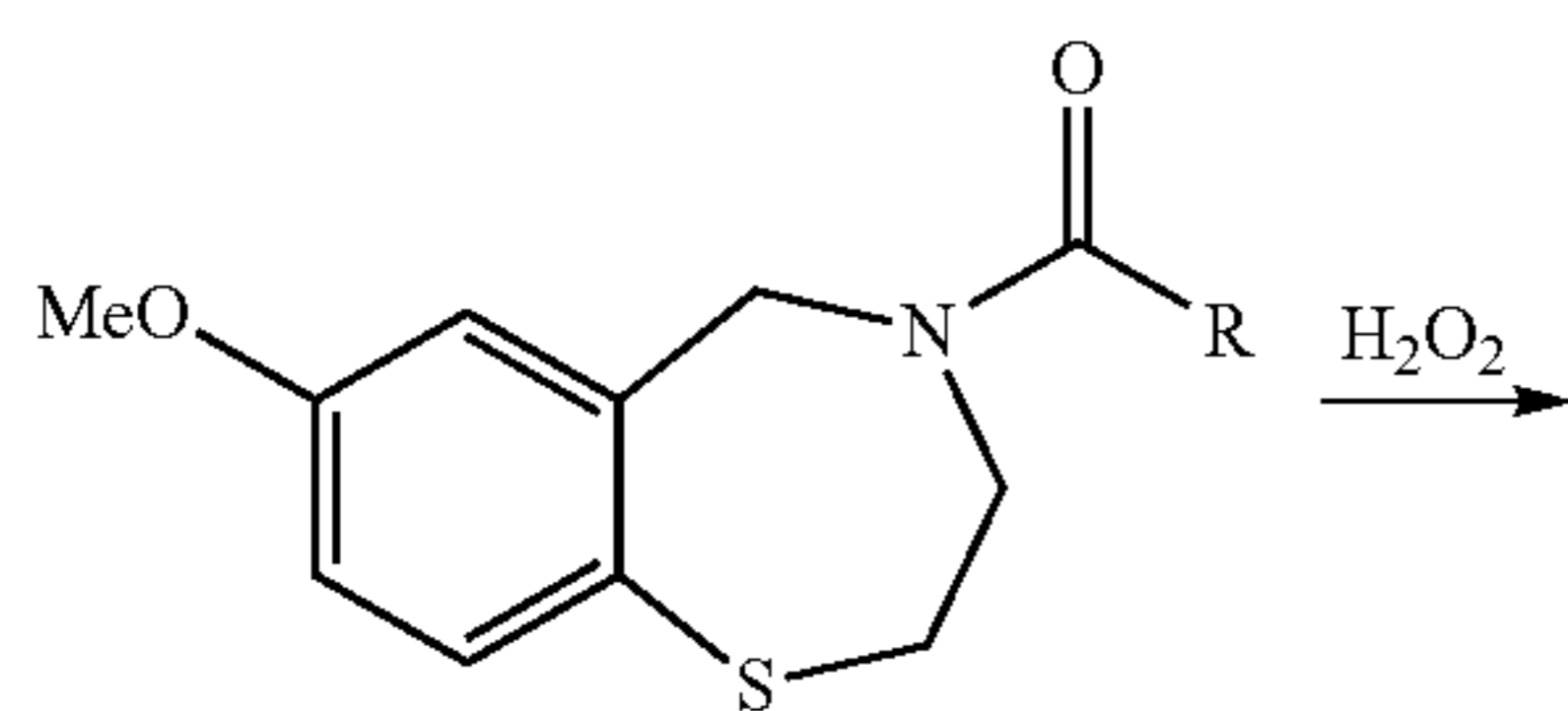
Scheme 7: Synthesis of S20 and S23
