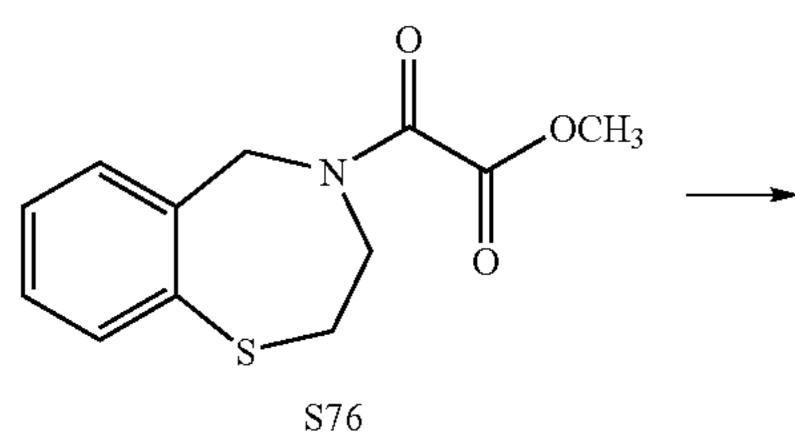
Scheme 12: Synthesis of S76-S81
