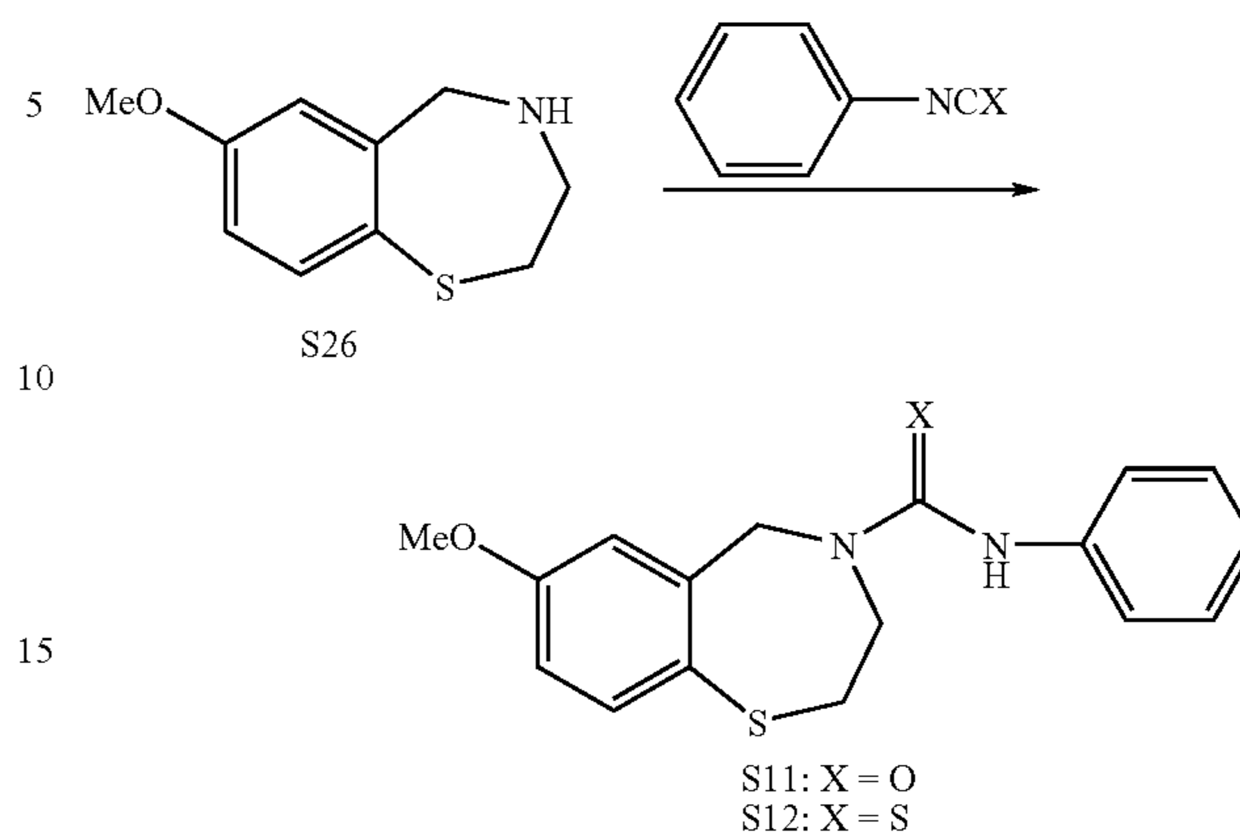
Scheme 4: Synthesis of S11 and S12
