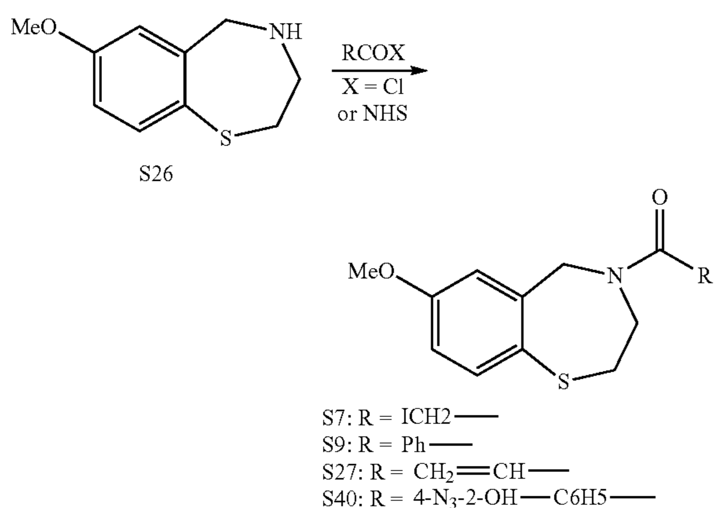
Scheme 3: Synthesis of S7, S9 and S40
