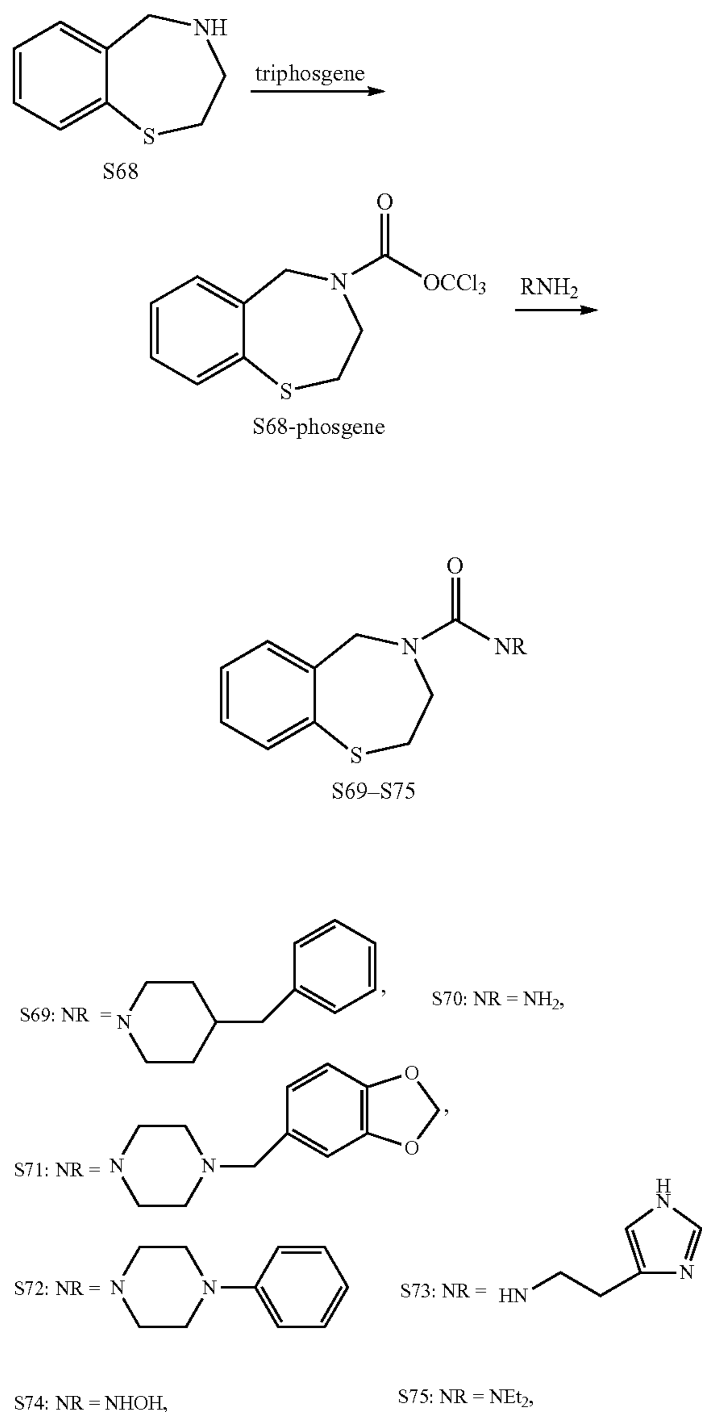
Scheme 11: Synthesis of urea-based analogs S69-S75
