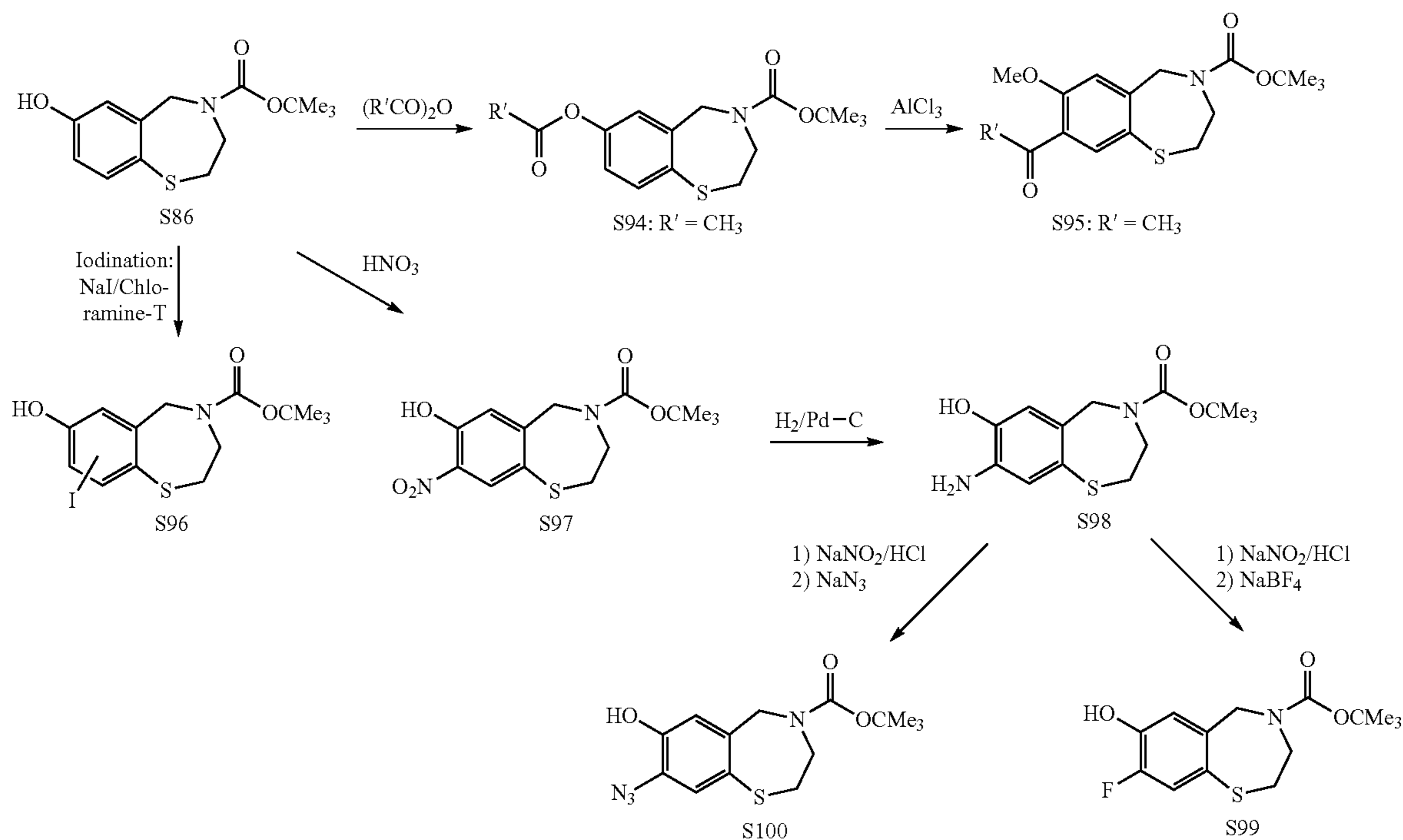
Scheme 15: Synthesis of S94-S100
