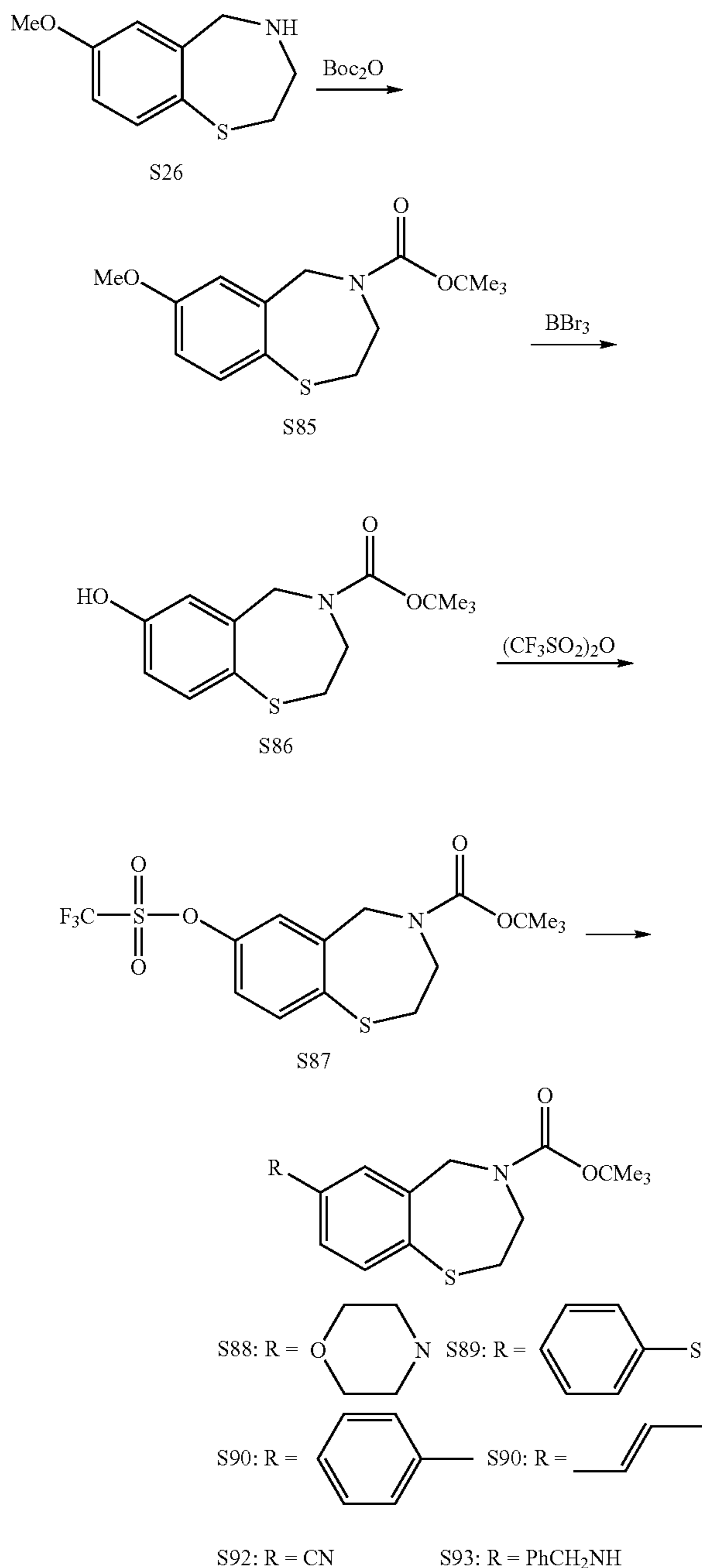
Scheme 14: Synthesis of S88-S93
