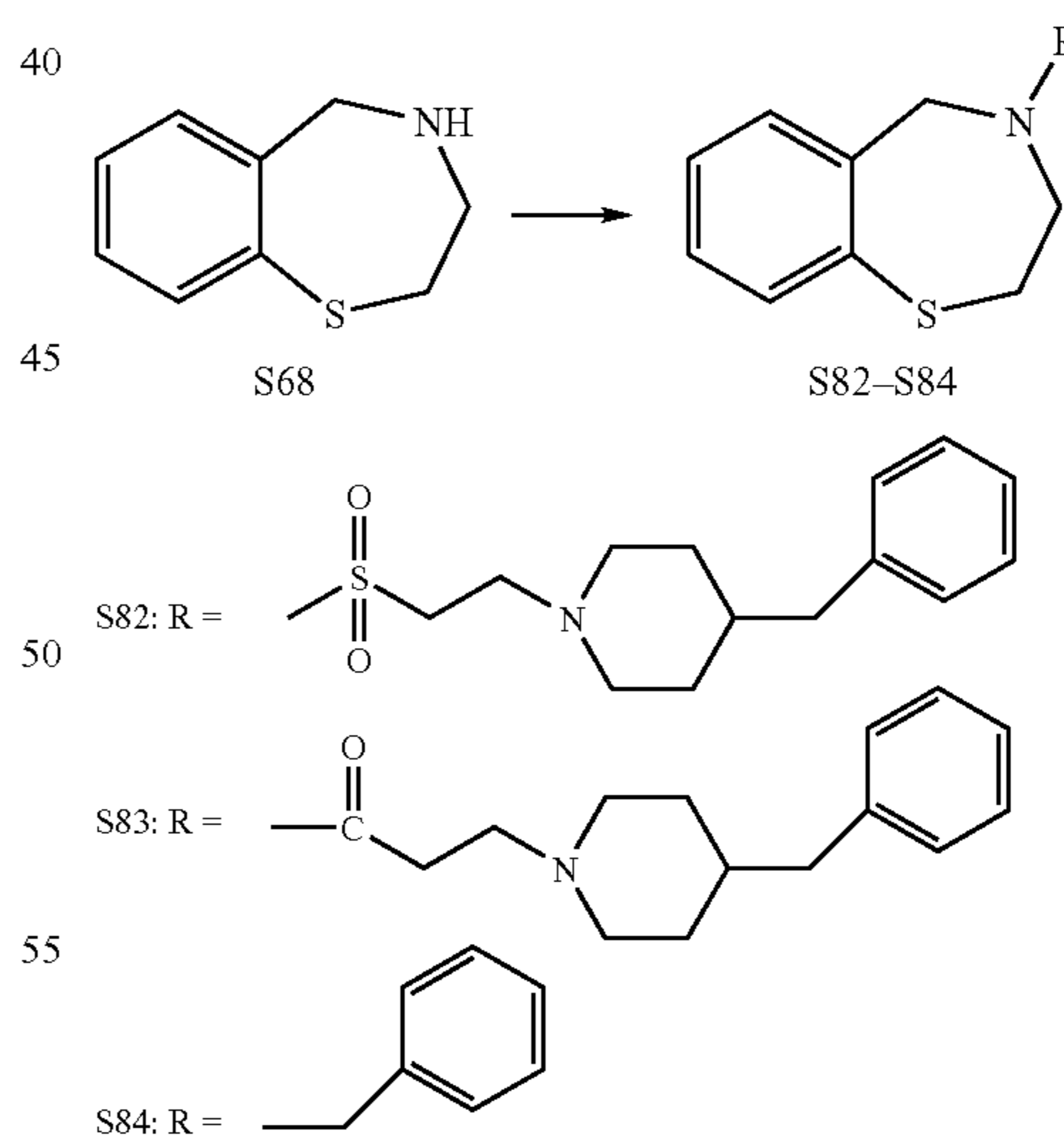
Scheme 13: Synthesis of S82-S84
