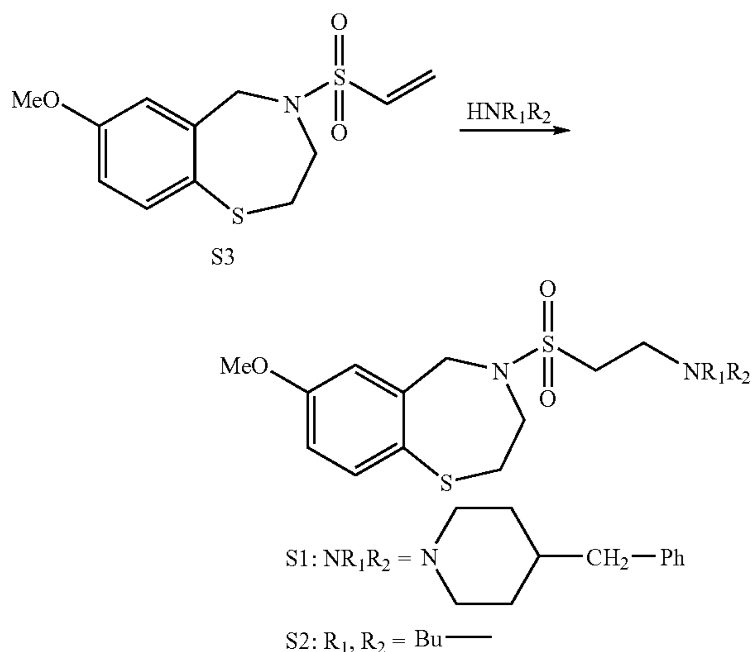
Scheme 2: Synthesis of S1 and S2
