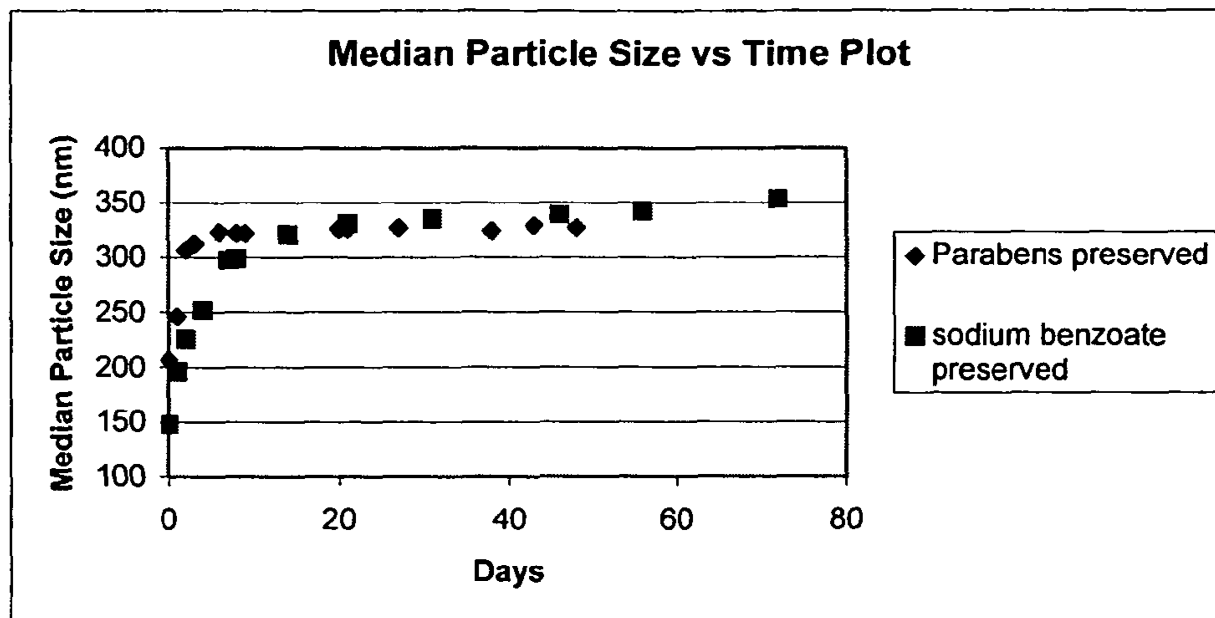
FIGURE 2. Curing of Parabens Preserved and Sodium Benzoate Preserved Ganaxalone Particles at Ambient Temperature: Parabens Preserved Ganaxalone Particles Become Fully Stable in 5-7 Days While the Benzoate Preserved Particles Take About 3 Weeks To Become Fully Stable (D50 Were Unsonicated).
