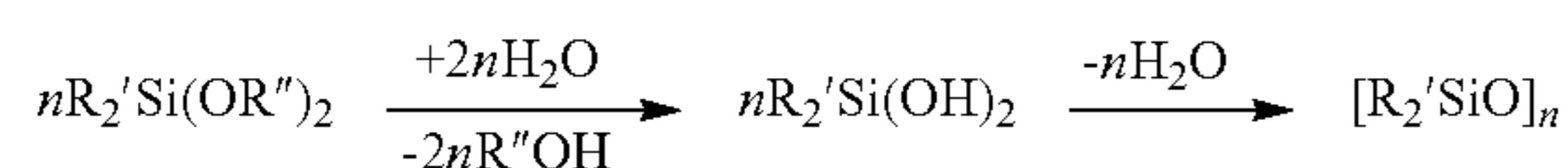
Reaction formula (12)
