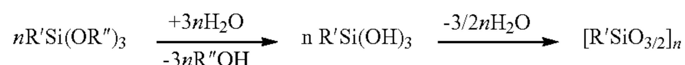
Reaction formula (12)
