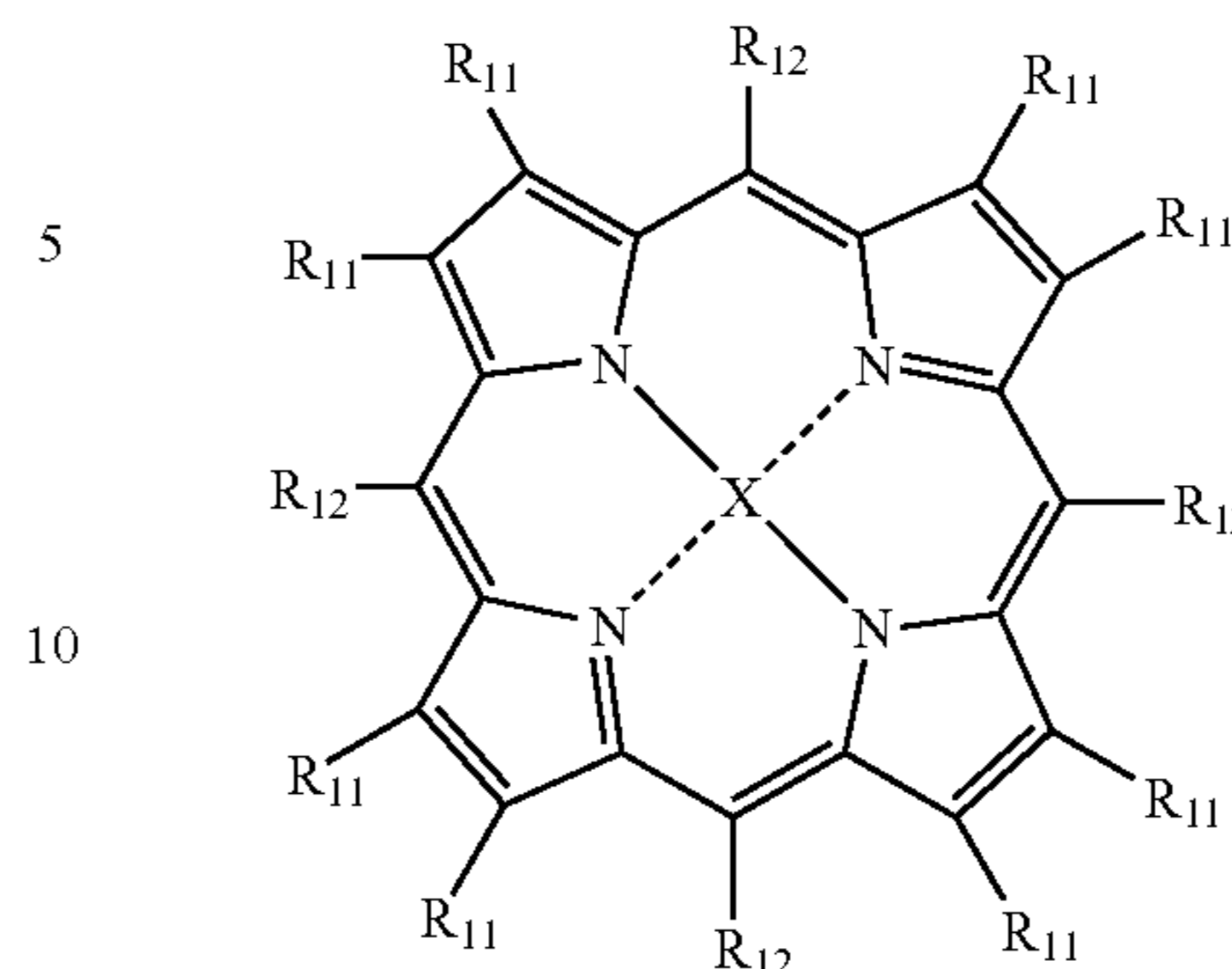
General formula (1)
