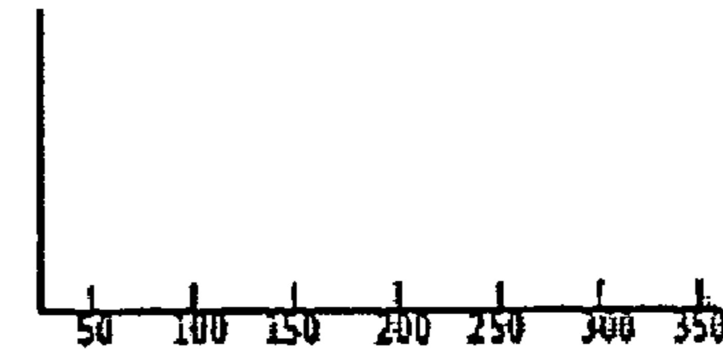
RBC HISTOGRAM
