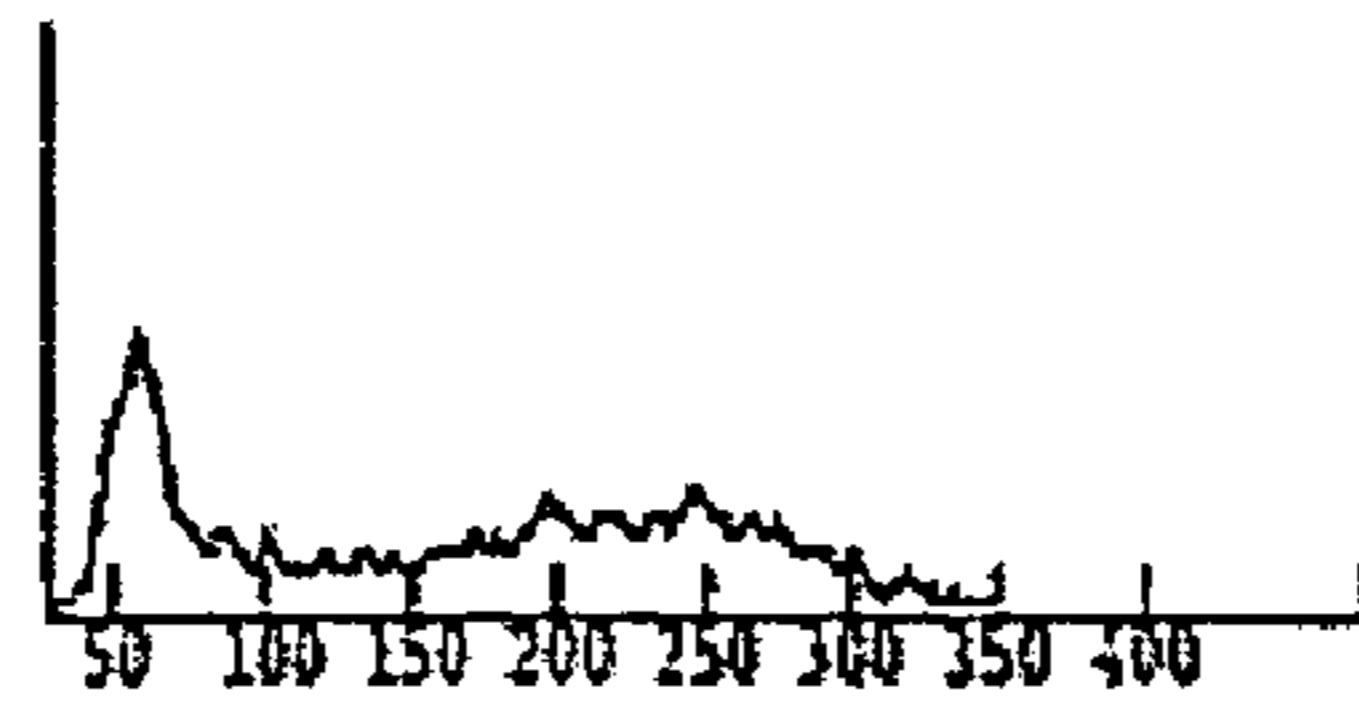
WBC HISTOGRAM
