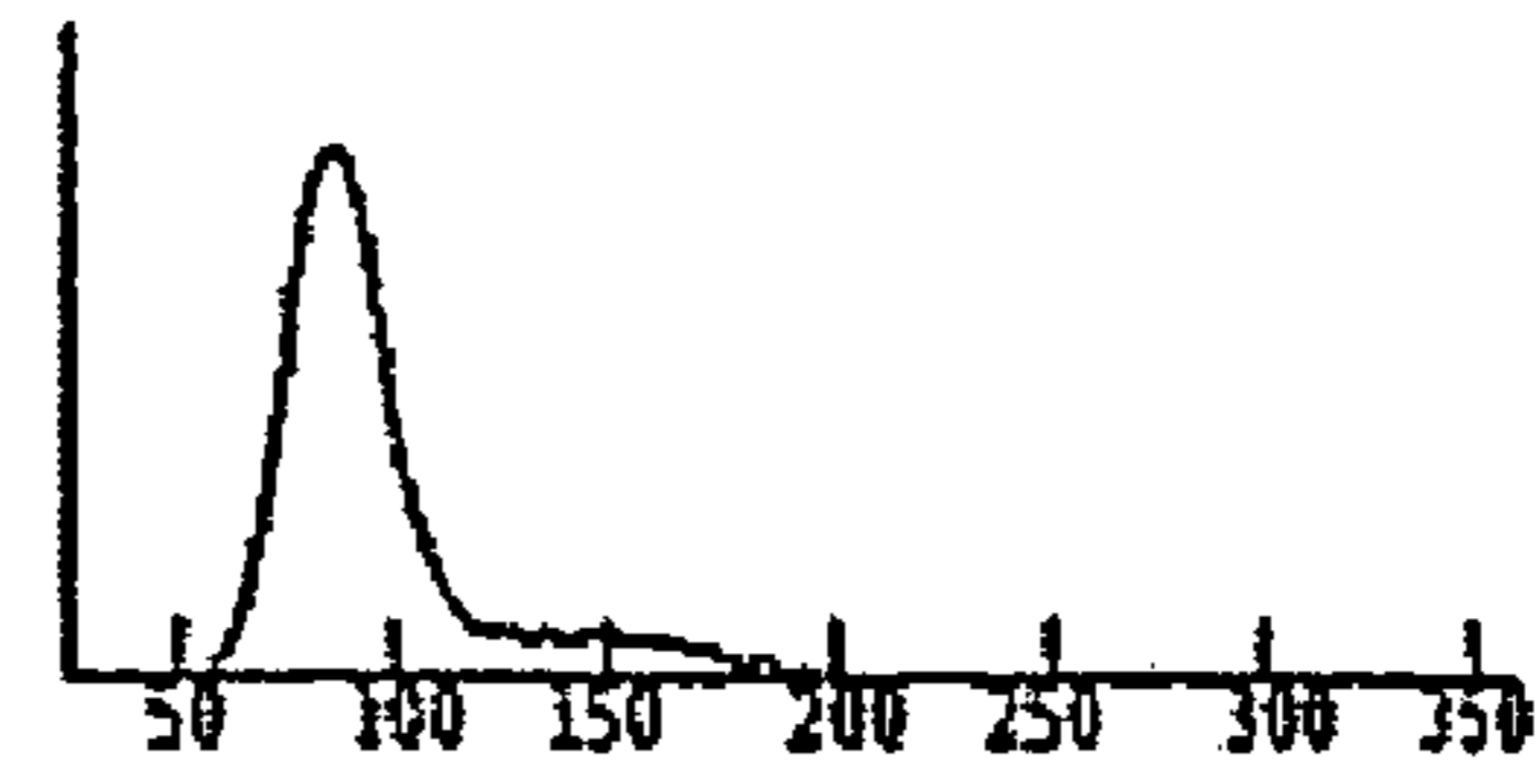
RBC HISTOGRAM
