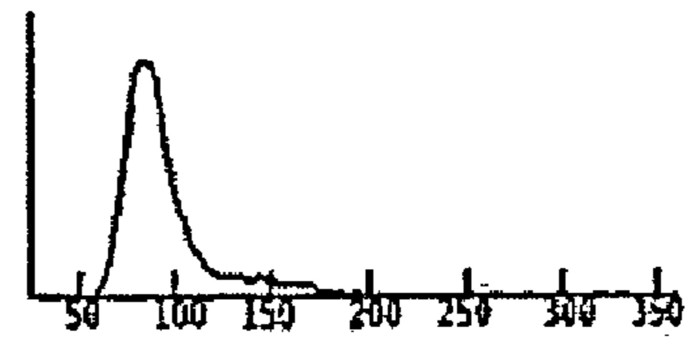
RBC HISTOGRAM
