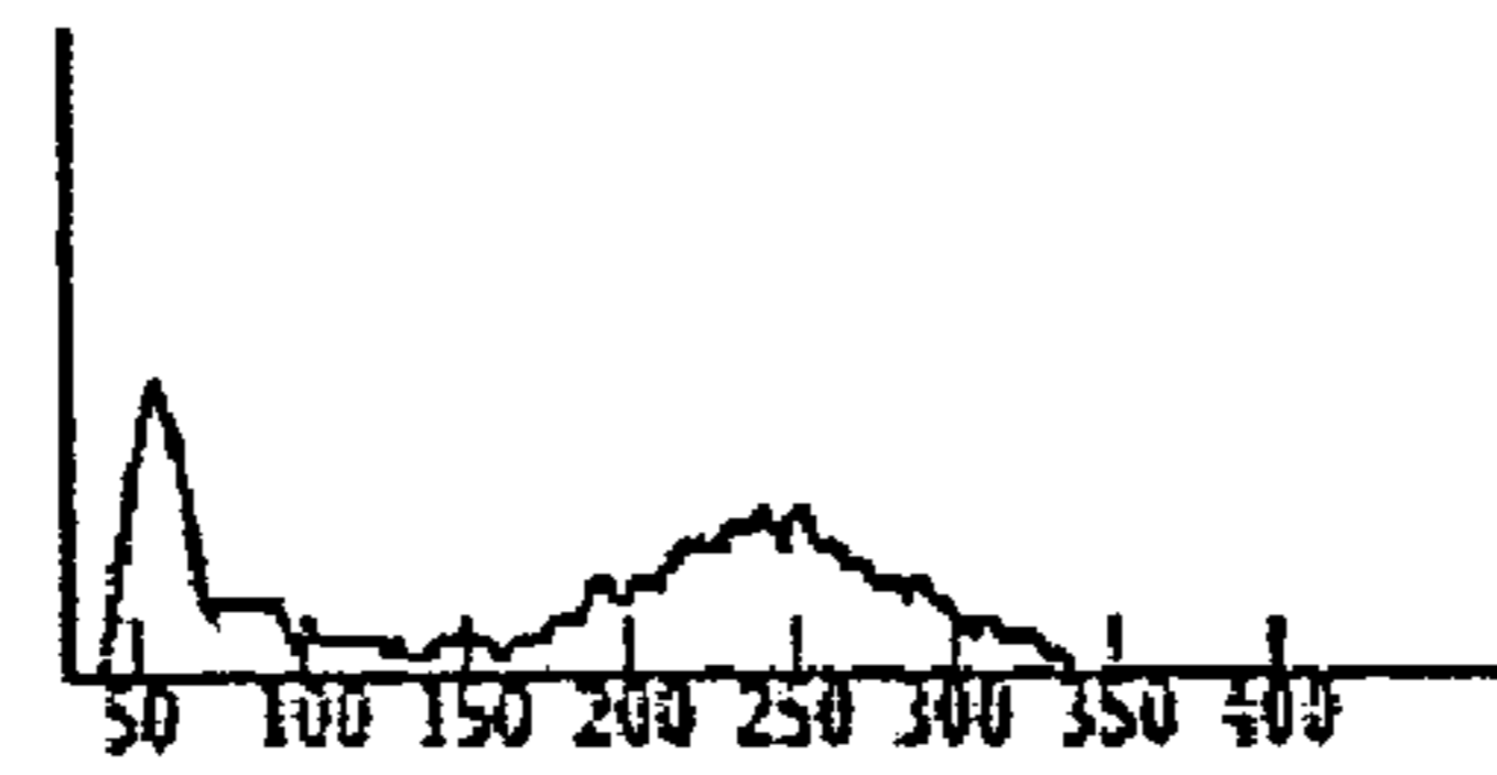
WBC HISTOGRAM
